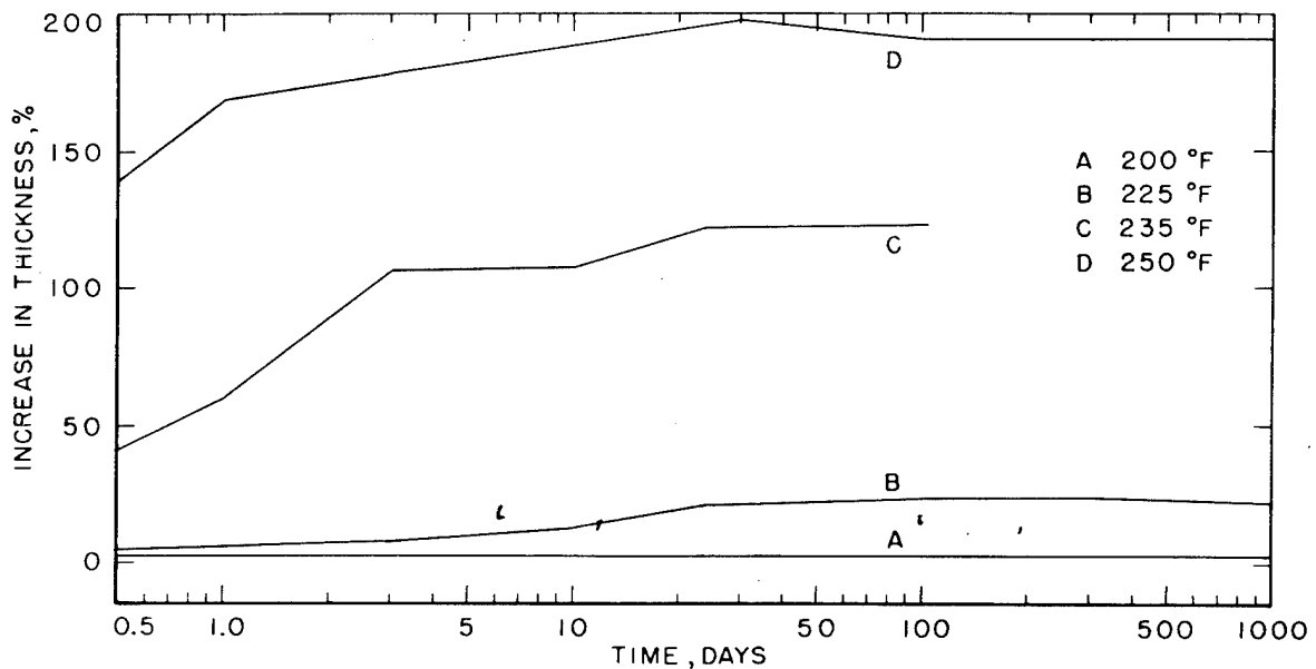
Figure 4.3-67 - Effect of Duration of Exposure at Various Temperatures on the Increase in Thickness due to Thermal Relaxation of 0.125-Inch-Thick MIL-P-25690 Material Stretched 75 Percent
