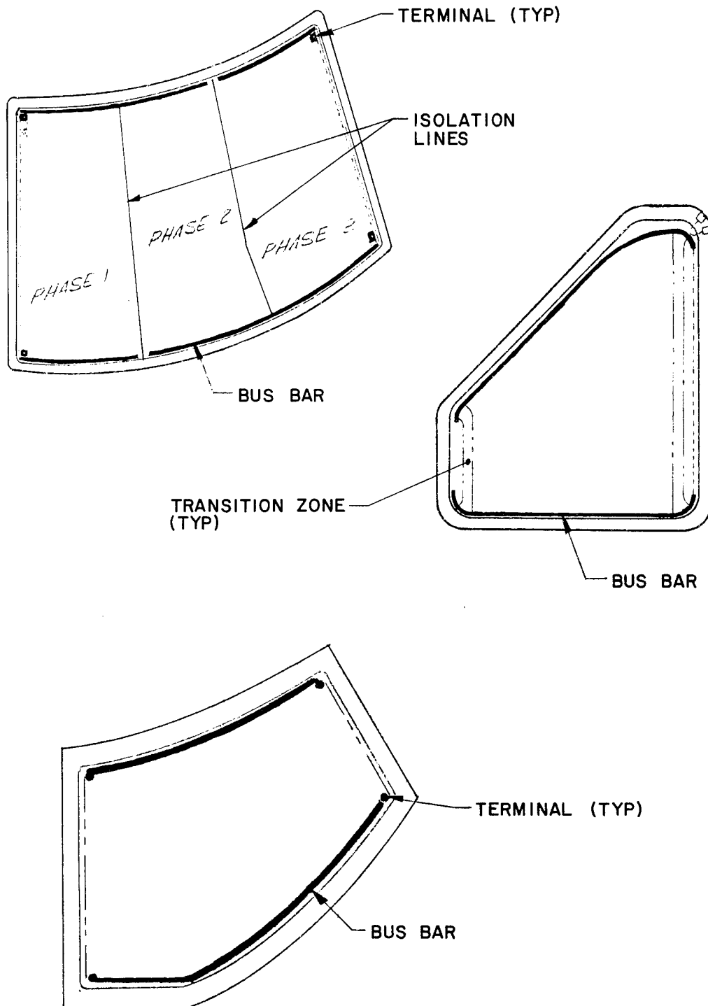
Figure 6.2-6 - Flat Pattern of Typical Electrically Heated Panels
