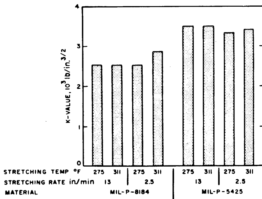
Figure 4.3-58 - Effect of Stretching Temperature and Stretching Rate on the K-Value of MIL-P-5425 and MIL-P-8184 Materials Tested at Room Temperature
