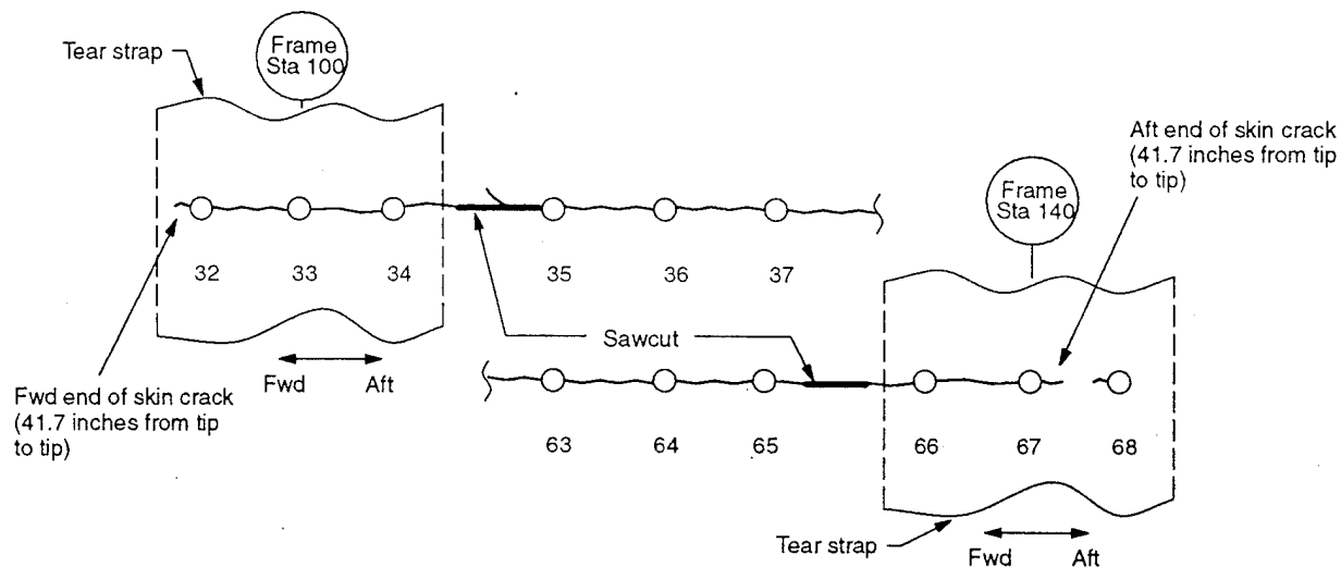
Figure 42. Crack Configuration Prior to Panel Failure
