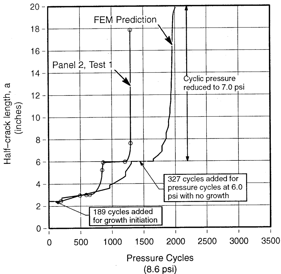
Figure 66. Crack Growth Prediction vs. Test Results for FAA 2, Test 1 (Varied MSD)
