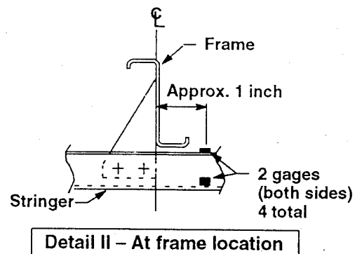
Figure C-3. Stiffener Strain Gage Locations of Panel FAA 1, Tests 1, 2 and FAA 2, Test 1
