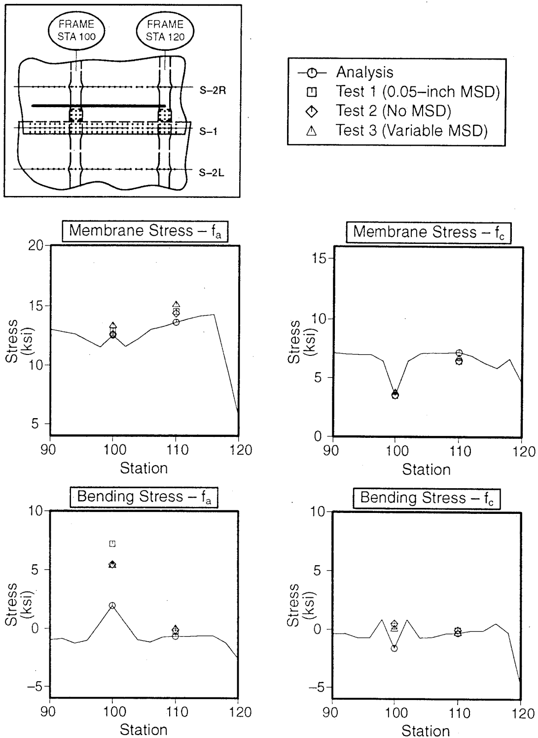
Figure E-8. Skin Stress Correlation at Stringer S-1 + 4.6 Inches for a Test Panel Containing a 5-Inch Sawcut
