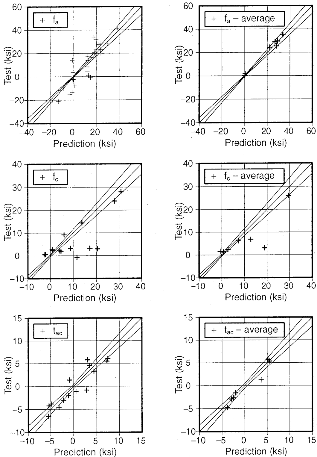
Figure E-3. Test / Analysis Strain Gage Correlation for FAA 1, Test 2. The Finite Element Model Contains a 38-Inch Crack and the Test Panel Contains a 36.71-Inch Crack
