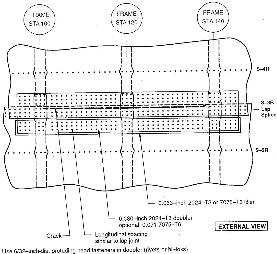
Figure 24. Panel Repair of FAA 1, Test 1
