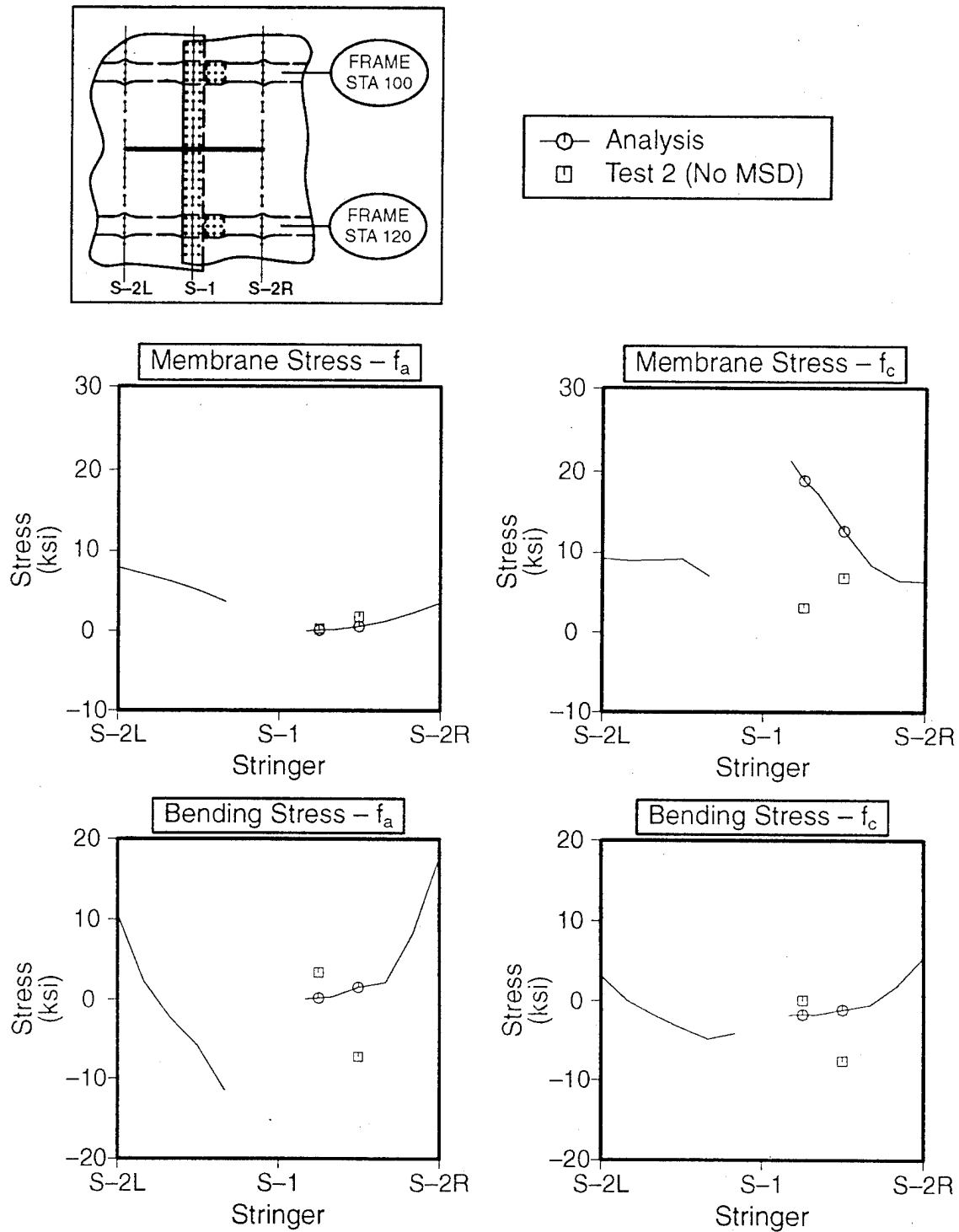
Figure E-24. Skin Stress Correlation at Station 110 for FAA 1, Test 2 (No MSD). Crack Length of 40 Inches With a Severed Central Frame
