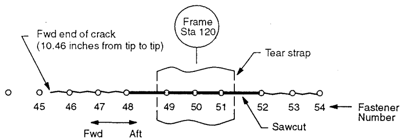
Figure 36. Crack Trajectory of Panel FAA 2, Test 1
