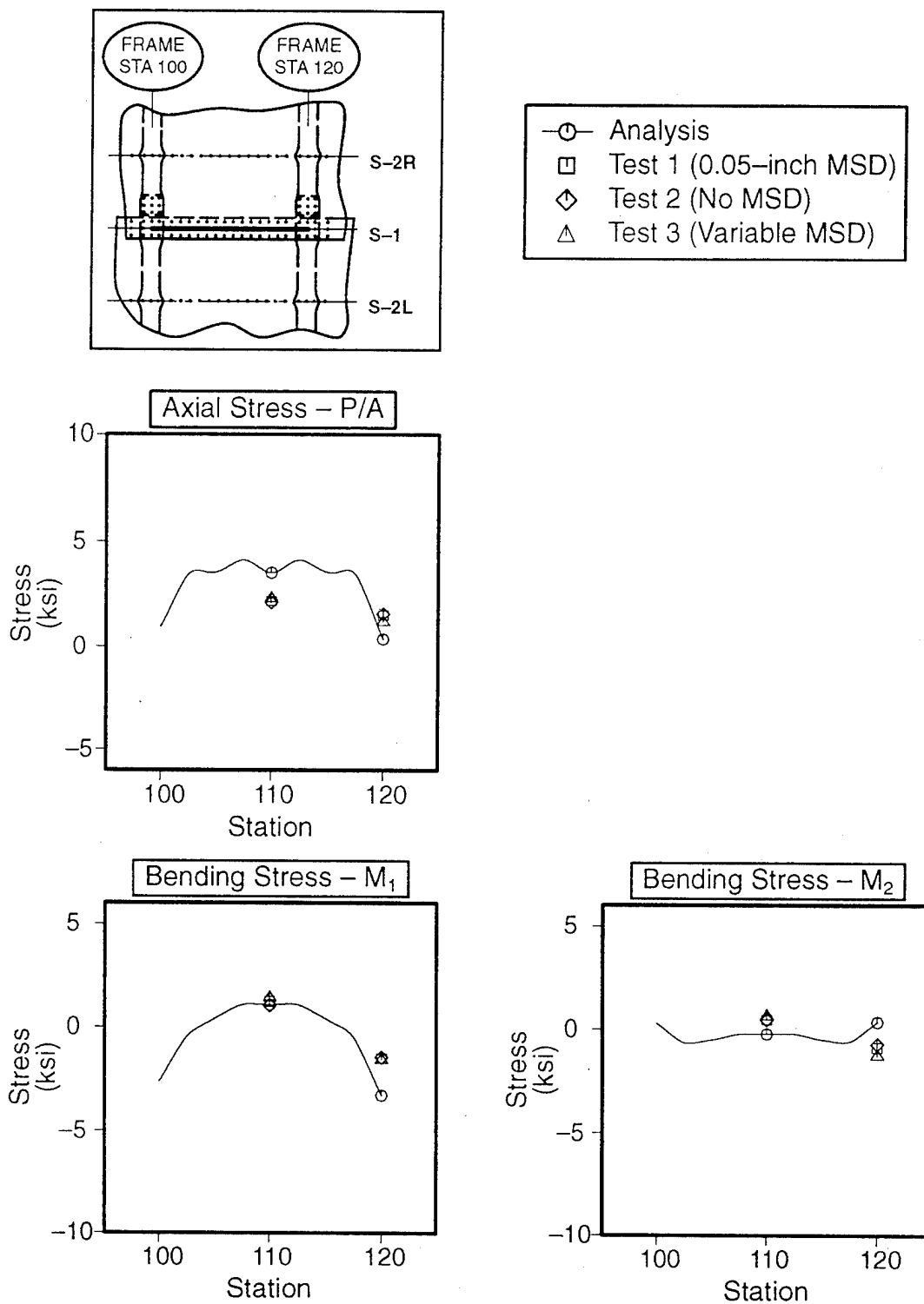
Figure 63. Stringer Stress Correlation at Stringer S-1 for an Intact Test Panel
