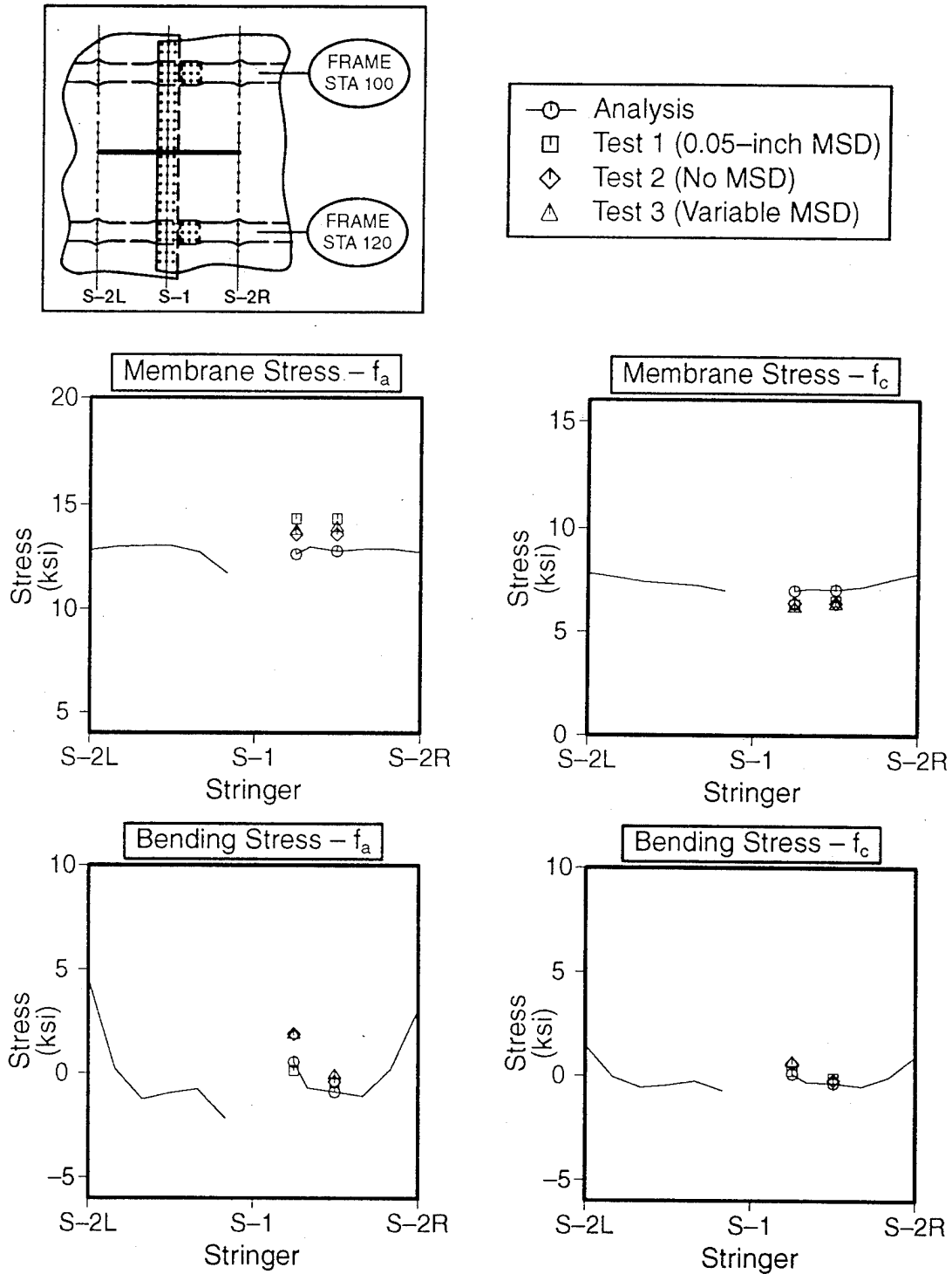
Figure 59. Skin Stress Correlation at Station 110 for an Intact Test Panel
