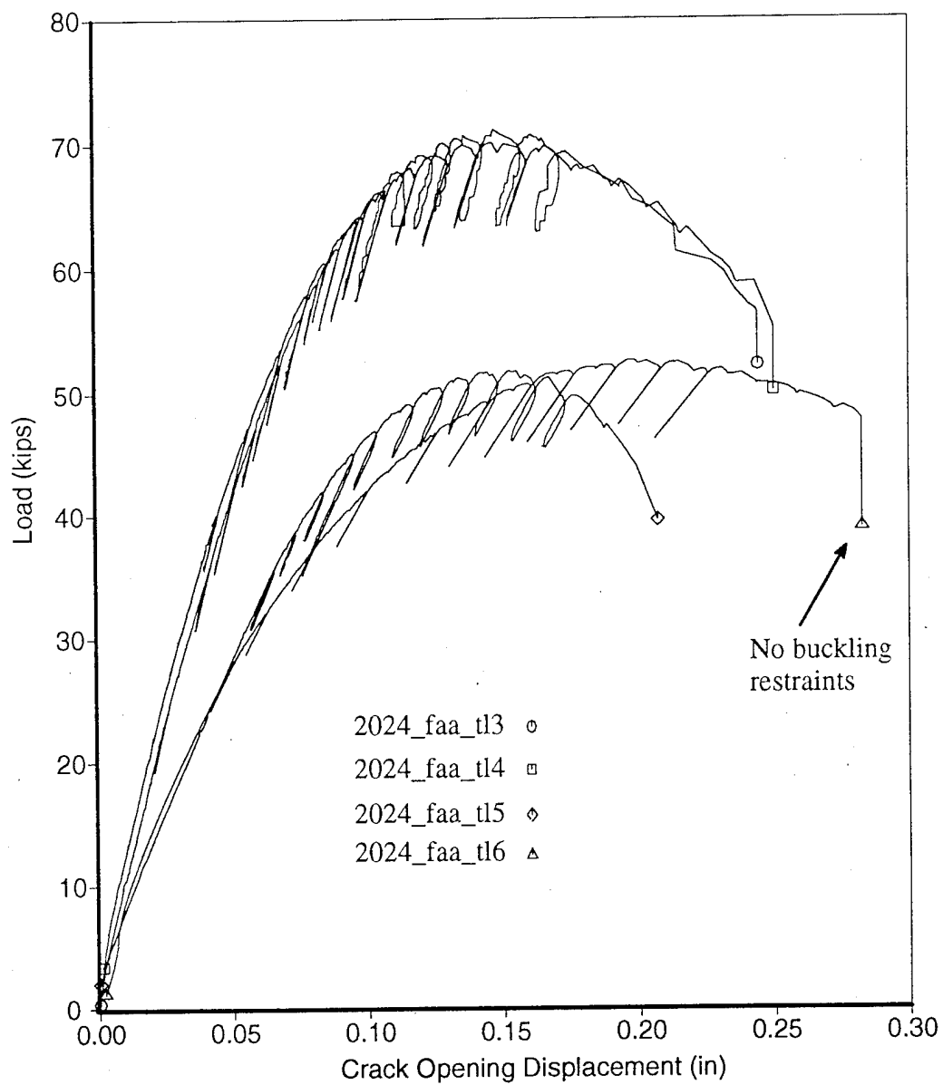
Figure B-1. Load Versus Crack Opening Displacement
