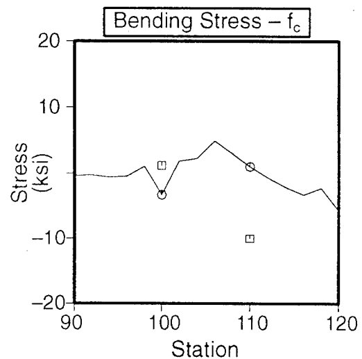
Figure E-14. Skin Stress Correlation at Stringer S-1 + 4.6 Inches for FAA 1, Test 2 (No MSD). The Finite Element Model Contains a 30-Inch Crack and the Test Panel Contains a 32.24-Inch Crack
