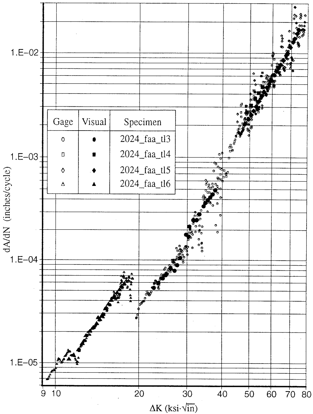
Figure 5. Crack Growth Rate Data Calculated From Fractomat and Visual Crack Length Measurements
