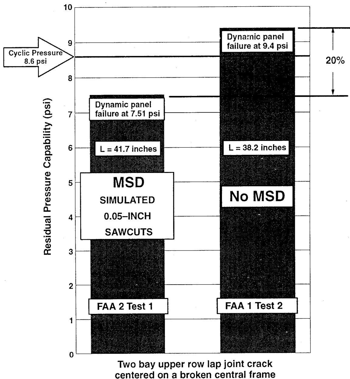
Figure 45. Panel FAA 1, Test 2 vs. FAA 2, Test 1 Residual Strength Comparison
