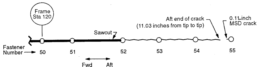
Figure 21. Crack Trajectory of Panel FAA 1, Test 1
