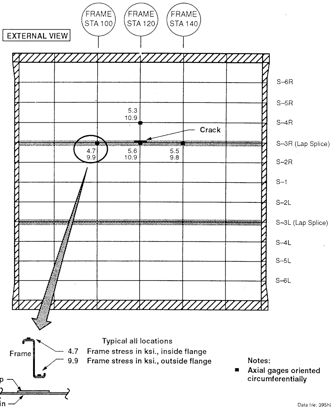
Figure C-17. Frame Stress of Panel FAA 1, Test 1 With 5.63-Inch Crack Length
