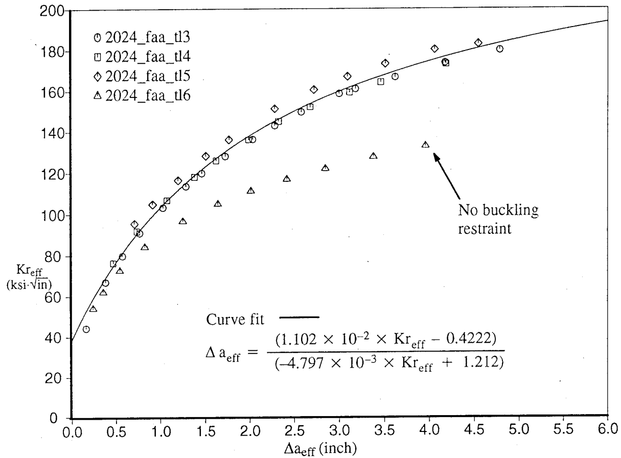
Figure 7. R-Curve Test Results
