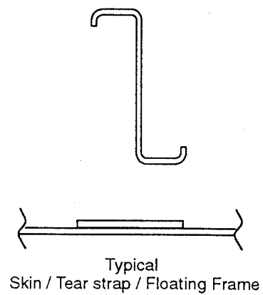
Figure 11. Structural Details of Panel FAA 1 and FAA 2
