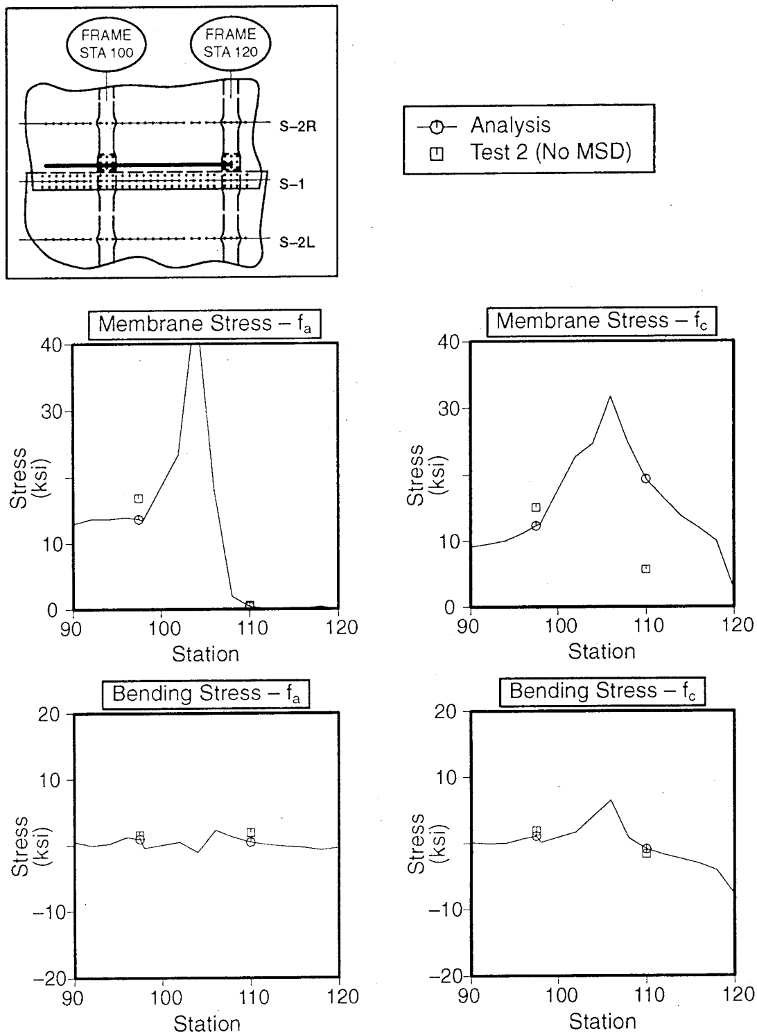
Figure E-13. Skin Stress Correlation at Stringer S-1 + 2.3 Inches for FAA 1, Test 2 (No MSD). The Finite Element Model Contains a 30-Inch Crack and the Test Panel Contains a 32.24-Inch Crack
