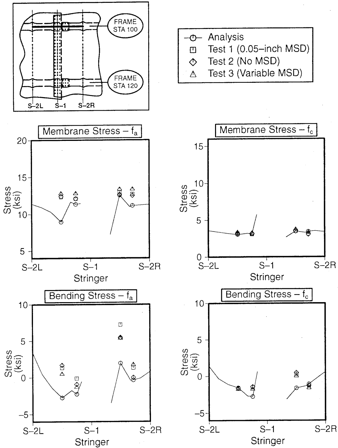
Figure E-5. Skin Stress Correlation at Station 100 for a Test Panel Containing a 5-Inch Sawcut
