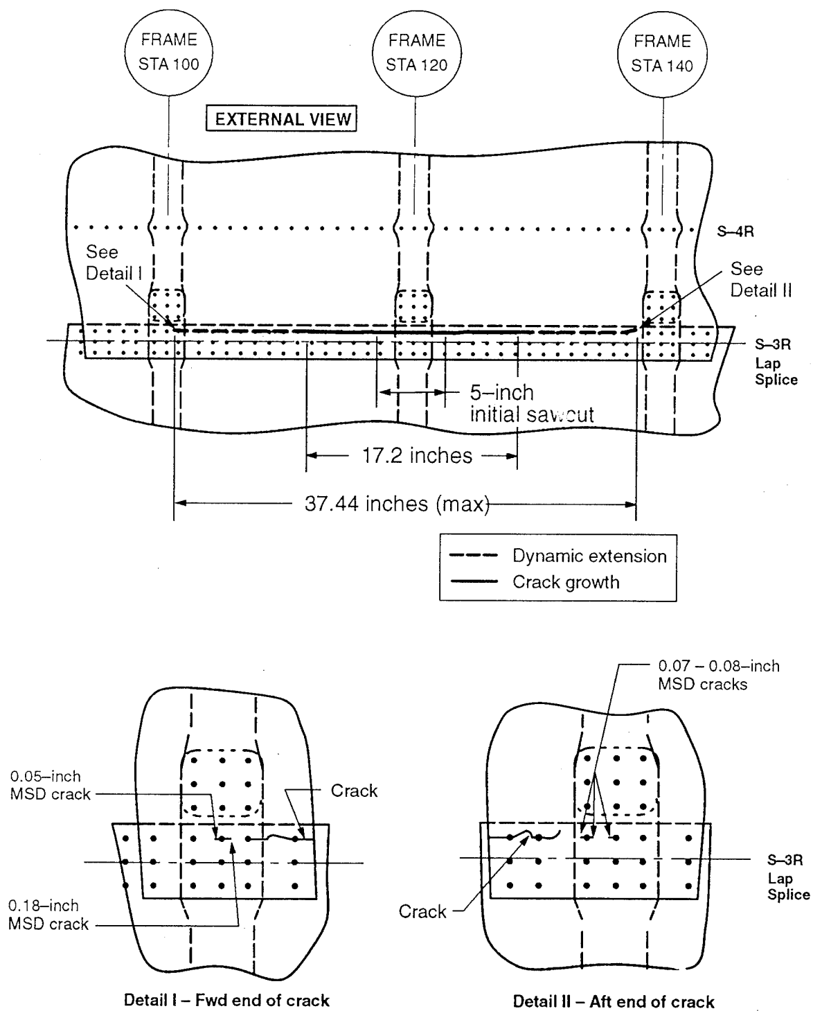
Figure 22. Crack Trajectory of Panel FAA 1, Test 1
