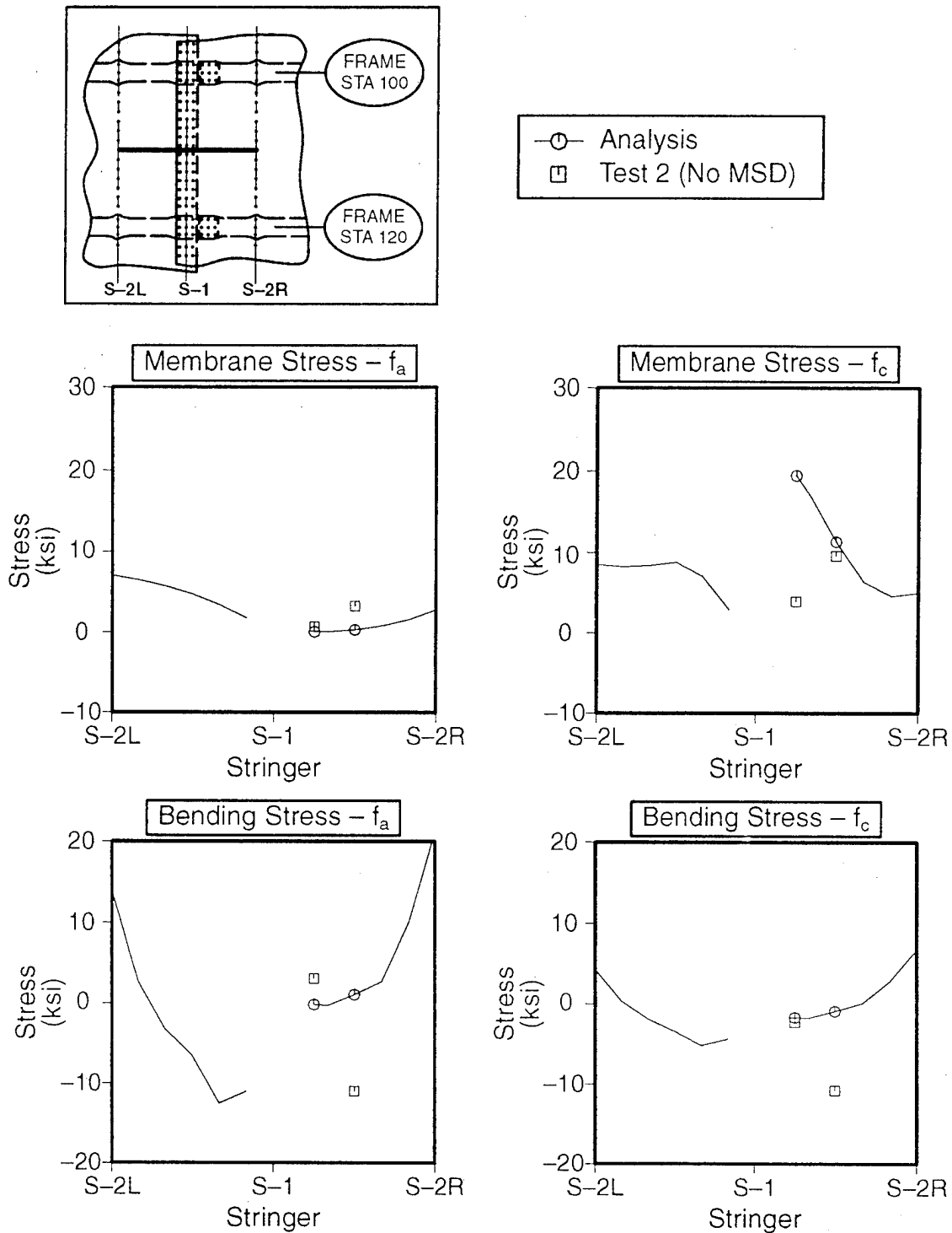
Figure E-18. Skin Stress Correlation at Station 110 for FAA 1, Test 2 (No MSD). The Finite Element Model Contains a 38-Inch Crack and the Test Panel Contains 36.71-Inch Crack
