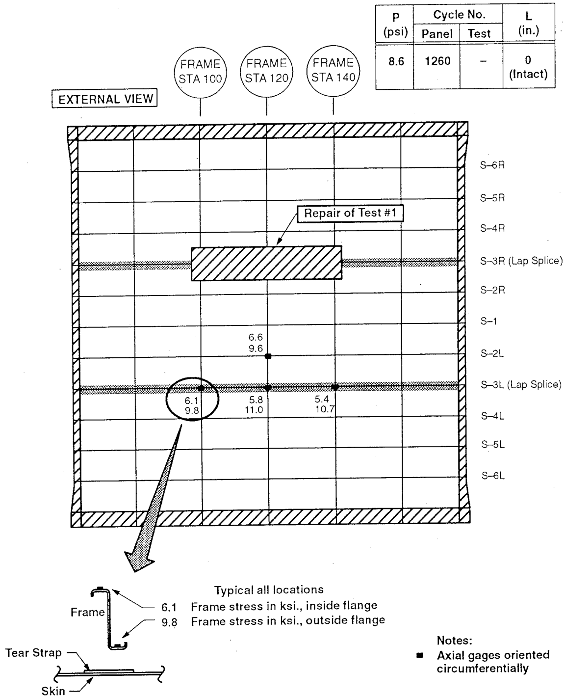
Figure C-25. Frame Stress of Panel FAA 1, Test 2 Intact Data
