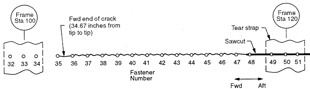
Figure 29. Crack Trajectory of Panel FAA 1, Test 2
