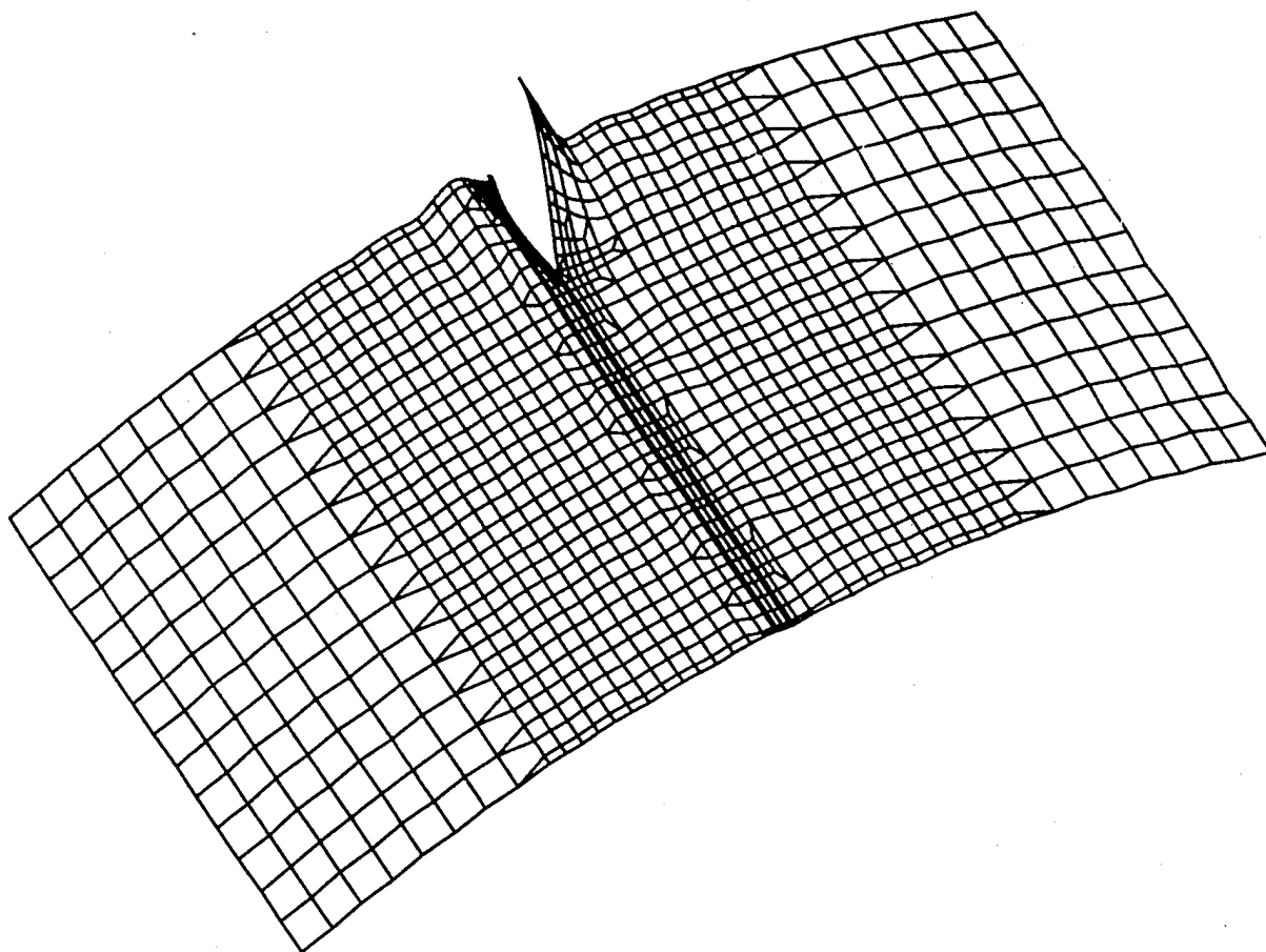
Figure 51. Displaced Skin Mesh Containing a 30-Inch Crack, Internal Pressure = 8.6 psi, Magnification Factor \approx 10\times
