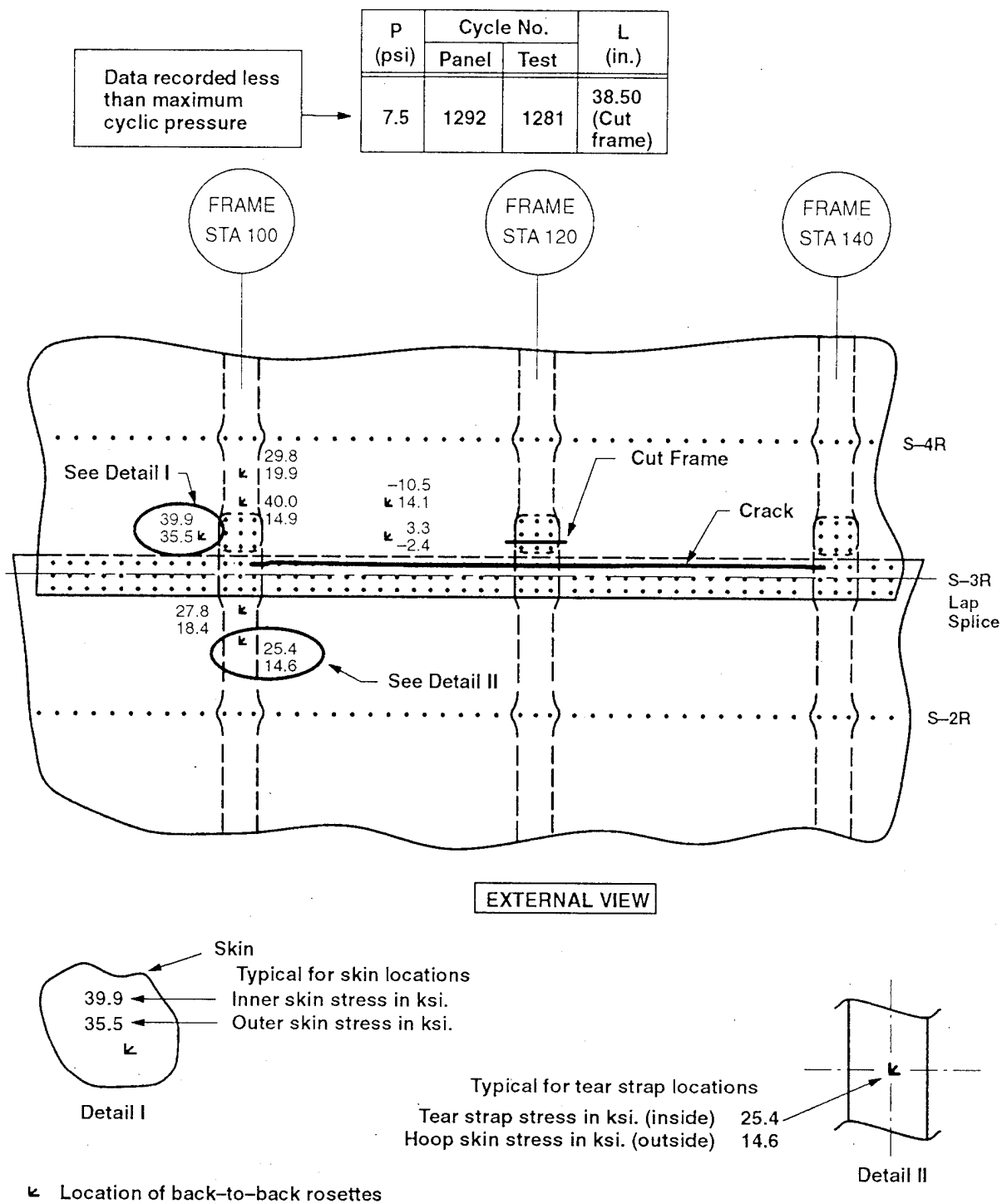
Figure C-63. Hoop Skin and Tear Strap Stress of Panel FAA 2, Test 1 With 38.50-Inch Crack Length and Cut Frame
