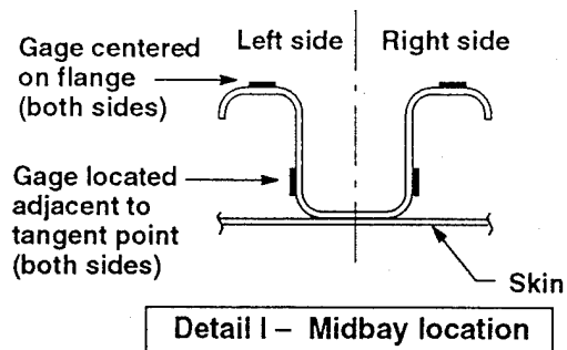
Figure C-3. Stiffener Strain Gage Locations of Panel FAA 1, Tests 1, 2 and FAA 2, Test 1
