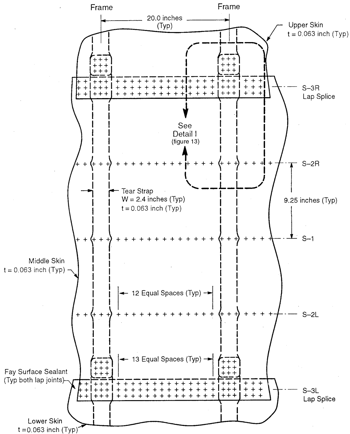
Figure 12. Structural Dimensions of Panel FAA 1 and FAA 2 With Bonded Tear Straps
