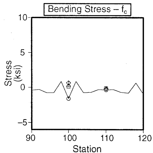
Figure 61. Skin Stress Correlation at Stringer S-1 + 4.6 Inches for an Intact Test Panel
