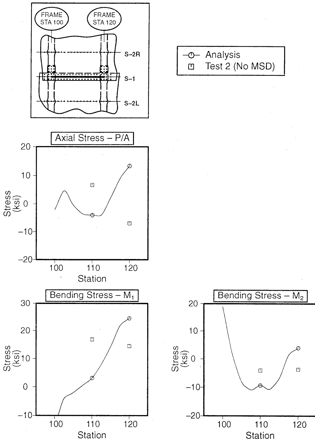
Figure E-28. Stringer Stress Correlation at Stringer S-1 for FAA 1, Test 2 at a Crack Length of 40 Inches With a Severed Central Frame
