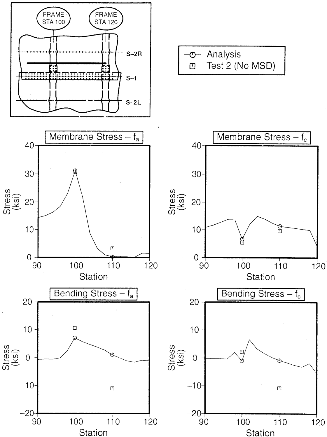
Figure E-20. Skin Stress Correlation at Stringer S-1 + 4.6 Inches for FAA 1, Test 2 (No MSD). The Finite Element Model Contains a 38-Inch Crack and the Test Panel Contains a 36.71-Inch Crack
