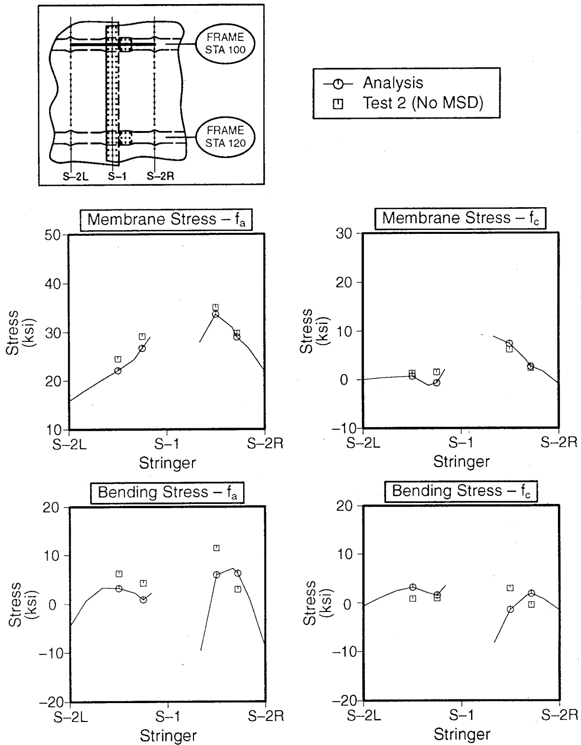
Figure E-23. Skin Stress Correlation at Station 100 for FAA 1, Test 2 (No MSD). Crack Length of 40 Inches With a Severed Central Frame
