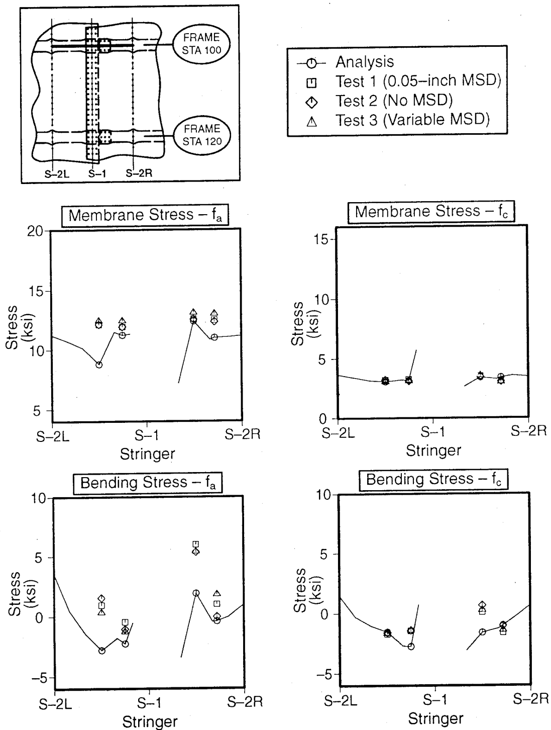
Figure 58. Skin Stress Correlation at Station 100 for an Intact Test Panel
