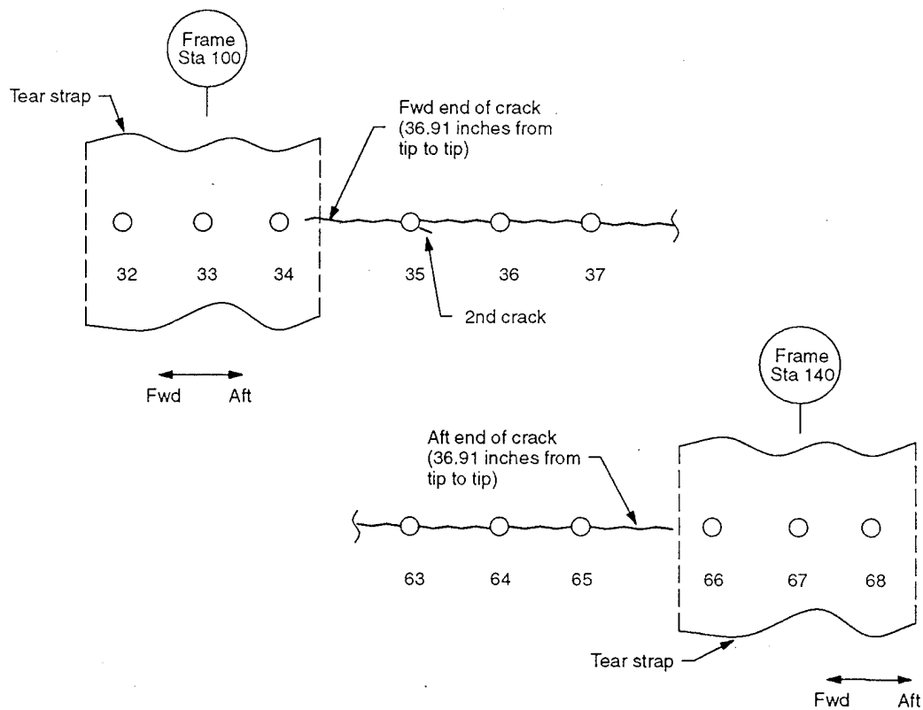
Figure 30. Crack Trajectory of Panel FAA 1, Test 2
