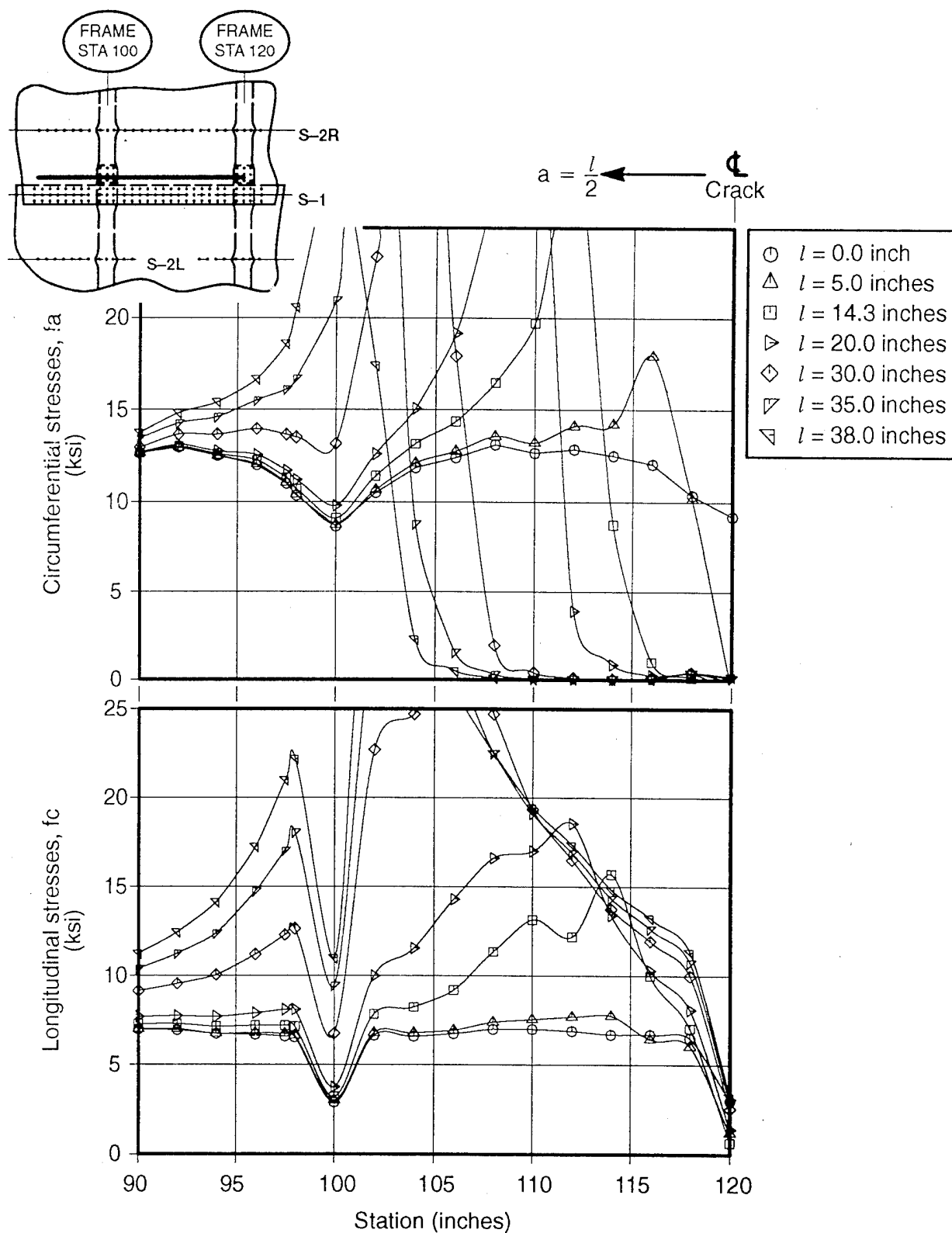
Figure 54. Predicted Midplane Stresses in the Upper Skin 2.3 Inches Right of the Lap Joint Stringer Centerline
