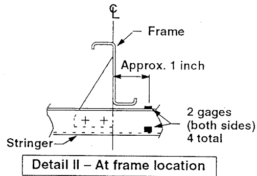
Figure C-10. Stiffener Strain Gage Identification of Panel FAA 2, Test 1
