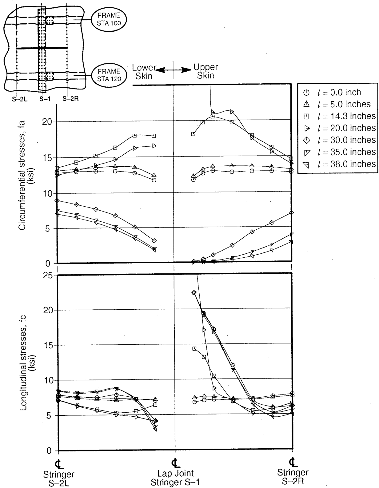
Figure 53. Predicted Midplane Stresses at Station 110
