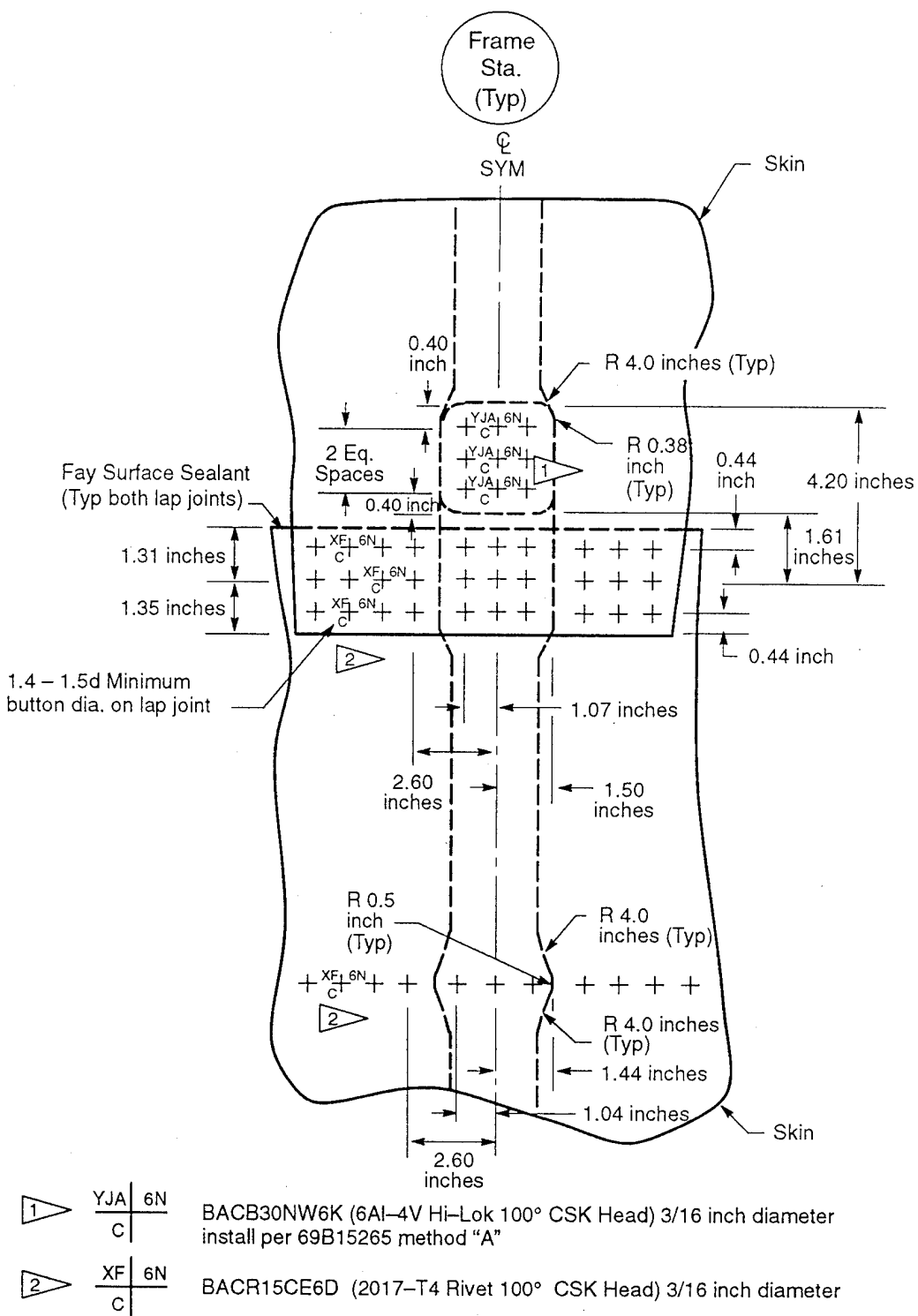
Figure 13. Structural Dimensions (Detail I) of Panel FAA 1 and FAA 2
