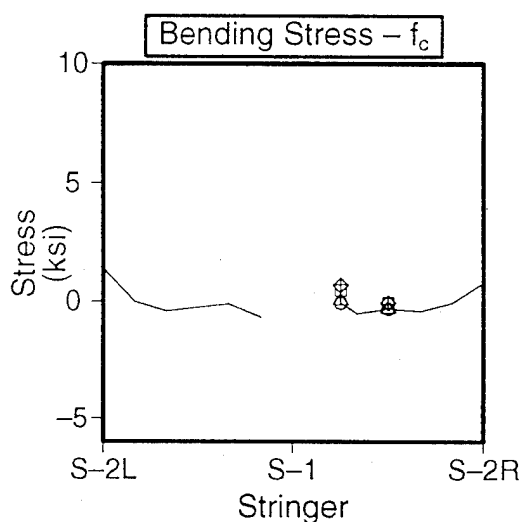
Figure E-6. Skin Stress Correlation at Station 110 for a Test Panel Containing a 5-Inch Sawcut
