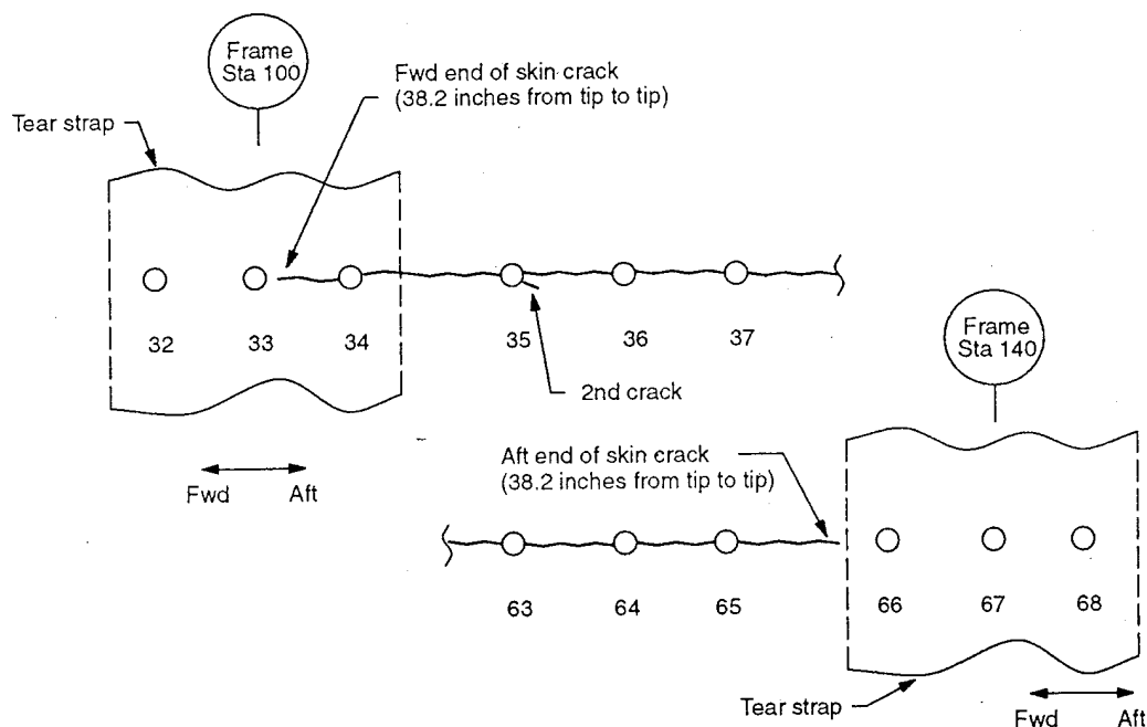
Figure 32. Crack Configuration Prior to Panel Failure
