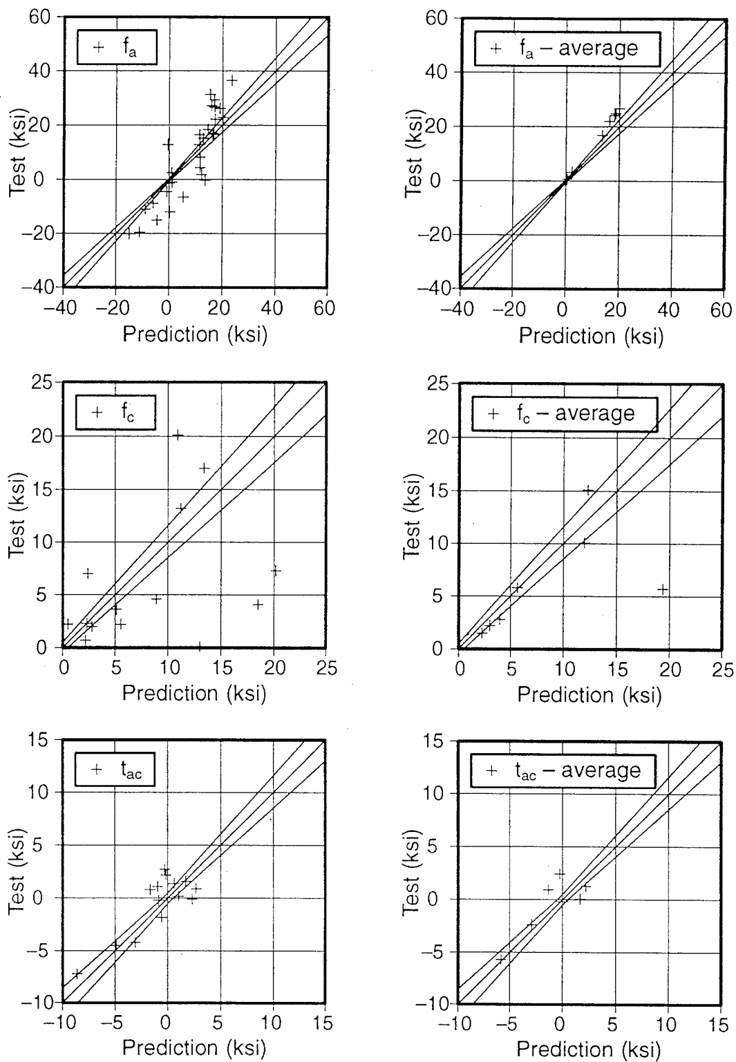
Figure E-2. Test / Analysis Strain Gage Correlation for FAA 1, Test 2 (No MSD). The Finite Element Model Contains a 30-Inch Crack and the Test Panel Contains a 32.24-Inch Crack
