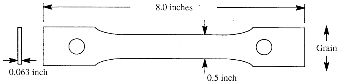
Figure 1. Tensile Specimen Geometry
