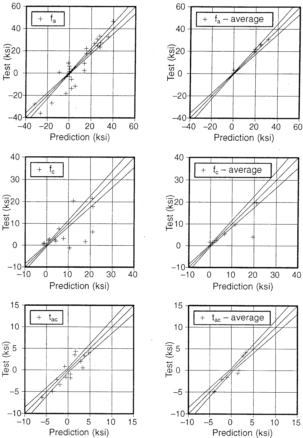
Figure E-4. Test / Analysis Strain Gage Correlation for FAA 1, Test 2 (No MSD) With a Severed Central Frame. The Finite Element Model Contains a 40-Inch Crack and the Test Panel Contains an Extending 36.71-Inch Crack
