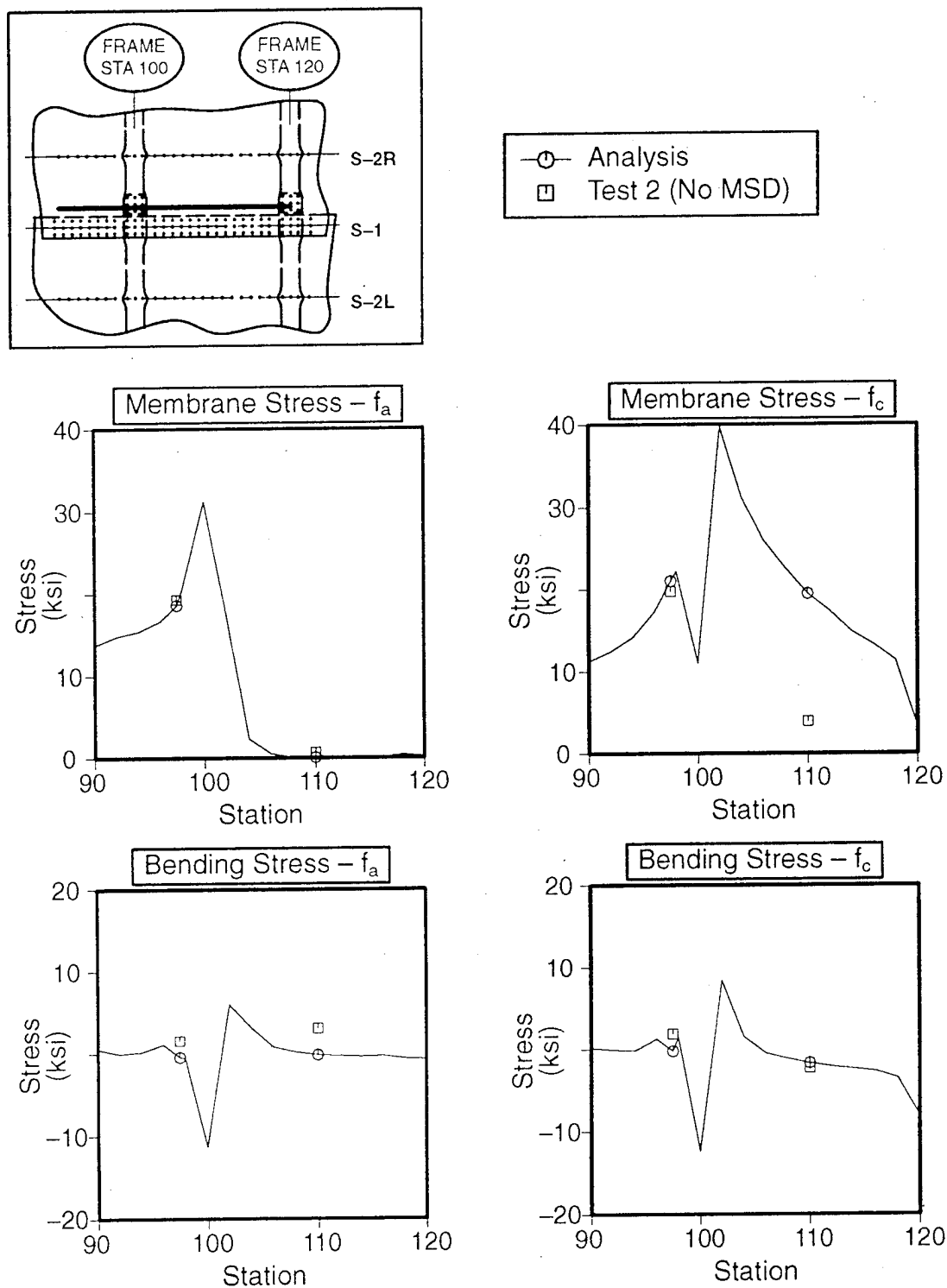
Figure E-19. Skin Stress Correlation at Stringer S-1 + 2.3 Inches for FAA 1, Test 2 (No MSD). The Finite Element Model Contains a 38-Inch Crack and the Test Panel Contains a 36.71-Inch Crack
