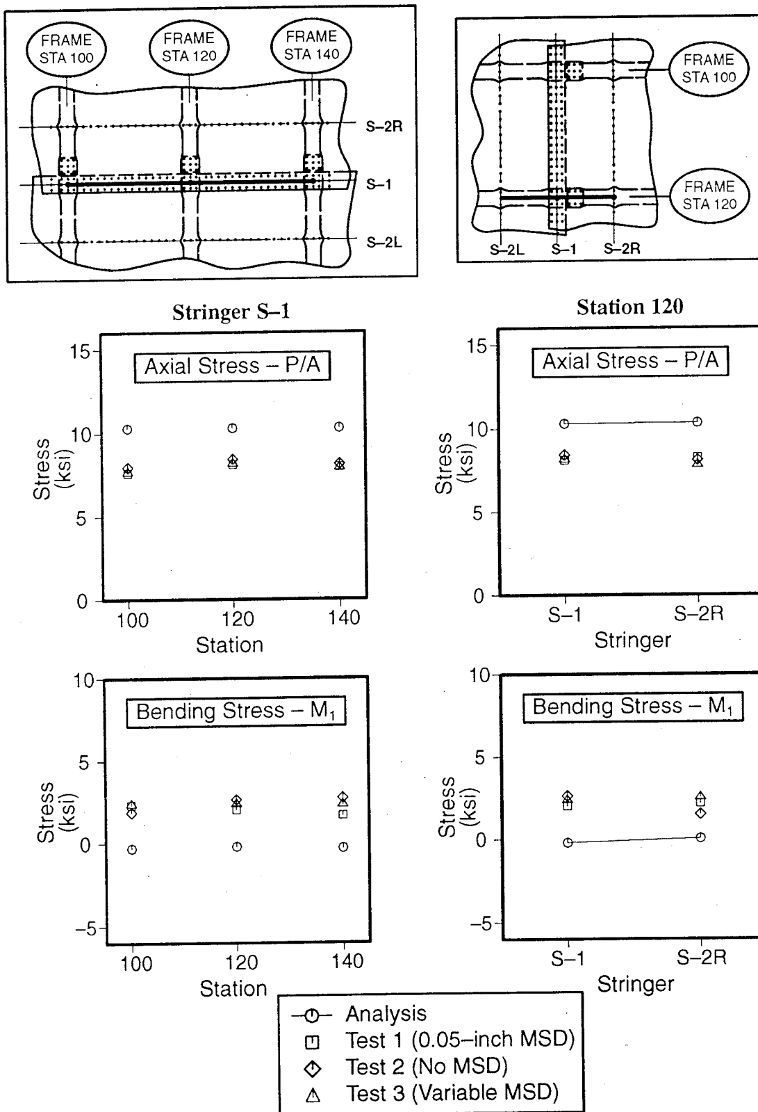
Figure 62. Frame Stress Correlations for an Intact Test Panel
