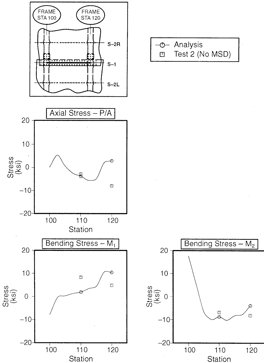
Figure E-22. Stringer Stress Correlation at Stringer S-1 for FAA 1, Test 2 (No MSD). The Finite Element Model Contains a 38-Inch Crack and the Test Panel Contains a 36.71-Inch Crack
