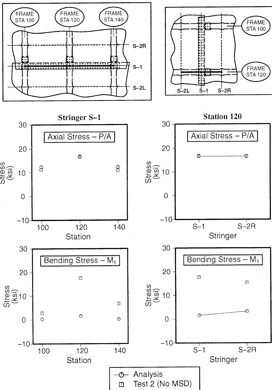
Figure E-21. Frame Stress Correlations for FAA 1, Test 2 (No MSD). The Finite Element Model Contains a 38-Inch Crack and the Test Panel Contains a 36.71-Inch Crack
