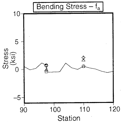
Figure E-7. Skin Stress Correlation at Stringer S-1 + 2.3 Inches for a Test Panel Containing a 5-Inch Sawcut.
