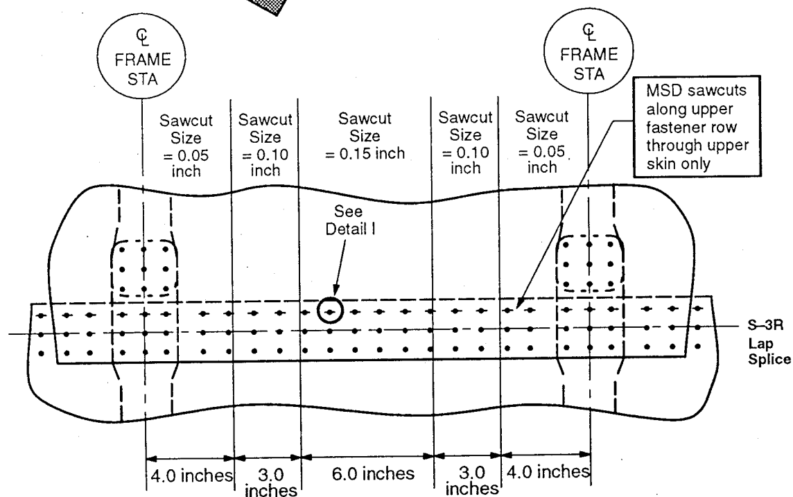
Figure 18. MSD Sawcut Details for Panel FAA 2, Test 1
