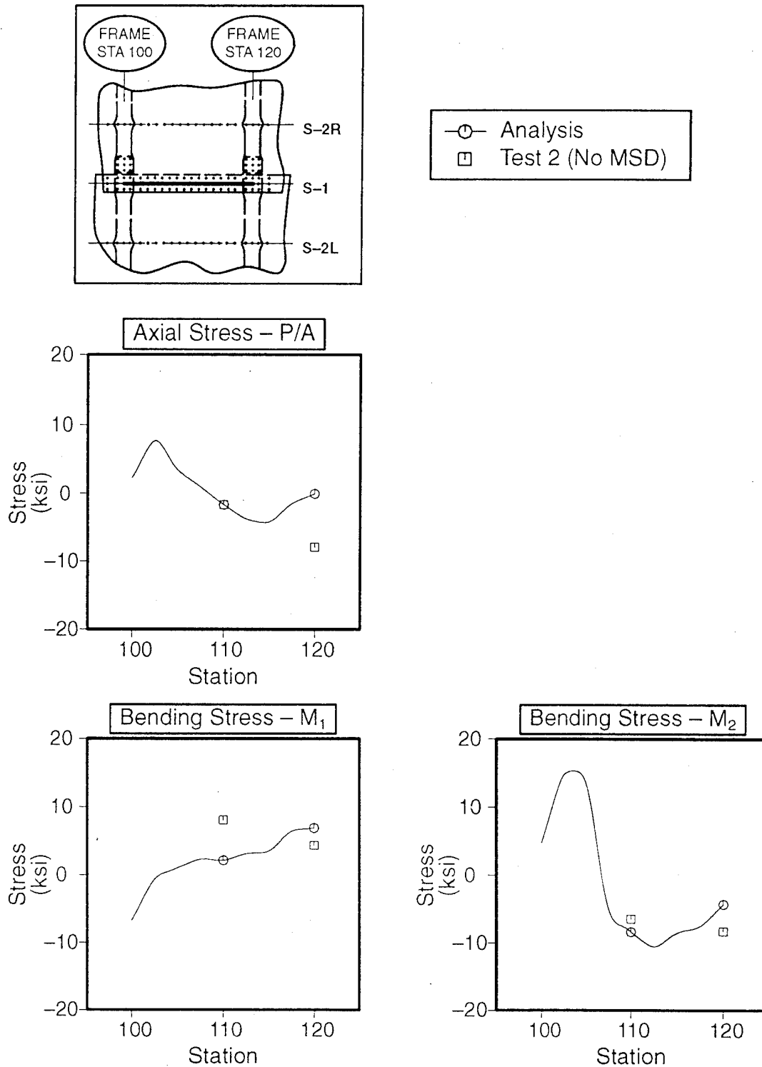
Figure E-16. Stringer Stress Correlation at Stringer S-1 for FAA 1, Test 2 (No MSD). The Finite Element Model Contains a 30-Inch Crack and the Test Panel Contains a 32.24-Inch Crack
