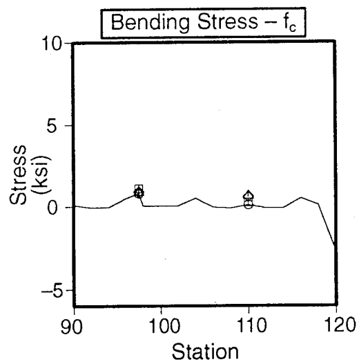
Figure 60. Skin Stress Correlation at Stringer S-1 + 2.3 Inches for an Intact Test Panel
