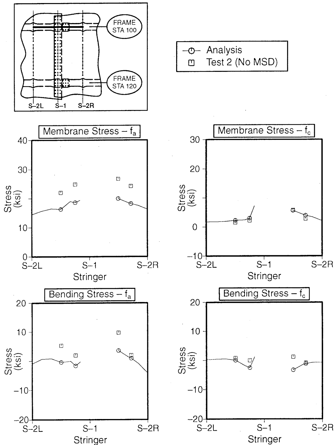
Figure E-11. Skin Stress Correlation at Station 100 for FAA 1, Test 2 (No MSD). The Finite Element Model Contains a 30-Inch Crack and the Test Panel Contains a 32.24-Inch Crack
