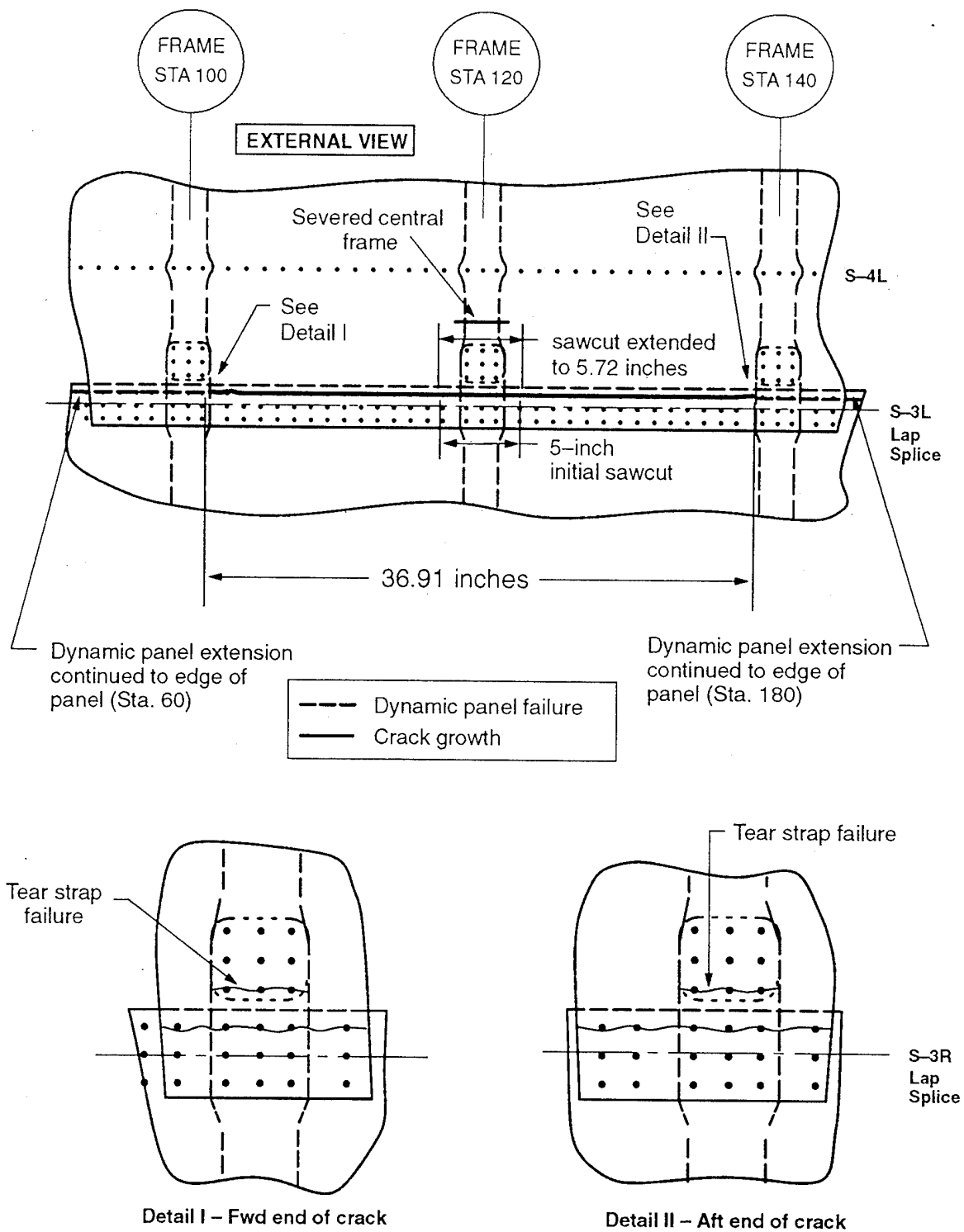
Figure 33. Crack Trajectory of Panel FAA 1, Test 2
