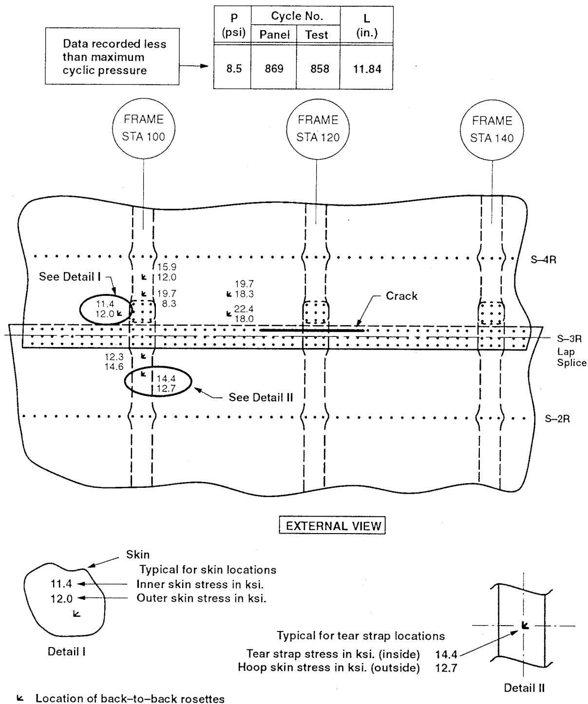
Figure C-55. Hoop Skin and Tear Strap Stress of Panel FAA 2, Test 1 With 11.84-Inch Crack Length
