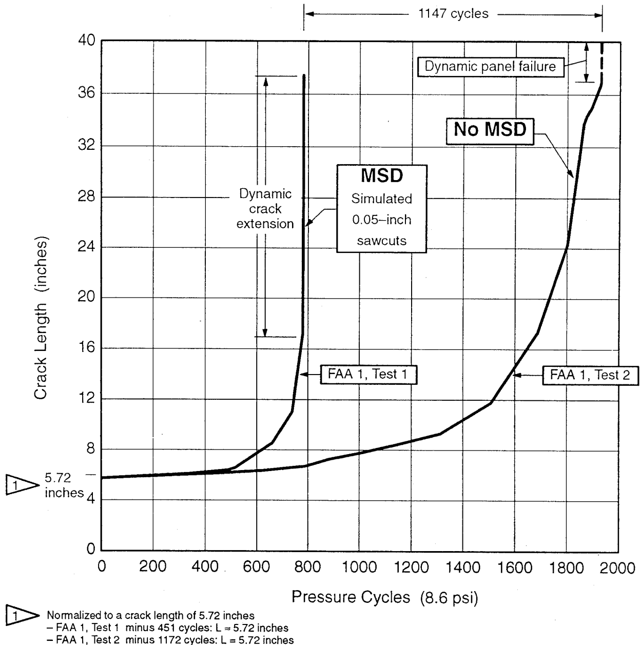
Figure 44. Panel FAA 1, Test 1 and Test 2 Crack Growth Comparison
