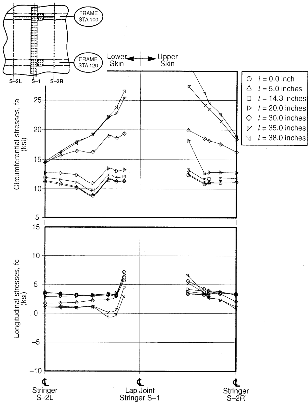
Figure 52. Predicted Midplane Stresses at Station 100
