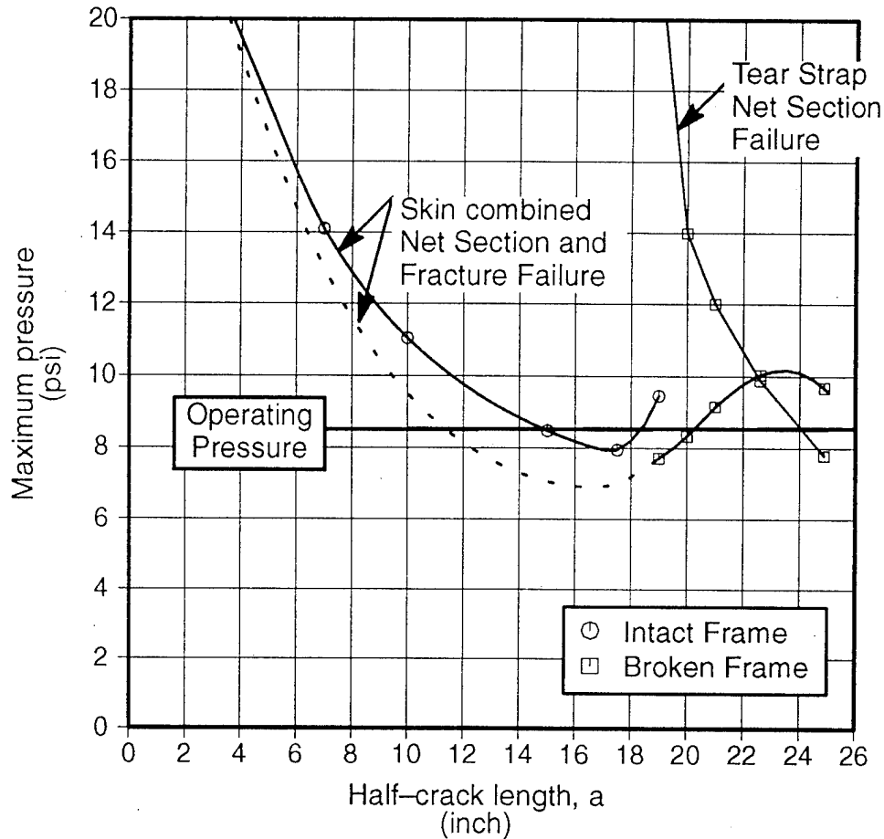
Figure 68. Residual Strength Prediction for a Lap Joint Upper Row Skin Crack
