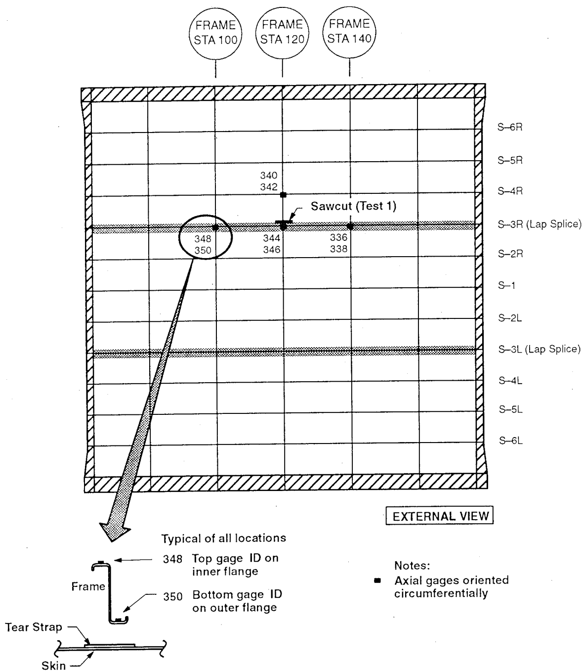
Figure C-9. Frame Strain Gage Identification of Panel FAA 2, Test 1
