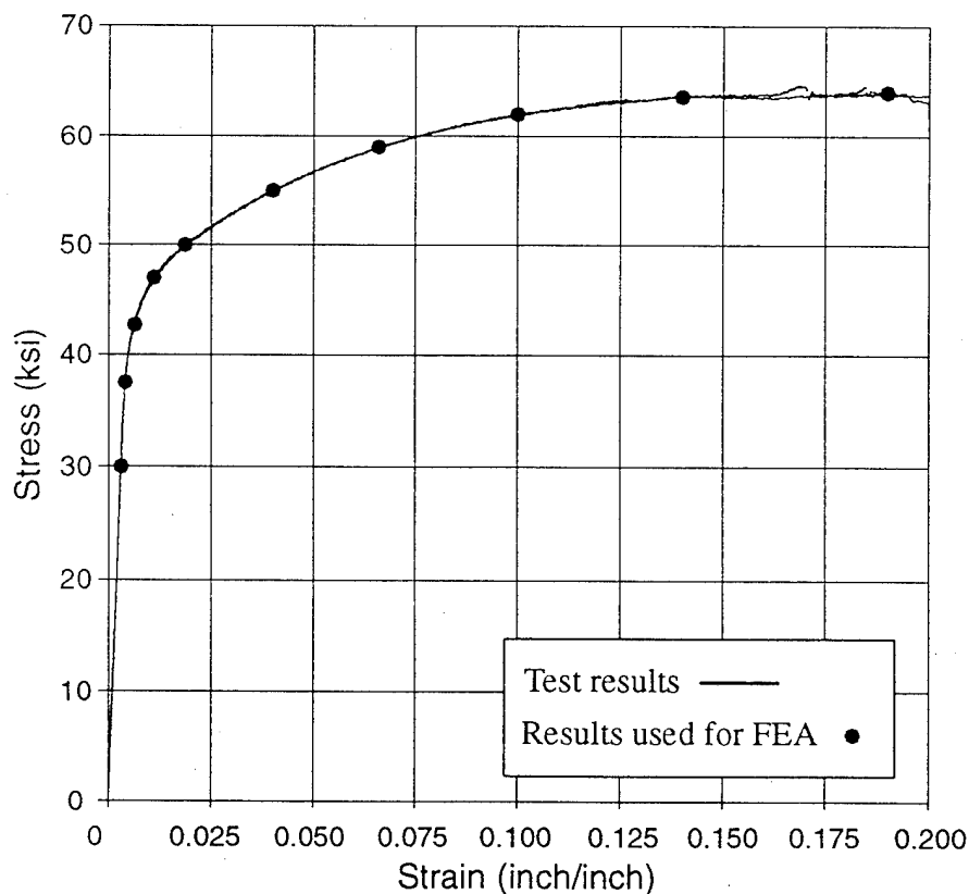
Figure 4. Engineering Stress-Strain Curve for 0.063-Inch-Thick 2024-T3 L-T Aluminum
