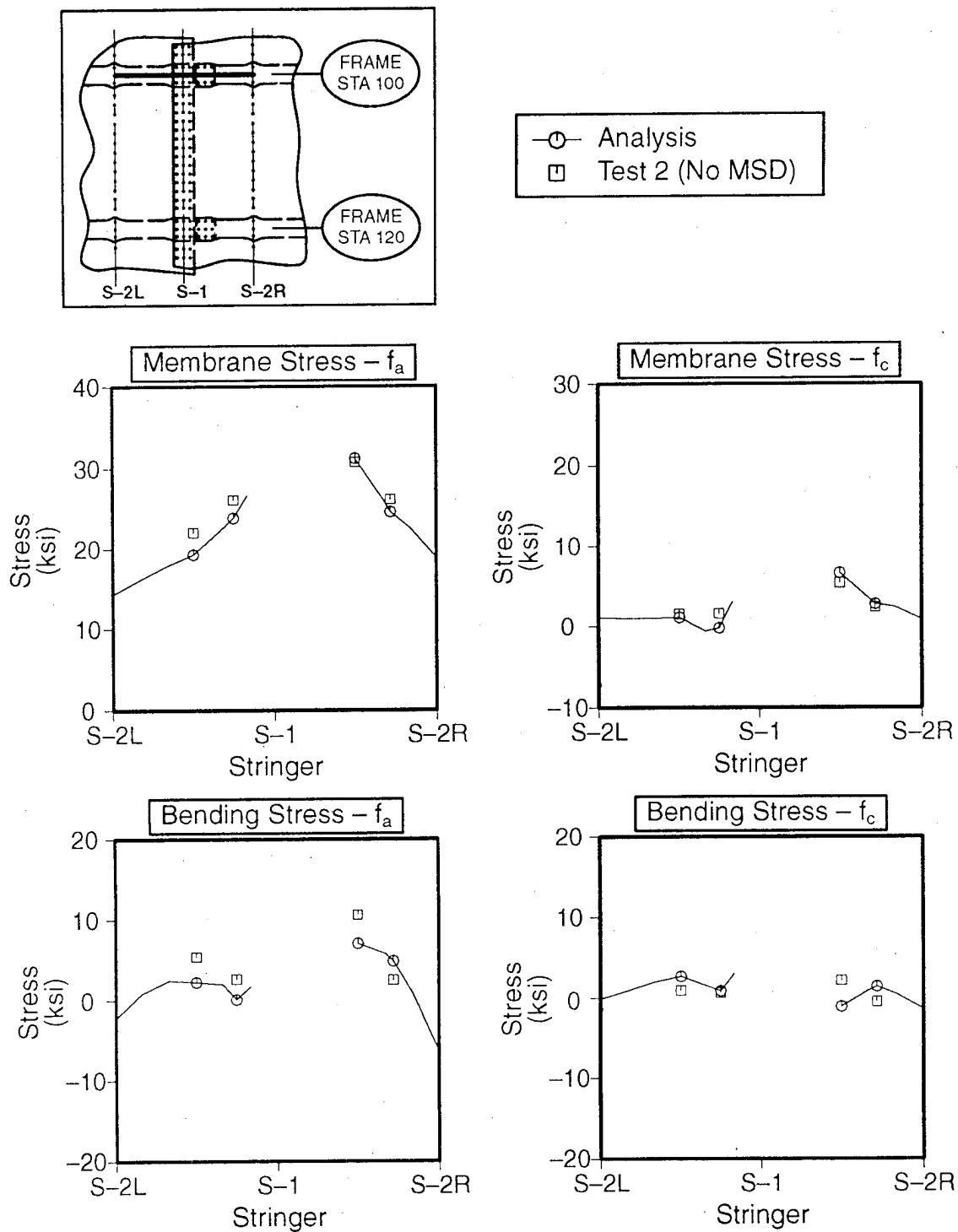
Figure E-17. Skin Stress Correlation at Station 100 for FAA 1, Test 2 (No MSD). The Finite Element Model Contains a 38-Inch Crack and the Test Panel Contains a 36.71-Inch Crack
