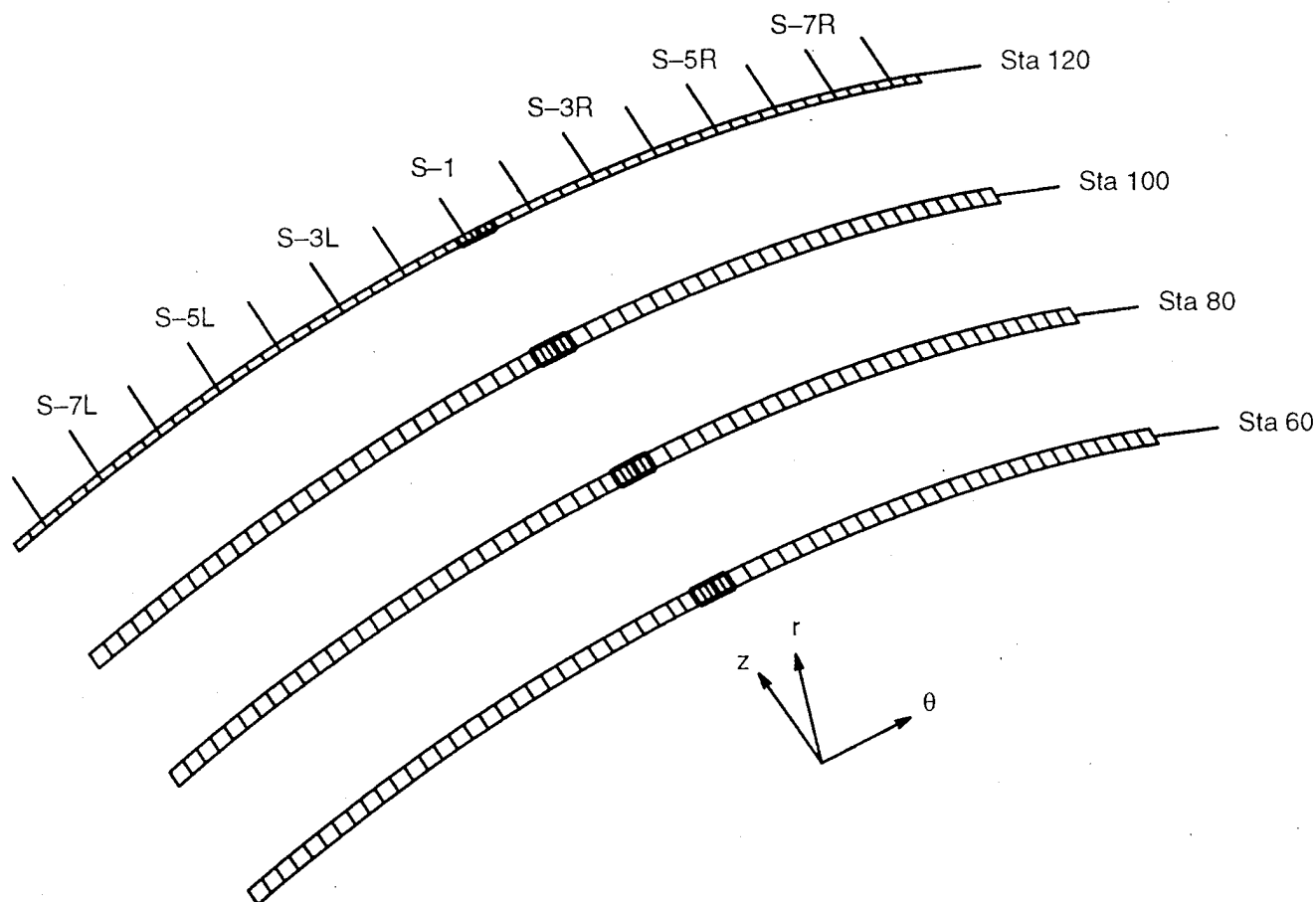
Figure 47. Tear Strap Mesh
