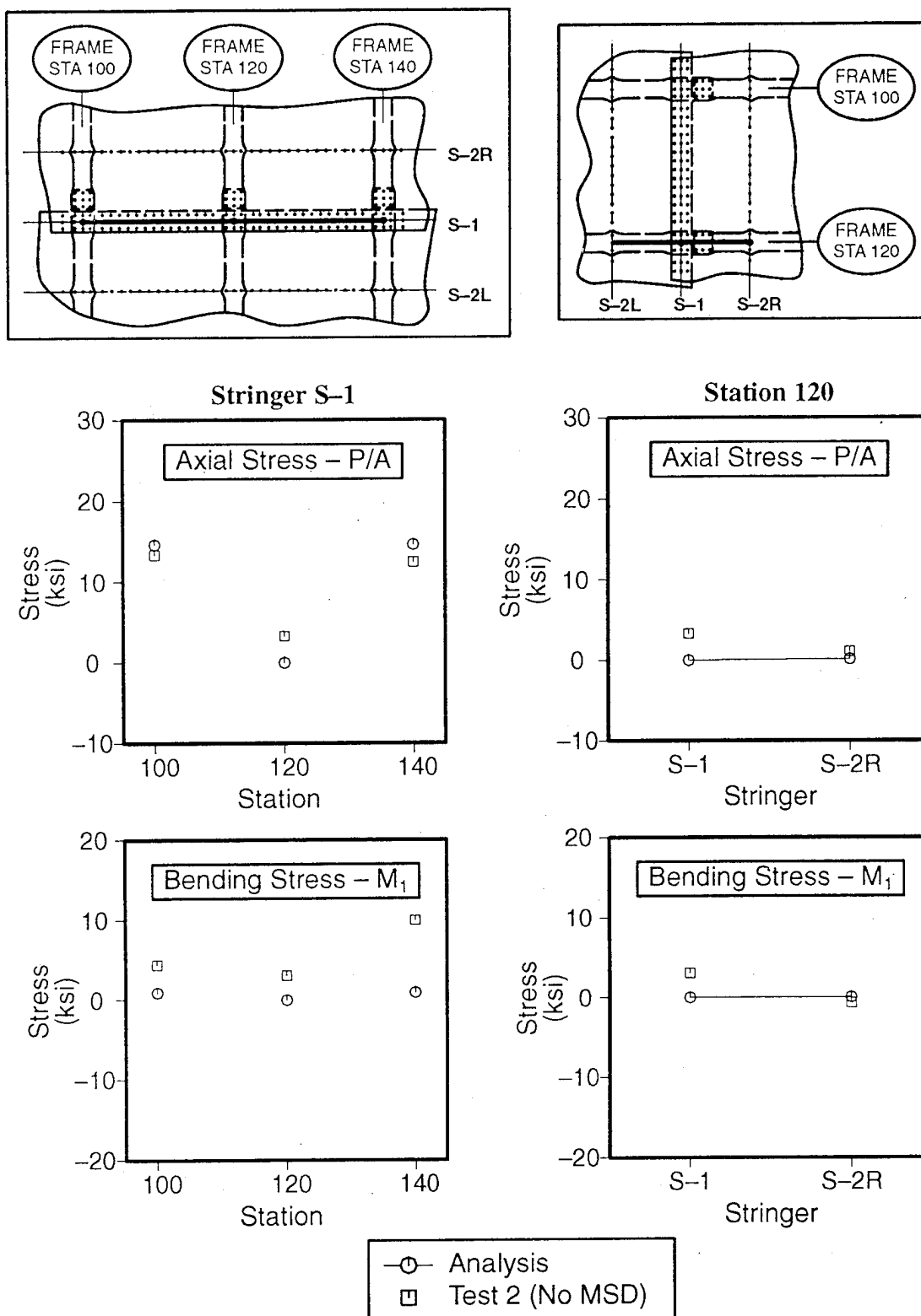
Figure E-27. Frame Stress Correlations for FAA 1, Test 2 (No MSD). Crack Length of 40 Inches With a Severed Central Frame
