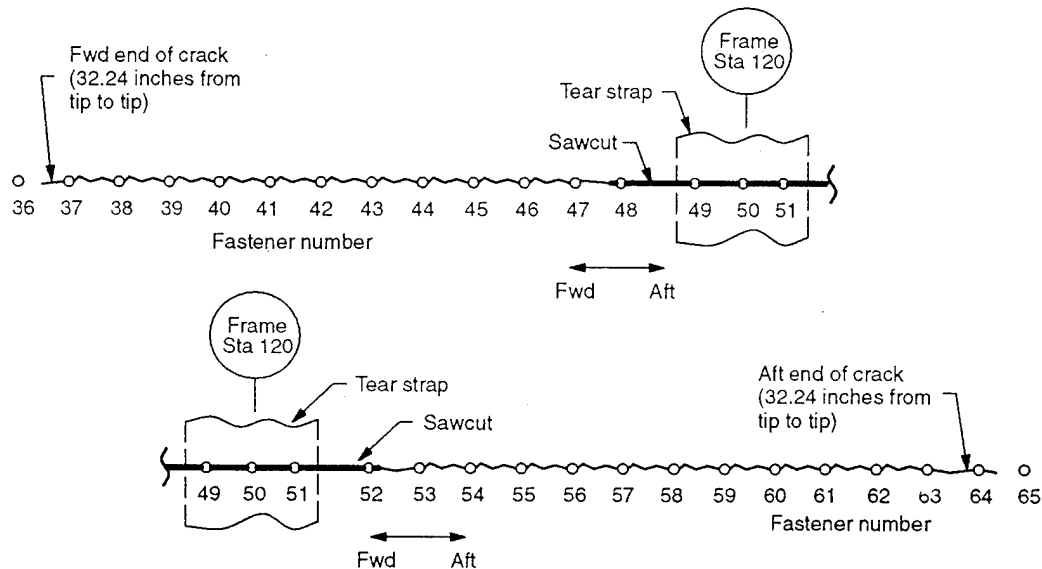
Figure 28. Crack Trajectory of Panel FAA 1, Test 2
