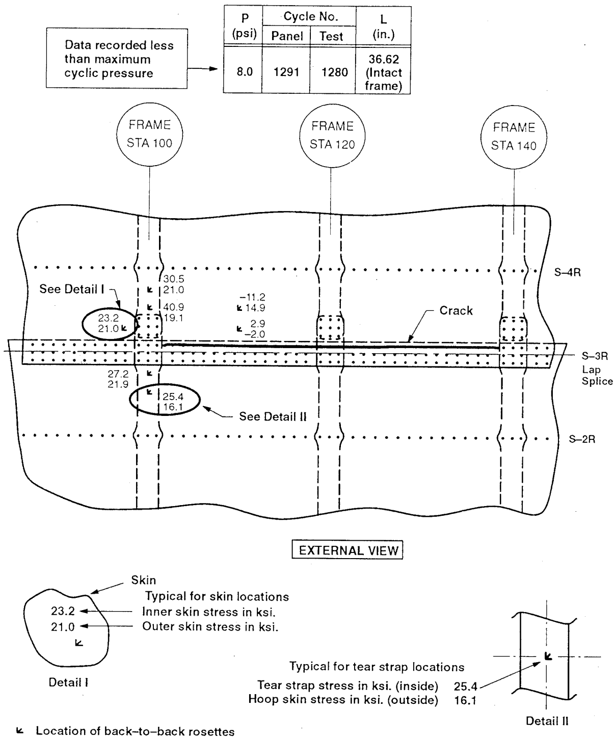
Figure C-59. Hoop Skin and Tear Strap Stress of Panel FAA 2, Test 1 With 36.62-Inch Crack Length and Intact Frame
