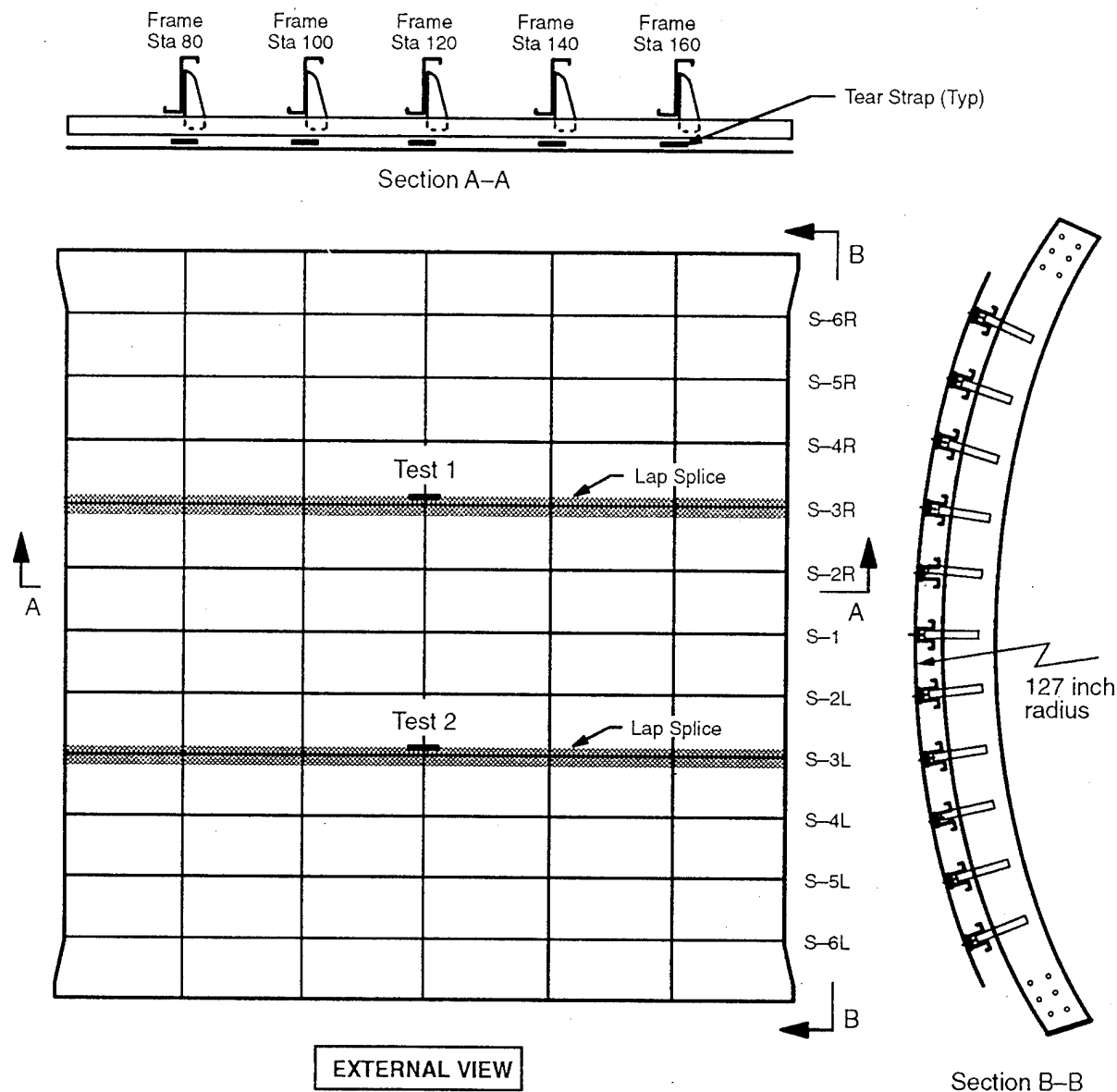
Figure 9. Structural Configuration and Test Locations of Panel FAA 1 and FAA 2
