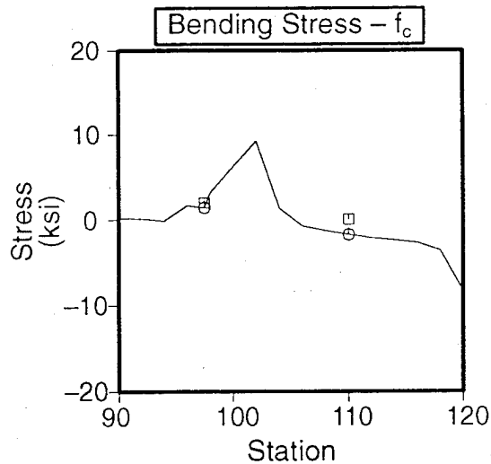
Figure E-25. Skin Stress Correlation at Stringer S-1 + 2.3 Inches for FAA 1, Test 2 (No MSD). Crack Length of 40 Inches With a Severed Central Frame
