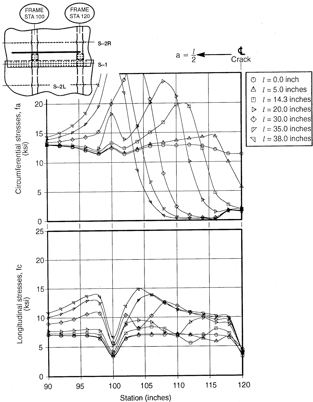
Figure 55. Predicted Midplane Stresses in the Upper Skin 4.6 Inches Right of the Lap Joint Stringer Centerline
