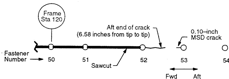
Figure 20. Crack Trajectory of Panel FAA 1, Test 1
