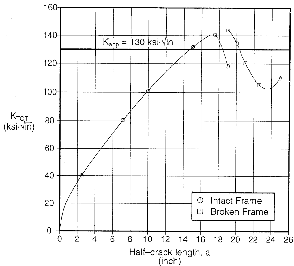
Figure 56. Stress Intensity Factor Predictions at Operating Pressure
