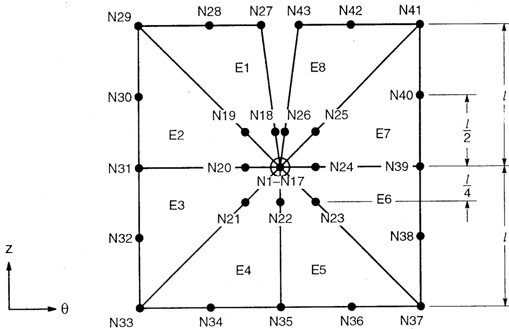
Figure D-1. Crack Tip Shell Elements
