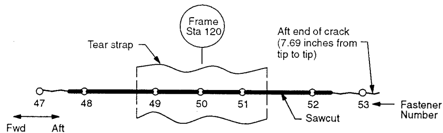
Figure 26. Crack Trajectory of Panel FAA 1, Test 2
