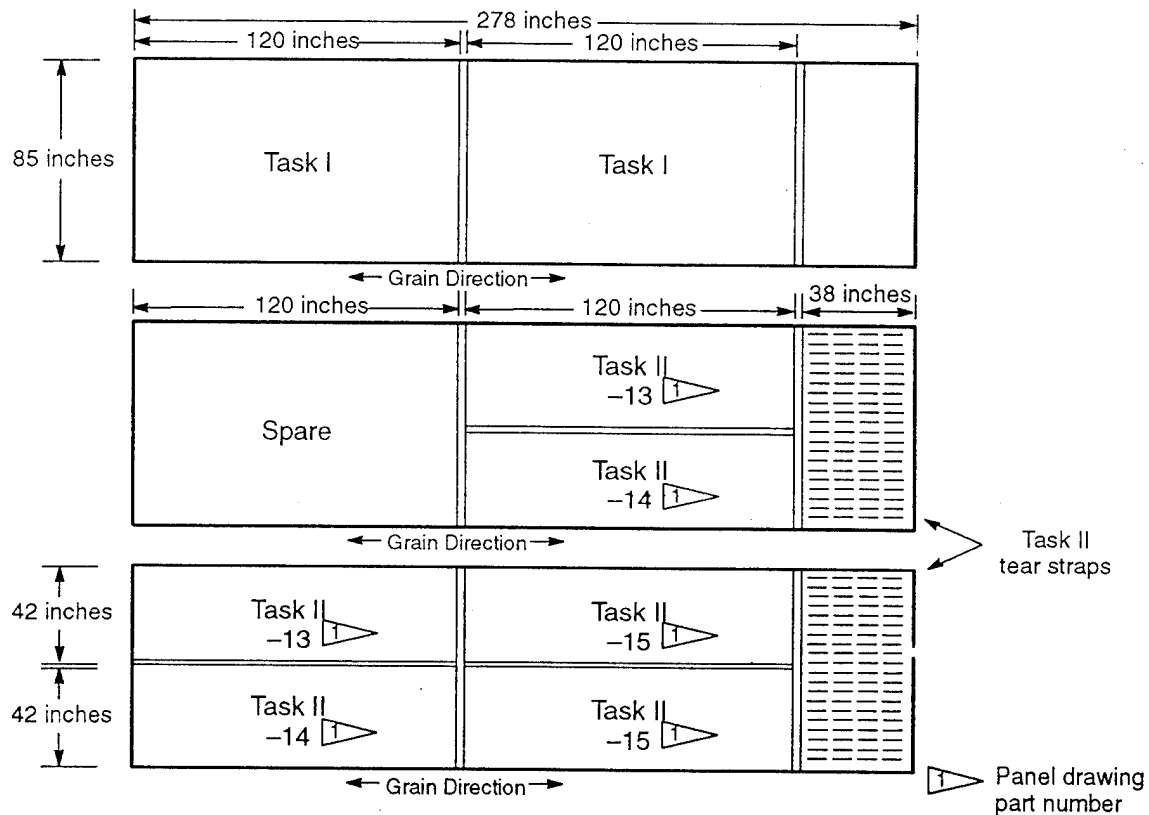
Figure 15. Skin Material Cutting Diagram
