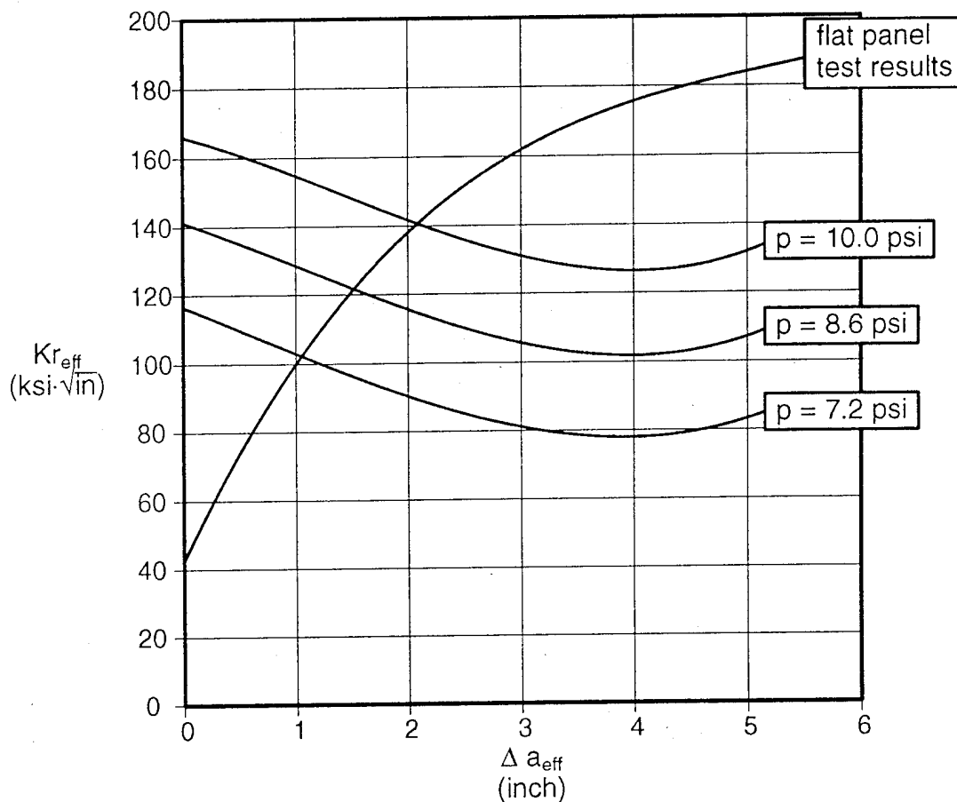
Figure 67. Predicted K_{r_{eff}} vs. \Delta a_{eff} for a_0 = 20 inches
