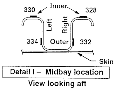
Figure C-10. Stiffener Strain Gage Identification of Panel FAA 2, Test 1
