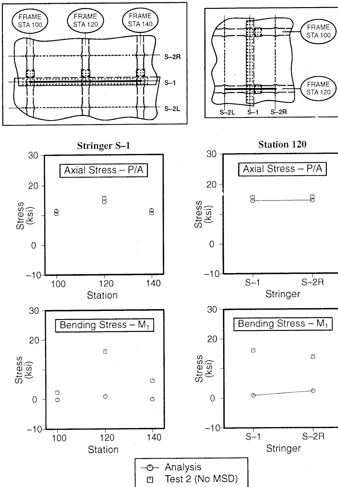
Figure E-15. Frame Stress Correlations for FAA 1, Test 2 (No MSD). The Finite Element Model Contains a 30-Inch Crack and the Test Panel Contains a 32.24-Inch Crack
