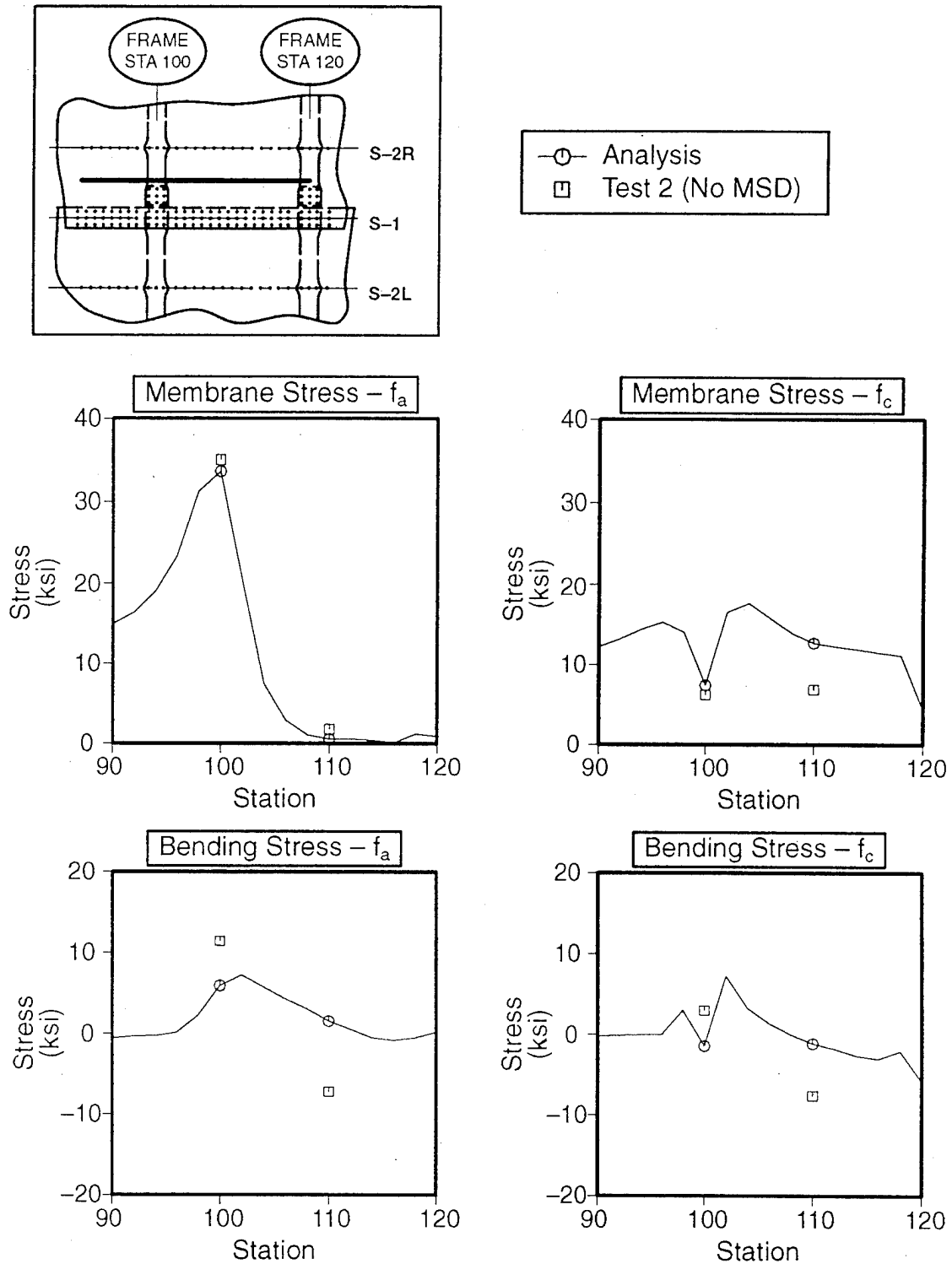
Figure E-26. Skin Stress Correlation at Stringer S-1 + 4.6 Inches for FAA 1, Test 2 (No MSD). Crack Length of 40 Inches With a Severed Central Frame
