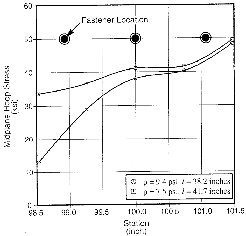
Figure 69. Comparison of the Predicted Midplane Hoop Stresses Along the Upper Row of Fasteners in the Tear Strap at Station 100 for the Residual Strength Tests
