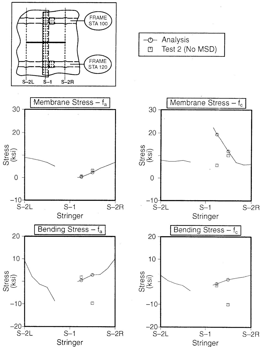
Figure E-12. Skin Stress Correlation at Station 110 for FAA 1, Test 2 (No MSD). The Finite Element Model Contains a 30-Inch Crack and the Test Panel Contains a 32.24-Inch Crack
