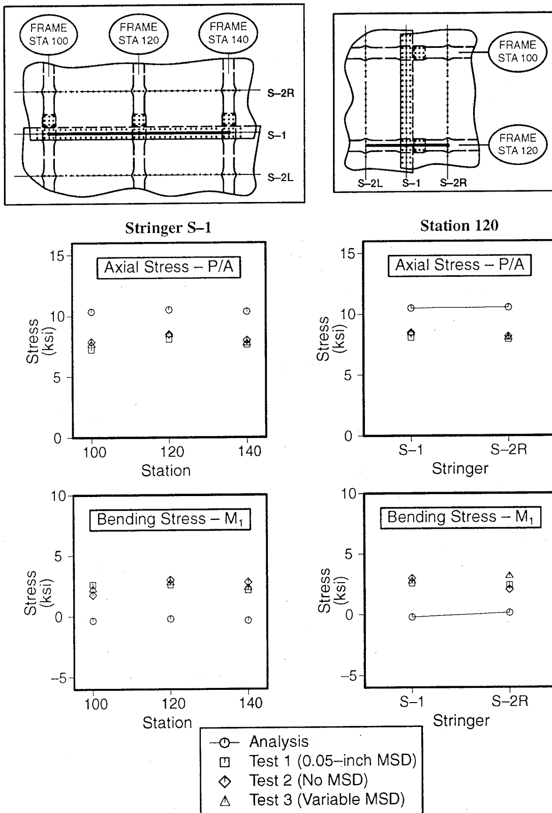
Figure E-9. Frame Stress Correlations for a Test Panel Containing a 5-Inch Sawcut
