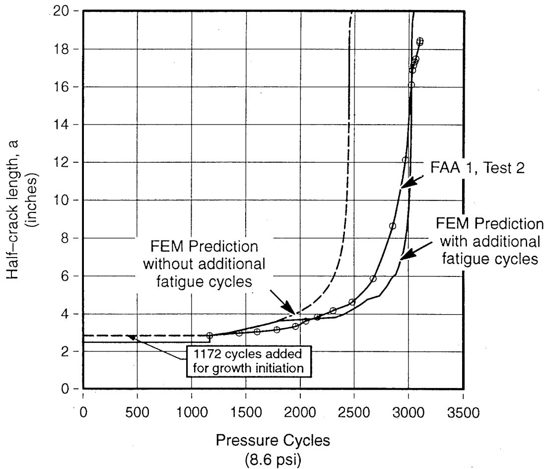
Figure 65. Crack Growth Prediction vs. Test Results for FAA 1, Test 2 (No MSD)
