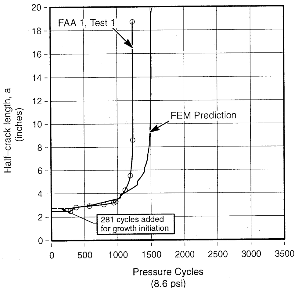
Figure 64. Crack Growth Prediction vs. Test Results for FAA 1, Test 1 (0.05-Inch MSD)
