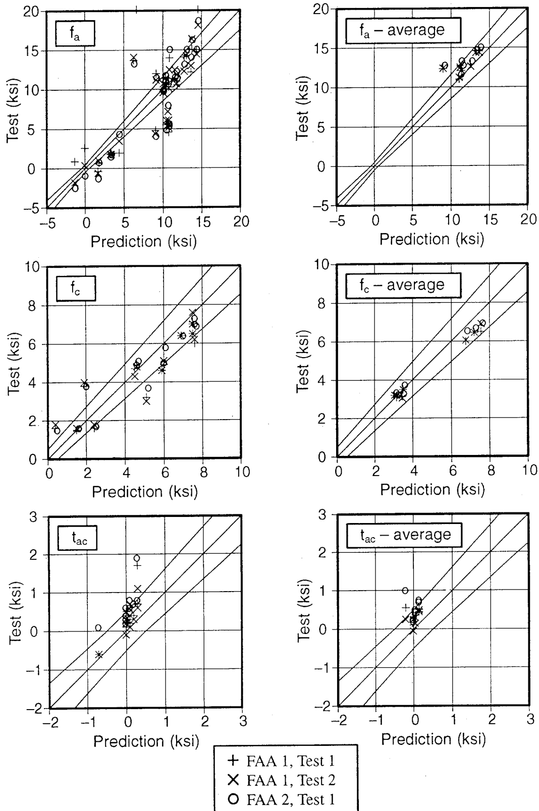
Figure E-1. Test / Analysis Strain Gage Correlation for Test Panels Containing a 5-inch Sawcut
