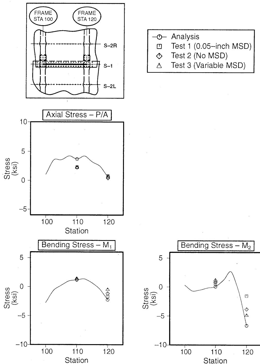
Figure E-10. Stringer Stress Correlation at Stringer S-1 for a Test Panel Containing a 5-Inch Sawcut
