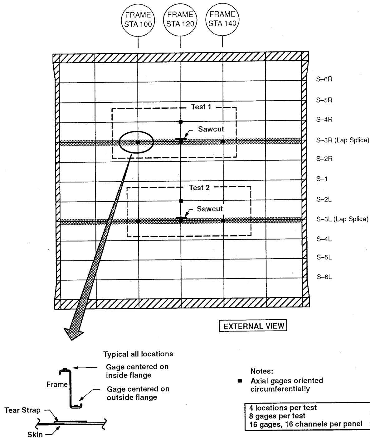
Figure C-2. Frame Strain Gage Locations of Panel FAA 1, Tests 1, 2 and FAA 2, Test 1
