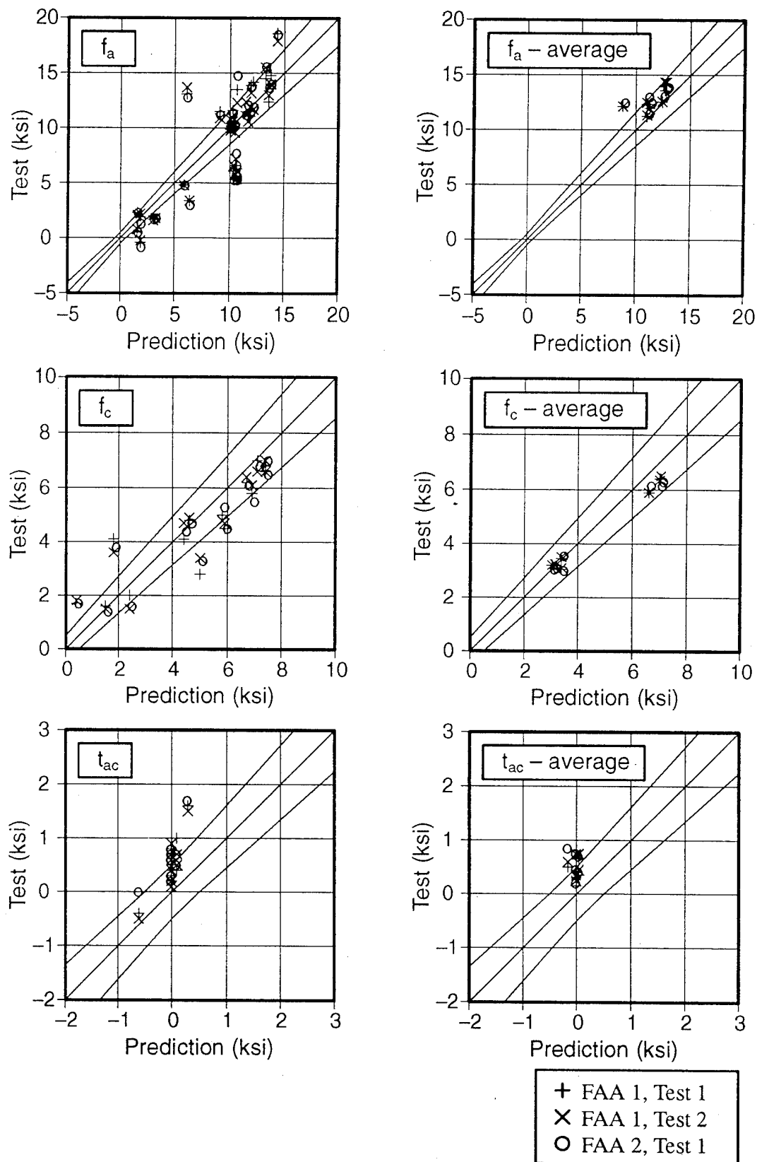
Figure 57. Test / Analysis Strain Gage Correlation for Intact Test Panels
