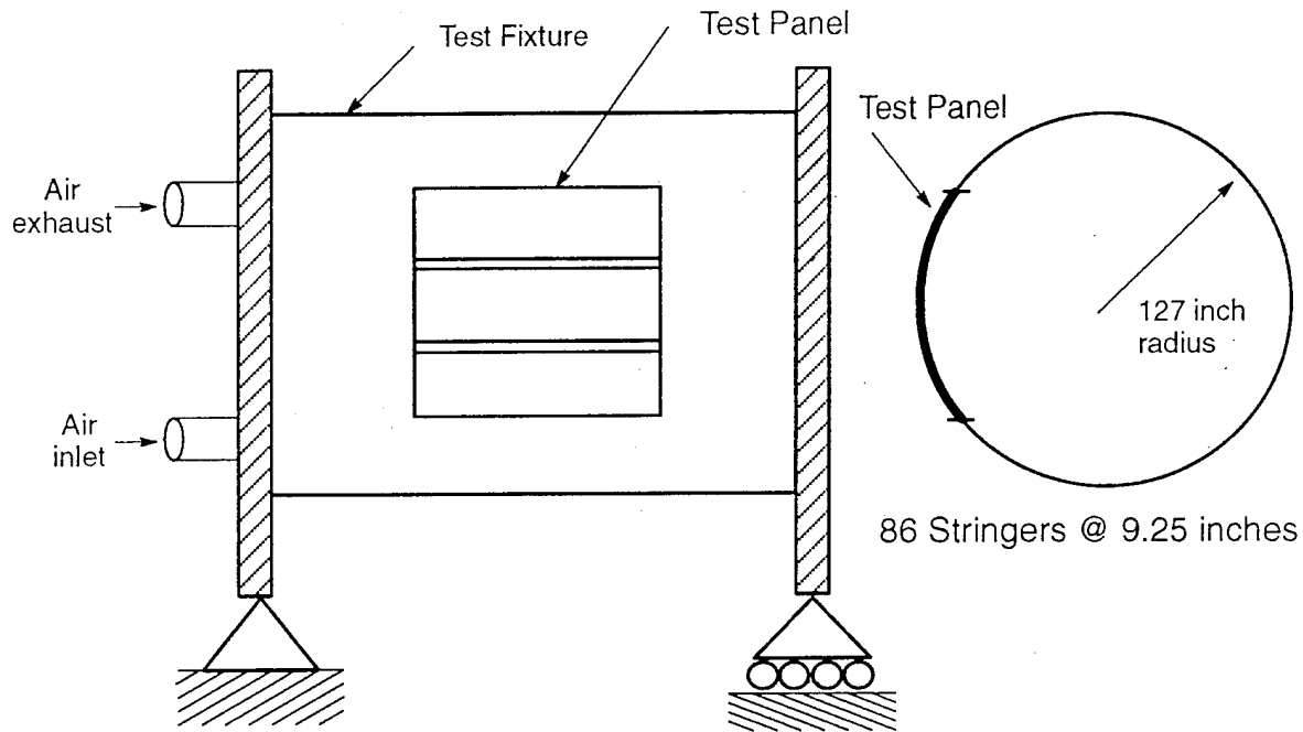
Figure 10. Wide-Body Pressure Test Fixture
