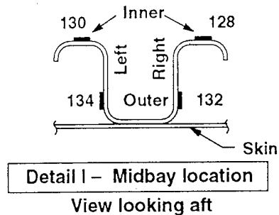
Figure C-7. Stiffener Strain Gage Identification of Panel FAA 1, Tests 1 and 2
