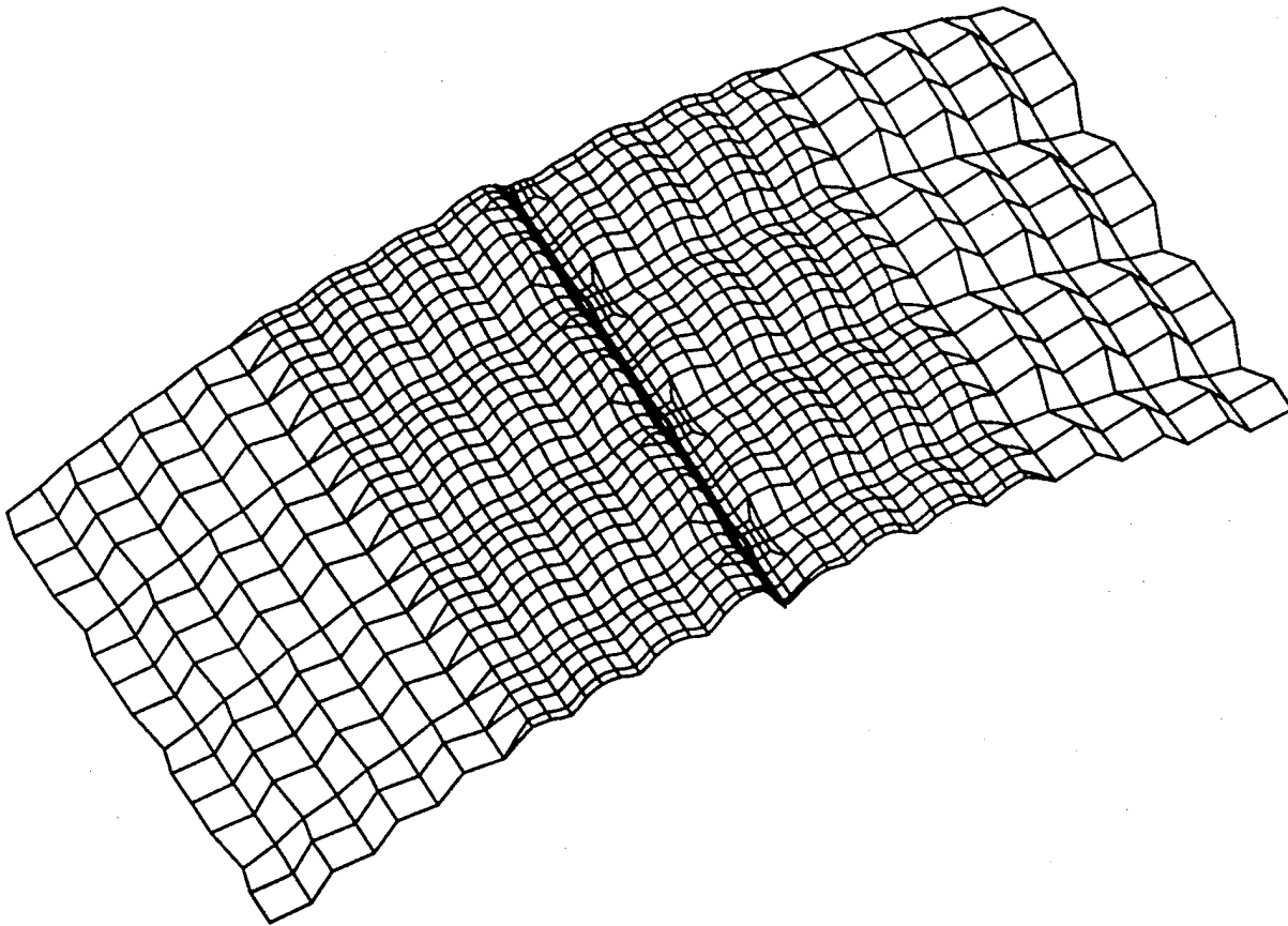
Figure 50. Displaced Intact Skin Mesh, Internal Pressure = 8.6 psi, Magnification Factor \approx 100\times
