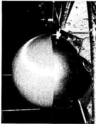
INITIAL KEVLAR-49 FILAMENT WINDINGS APPLIED TO 301 CRES LINER
