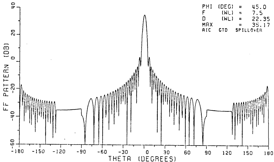
Figure 7c. Full far field pattern of Example 2 computed by OSU Reflector Antenna Code. PHI=45.0 degrees.
