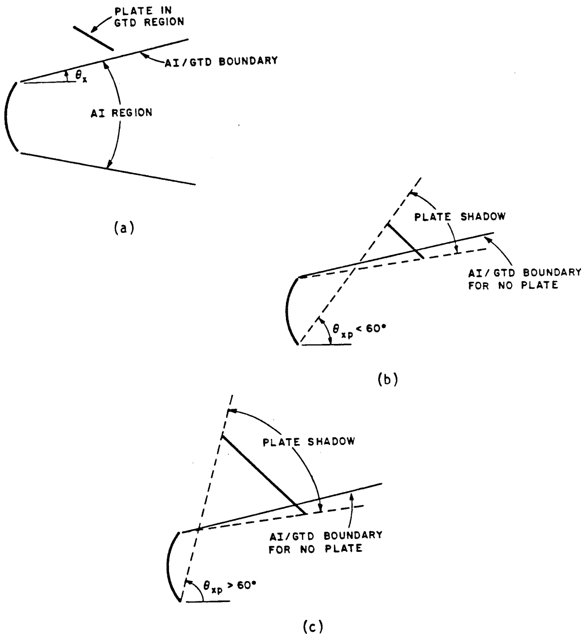
Figure 4. Regions for each source model. a) Plate in the GTD region. The code uses the YSUM model in the AI region and the GTD region, unless LAISC=F or LGTDSC=F. b) Part of plate extends into the AI region adjust AI/GTD switching angle \theta_x > \theta_{xp} (if LAISC=LGTDSC=T). c) Part of plate extends into the AI region and plate shadow extends beyond 60^\circ adjust AI/GTD switching angle \theta_x = 60^\circ (if LAISC=LGTDSC=T).
