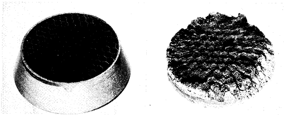
Front surface before test
