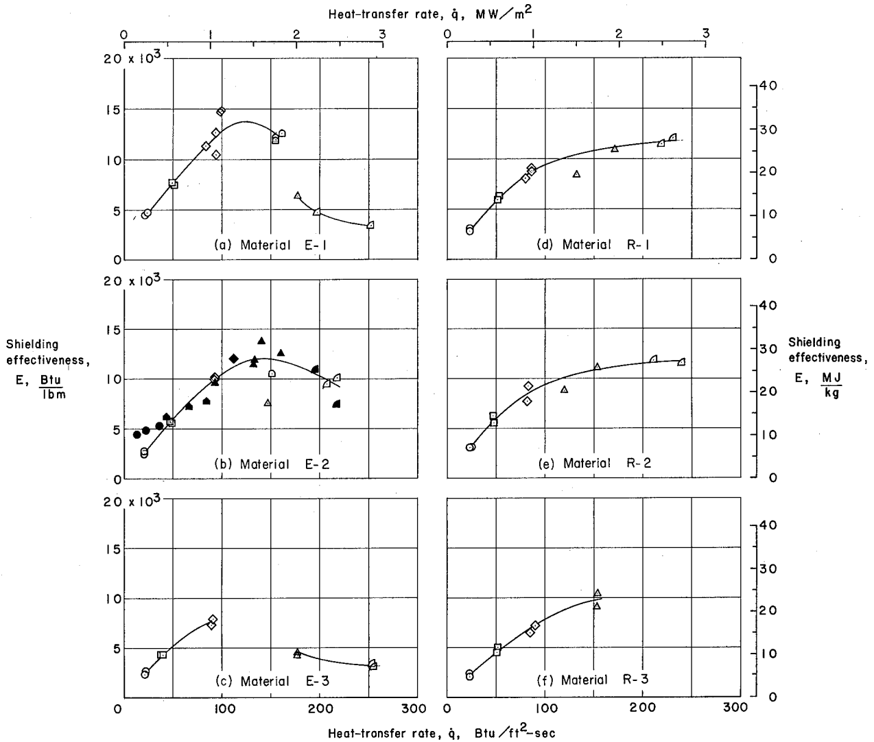
Figure 10.- Shielding effectiveness for a back-surface temperature rise of 300° F (167° K).
