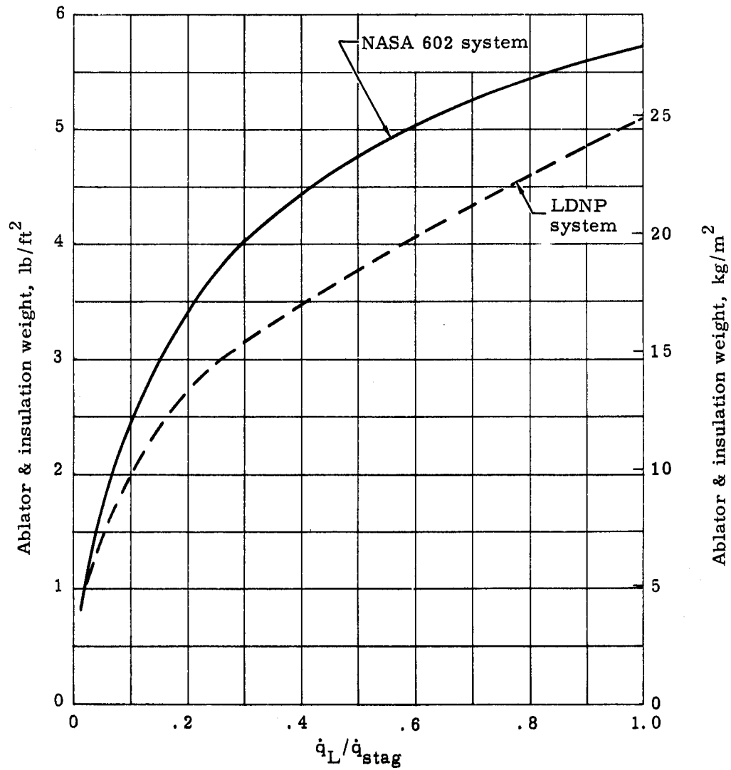
FIGURE 55. HEAT SHIELD WEIGHT CURVE (OVERSHOOT RE-ENTRY TRAJECTORY)
