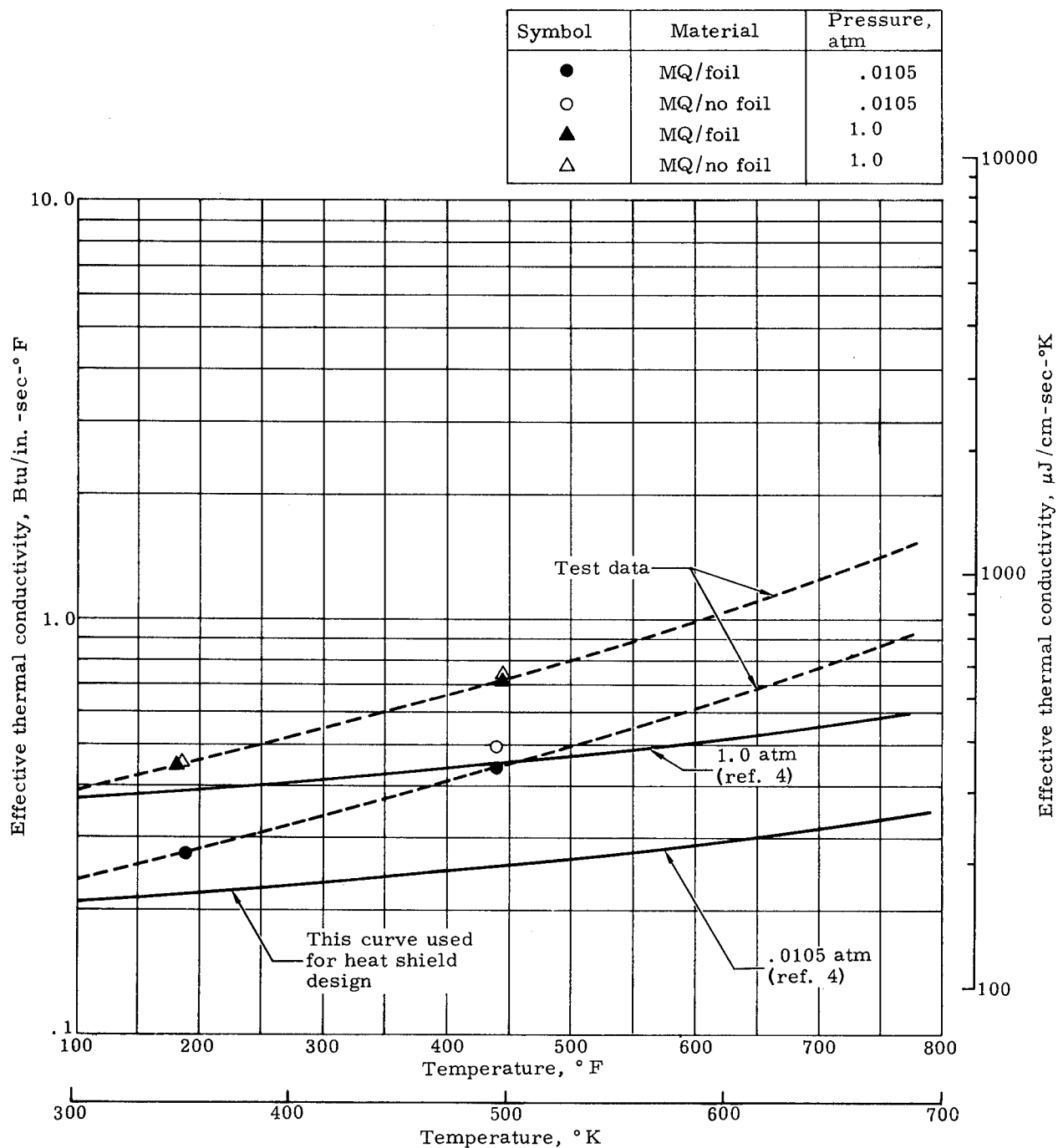
FIGURE 58. COMPARISON OF MICROQUARTZ THERMAL CONDUCTIVITY VALUES
