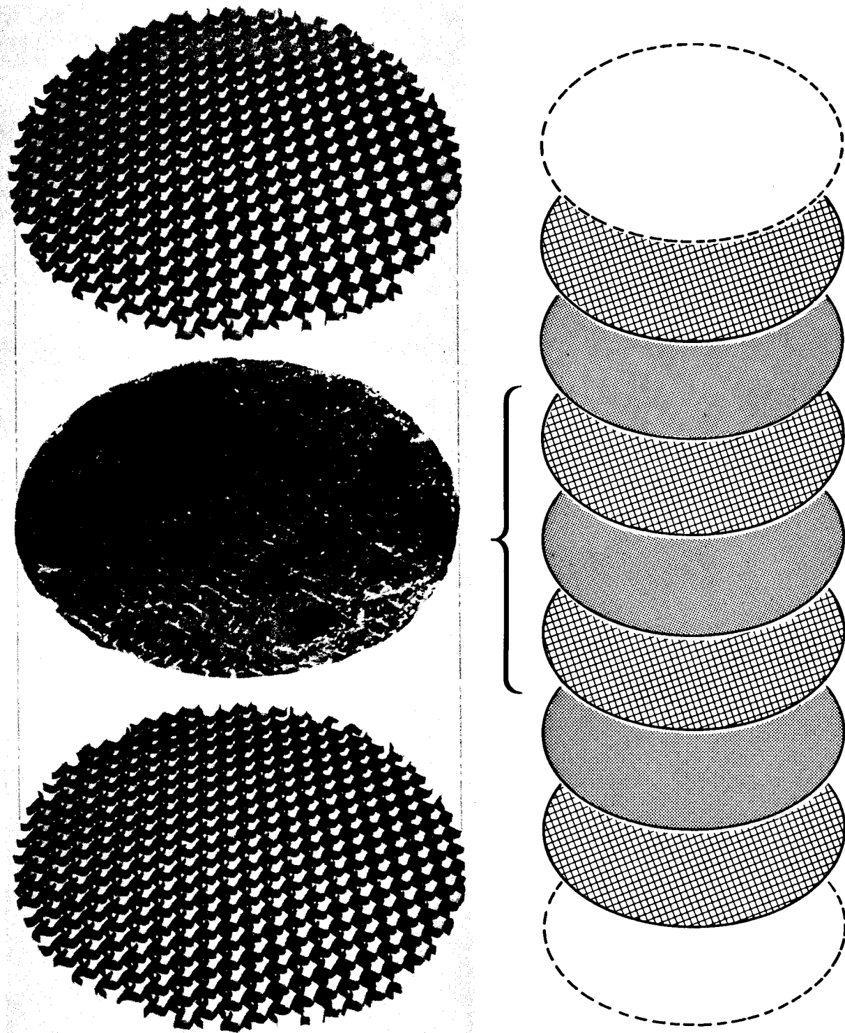
FIGURE 60. INTEGRAL INSULATION/SUPPORT CONCEPT TEST SPECIMEN
