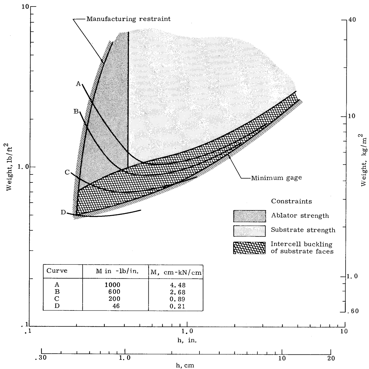
FIGURE 96. DESIGN CONSTRAINT RELATIONSHIPS [17-7PH STEEL SUBSTRATE WITH 1.50-IN. (3.81 CM) NASA 602 ABLATOR, 70° F (294.4° K) CONDITION]
