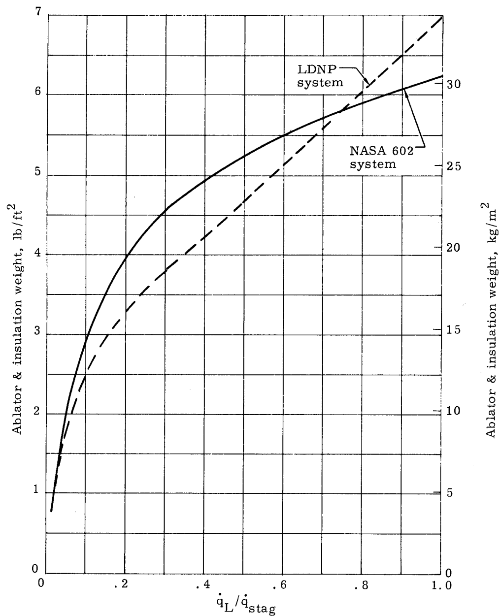
FIGURE 54. HEAT SHIELD WEIGHT CURVE (NOMINAL RE-ENTRY TRAJECTORY)
