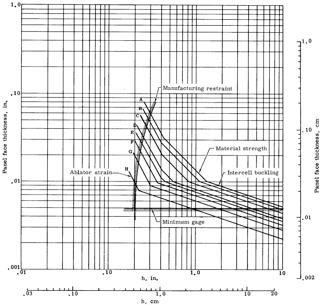
FIGURE 75. SUBSTRATE PANEL DESIGN CONSTRAINTS [17-7PH STEEL SUBSTRATE PANEL WITH 1.50-IN. (3.81 CM) NASA 602 ABLATOR, 70° F (294.4° K) CONDITION]
