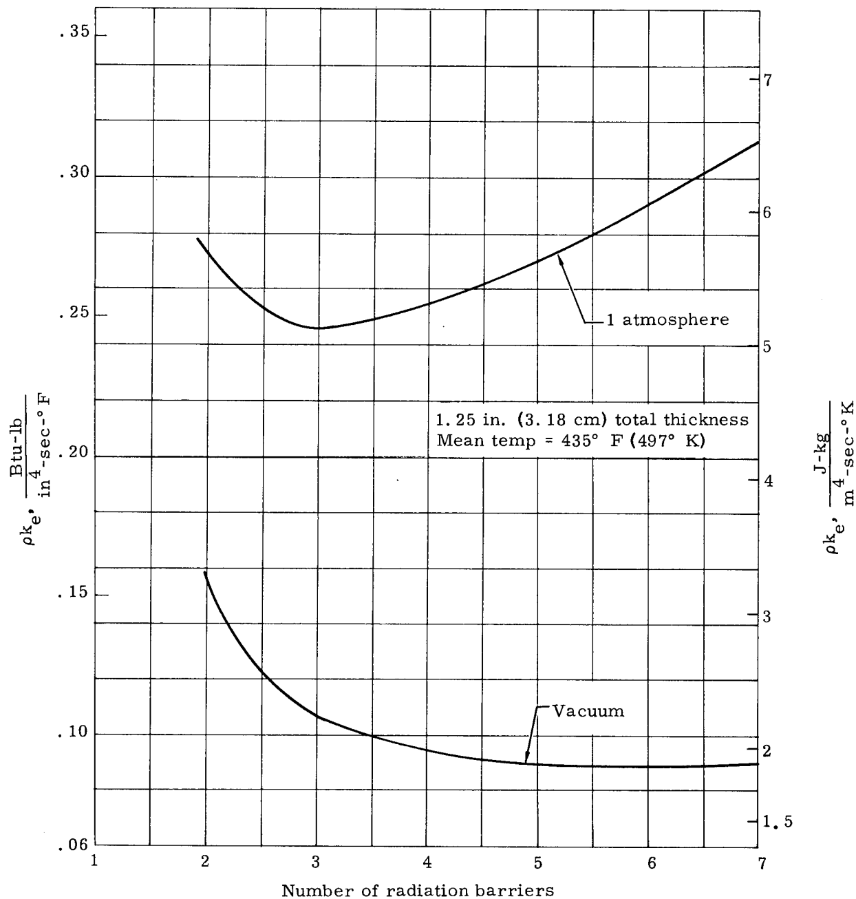
FIGURE 61. FLEXCORE HONEYCOMB/ALUMINUM FOIL INSULATION OPTIMIZATION
