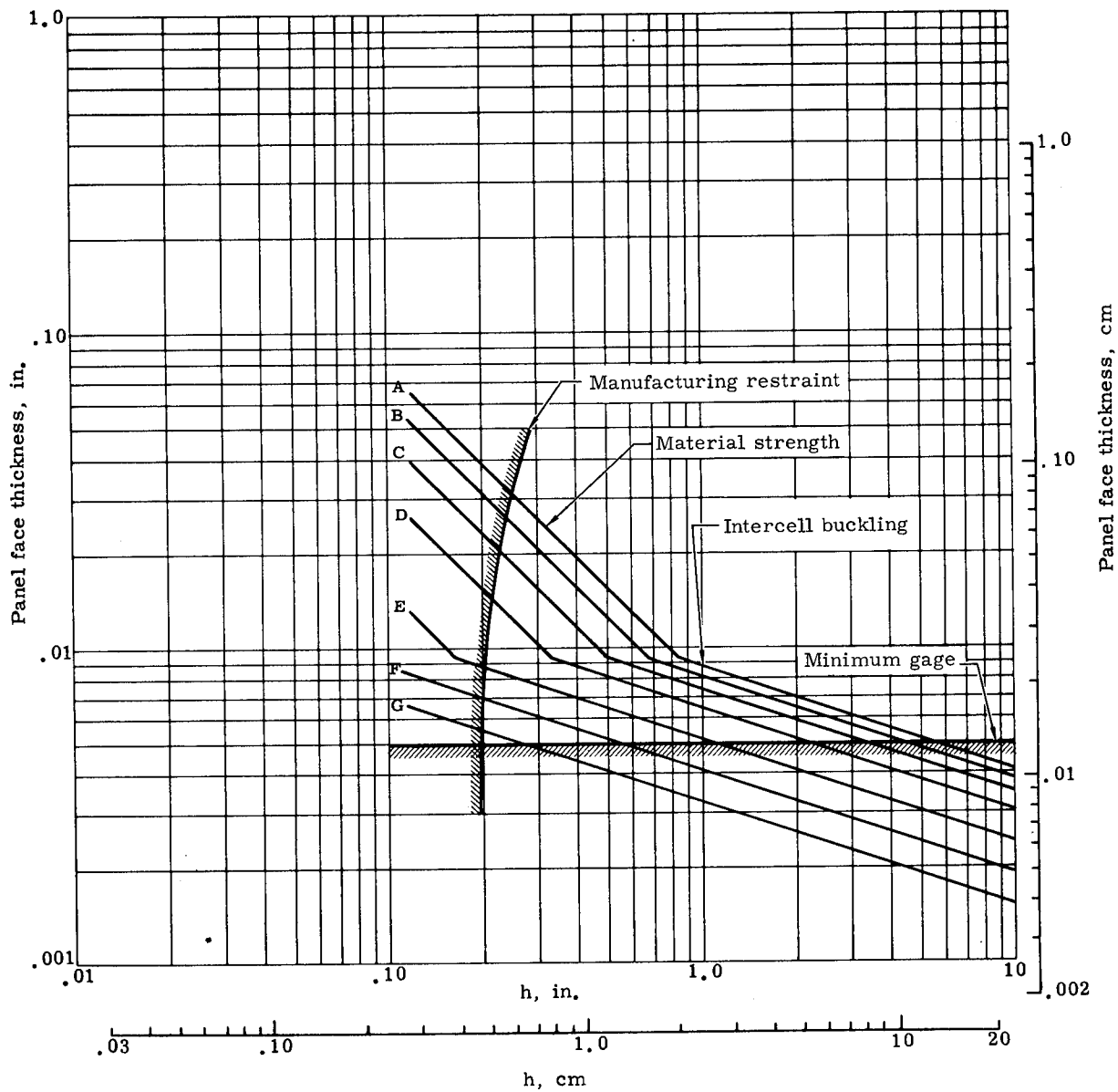
FIGURE 81. SUBSTRATE PANEL DESIGN CONSTRAINTS [17-7PH STEEL SUBSTRATE PANEL, 800° F (700° K) CONDITION]
