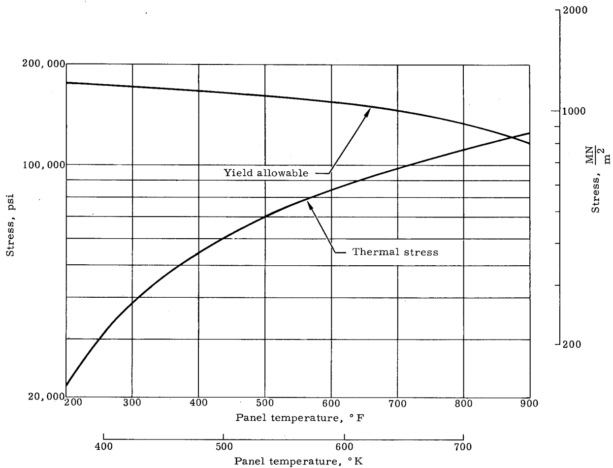
FIGURE 48. THERMAL STRESSES IN RIGIDLY SUPPORTED STAINLESS STEEL SUBSTRATE PANELS
