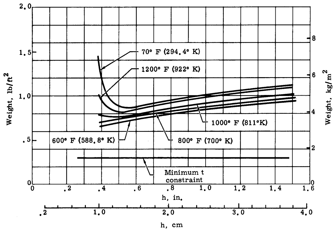
FIGURE 32. STAINLESS STEEL SINGLE SKIN CORRUGATION PANEL OPTIMUM WEIGHT CURVES
