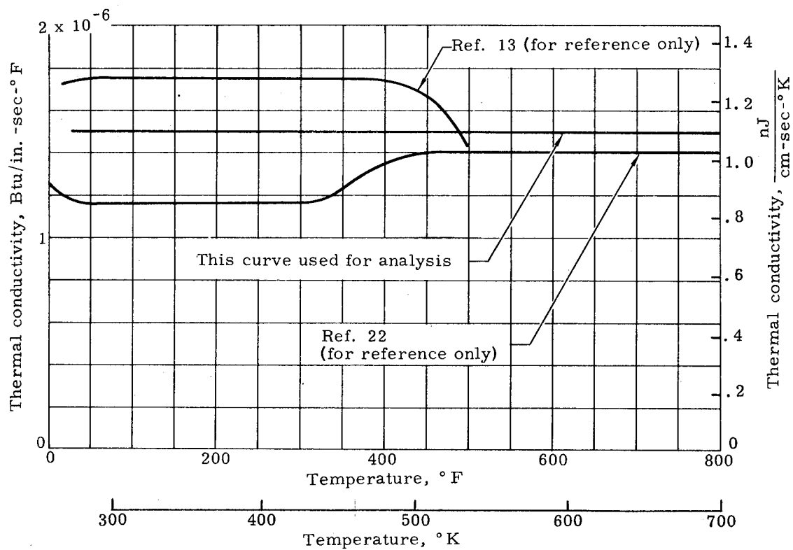
FIGURE 14. LOW DENSITY NYLON PHENOLIC THERMAL CONDUCTIVITY FOR VIRGIN MATERIAL
