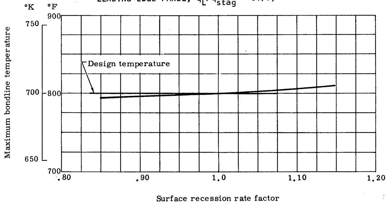
FIGURE 127a. EFFECT OF VARIATION IN CHAR SURFACE RECESSION RATES ON HEAT SHIELD TEMPERATURES (LDNP ABLATOR, OVERSHOOT RE-ENTRY, LEADING EDGE PANEL, \dot{q}_L/\dot{q}_{stag} = 0.70 )
