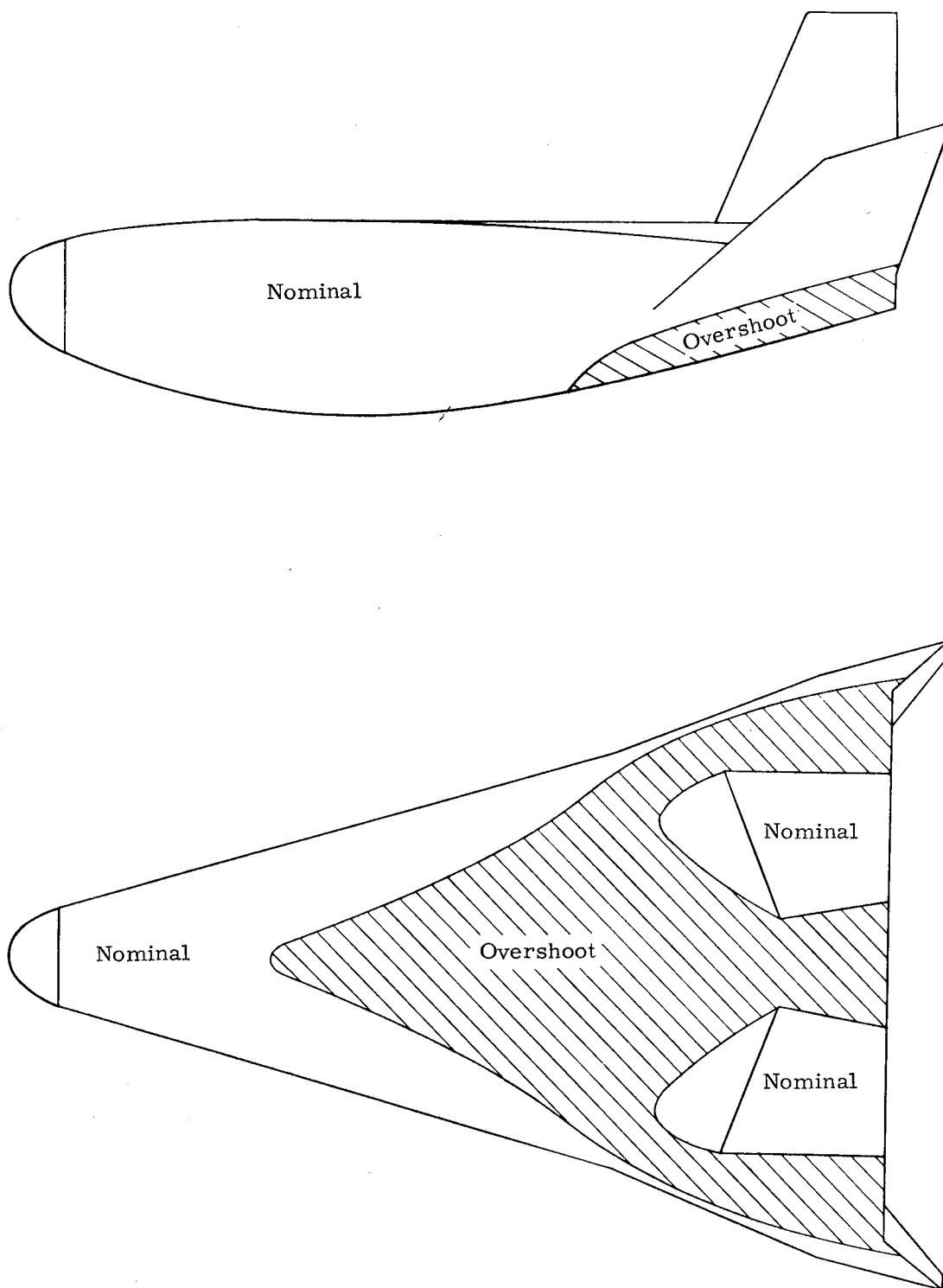
FIGURE 56. CRITICAL TRAJECTORIES FOR ABLATOR THICKNESS DETERMINATION (low density nylon phenolic)
