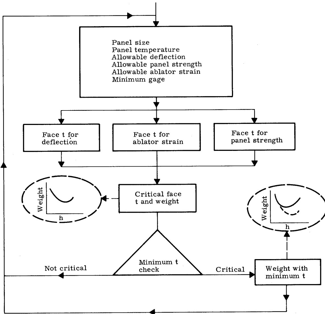
FIGURE 26. HONEYCOMB SUBSTRATE PANEL OPTIMIZATION PROGRAM
