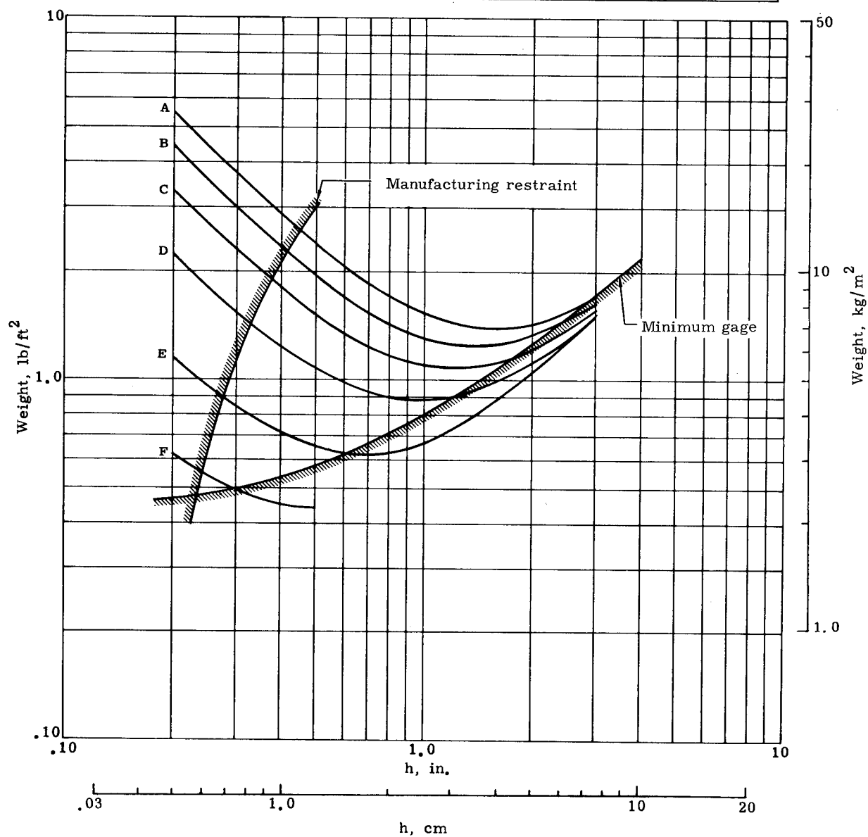
FIGURE 93. SUBSTRATE PANEL DESIGN OPTIMIZATION CURVES [PHENOLIC/GLASS SUBSTRATE PANEL, 800° F (700° K) CONDITION]
