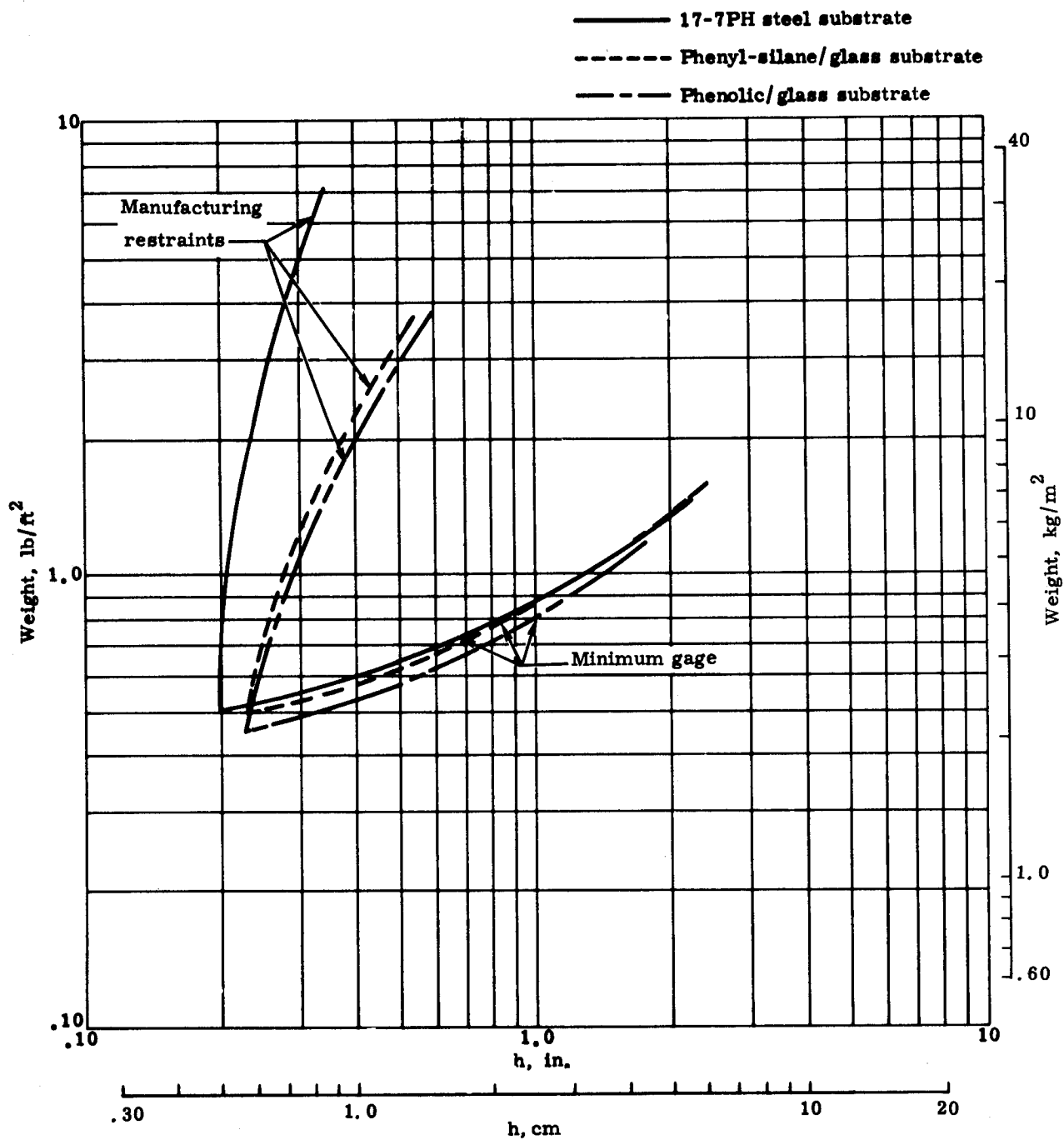
FIGURE 99. SUBSTRATE PANEL DESIGN CORRIDORS
