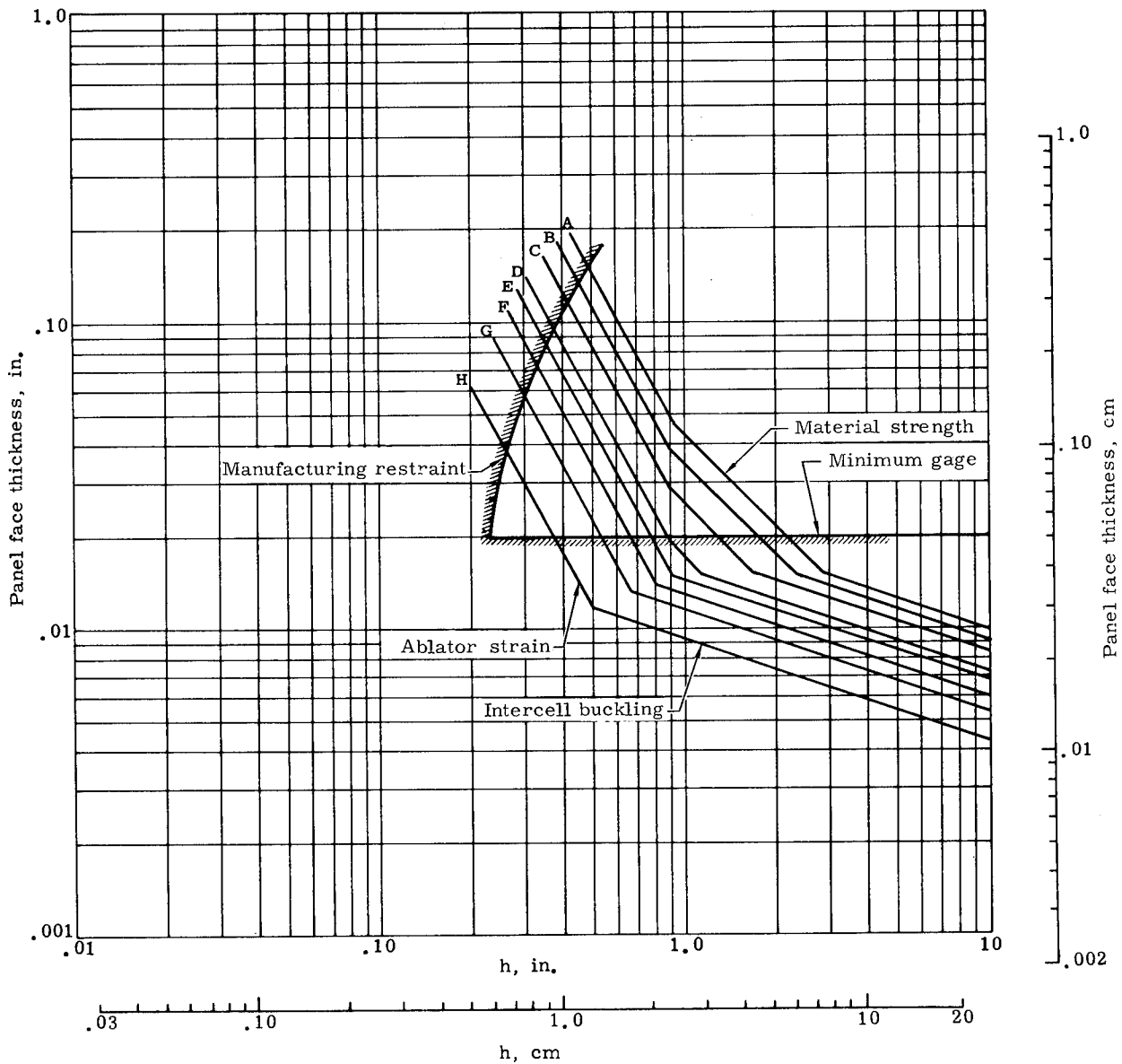
FIGURE 71. SUBSTRATE PANEL DESIGN CONSTRAINTS [PHENOLIC/GLASS SUBSTRATE PANEL WITH 1.50-IN. (3.81 CM) NASA 602 ABLATOR, 70° F (294.4° K) CONDITION]
