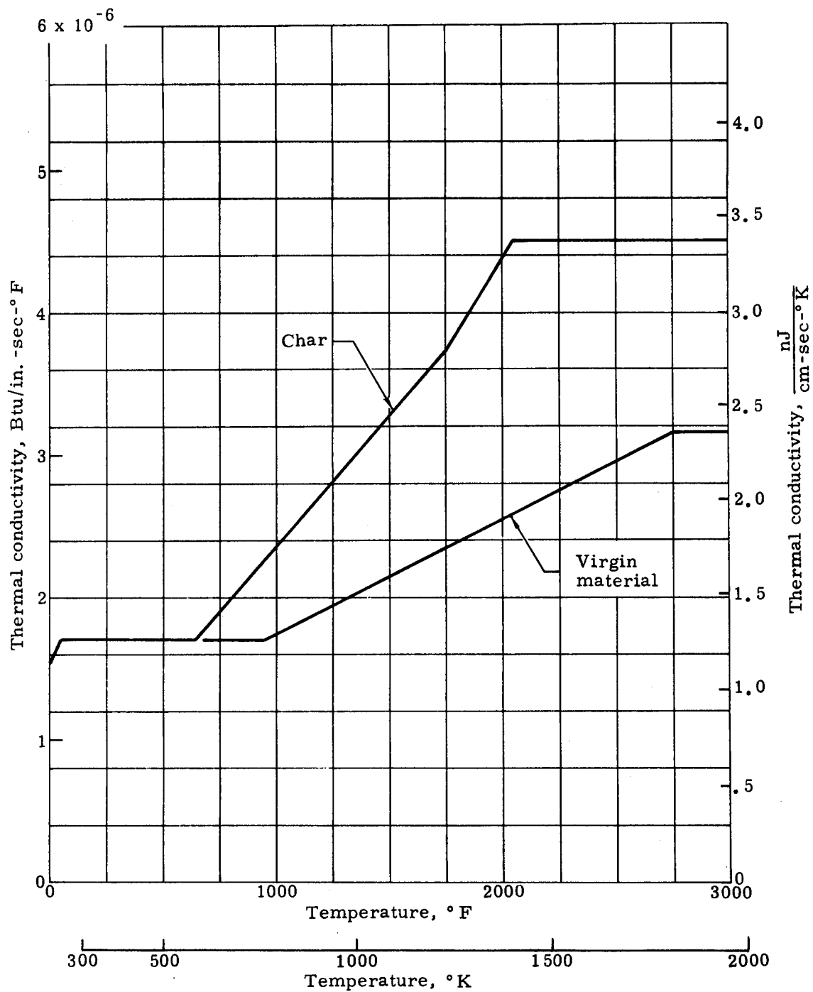
FIGURE 19. NASA 602 THERMAL CONDUCTIVITY
