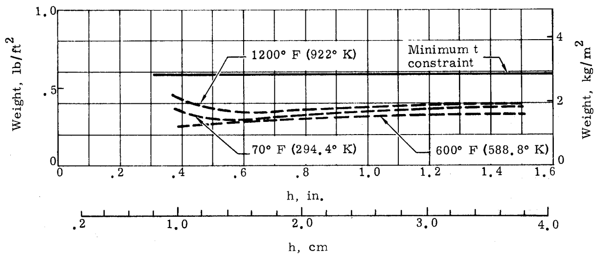
FIGURE 34. BERYLLIUM SINGLE SKIN CORRUGATION PANEL OPTIMUM WEIGHT CURVES
