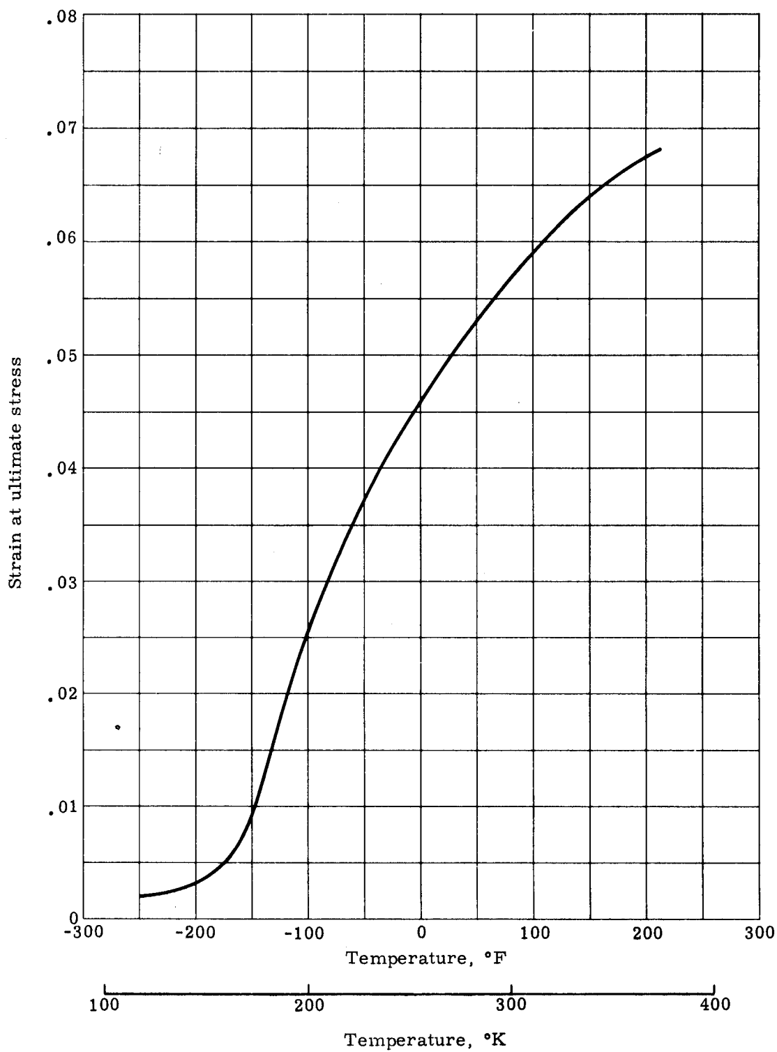
FIGURE 21. NASA 602 IN HONEYCOMB MATRIX ULTIMATE TENSILE STRAIN VERSUS TEMPERATURE (REF. 13)
