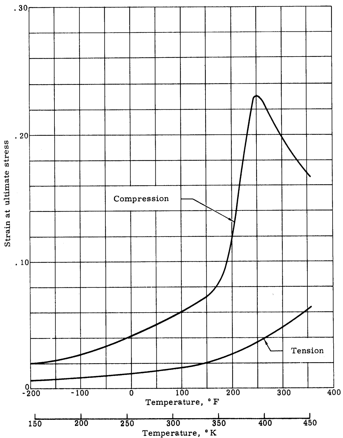
FIGURE 17. LOW DENSITY NYLON PHENOLIC ULTIMATE STRAIN DATA (Ref. 13)
