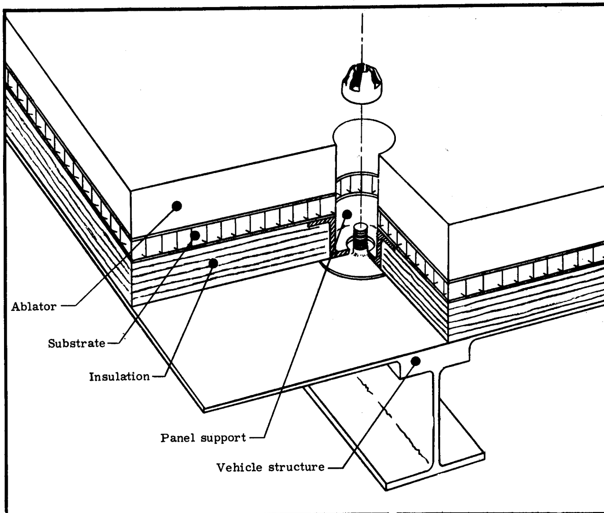
Figure 1. Double Wall Ablative Heat Shield Concept
