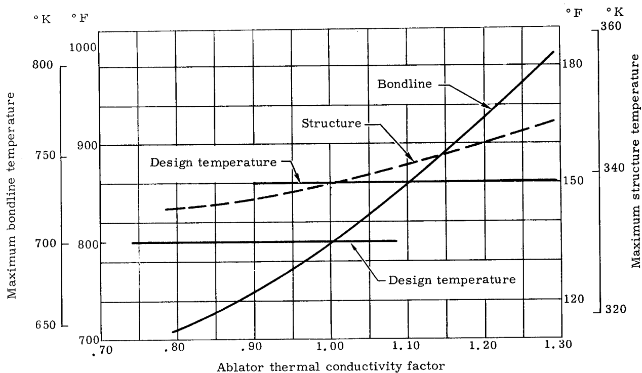
FIGURE 124a. EFFECT OF VARIATION IN ABLATOR THERMAL CONDUCTIVITY ON HEAT SHIELD TEMPERATURES (NASA 602 ABLATOR, OVERSHOOT RE-ENTRY, LEADING EDGE PANEL, \dot{q}_L/\dot{q}_{stag} = 0.70 )
