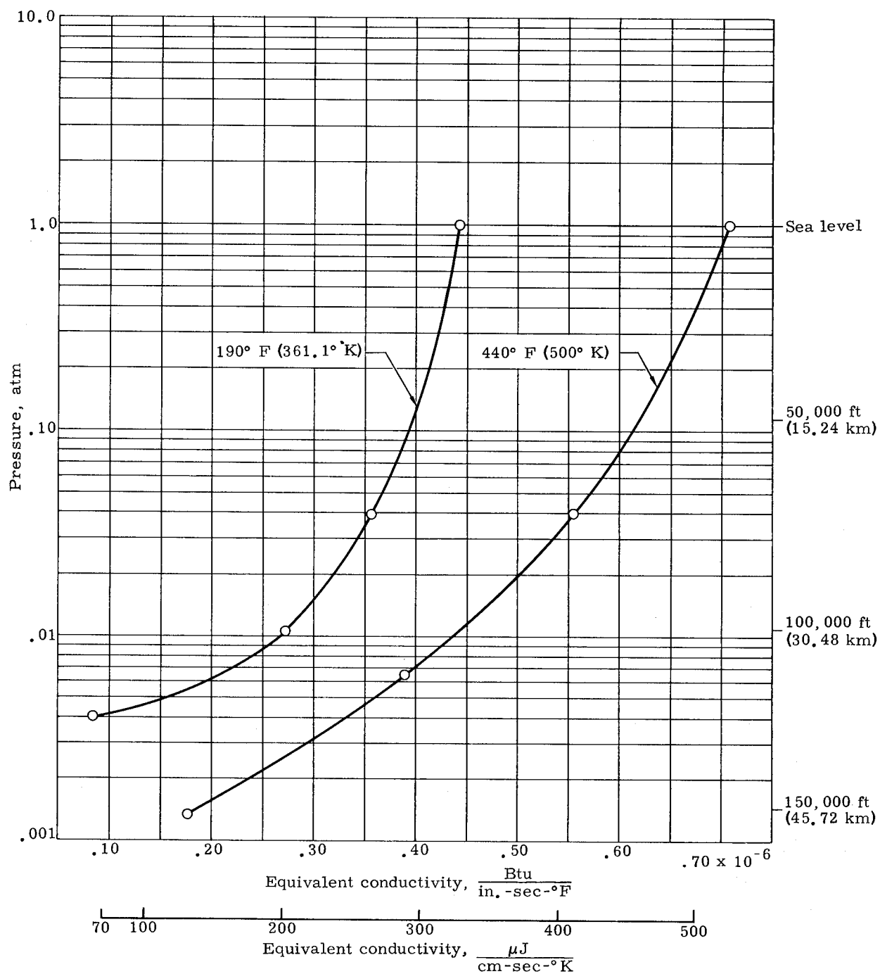
FIGURE 59. PRESSURE DEPENDENCE OF MICROQUARTZ/FOIL INSULATION THERMAL CONDUCTIVITY AT TWO TEMPERATURES
