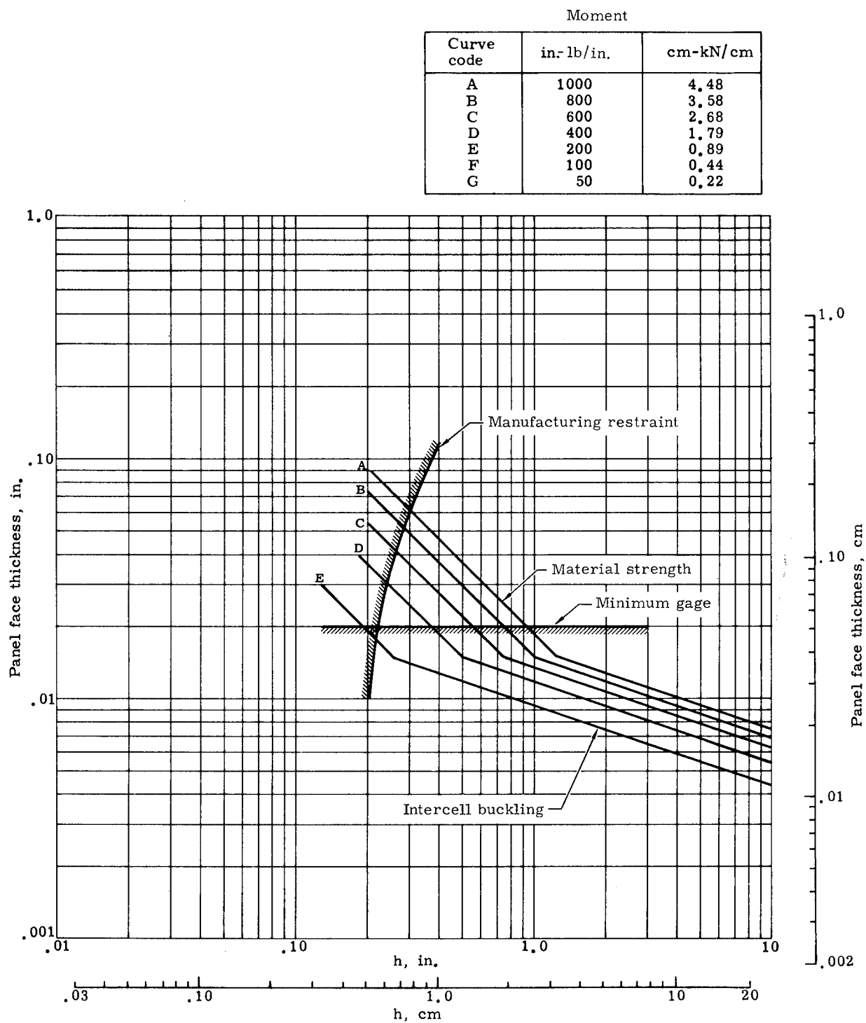
FIGURE 76. SUBSTRATE PANEL DESIGN CONSTRAINTS [PHENOLIC/GLASS SUBSTRATE PANEL, 300° F (422.2° K) CONDITION]
