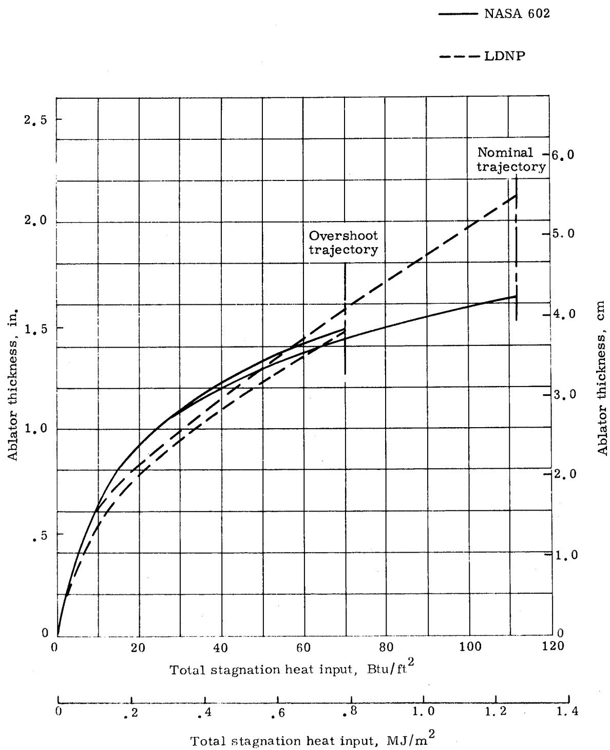
FIGURE 53. COMPARISON OF ABLATOR THICKNESS DESIGN CURVES ON A TOTAL HEAT BASIS
