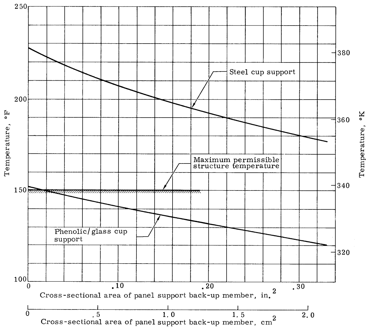
FIGURE 66. MAXIMUM STRUCTURE TEMPERATURE AT TOUCHDOWN WITH HEAT SHORT EFFECT CONSIDERED
