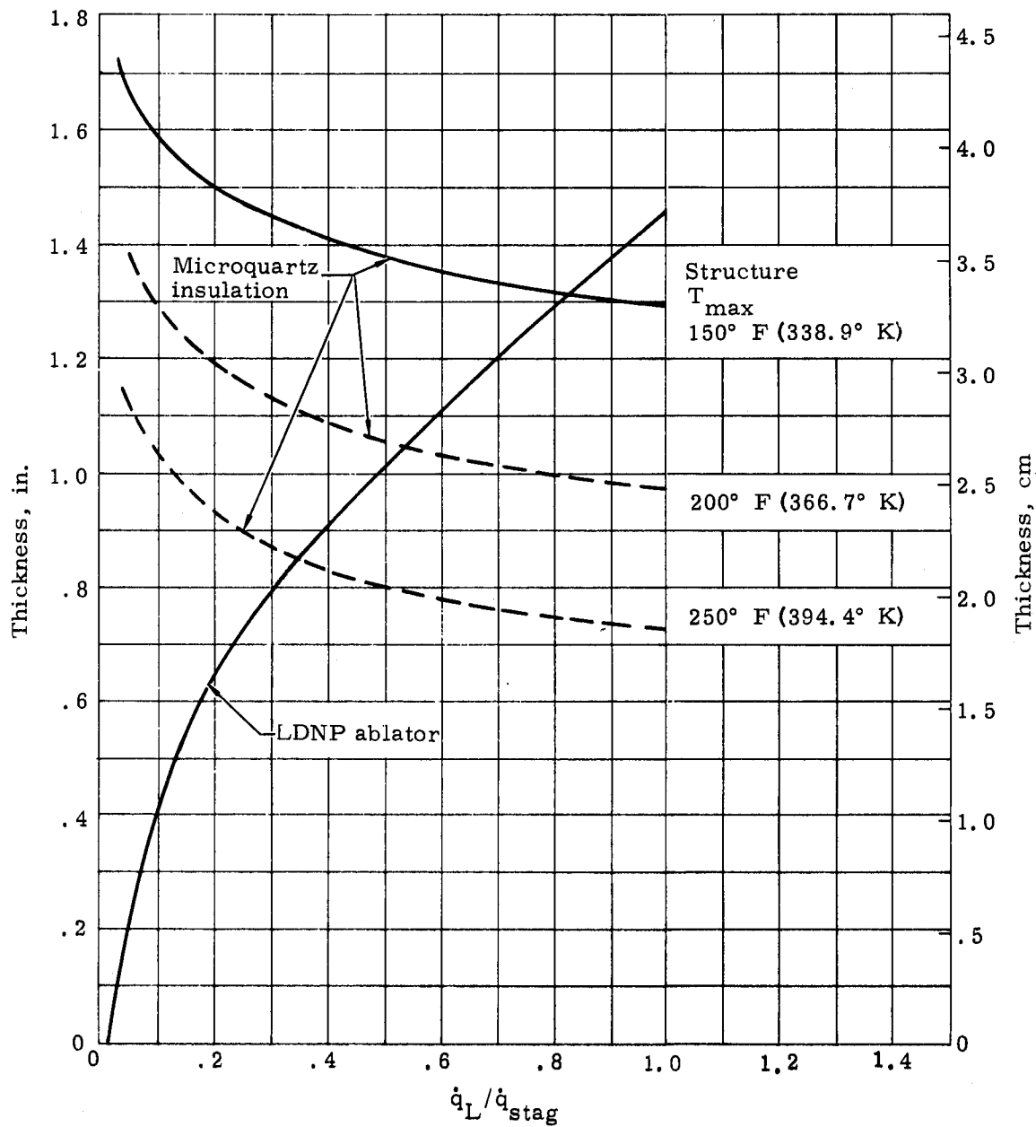
FIGURE 51. HEAT SHIELD DESIGN CURVE (OVERSHOOT TRAJECTORY, LDNP ABLATOR)
