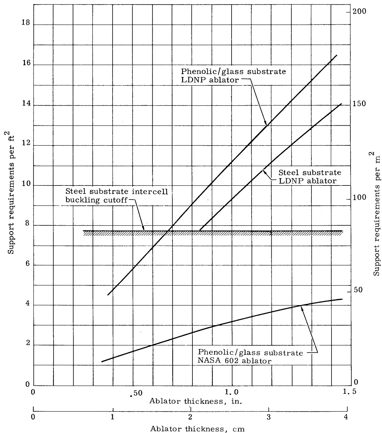
FIGURE 101. PANEL SUPPORT REQUIREMENTS FOR OPTIMUM MOMENTS [70°F (294.4°K) CONDITION, 12 PSI (82.74 kN/m 2 ) PRESSURE]
