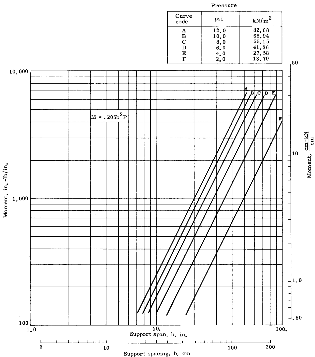
FIGURE 102. CRITICAL PANEL MOMENT VERSUS SUPPORT SPAN AND PRESSURE ASPECT RATIO = 1.0 = a/b
