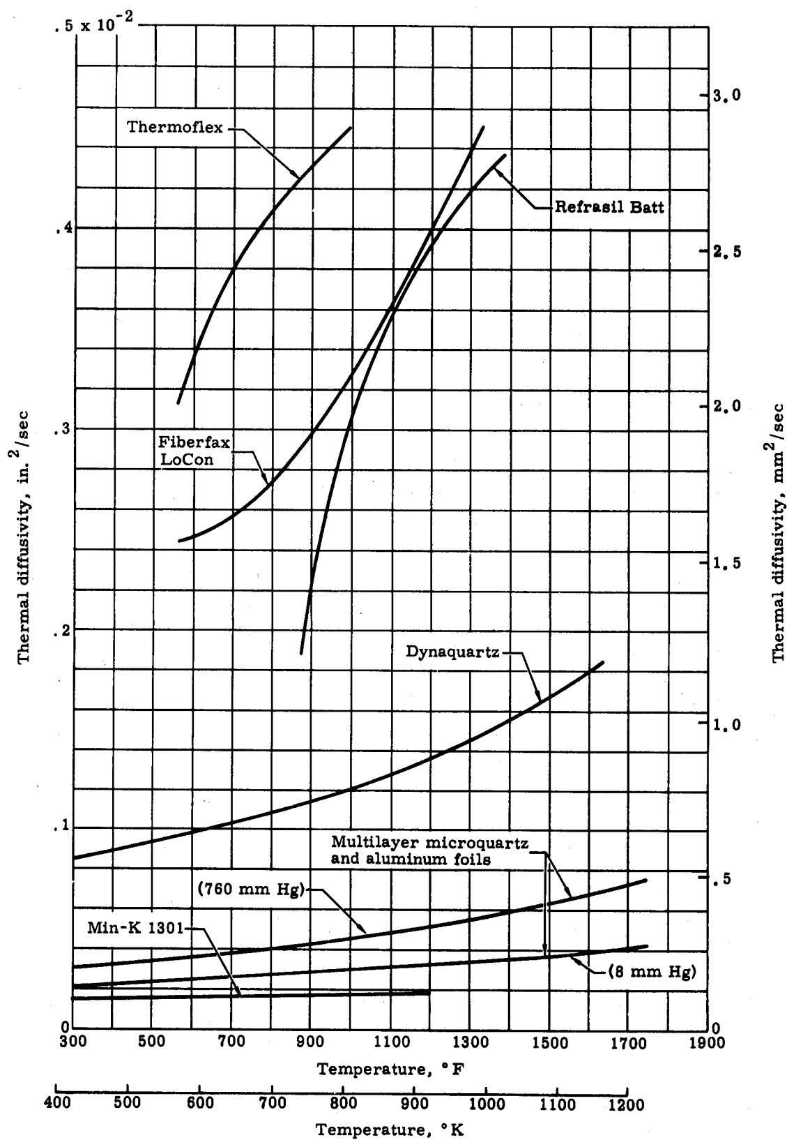
FIGURE 10. CANDIDATE INSULATION MATERIALS (THERMAL DIFFUSIVITY VERSUS TEMPERATURE) (Refs. 4 and 21)
