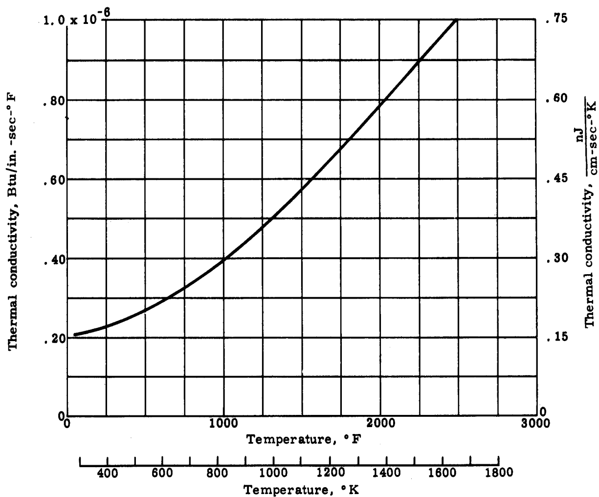
FIGURE 12. MULTILAYER MICROQUARTZ THERMAL CONDUCTIVITY VERSUS TEMPERATURE AT 8mm Hg (Ref. 4)
