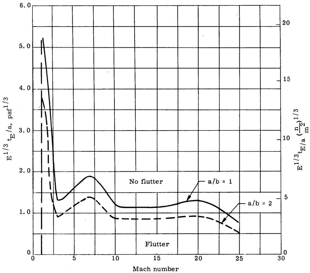
FIGURE 107. HL-10 FLUTTER ENVELOPE
