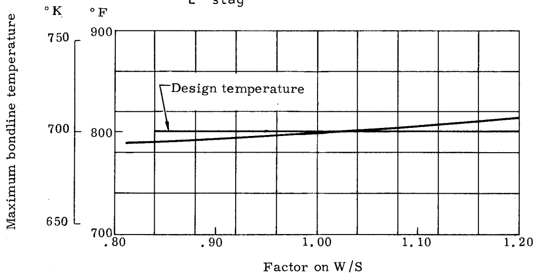
FIGURE 122a. EFFECT OF VARIATION IN VEHICLE W/S ON HEAT SHIELD TEMPERATURES (NASA 602 ABLATOR, NOMINAL RE-ENTRY, LEADING EDGE PANEL, \dot{q}_L/\dot{q}_{stag} = 0.565 )
