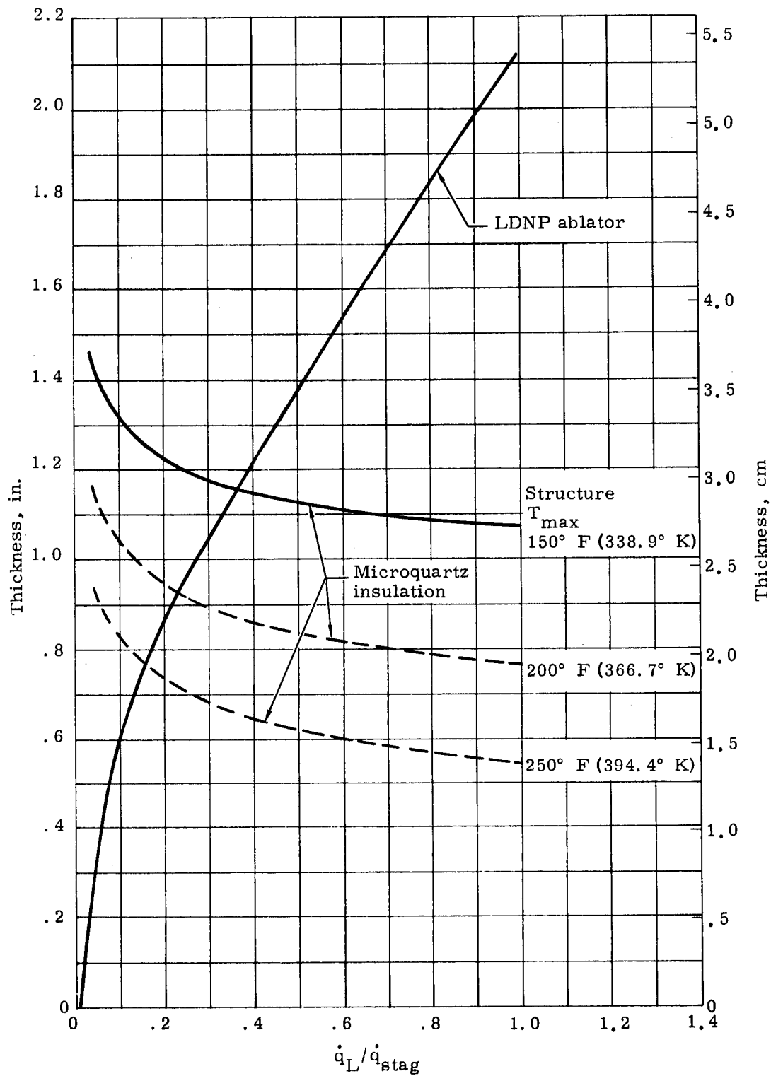
FIGURE 49. HEAT SHIELD DESIGN CURVE (NOMINAL TRAJECTORY, LDNP ABLATOR)
