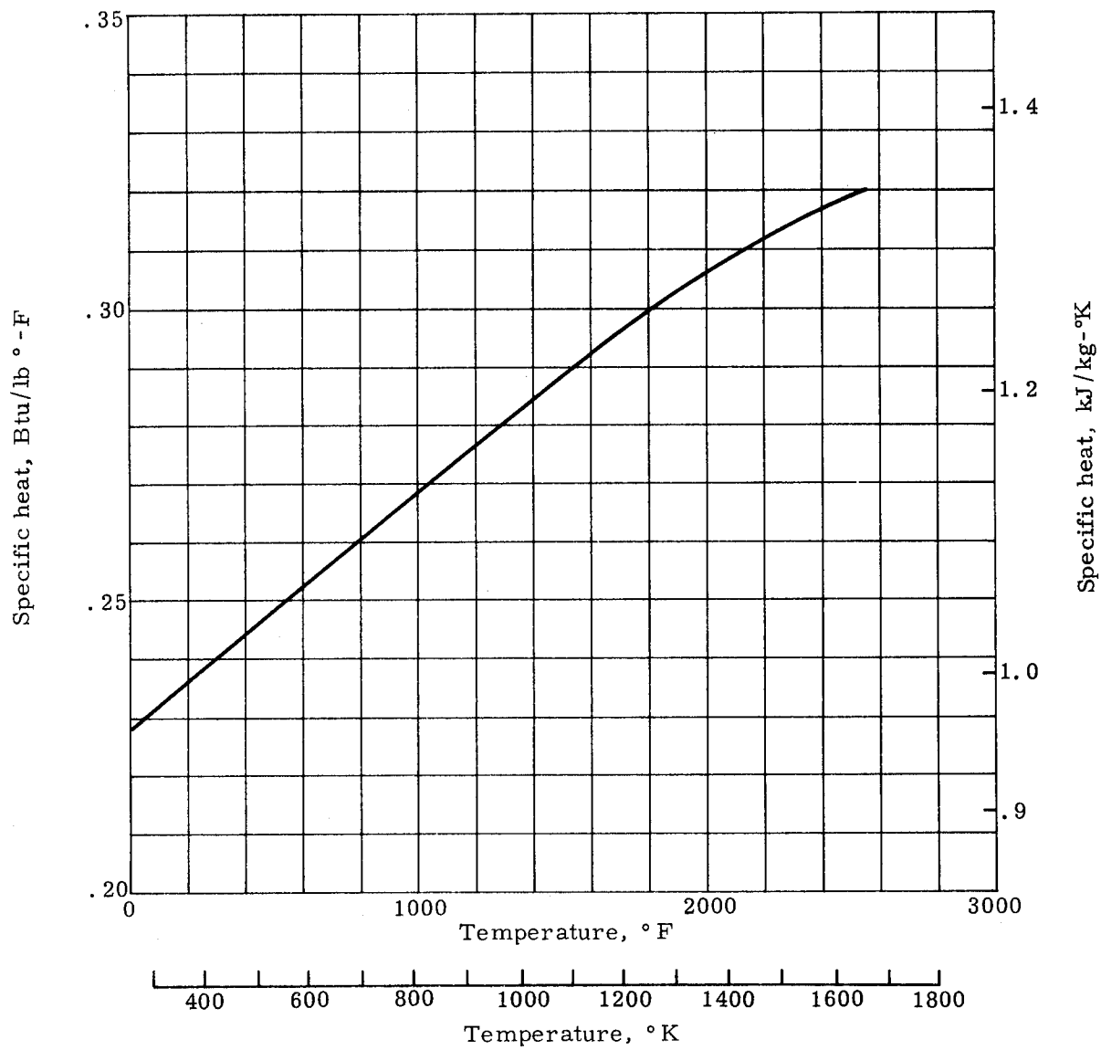
FIGURE 11. MULTILAYER MICROQUARTZ SPECIFIC HEAT VERSUS TEMPERATURE (Ref. 4)
