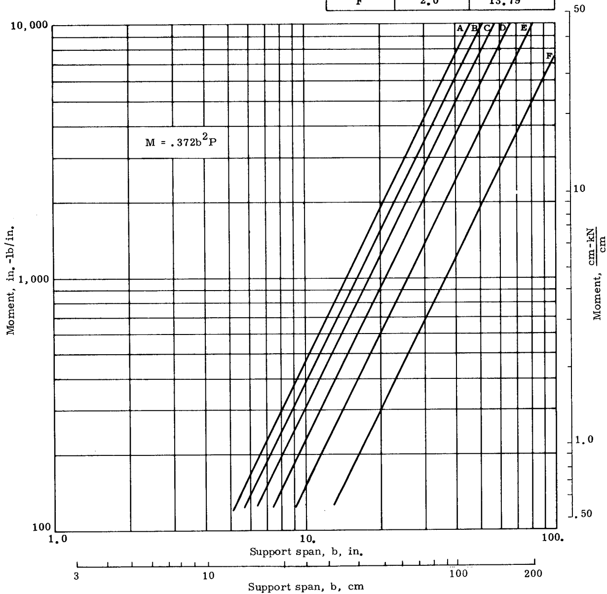
FIGURE 103. CRITICAL PANEL MOMENT VERSUS SUPPORT SPAN AND PRESSURE ASPECT RATIO = 1.5 = a/b
