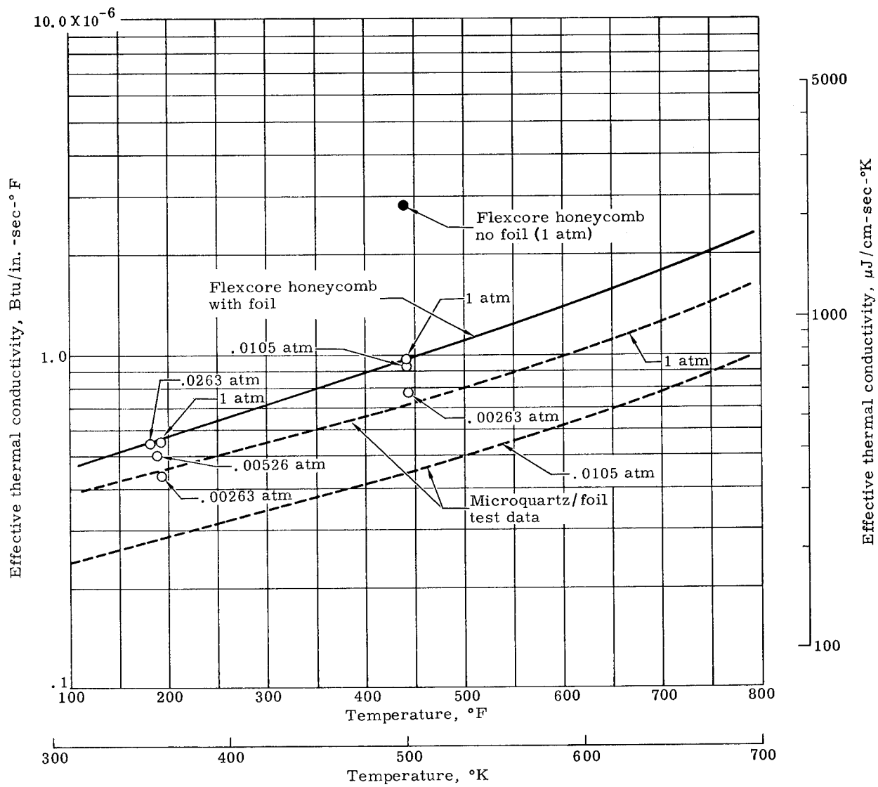
FIGURE 62. EFFECTIVE THERMAL CONDUCTIVITY VERSUS TEMPERATURE AND PRESSURE FOR FLEXCORE HONEYCOMB WITH ALUMINUM FOIL
