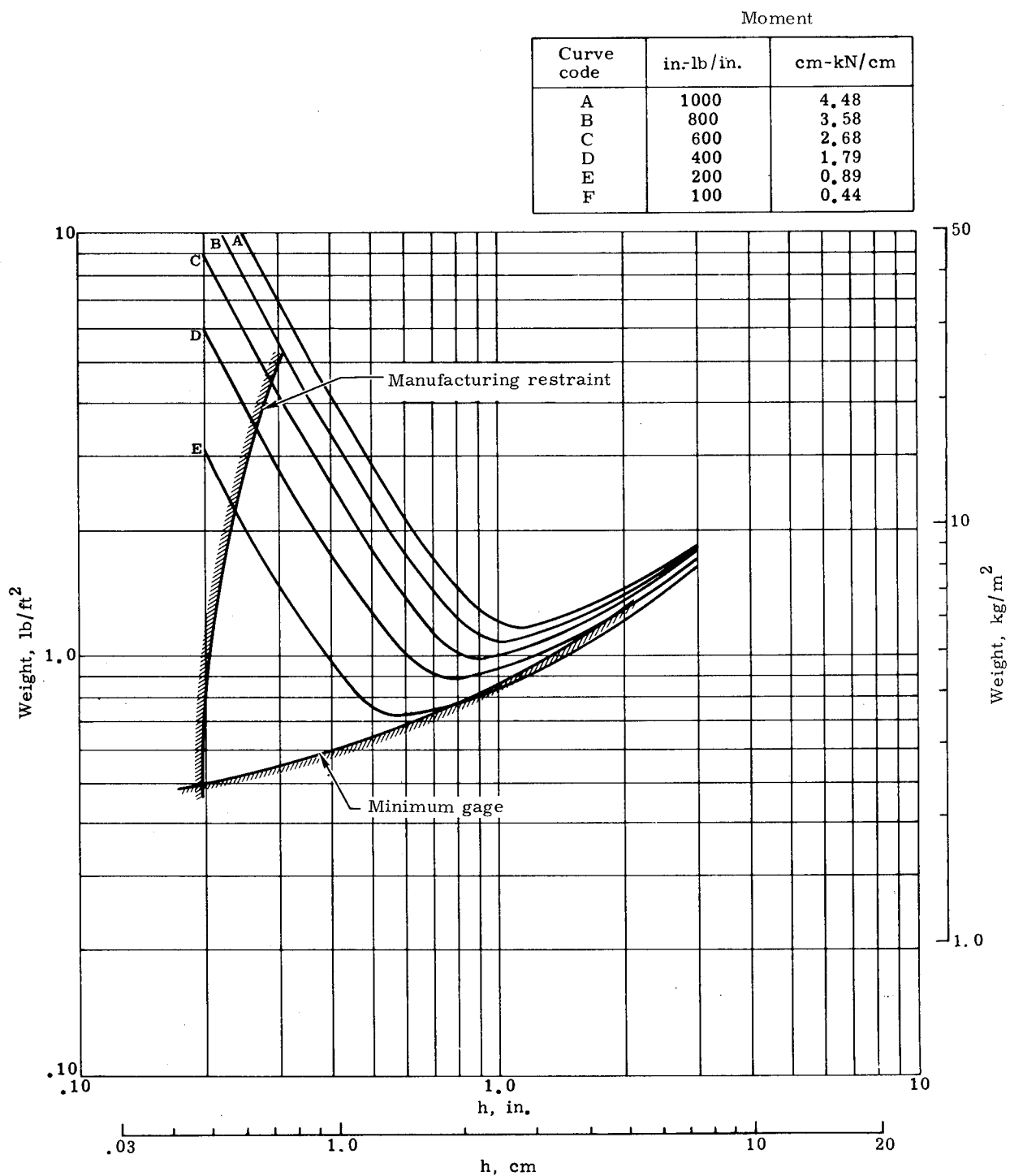
FIGURE 87. SUBSTRATE PANEL DESIGN OPTIMIZATION CURVES [17-7PH STEEL SUBSTRATE WITH 1.50-IN. (3.81 CM) LDNP ABLATOR, 70° F (294.4° K) CONDITION]
