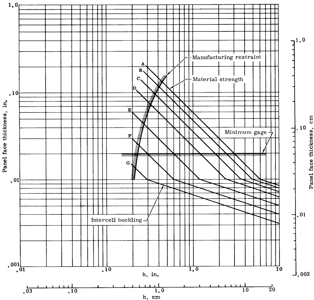
FIGURE 79. SUBSTRATE PANEL DESIGN CONSTRAINTS [PHENOLIC/GLASS SUBSTRATE PANEL, 800° F (700° K) CONDITION]
