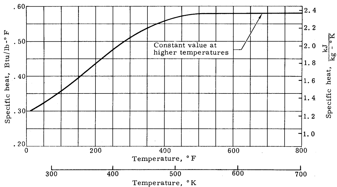
FIGURE 13. LOW DENSITY NYLON PHENOLIC SPECIFIC HEAT FOR VIRGIN AND CHAR MATERIAL (Ref. 13)
