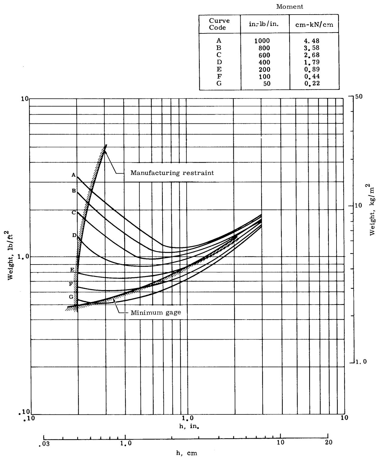
FIGURE 95. SUBSTRATE PANEL DESIGN OPTIMIZATION CURVES [17-7PH STEEL SUBSTRATE PANEL, 800° F (700° K) CONDITION]
