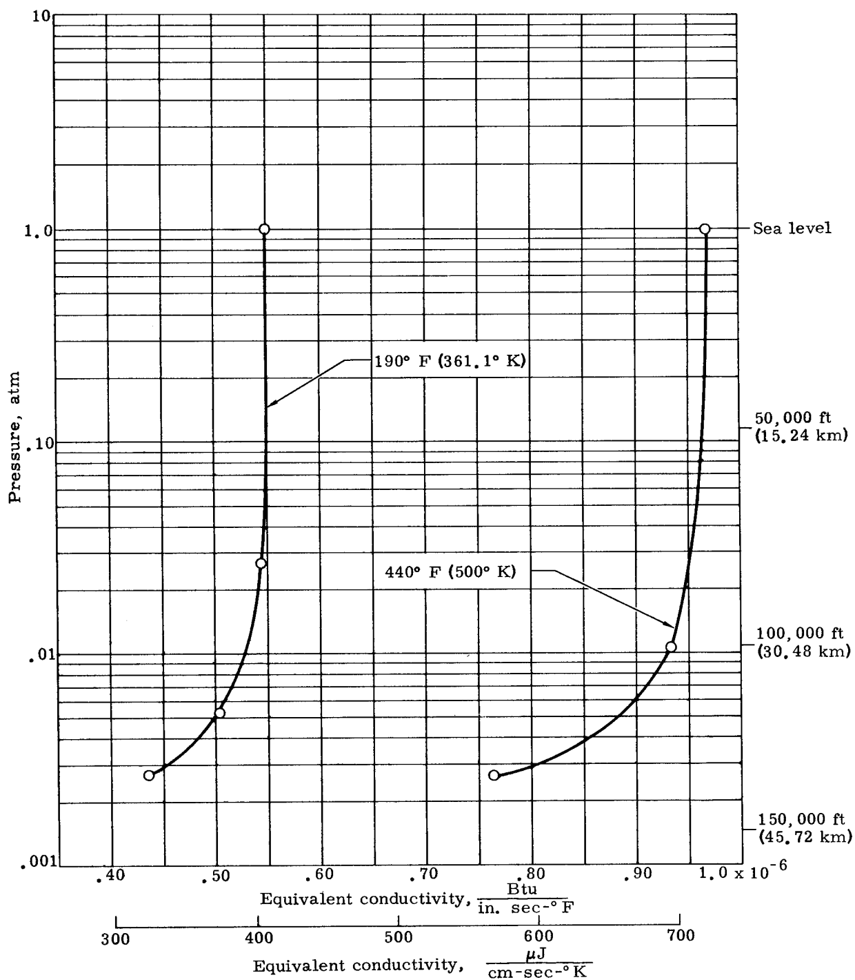
FIGURE 63. PRESSURE DEPENDENCE OF FLEXCORE HONEYCOMB WITH FOIL INSULATION THERMAL CONDUCTIVITY AT TWO TEMPERATURES
