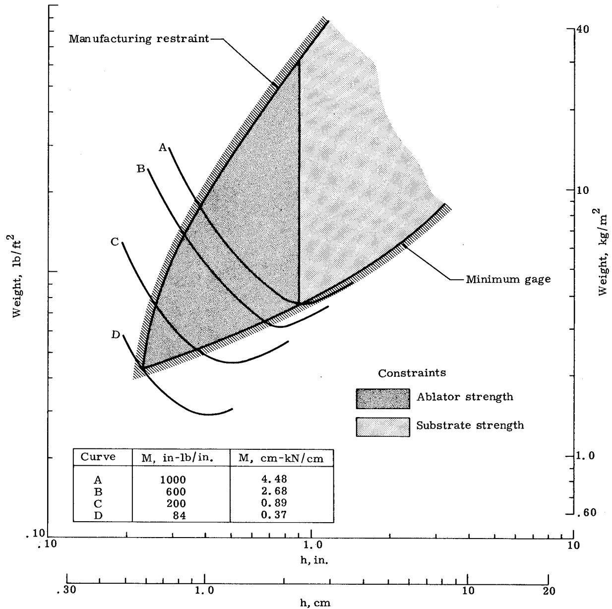
FIGURE 97. DESIGN CONSTRAINT RELATIONSHIPS [PHENOLIC/GLASS SUBSTRATE WITH 1.50-IN. (3.81 CM) NASA 602 ABLATOR, 70° F (294.4° K) CONDITION]
