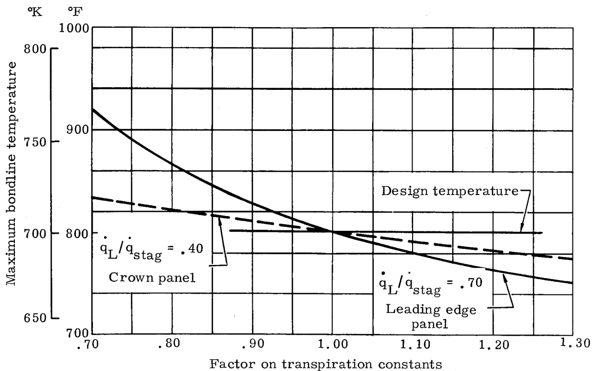
FIGURE 129a. EFFECT OF VARIATION OF TRANSPARATION FACTOR ON HEAT SHIELD TEMPERATURES (LDNP ABLATOR, OVERSHOOT RE-ENTRY)
