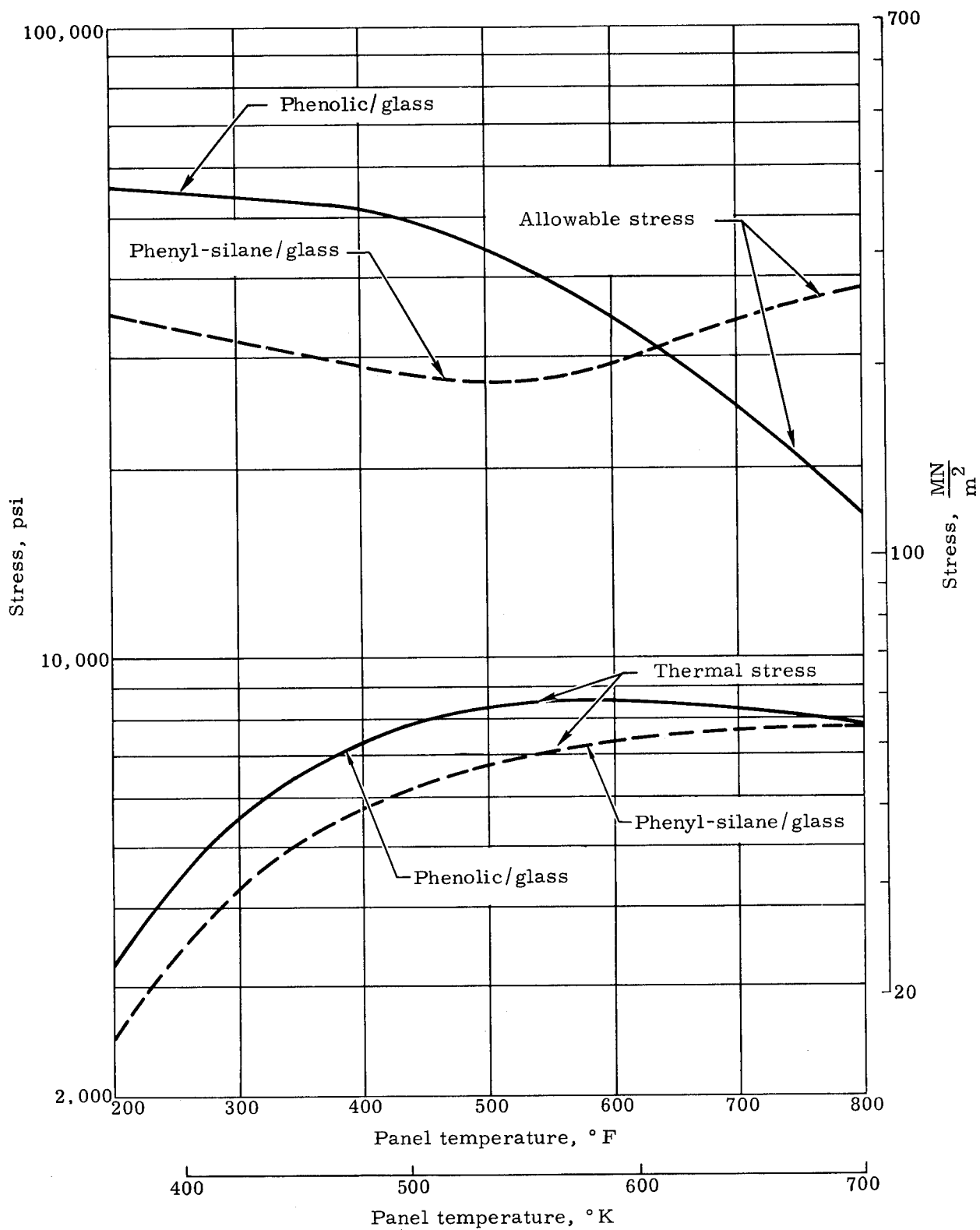
FIGURE 47. THERMAL STRESSES IN RIGIDLY SUPPORTED PLASTIC LAMINATE SUBSTRATE PANELS
