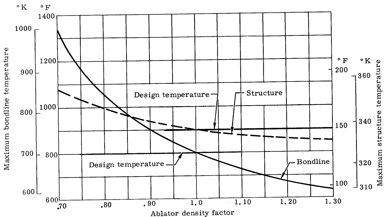
FIGURE 126a. EFFECT OF VARIATION IN ABLATOR DENSITY ON HEAT SHIELD TEMPERATURES (NASA 602 ABLATOR, OVERSHOOT RE-ENTRY, LEADING EDGE PANEL, q_L/q_{stag} = 0.70 )
