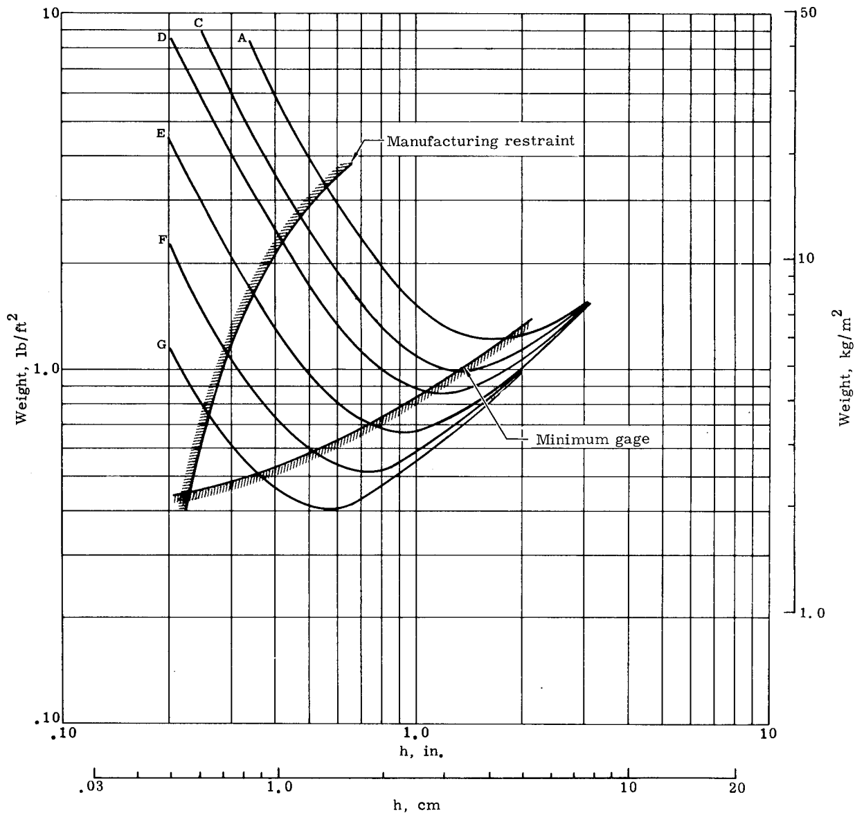
FIGURE 83. SUBSTRATE PANEL DESIGN OPTIMIZATION CURVES [PHENOLIC/GLASS SUBSTRATE WITH 1.50-IN. (3.81 CM) LDNP ABLATOR, 70° F (294.4°K) CONDITION]
