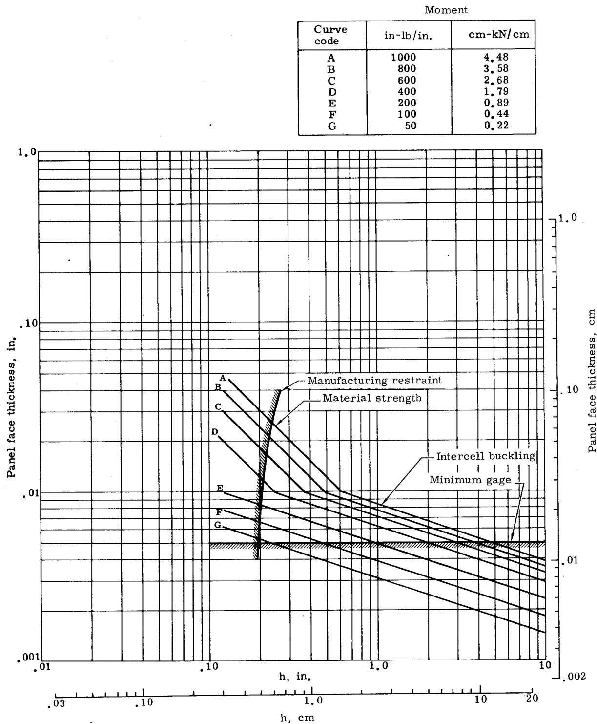
FIGURE 78. SUBSTRATE PANEL DESIGN CONSTRAINTS [17-7PH STEEL SUBSTRATE PANEL, 300° F (422.2° K) CONDITION]
