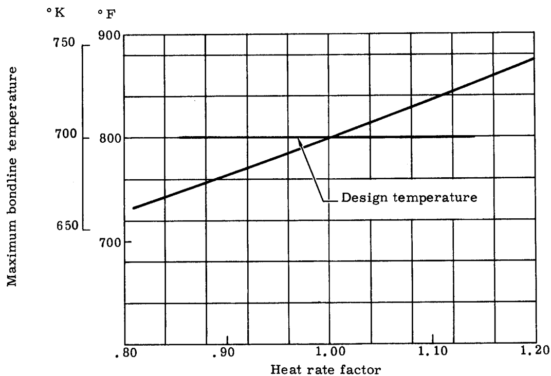
FIGURE 121a. EFFECT OF VARIATION IN HEAT RATE FACTOR ON HEAT SHIELD TEMPERATURES (NASA 602 ABLATOR, OVERSHOOT RE-ENTRY, LEADING EDGE PANEL, \dot{q}_L/\dot{q}_{stag} = 0.70 )
