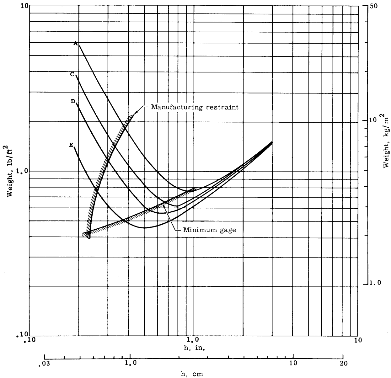
FIGURE 85. SUBSTRATE PANEL DESIGN OPTIMIZATION CURVES [PHENOLIC/GLASS SUBSTRATE WITH 1.50-IN. (3.81 CM) NASA 602 ABLATOR, 70° F (294.4° K) CONDITION]
