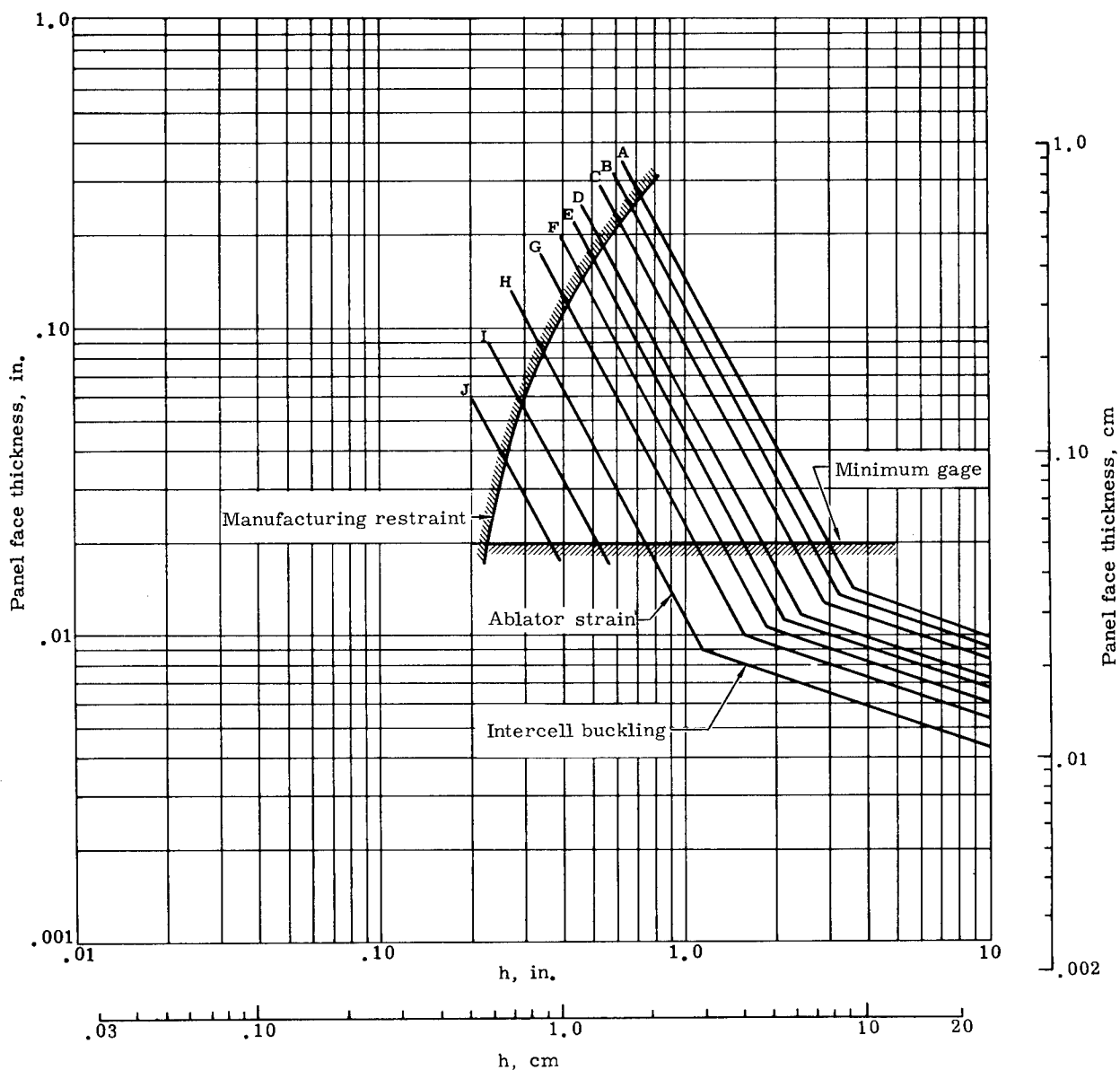
FIGURE 69. SUBSTRATE PANEL DESIGN CONSTRAINTS [PHENOLIC/GLASS SUBSTRATE PANEL WITH 1.50-IN. (3.81 CM) LDNP ABLATOR, 70° F (294.4° K) CONDITION]
