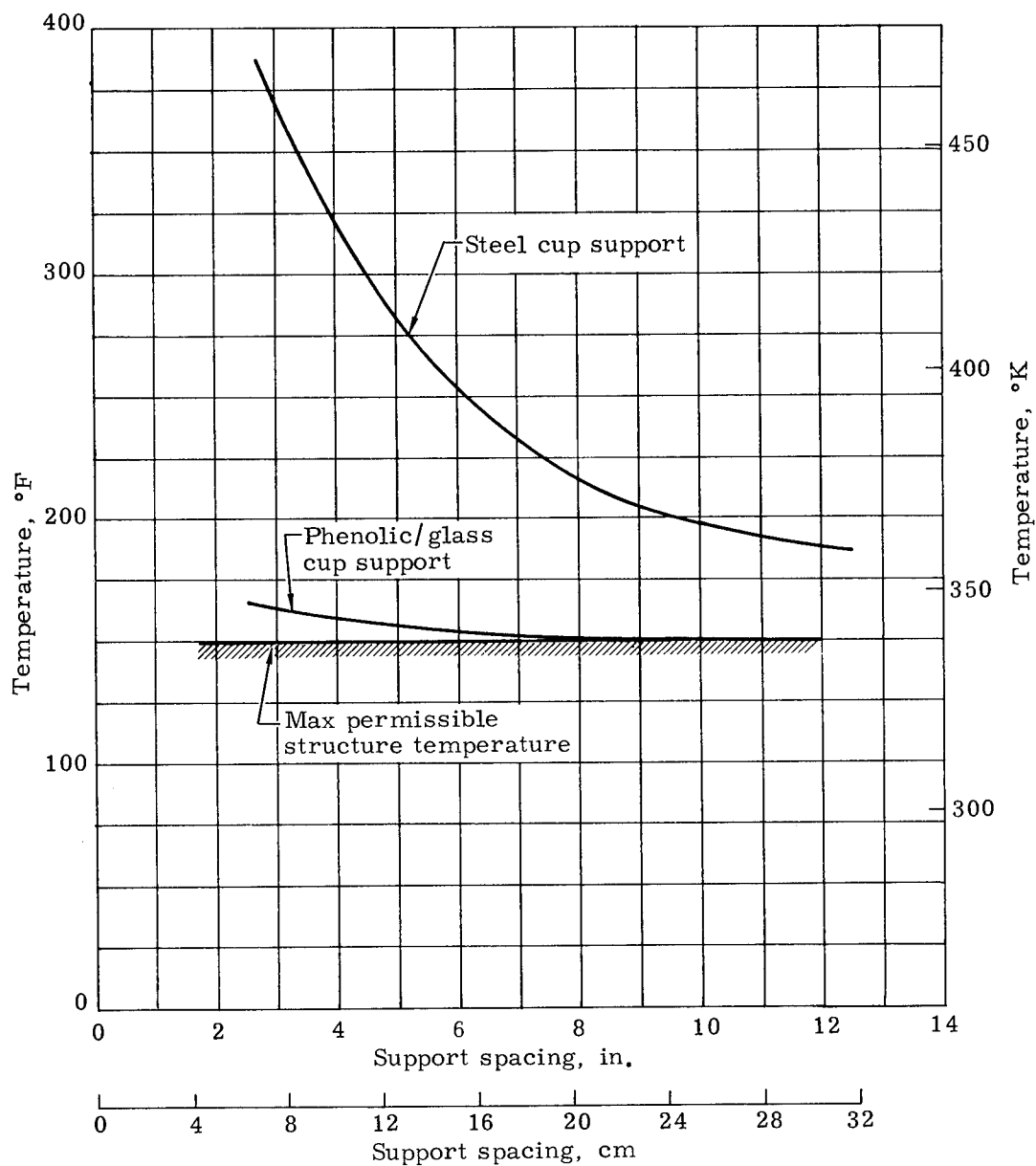
FIGURE 67. EFFECT OF SUPPORT SPACING ON HEAT SHORT EFFECT (ALUMINUM SKIN ONLY, NO HARD POINT)
