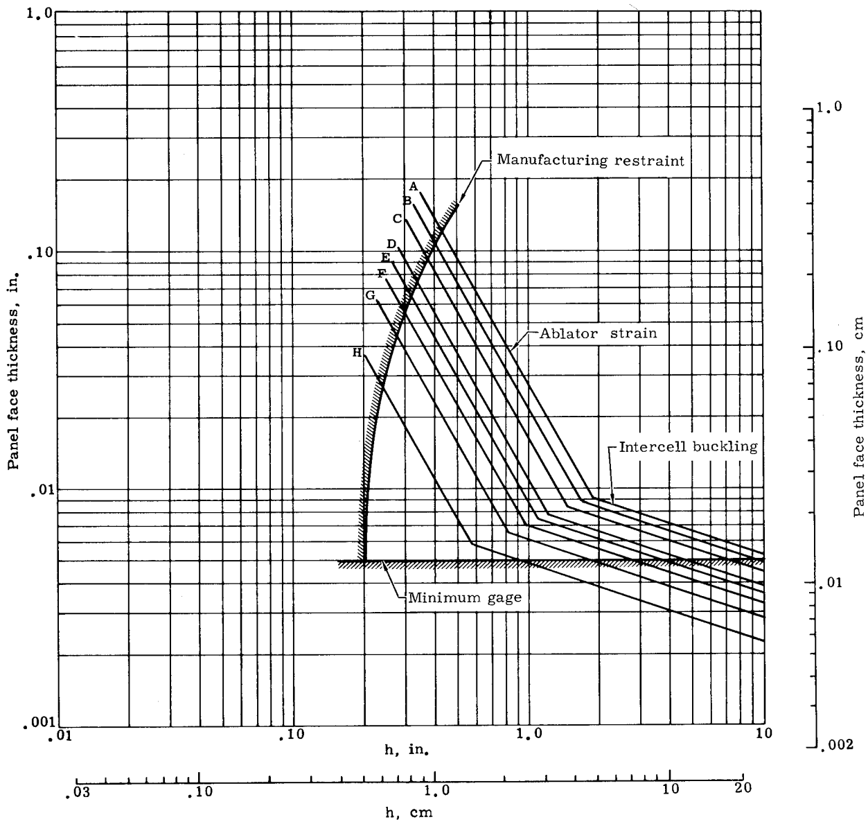
FIGURE 73. SUBSTRATE PANEL DESIGN CONSTRAINTS [17-7PH STEEL SUBSTRATE PANEL WITH 1.50-IN. (3.81 CM) LDNP ABLATOR, 70° F (294.4° K) CONDITION]
