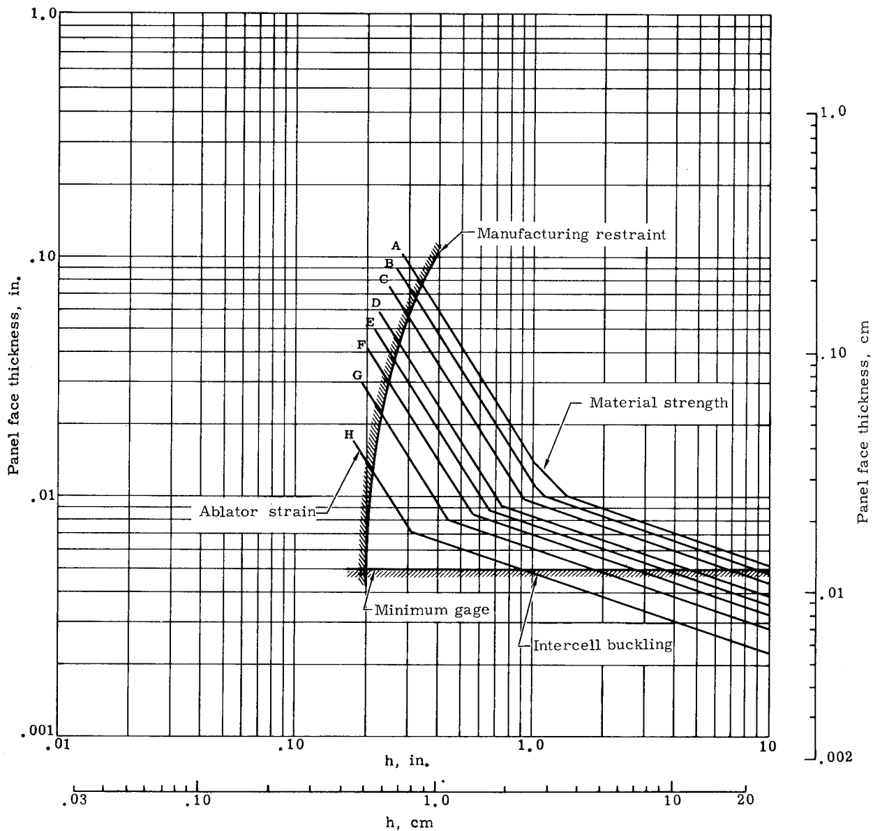
FIGURE 72. SUBSTRATE PANEL DESIGN CONSTRAINTS [17-7PH STEEL SUBSTRATE PANEL WITH 0.50-IN. (1.27 CM) LDNP ABLATOR, 70° F (294.4° K) CONDITION]
