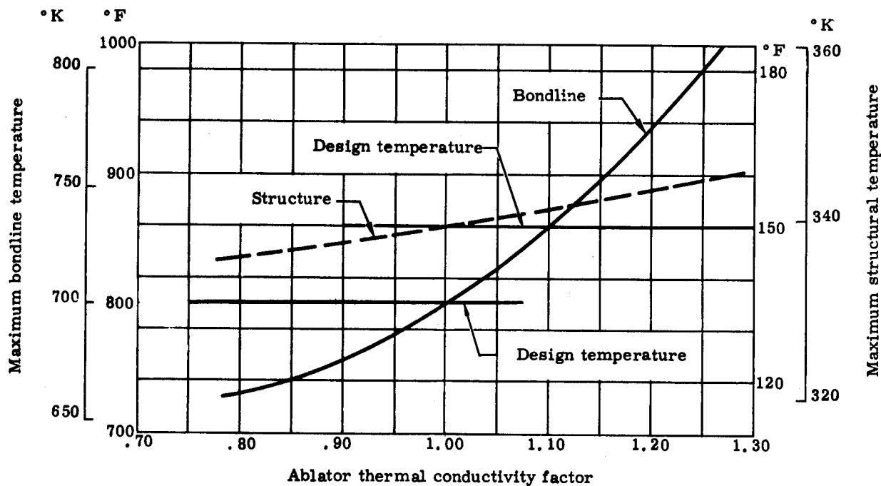
FIGURE 123a. EFFECT OF VARIATION IN ABLATOR THERMAL CONDUCTIVITY ON HEAT SHIELD TEMPERATURES (LDNP ABLATOR, OVERSHOOT RE-ENTRY, LEADING EDGE PANEL, \dot{q}_L/\dot{q}_{stag} = 0.70 )
