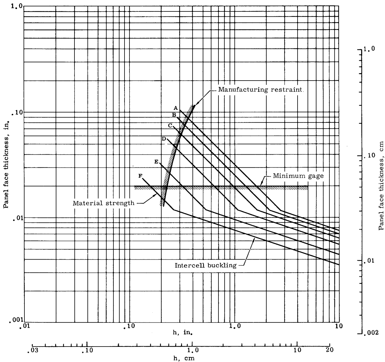
FIGURE 77. SUBSTRATE PANEL DESIGN CONSTRAINTS [PHENYL-SILANE/GLASS SUBSTRATE PANEL, 300° F (422.2° K) CONDITION]
