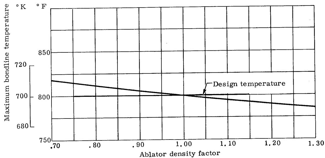
FIGURE 126a. EFFECT OF VARIATION IN ABLATOR DENSITY ON HEAT SHIELD TEMPERATURES (NASA 602 ABLATOR, OVERSHOOT RE-ENTRY, LEADING EDGE PANEL, q_L/q_{stag} = 0.70 )
