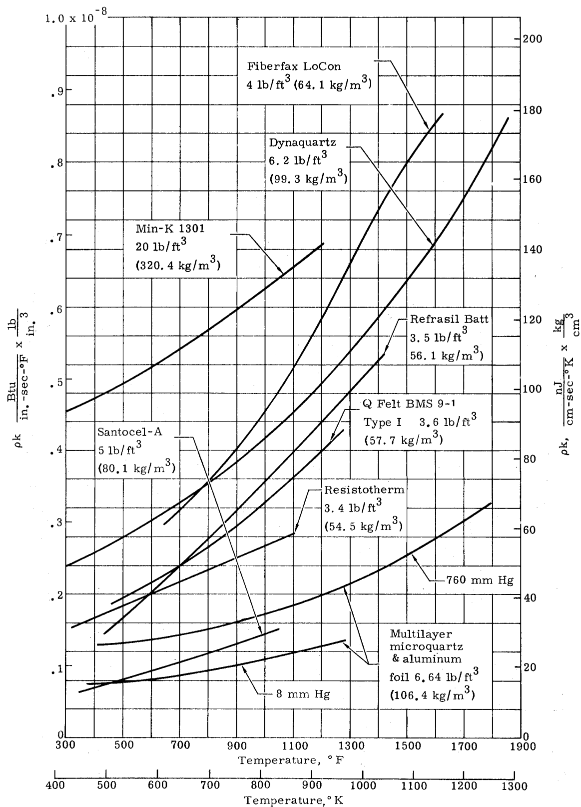
FIGURE 9. CANDIDATE INSULATION MATERIALS ( \rho k VERSUS TEMPERATURE) (Refs. 4 and 21)
