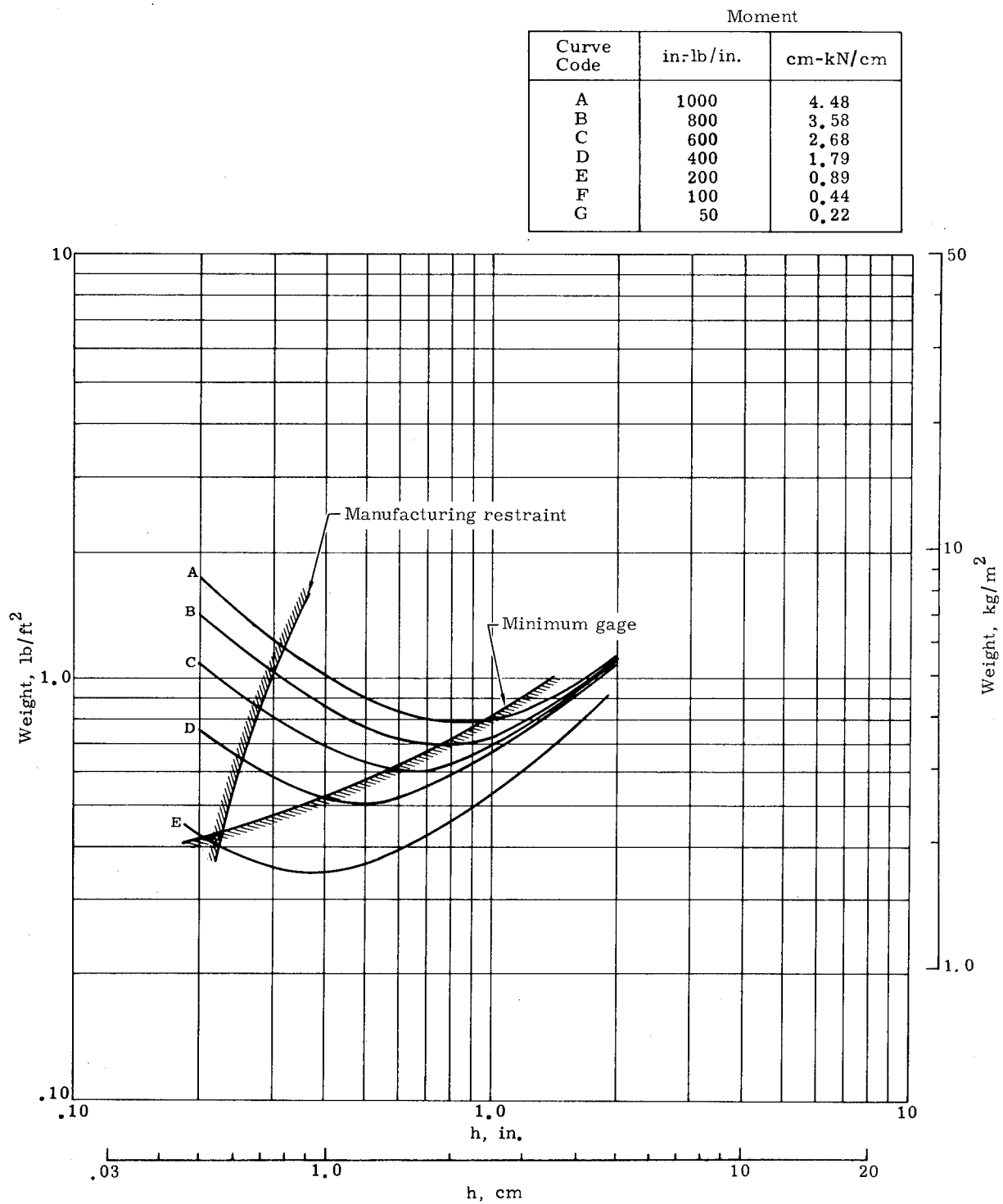
FIGURE 90. SUBSTRATE PANEL DESIGN OPTIMIZATION CURVES [PHENOLIC/GLASS SUBSTRATE PANEL, 300° F (422.2° K) CONDITION]
