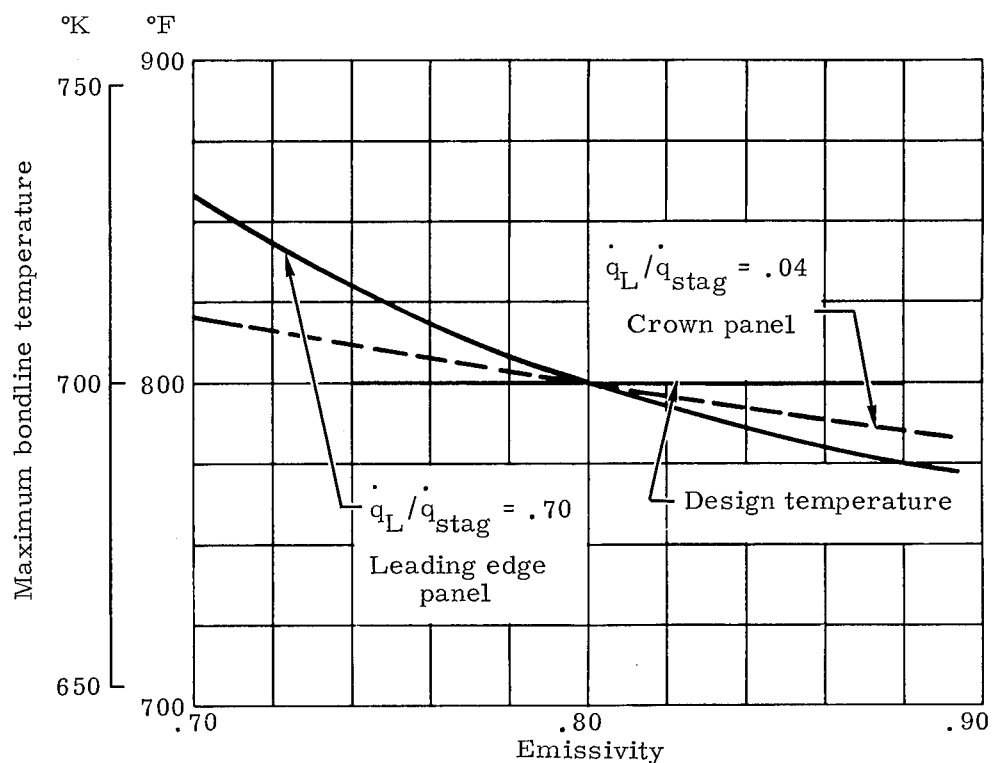
FIGURE 128a. EFFECT OF VARIATION OF CHAR EMISSIVITY ON HEAT SHIELD TEMPERATURES (LDNP ABLATOR, OVERSHOOT RE-ENTRY)
