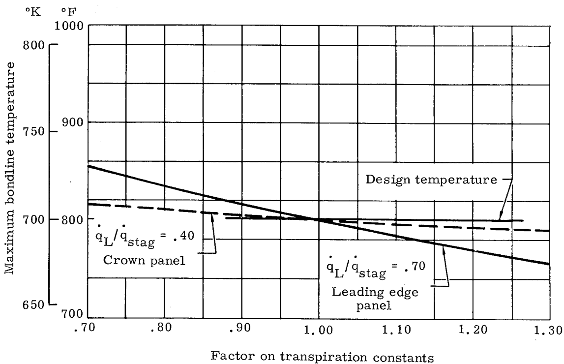
FIGURE 129b. EFFECT OF VARIATION OF TRANSPARATION FACTOR ON HEAT SHIELD TEMPERATURES (NASA 602 ABLATOR, OVERSHOOT RE-ENTRY)
