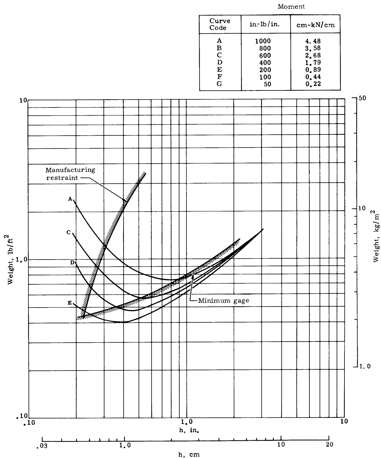
FIGURE 84. SUBSTRATE PANEL DESIGN OPTIMIZATION CURVES [PHENOLIC/GLASS SUBSTRATE WITH 0.50-IN. (1.27 CM) NASA 602 ABLATOR, 70° F (294.4° K) CONDITION]
