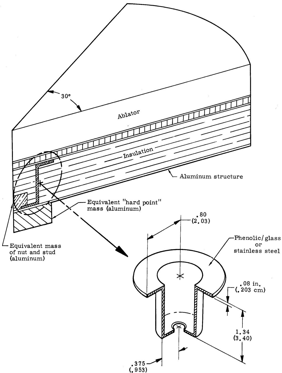
FIGURE 65. HEAT SHORT PROBLEM ANALYTICAL MODEL
