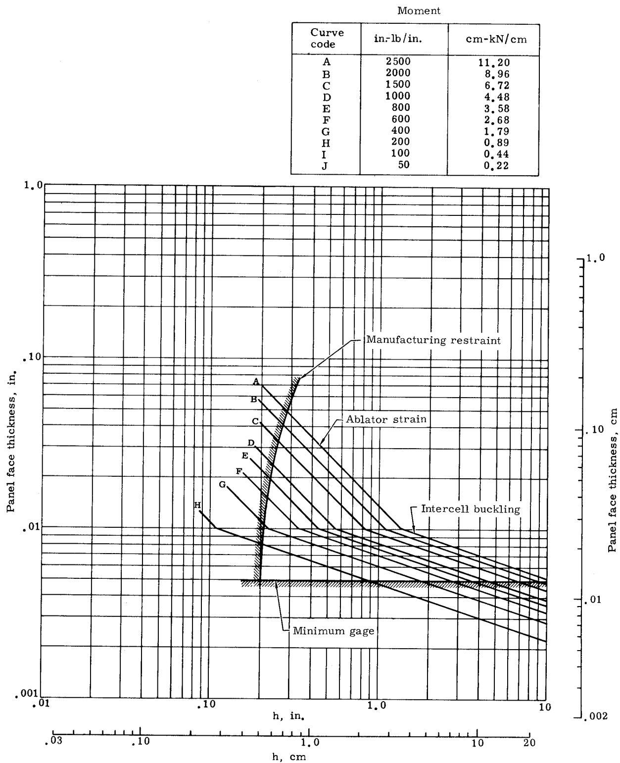
FIGURE 74. SUBSTRATE PANEL DESIGN CONSTRAINTS [17-7PH STEEL SUBSTRATE PANEL WITH 0.50-IN. (1.27 CM) NASA 602 ABLATOR, 70° F (294.4° K) CONDITION]
