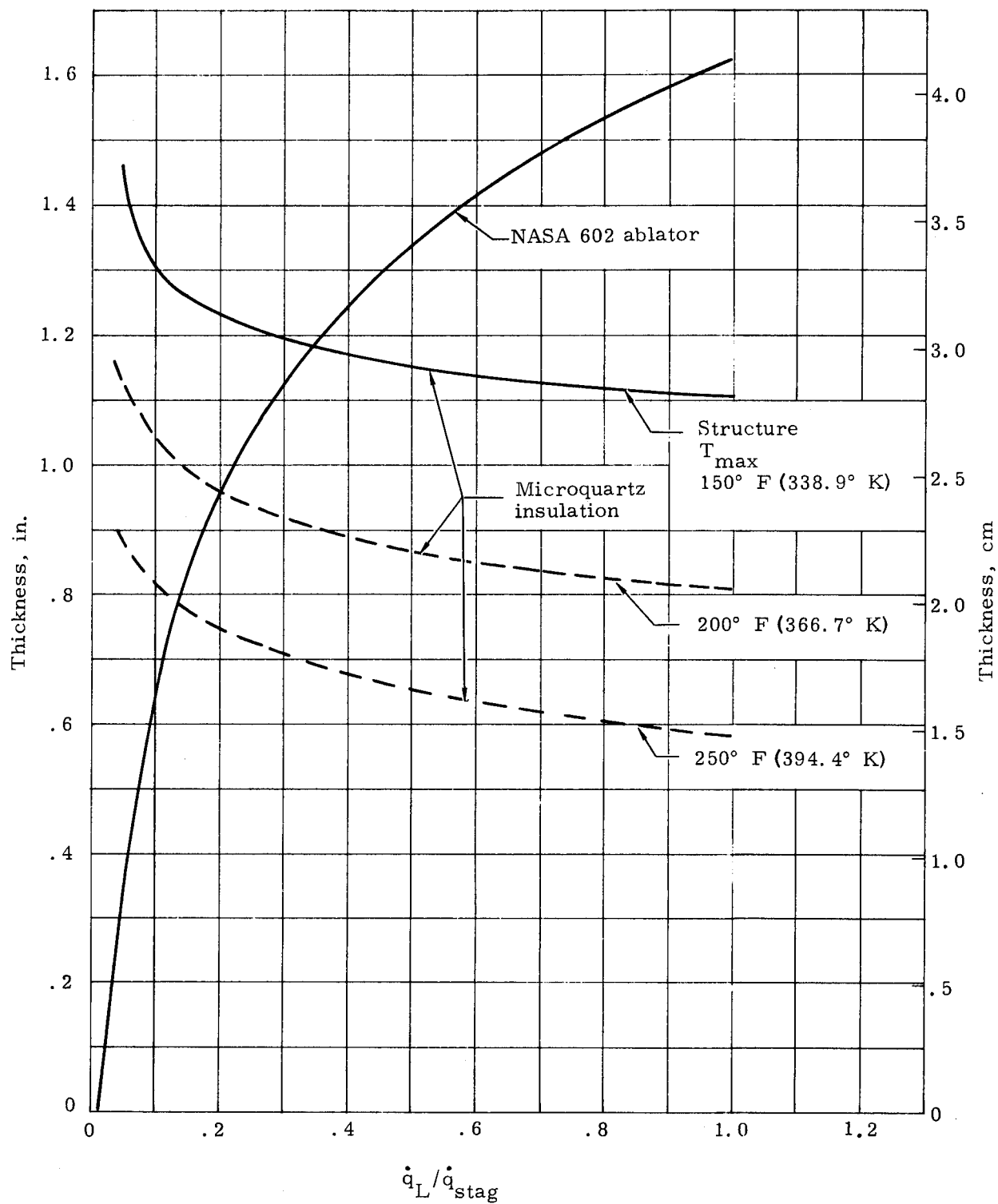
FIGURE 50. HEAT SHIELD DESIGN CURVE (NOMINAL TRAJECTORY, NASA 602 ABLATOR)
