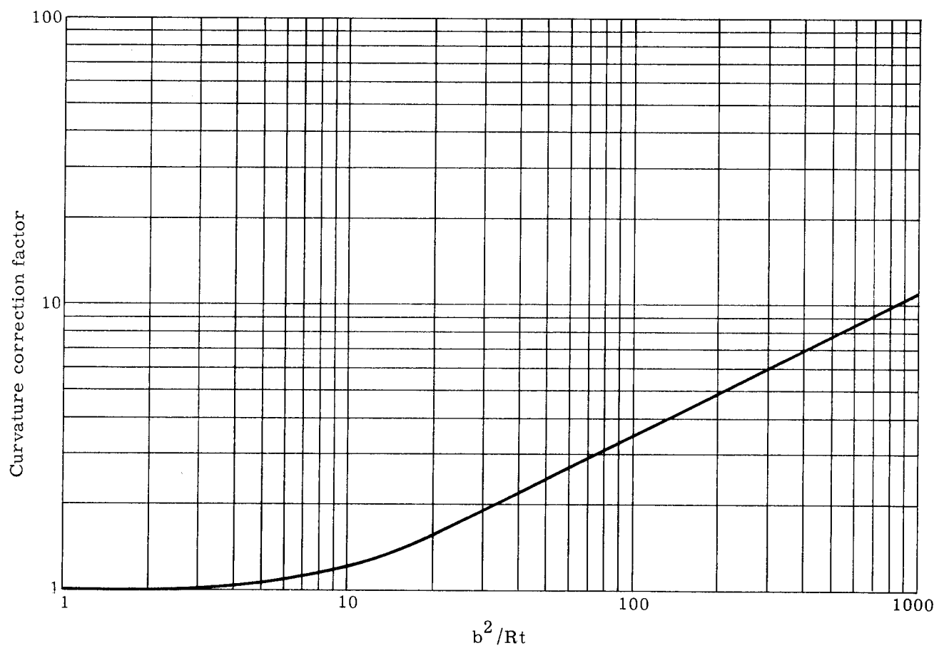
FIGURE 108. CURVATURE CORRECTION FACTOR
