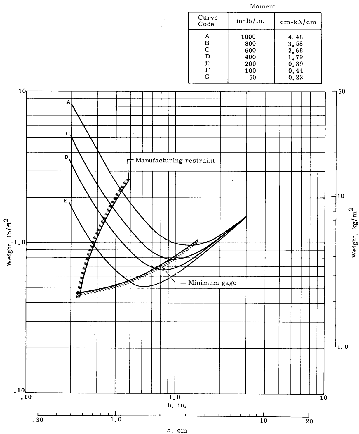
FIGURE 82. SUBSTRATE PANEL DESIGN OPTIMIZATION CURVES [PHENOLIC/GLASS SUBSTRATE WITH 0.50-IN. (1.27 CM) LDNP ABLATOR, 70° F (294.4° K) CONDITION]
