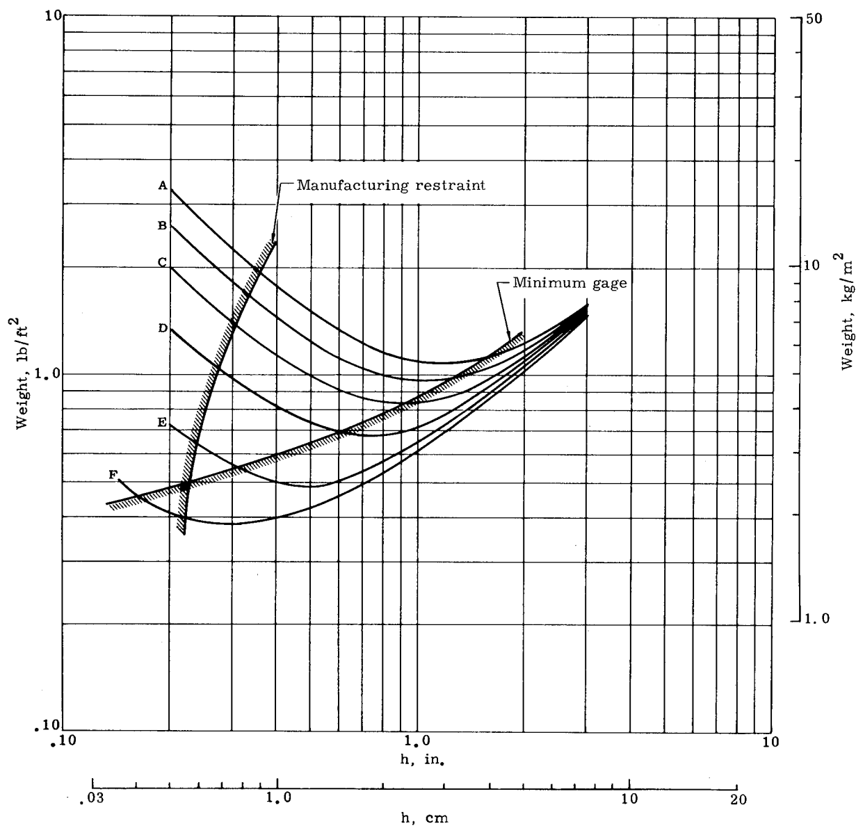
FIGURE 91. SUBSTRATE PANEL DESIGN OPTIMIZATION CURVES [PHENYL-SILANE/GLASS SUBSTRATE PANEL, 300° F (422.2° K) CONDITION]
