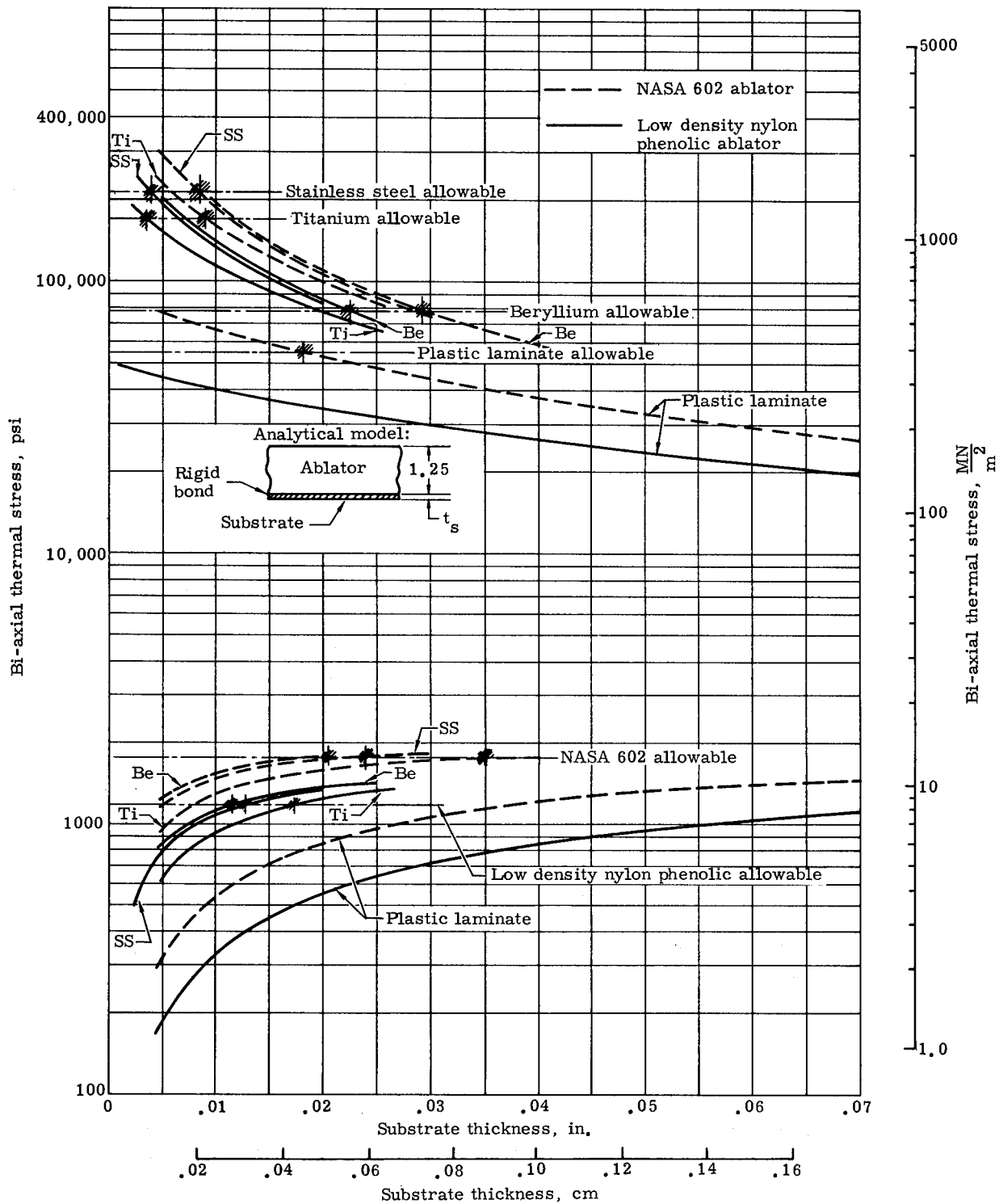
FIGURE 25. THERMAL STRESS COMPARISONS (UNIFORM COLD SOAK AT -110^{\circ} F OR 194.4^{\circ} K )
