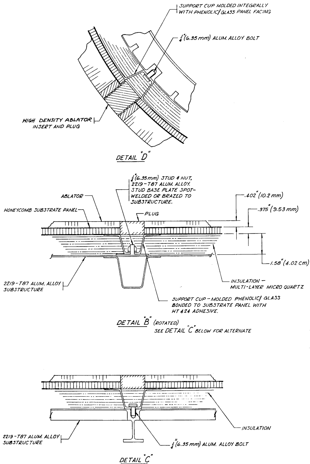
FIGURE 119. ALTERNATE DESIGNS FOR ATTACHMENT
