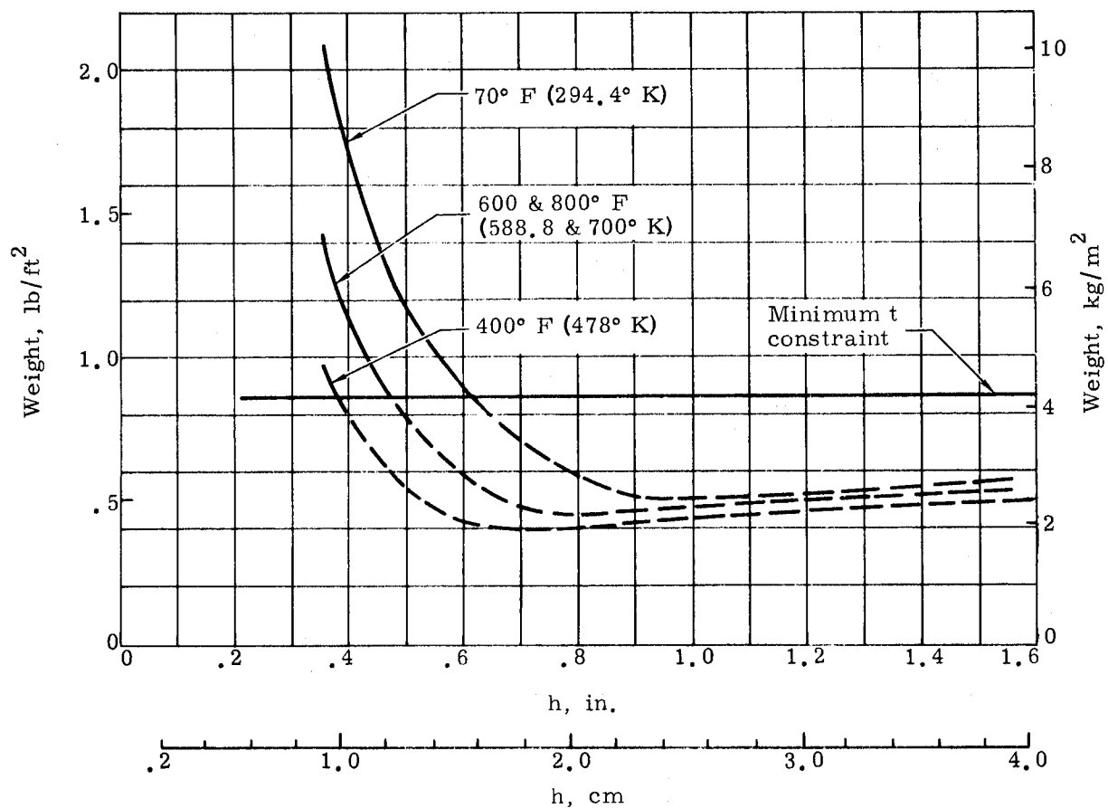
FIGURE 35. PHENOLIC/GLASS LAMINATE SINGLE SKIN CORRUGATION PANEL OPTIMUM WEIGHT CURVES
