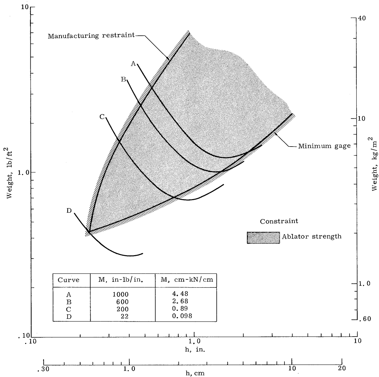
FIGURE 98. DESIGN CONSTRAINT RELATIONSHIPS [PHENOLIC/GLASS SUBSTRATE WITH 1.50-IN. (3.81 CM) LDNP ABLATOR, 70° F (294.4° K) CONDITION]
