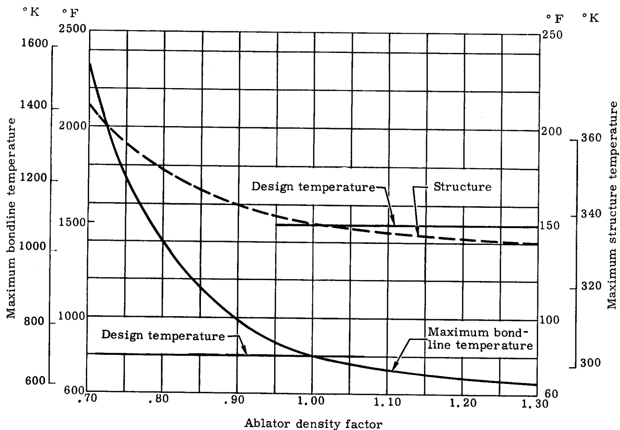
FIGURE 125a. EFFECT OF VARIATION IN ABLATOR DENSITY ON HEAT SHIELD TEMPERATURES (LDNP ABLATOR, OVERSHOOT RE-ENTRY, LEADING EDGE PANEL, q_L/q_{stag} = 0.70 )
