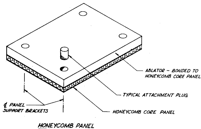
FIGURE 2. PRELIMINARY SUBSTRATE PANEL CONCEPTS
