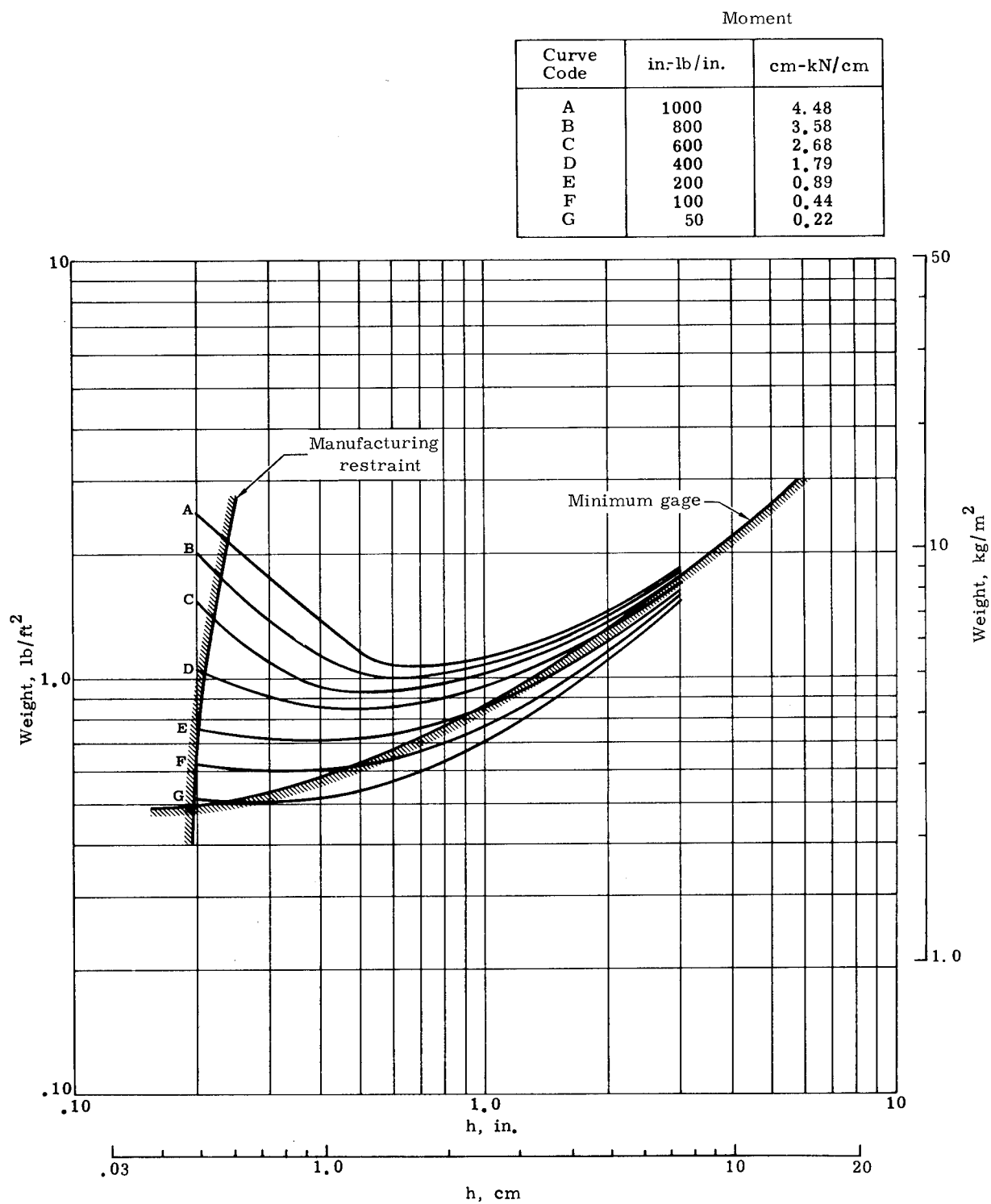
FIGURE 92. SUBSTRATE PANEL DESIGN OPTIMIZATION CURVES [17-7PH STEEL SUBSTRATE PANEL, 300° F (422.2° K) CONDITION]
