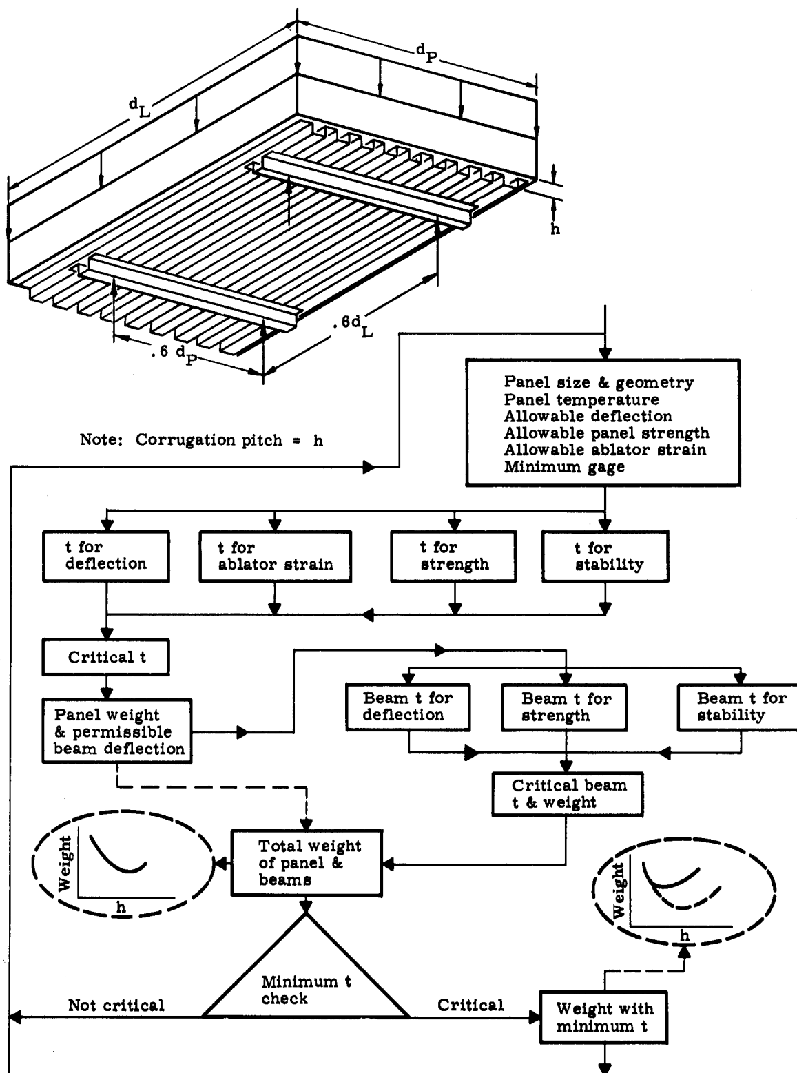
FIGURE 27. SINGLE SKIN CORRUGATION SUBSTRATE PANEL OPTIMIZATION PROGRAM
