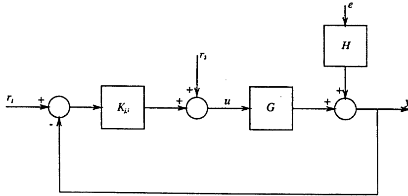
Figure 3. Closed-loop system
