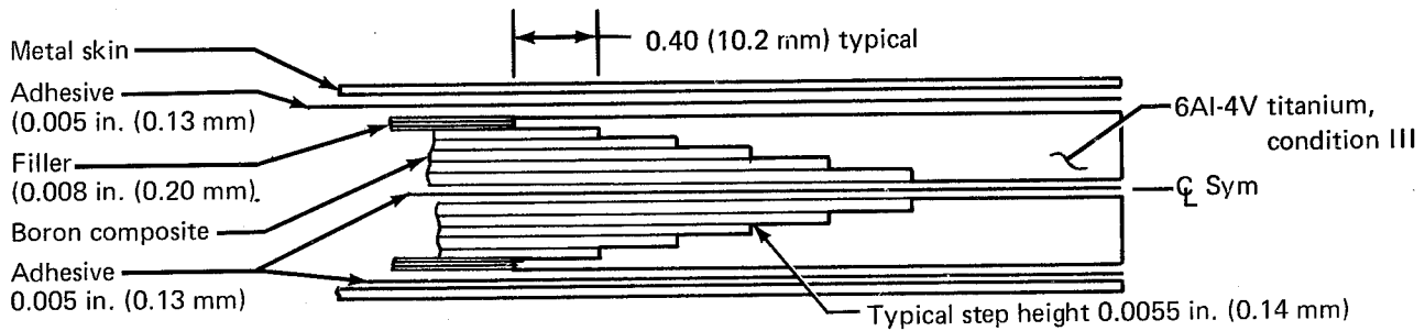
TYPICAL SECTION THROUGH TRANSITION REGION
