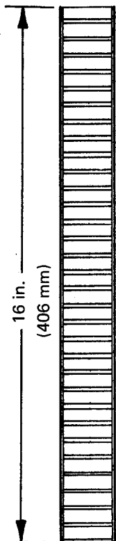
PANEL CROSS SECTION
