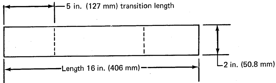
STEPPED-JOINT SPECIMEN PLAN VIEW
