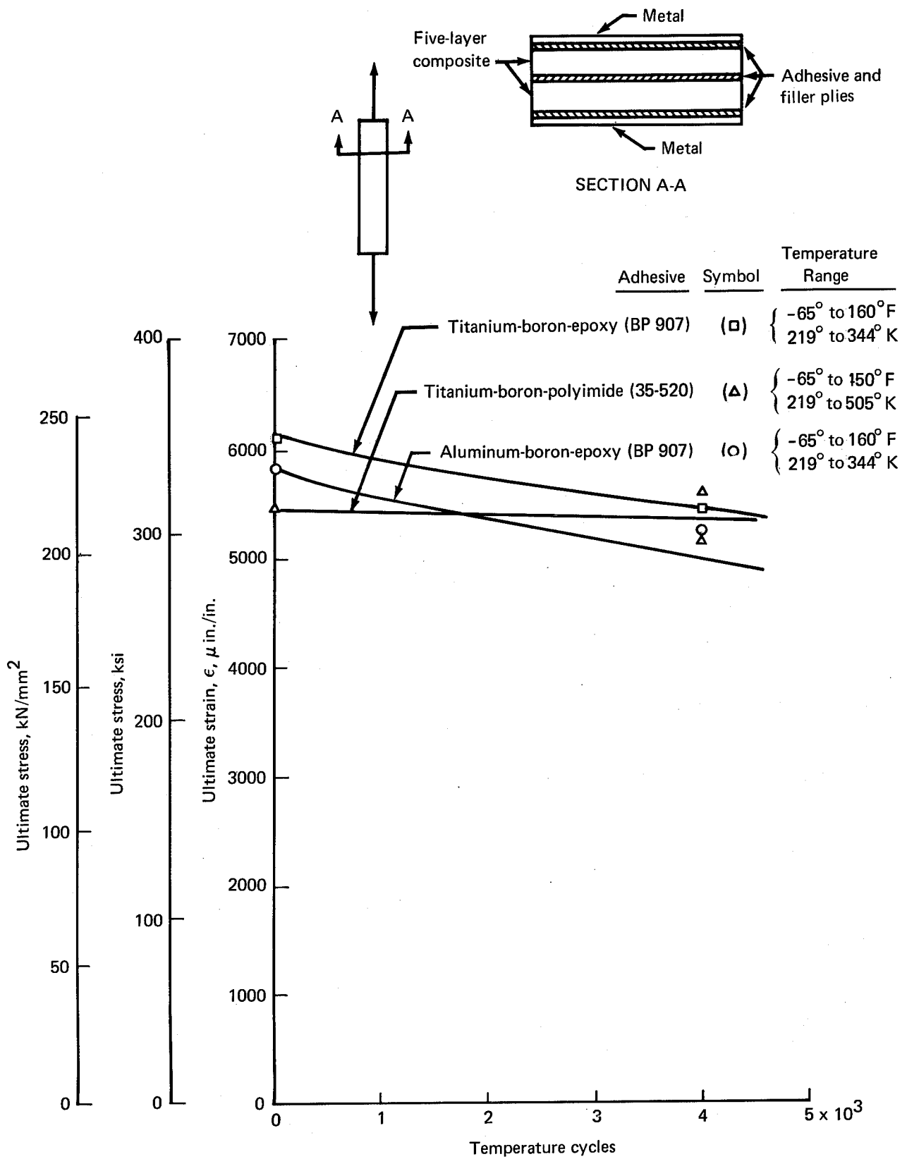
FIGURE 19.—STEPPED-JOINT ULTIMATE FIBER STRENGTH AS A FUNCTION OF TEMPERATURE CYCLES
