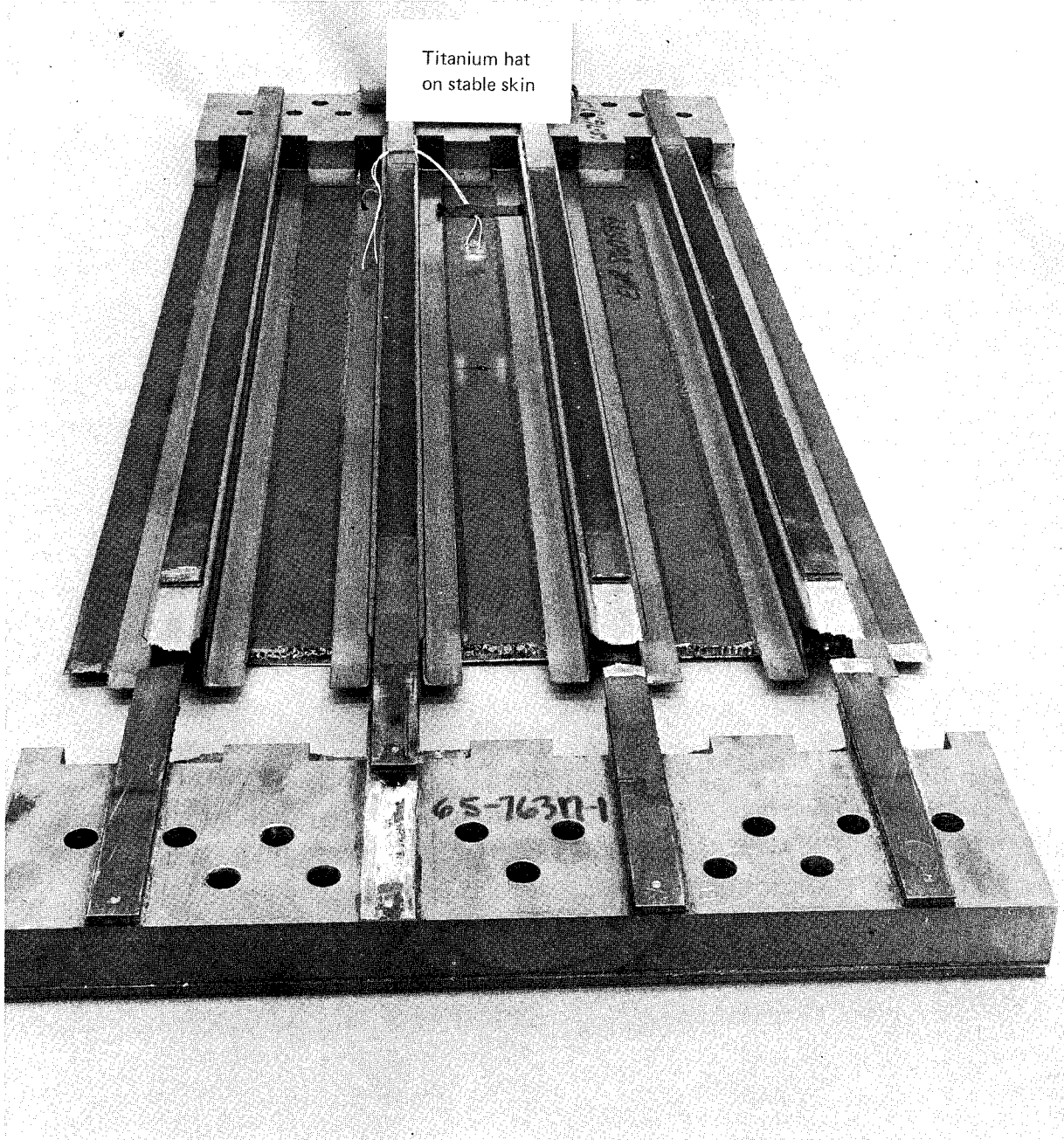
FIGURE 57.—FRACTURE IN CONCEPT 4b
