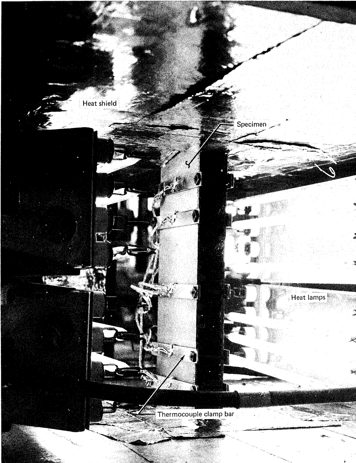
FIGURE 3.—FATIGUE TESTING AT 450° F (505° K)
