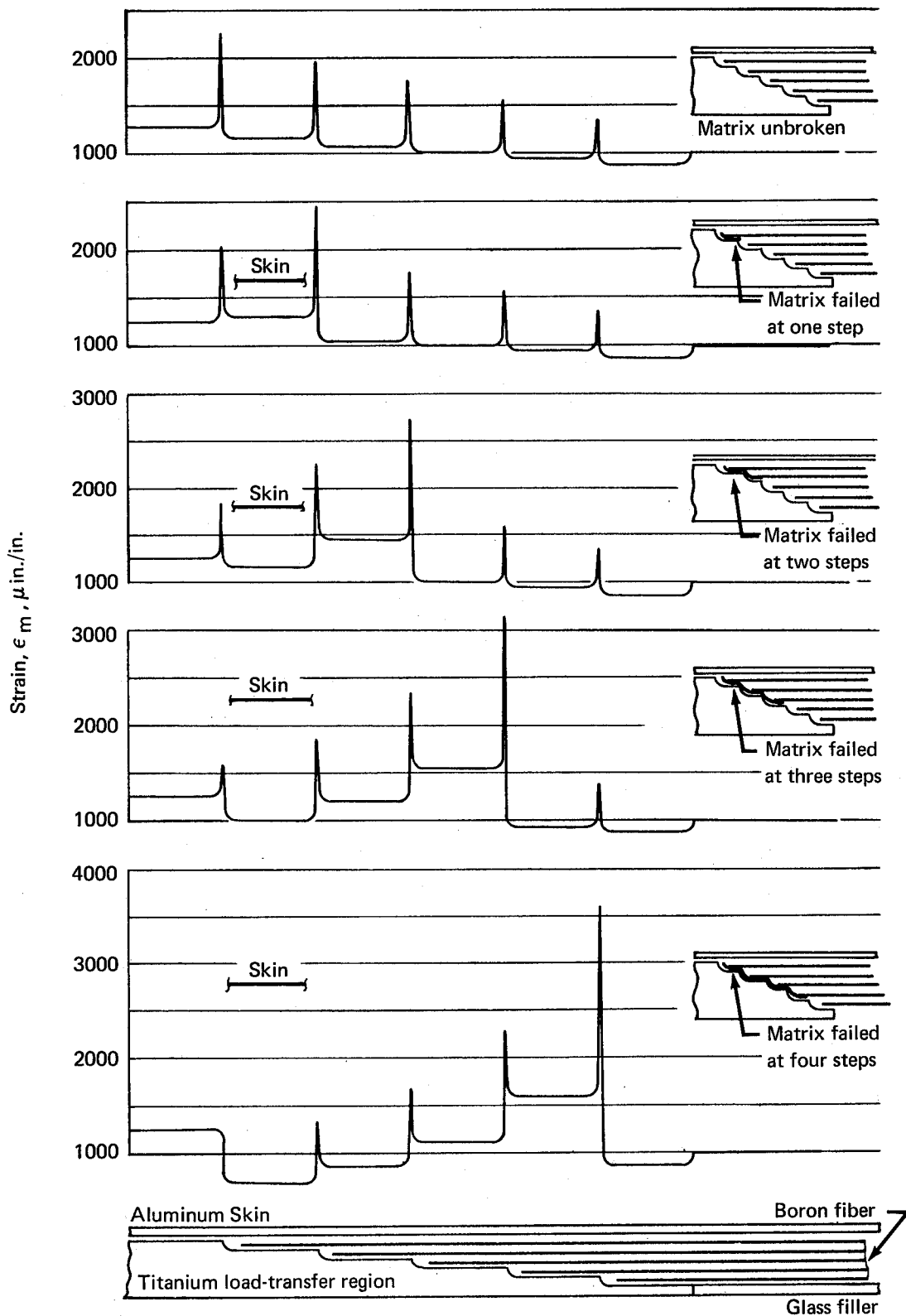
FIGURE 15.—STRAIN IN TITANIUM LOAD TRANSFER REGION FOR ALUMINUM-BORON-EPOXY FATIGUE SPECIMENS
