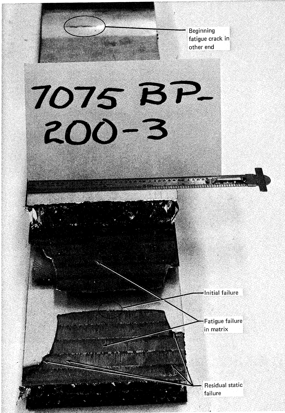
FIGURE 6.—ALUMINUM-BORON-EPOXY SPECIMEN CYCLED AT 16.7 HZ FOR 14 790 CYCLES
