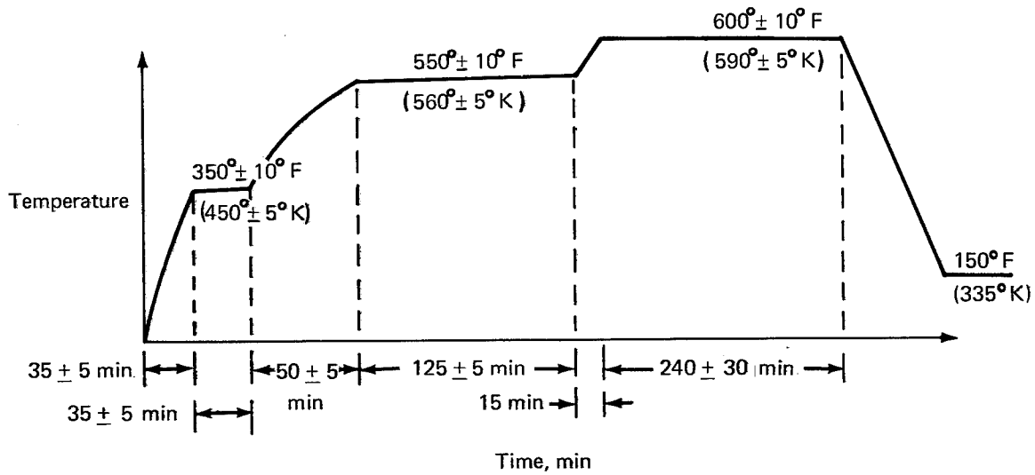
35-520 AND FM 34 POSTCURE CYCLE
