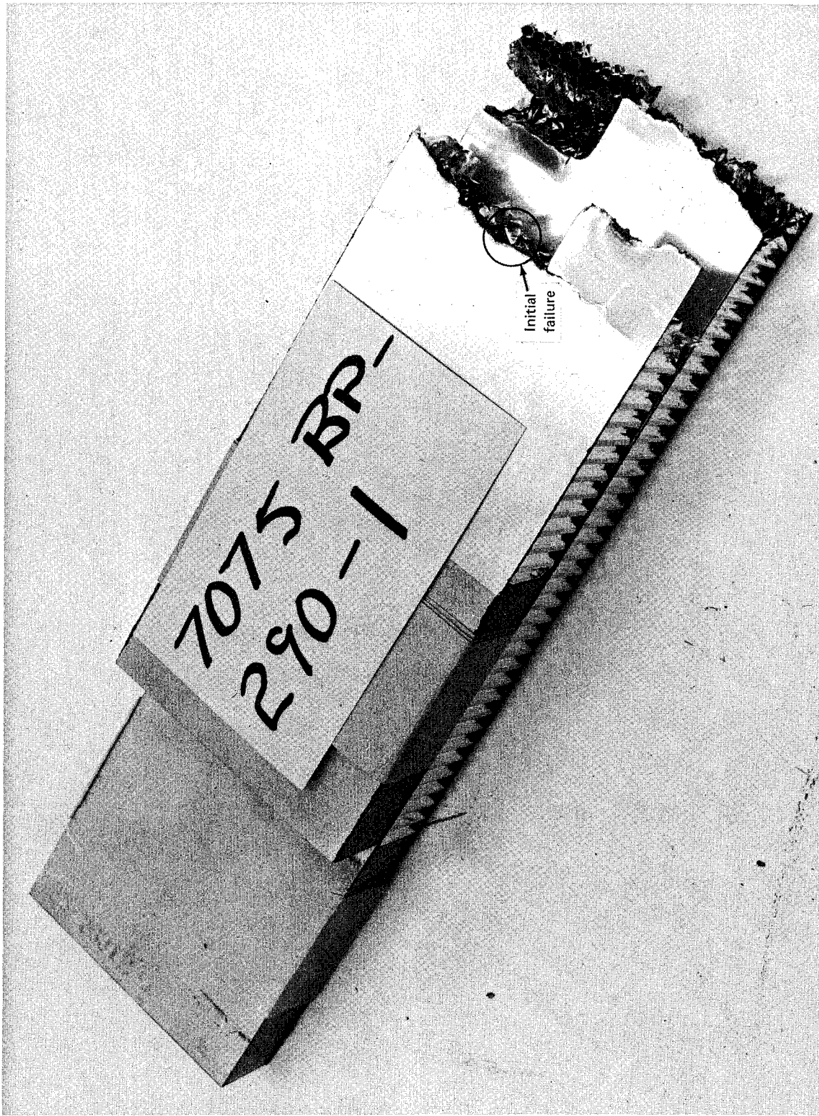
FIGURE 5.— ALUMINUM-BORON-EPOXY FATIGUE SPECIMEN CYCLED AT 0.12 HZ FOR 17 CYCLES
