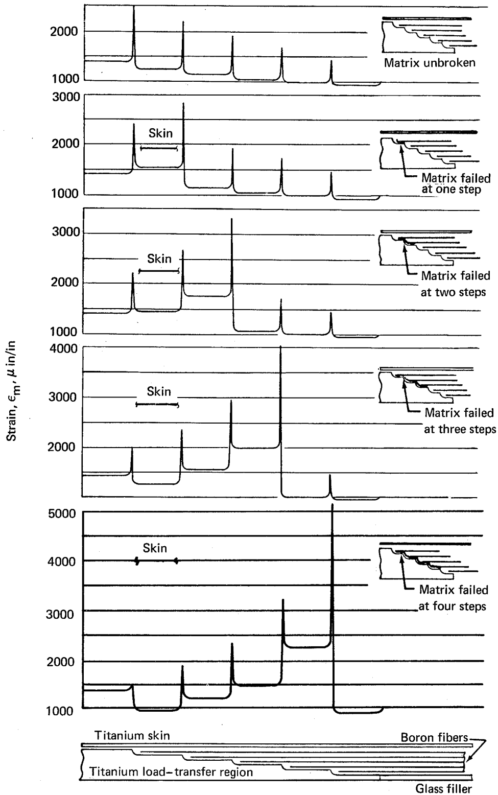
FIGURE 17.—STRAIN IN TITANIUM LOAD TRANSFER REGION FOR TITANIUM-BORON-POLYIMIDE FATIGUE SPECIMENS
