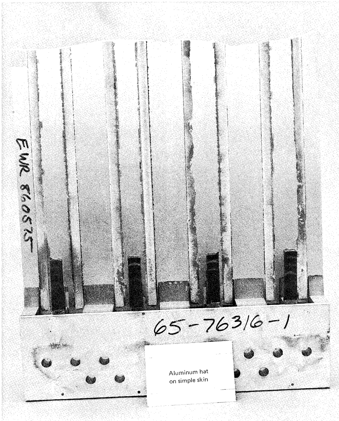
FIGURE 54.—ADHESIVE FAILURE SURFACES ON CONCEPT 3a AFTER COMPRESSION DEBONDING
