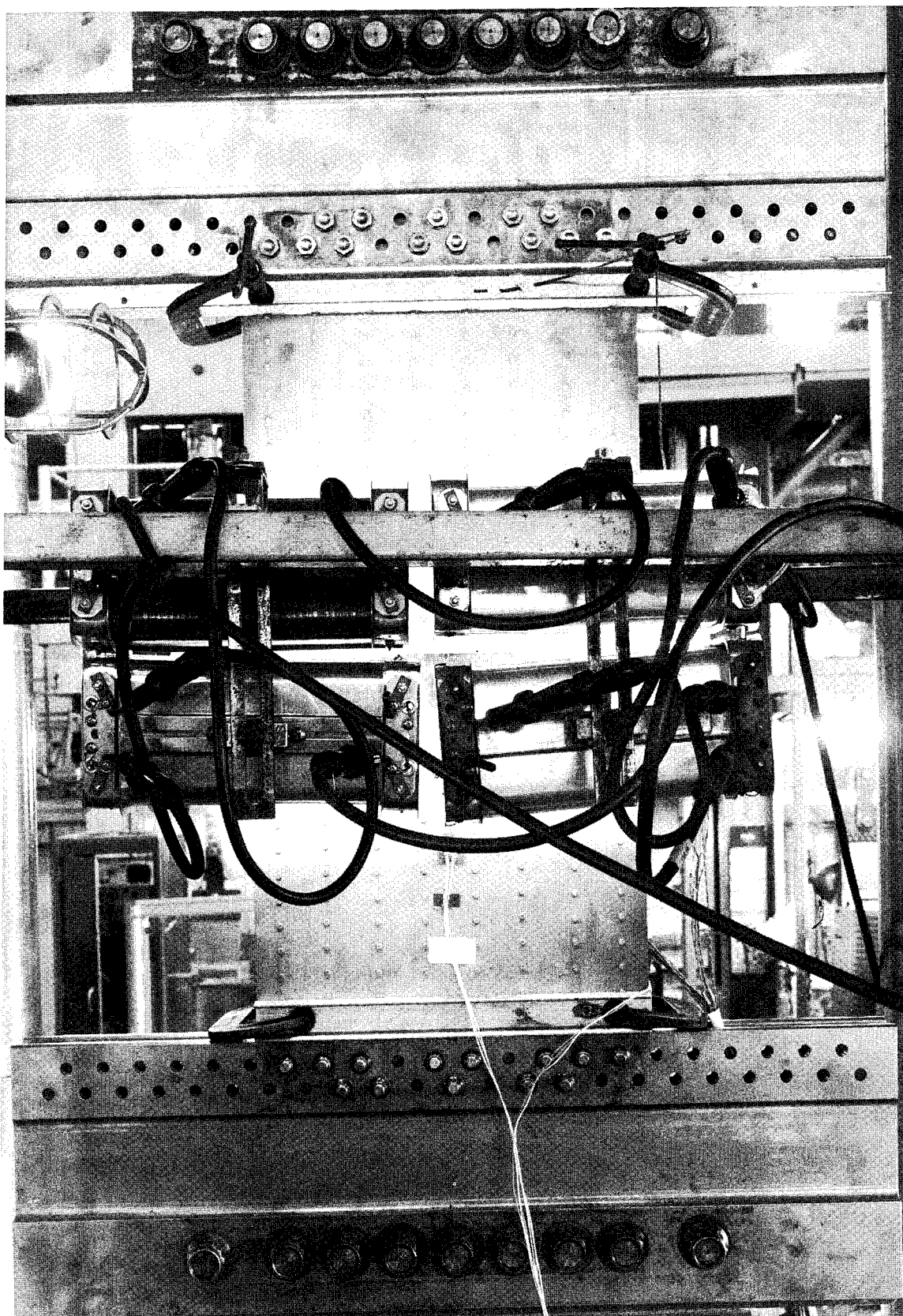
FIGURE 33.—ELEVATED-TEMPERATURE TEST IN 150-KIP ELECTROMECHANICAL RESEARCH MACHINE
