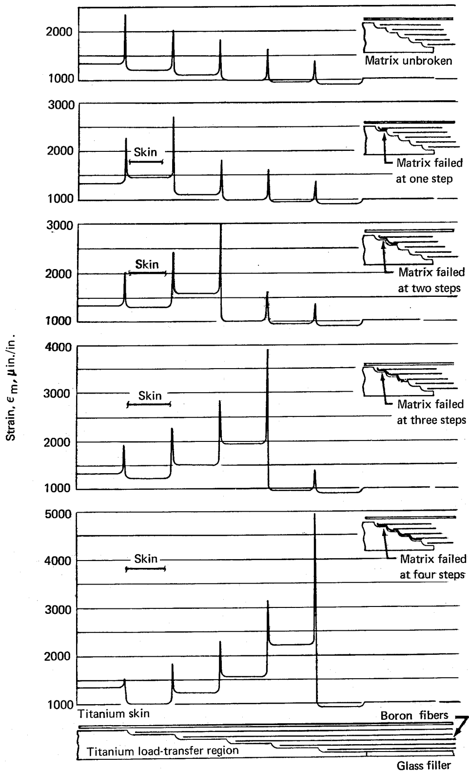
FIGURE 16.—STRAIN IN TITANIUM LOAD TRANSFER REGION FOR TITANIUM-BORON-EPOXY FATIGUE SPECIMENS
