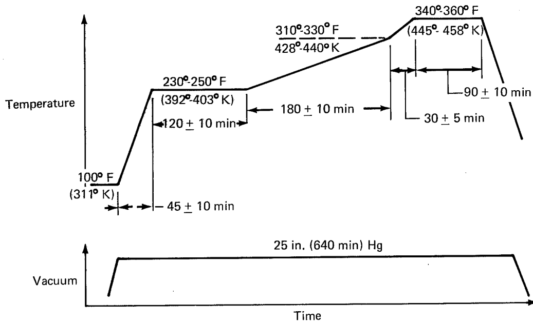
35-520 CURE CYCLE
