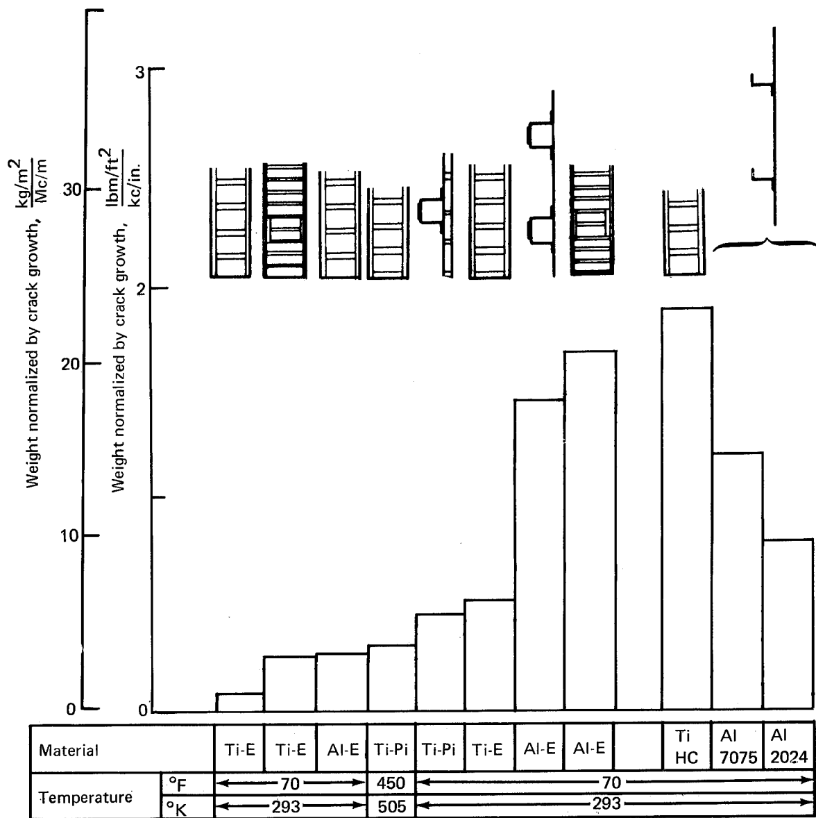
FIGURE 59.— WEIGHT COMPARISON BASED ON CRACK GROWTH RATE
