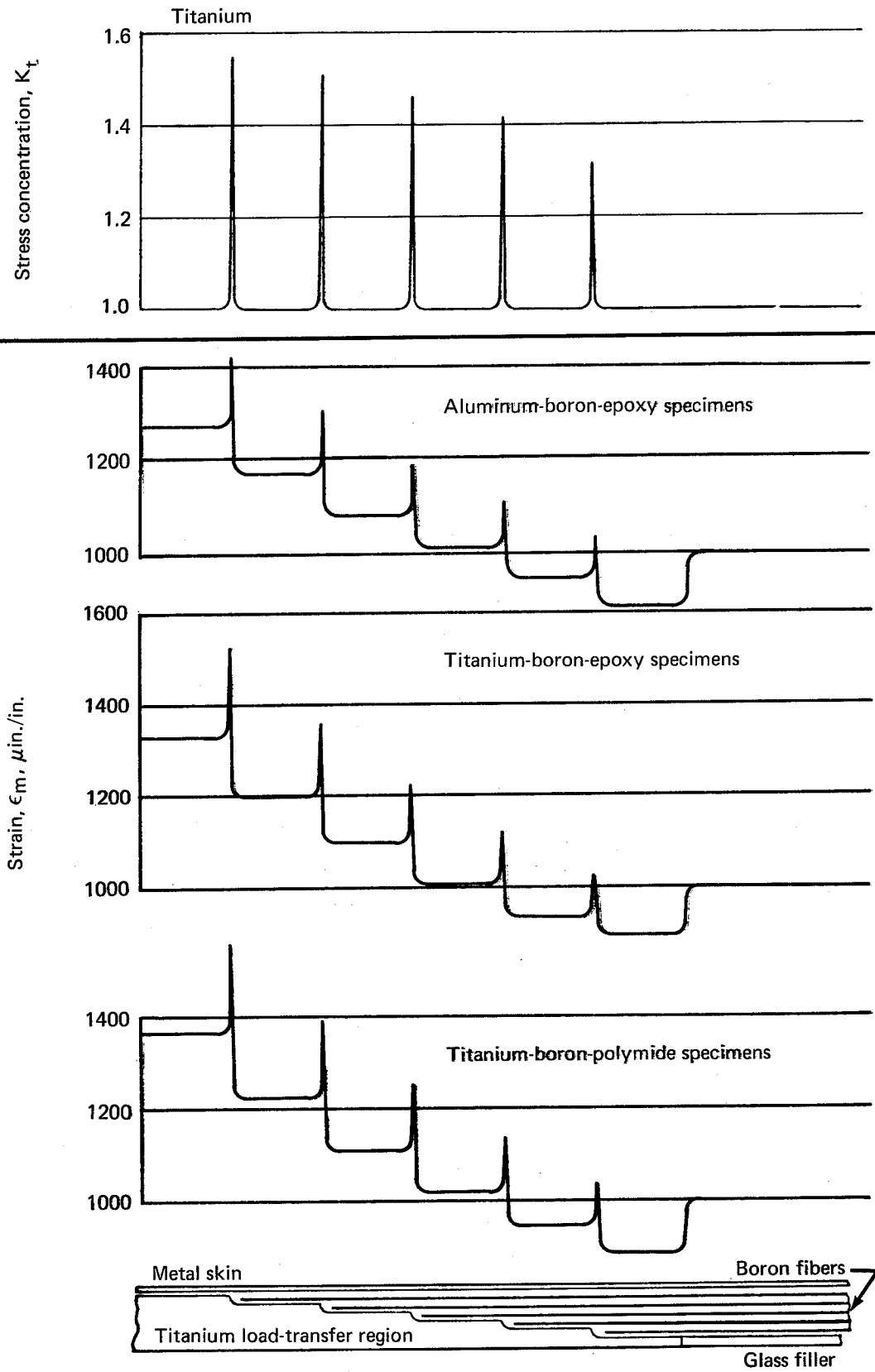
FIGURE 14.—STRAIN IN TITANIUM LOAD TRANSFER REGION FOR FATIGUE SPECIMENS
