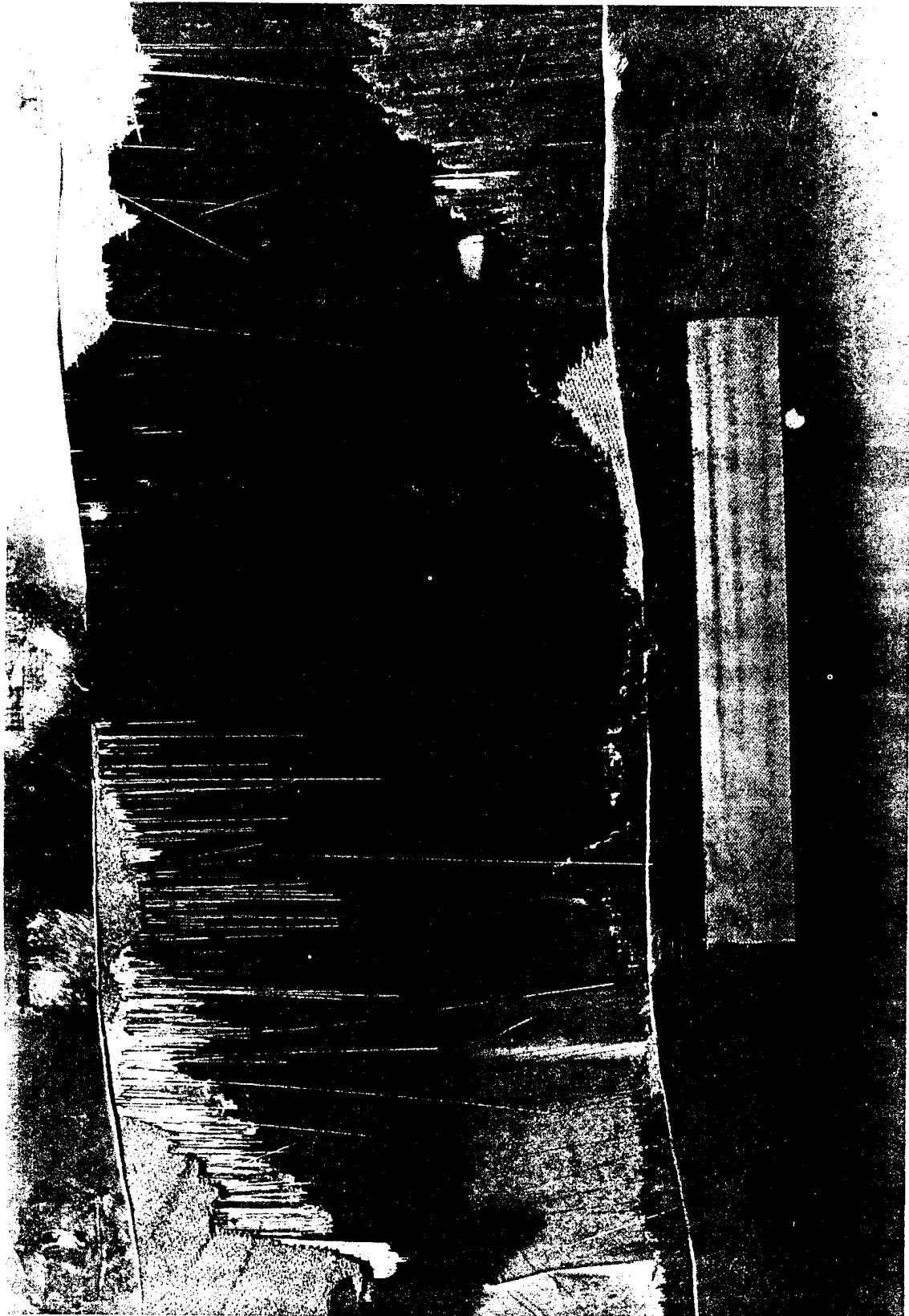
FIGURE 49.— FRACTURE IN CONCEPT 1c AFTER ELEVATED-TEMPERATURE TEST
