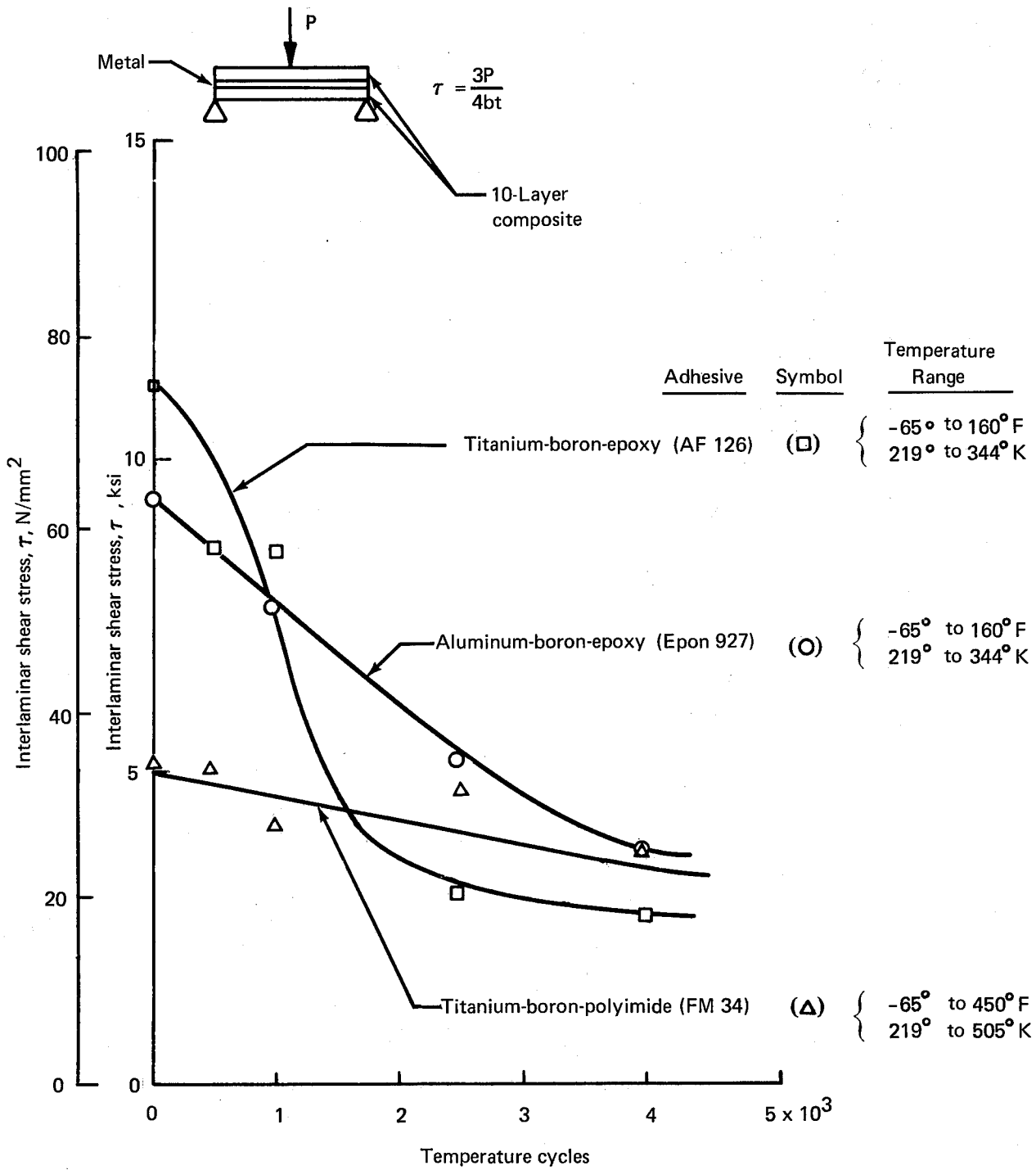
FIGURE 20.—INTERLAMINAR SHEAR STRENGTH AS A FUNCTION OF TEMPERATURE CYCLES
