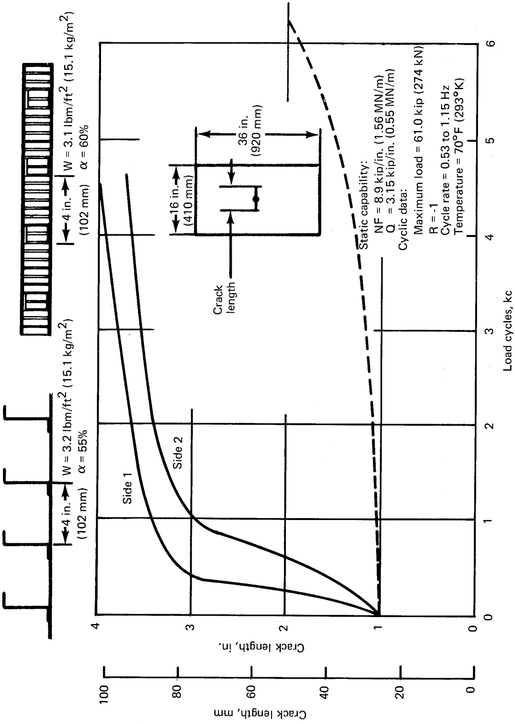
FIGURE 38.—CRACK GROWTH AND RESIDUAL STRENGTH COMPARISON OF FIBER-REINFORCED (BORON EPOXY) 7075-T6 AND CONVENTIONAL 7075-T6 ZEE STRINGER CONSTRUCTION
