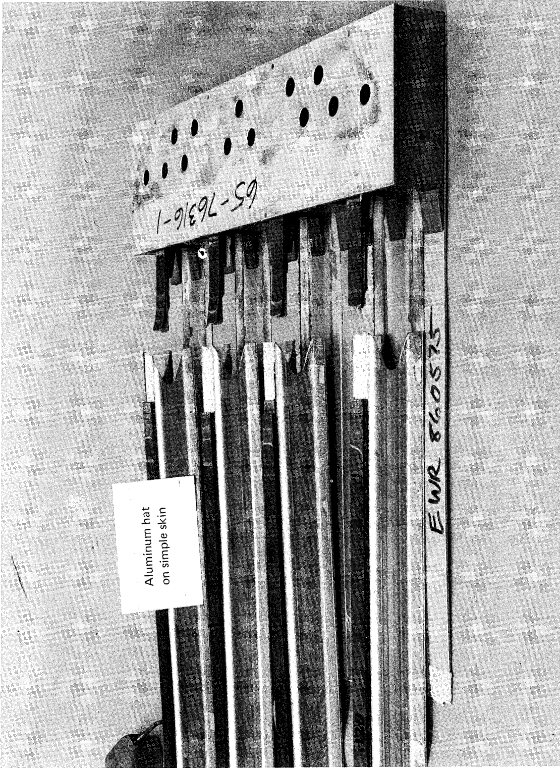
FIGURE 53.—FRACTURE IN CONCEPT 3a
