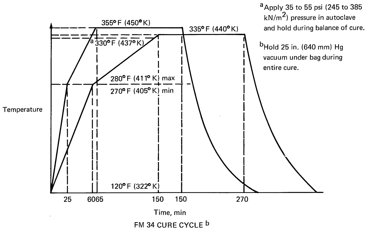
FIGURE 62.—CURE CYCLES FOR EPON 927 AND 933 EPOXY AND FM 34 POLYIMIDE ADHESIVES
