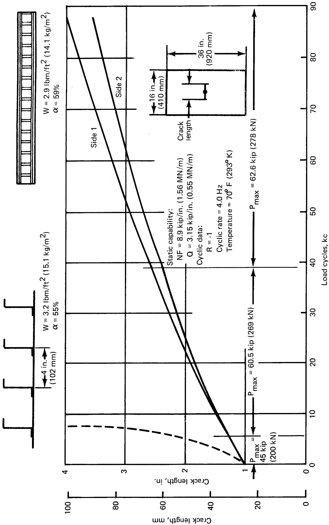
FIGURE 35.—CRACK GROWTH AND RESIDUAL STRENGTH COMPARISON OF FIBER-REINFORCED 6AL-4V TITANIUM AND CONVENTIONAL 7075-T6 ZEE STRINGER CONSTRUCTION
