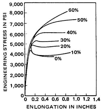
Figure 60. Stress-elongation curves for unidirectionally rolled ABS polymer (Cyclocac MS) tested in the rolling direction (21)
