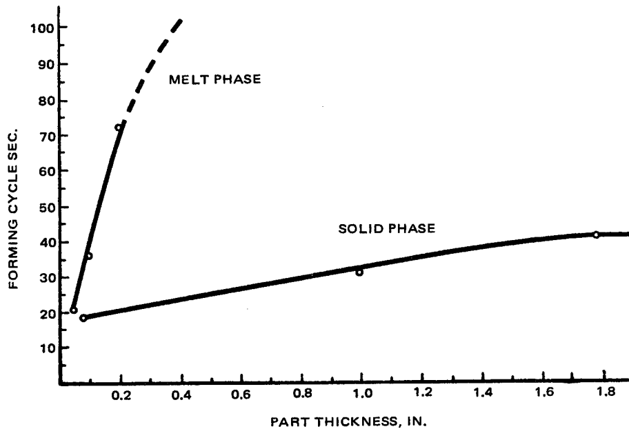
Figure 73. Effect of part thickness on forming speeds (2)
