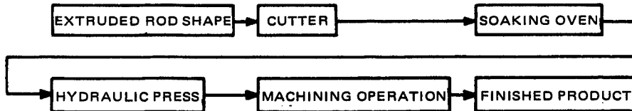
Figure 74. Forging operation (4)
