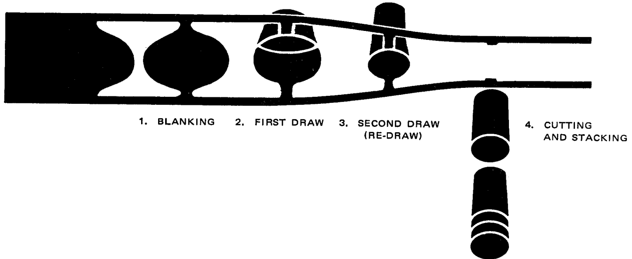
Figure 25. Web carrier (9)
