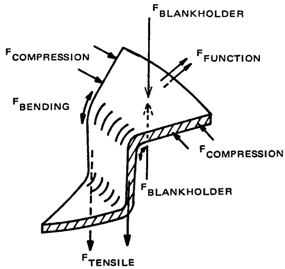
Figure 43. Forces in deep drawing (17)
