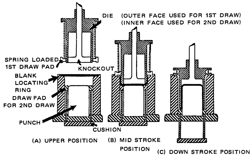
Figure 23. Combination tool for successive 1st draw and 2nd inverted draw in one operation (6)
