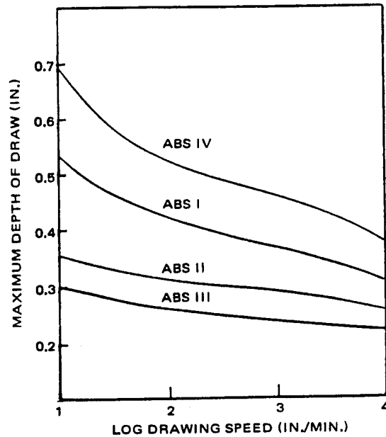
Figure 41. Maximum depth of draw of extruded ABS polymers (16)
