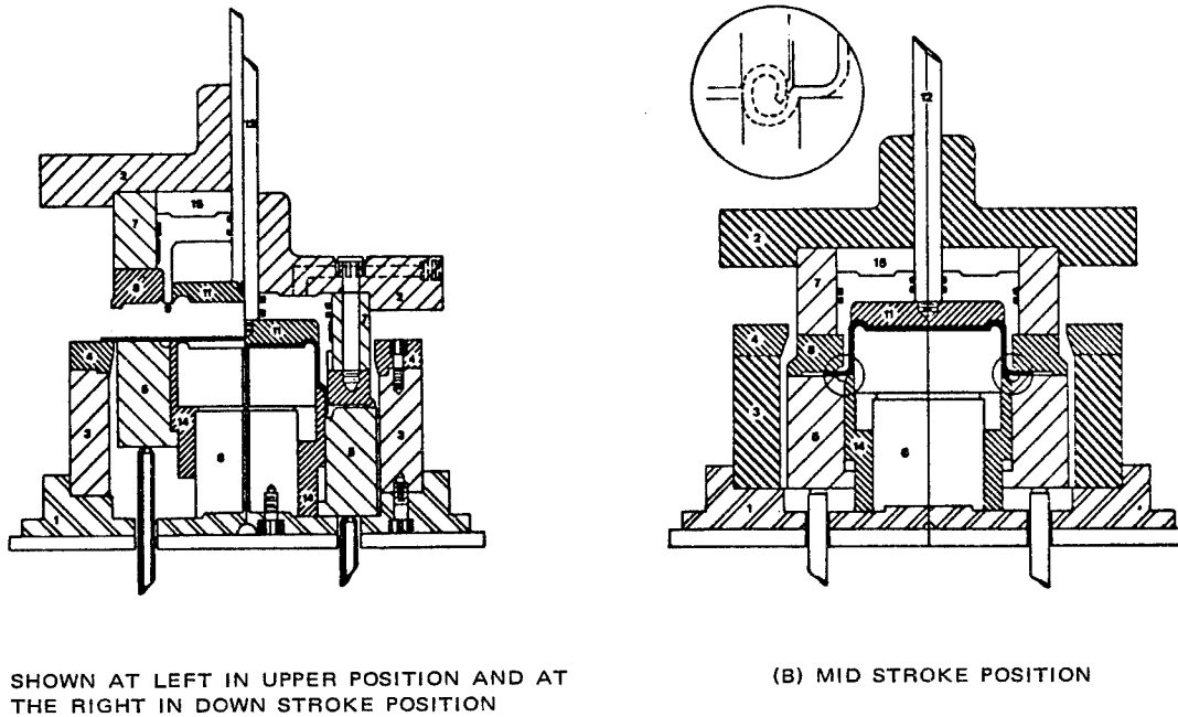
Figure 24. Tool for combination blanking, drawing, wiping, coining and curling (6)
