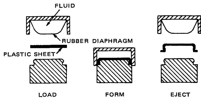
Figure 14. Hydrostatic forming (10)
