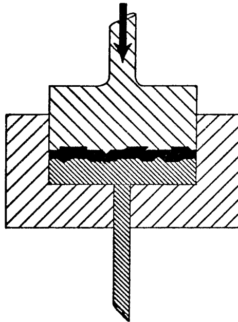
Figure 16. Coining tool (6)
