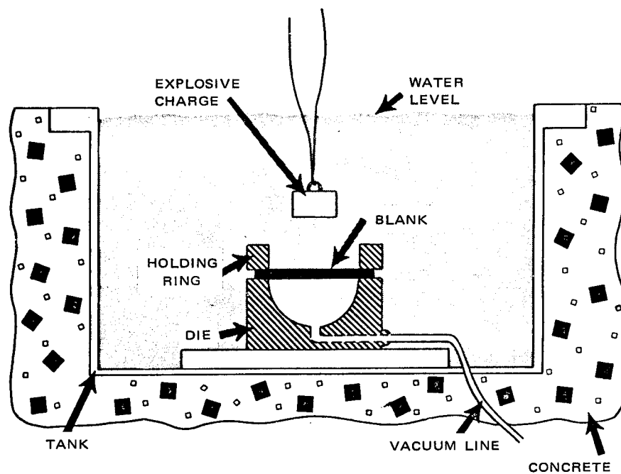
Figure 18. Explosive forming (6)
