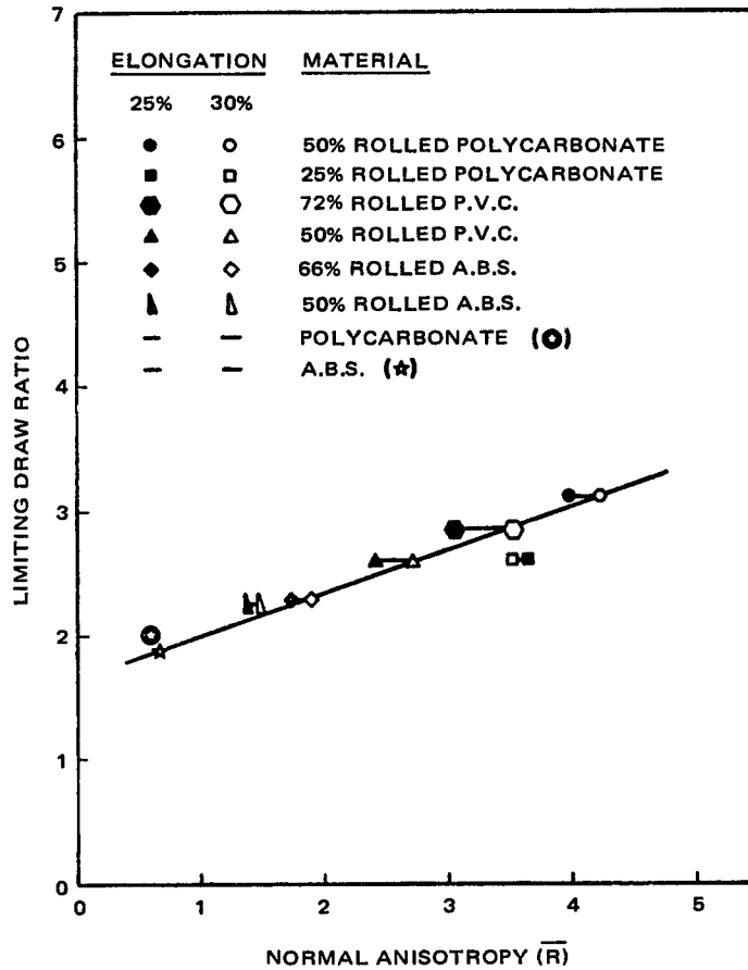
Figure 51. Limiting draw ratio vs. normal anisotropy (20)
