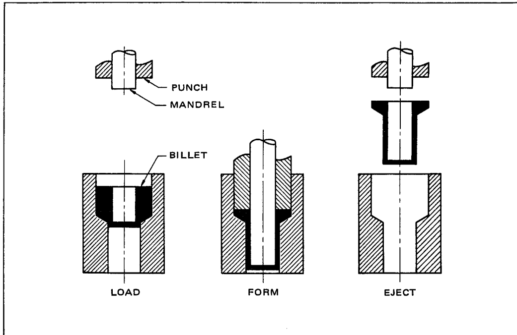
Figure 6. Forward extrusion (2)
