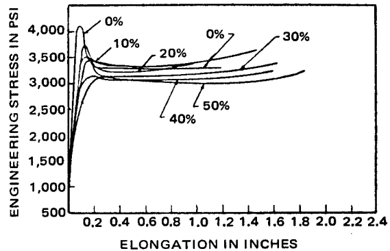
Figure 61. Stress-elongation curves for uniaxially rolled ABS plastic (Cyclocac MS) tested at 90° to the roll direction (22)
