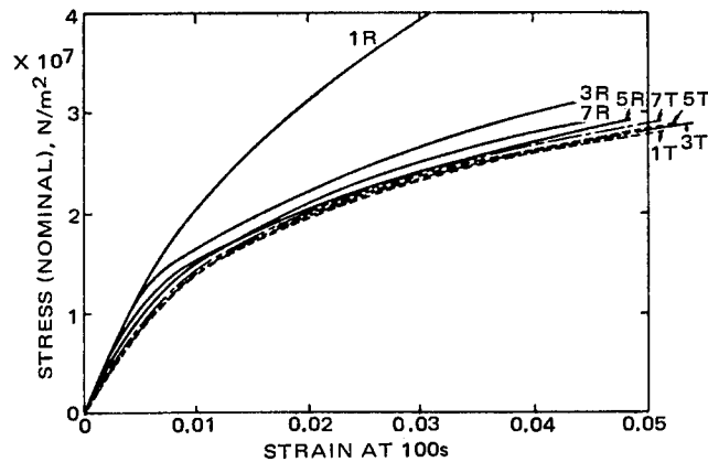
Figure 55. Radial and transverse 100 s isochronous stress/strain curves for forged polypropylene (5)
