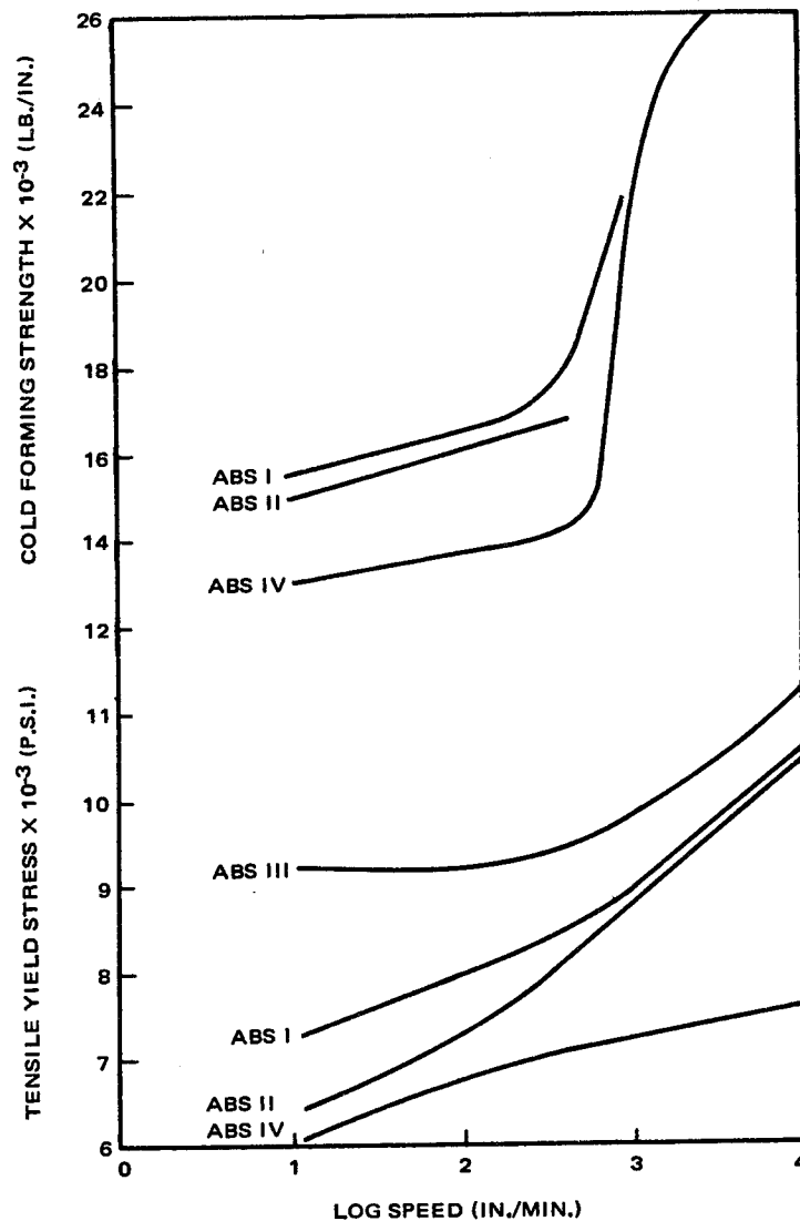
Figure 38. Tensile yield stress and cold forming strength of extruded ABS polymers (16)
