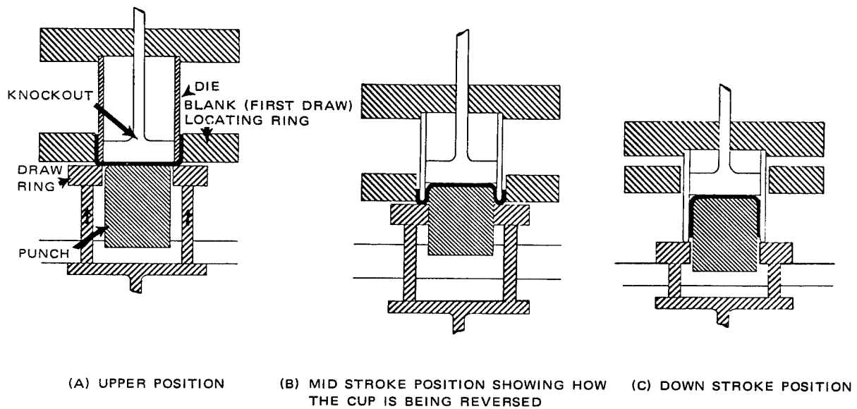
Figure 22. Inverted redraw tool (6)
