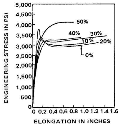
Figure 62. Stress-elongation curves for cross rolled ABS polymer (Cyclocac MS) tested in one of the rolling directions (21)
