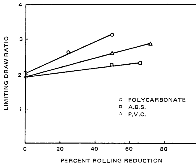
Figure 50. Limiting draw ratio vs. biaxial roll reduction (20)
