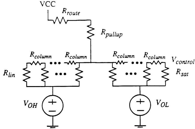
Figure 4.16: Approximate equivalent circuit of a PRL datapath module and a column driver.
