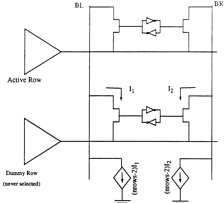
Fig. 5.21: A model of the data-dependent bit-line clamping.
