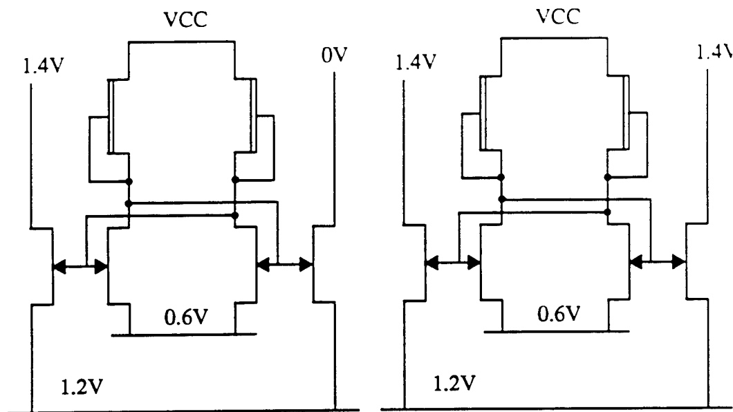
Fig. 2.10: CMMC cell bias during write. (a) selected cell for writing; (b) other cells in selected row.
