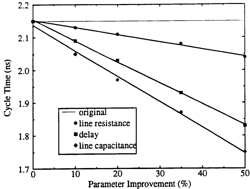
Fig. 5.34: 8kb SRAM cycle time sensitivity to liner resistance, raw gate delay and line capacitance.
