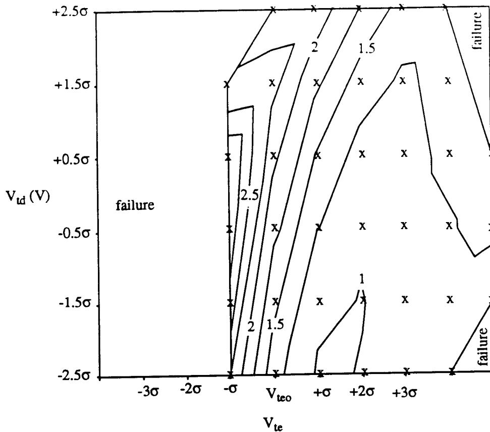
Fig. 3.18: Simulated access time of the asynchronous SRAM as a function of enhancement and depletion threshold voltages.
