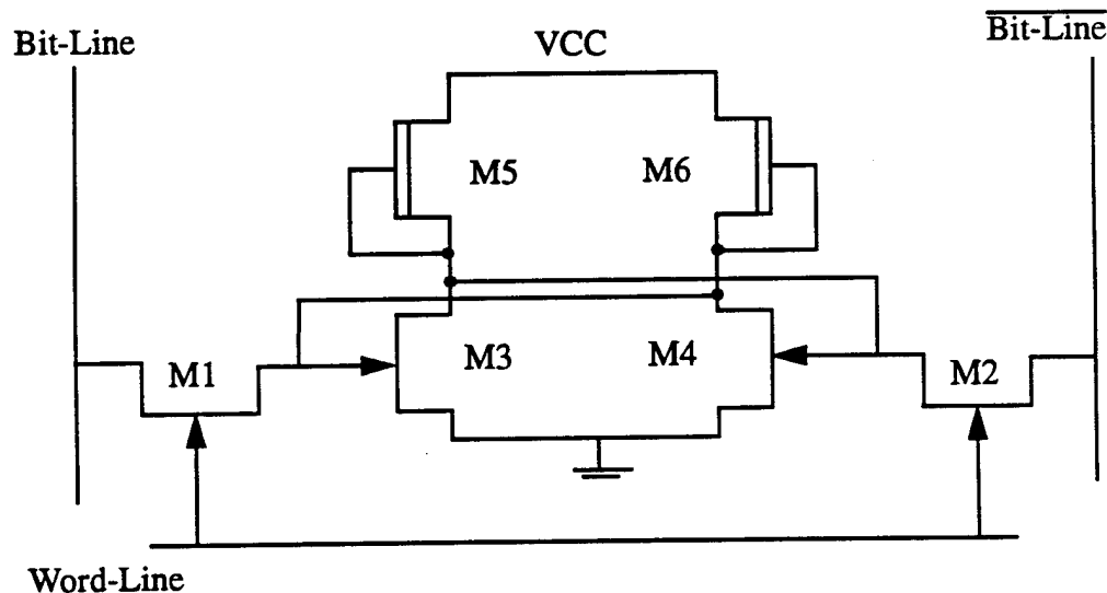
Fig. 2.5: Conventional memory cell
