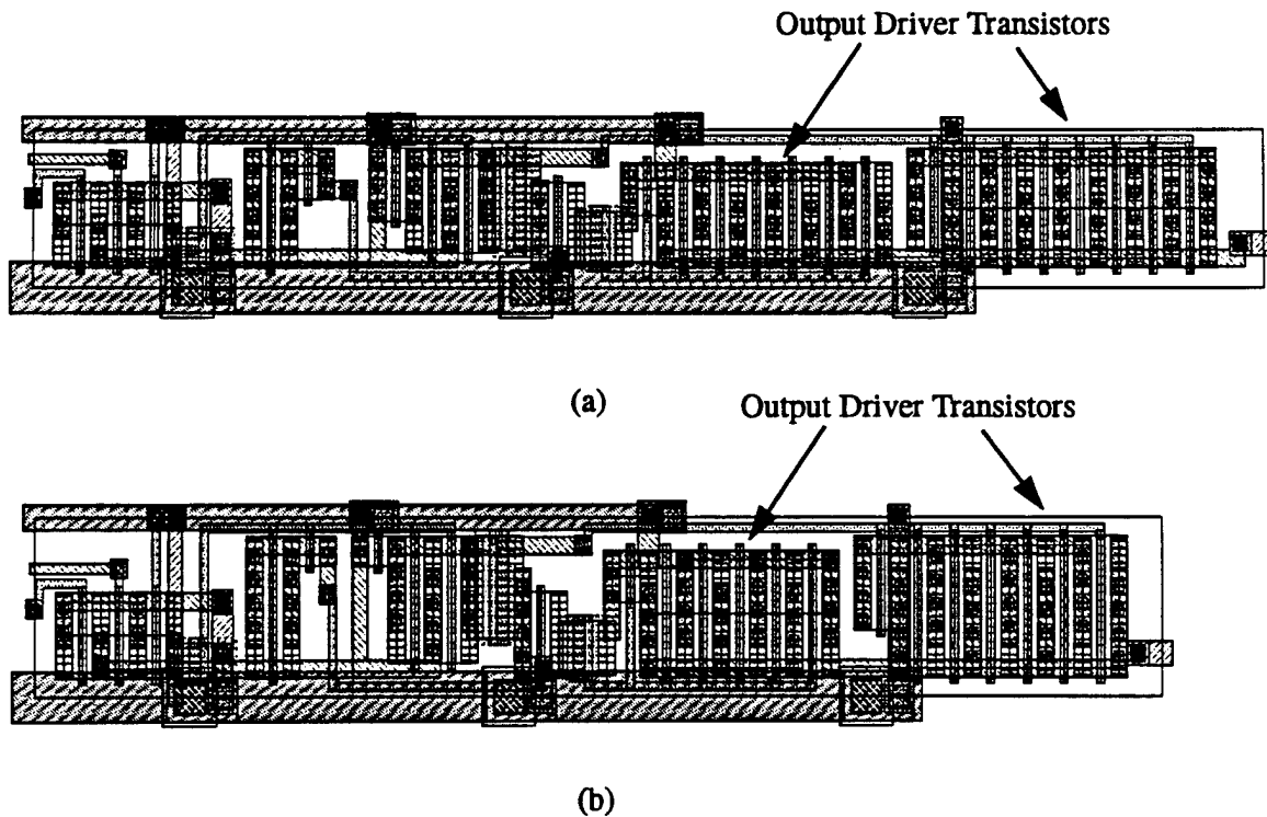
Fig. 5.16: Examples of the scalable word-driver.
