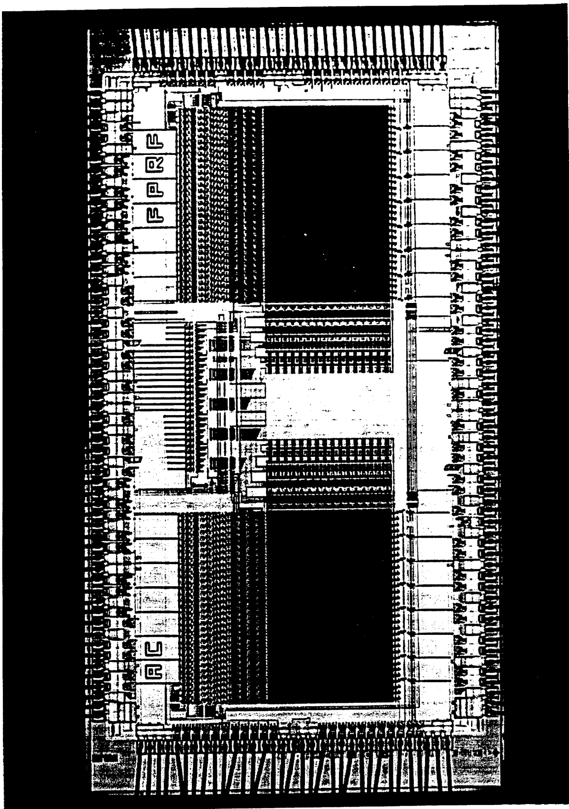
Fig. 2.23: Photomicrograph of the 5-port synchronous SRAM.
