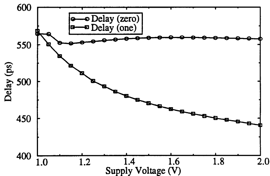
Figure 4.10: Effect of supply voltage on DCFL datapath propagation delays.
