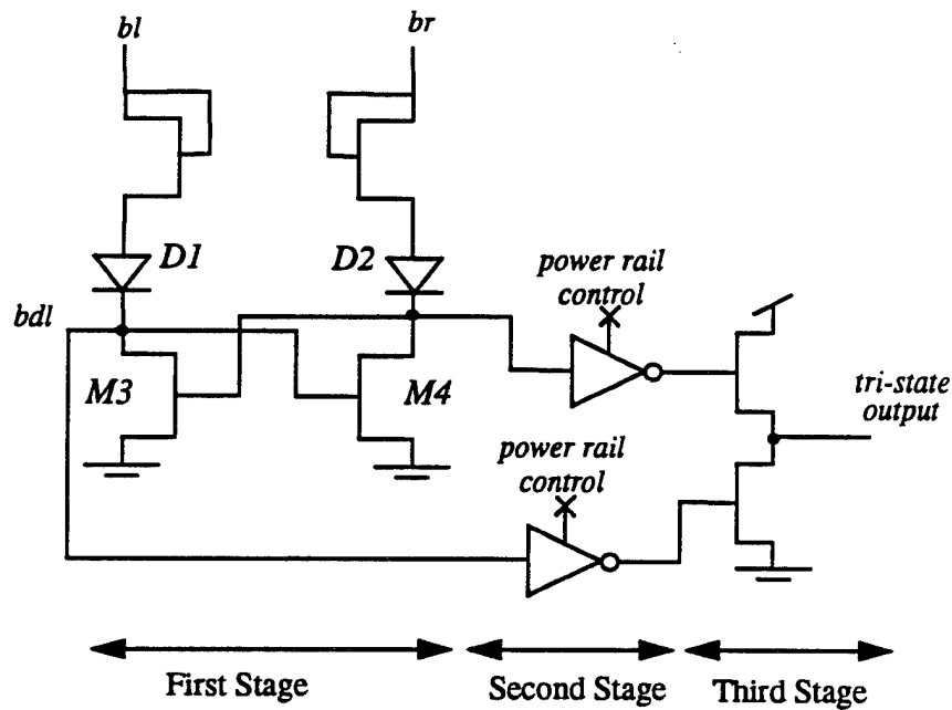
Fig. 5.10: Sense-amplifier schematic.
