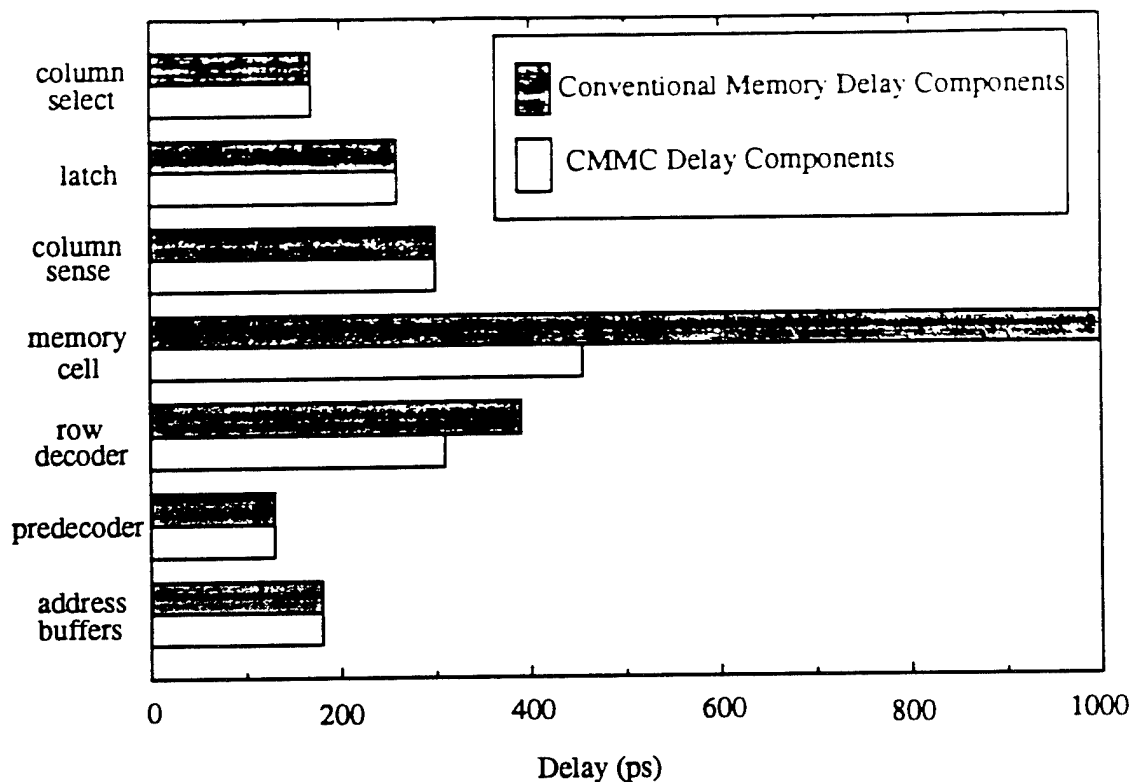
Fig. 2.9: Delay comparisons for the access times of a 4kb SRAM.
