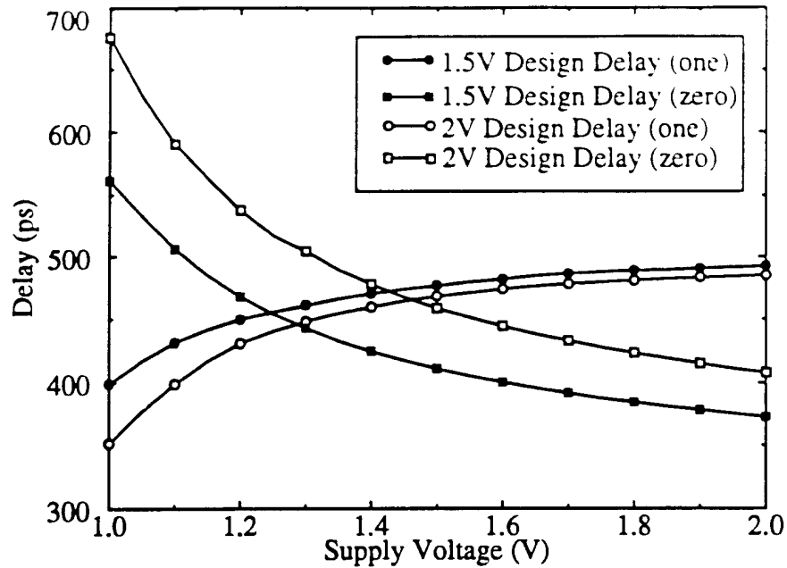
Figure 4.9: Effect of supply voltage on PRL datapath propagation delays.
