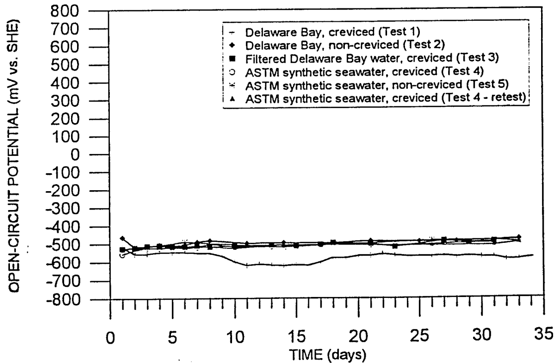
Figure 23. Open-circuit potential vs. time for weldment #8-b (AL 5086/AL 5556, brushed).
