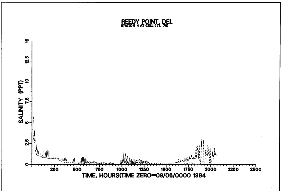
Figure 18d. Computed (___) versus recorded (---) salinity at Reedy Point (2.5 m)
