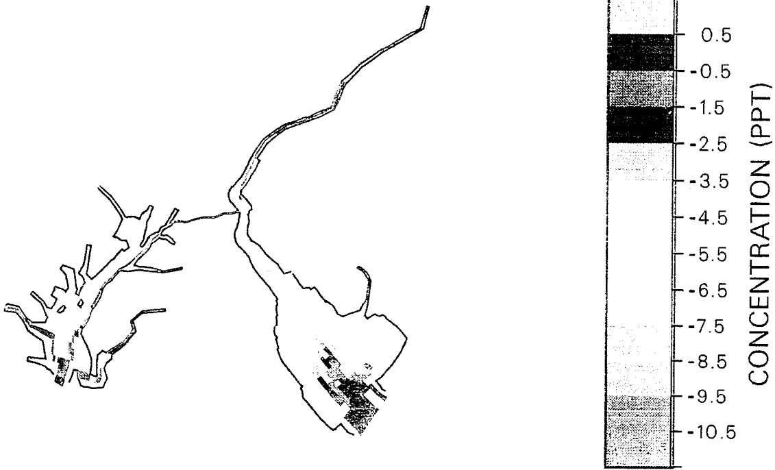
Figure 28d. Differences of seasonal averaged salinity (1972 vs 1985) in layer 10 (9.8 m)
