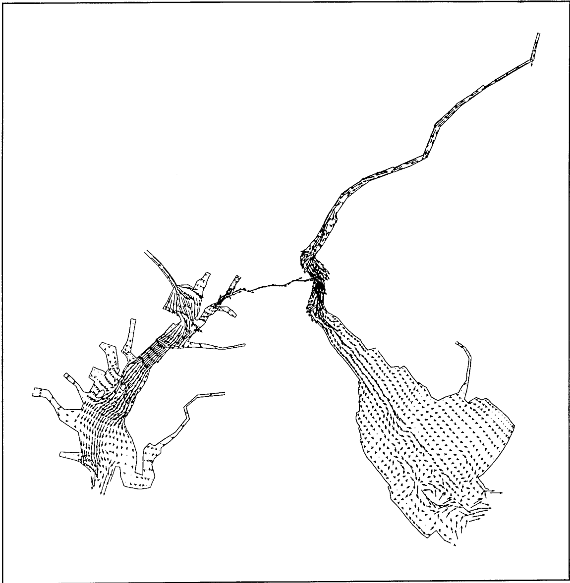
Figure 25a. Seasonal averaged flow (highest-low flow, 1972) in layer 16 (0.8 m)
