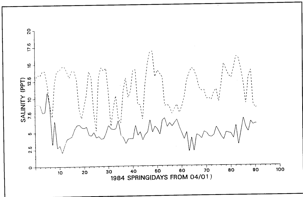
Figure 15b. Synthesized surface (solid line) and bottom (dashed line) salinity boundary at Chesapeake Bay Bridge
