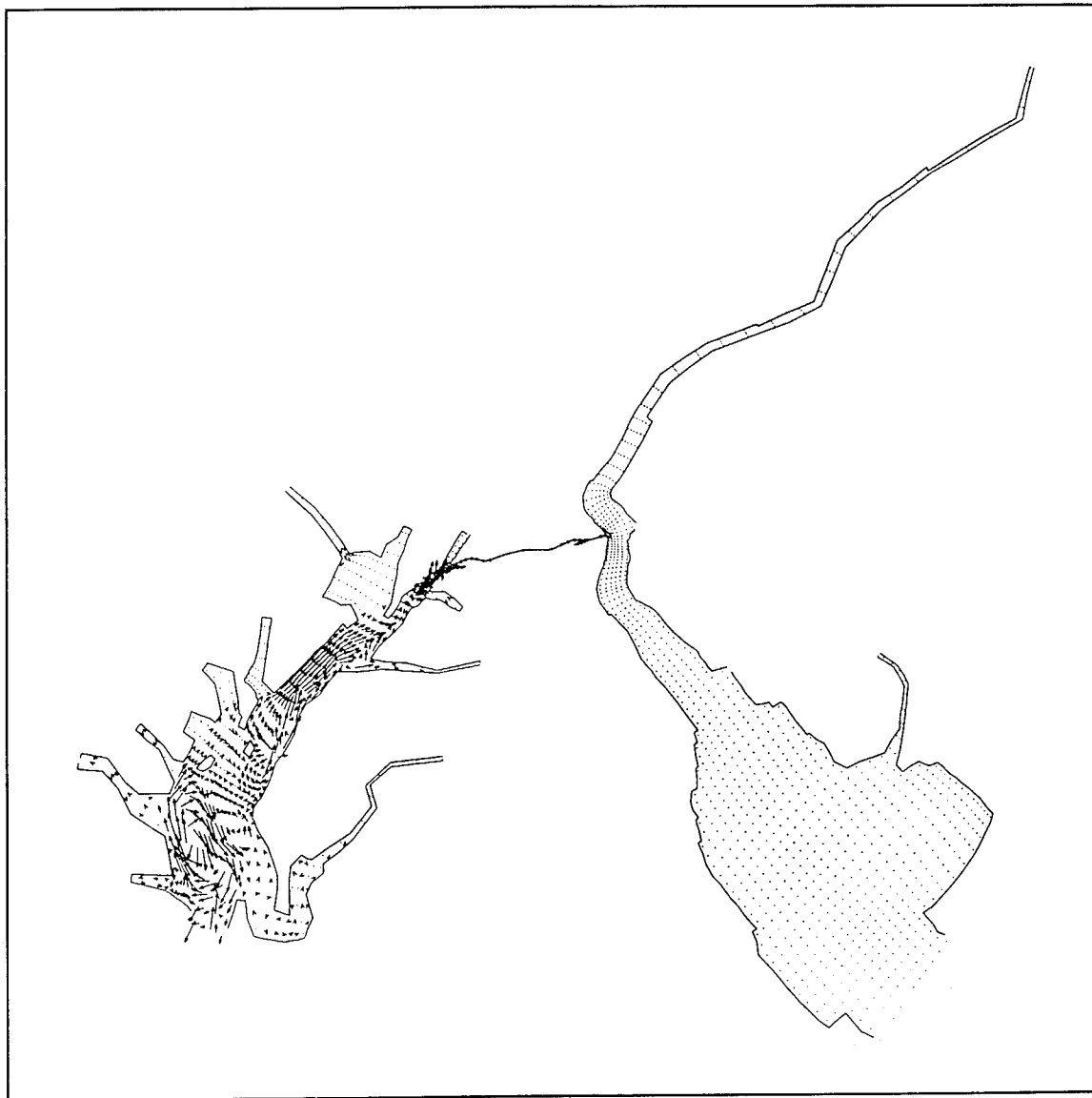
Figure 31a. Differences of seasonal averaged flow (highest-high, 1972) due to proposed channel deepening in layer 16 (0.8 m)
