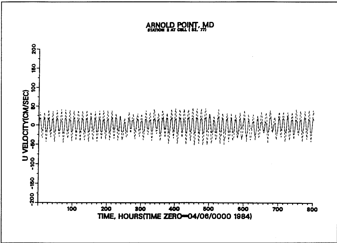
Figure 8c. Computed (____) versus recorded (----) velocity at Arnold Point (4 m)
