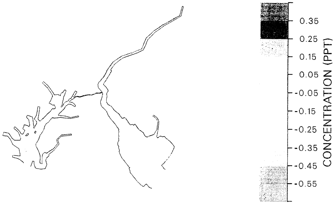
Figure 31b. Differences of seasonal averaged salinity (highest-high, 1972) due to proposed channel deepening in layer 16 (0.8 m)
