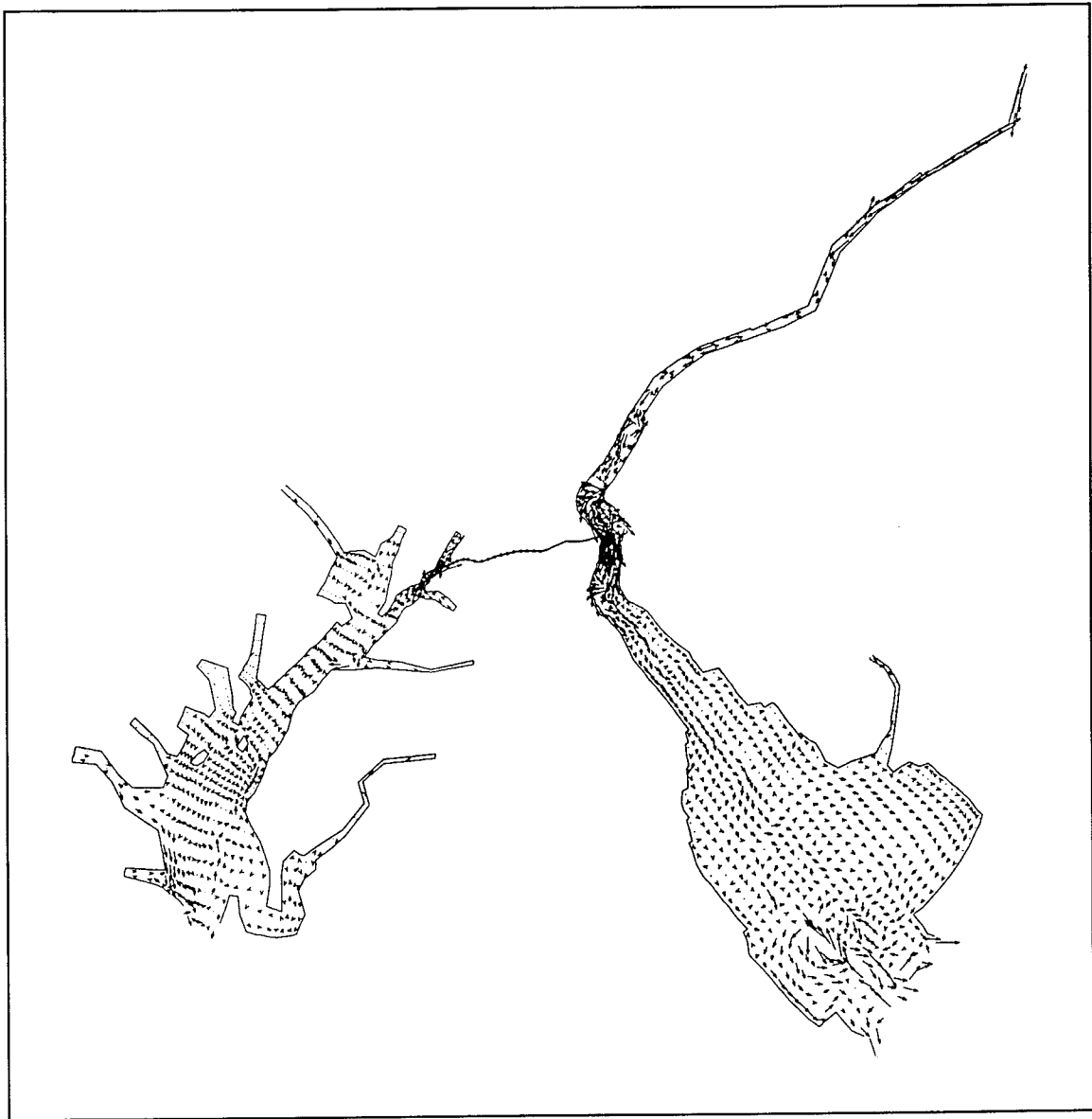
Figure 23a. Seasonal averaged flow (lowest-low flow, 1964) in layer 16 (0.8 m)
