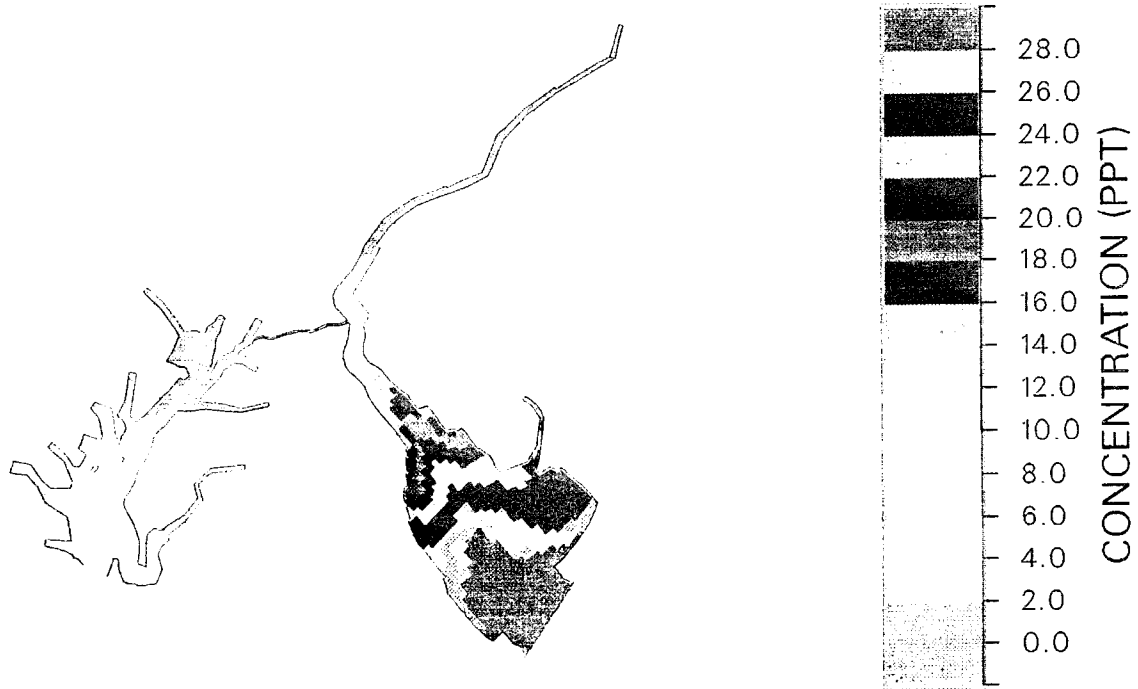
Figure 11a. Seasonal (Fall 1984) averaged salinity (Layer 16, 0.8 m)
