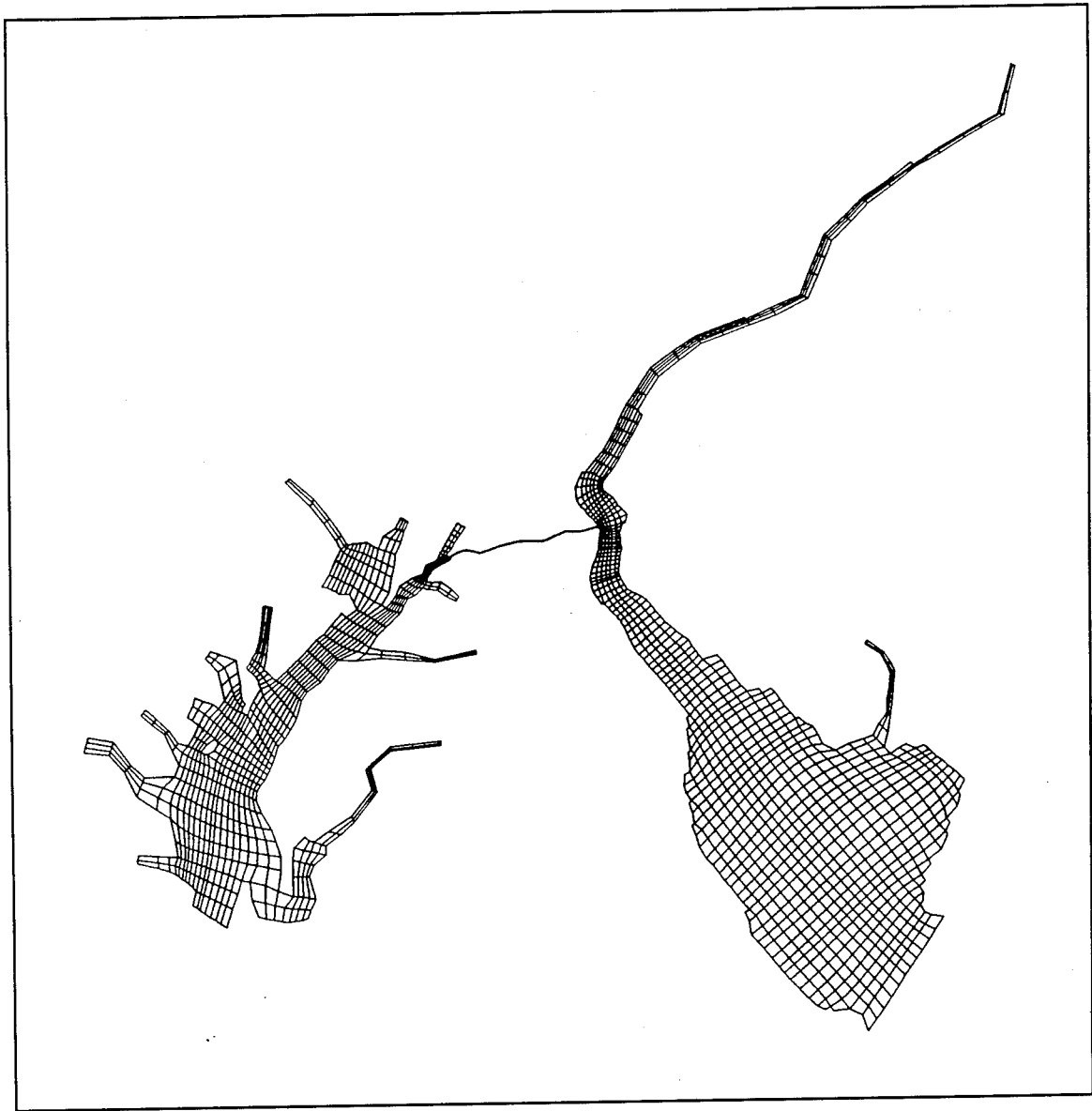
Figure 2. Computational Grid
