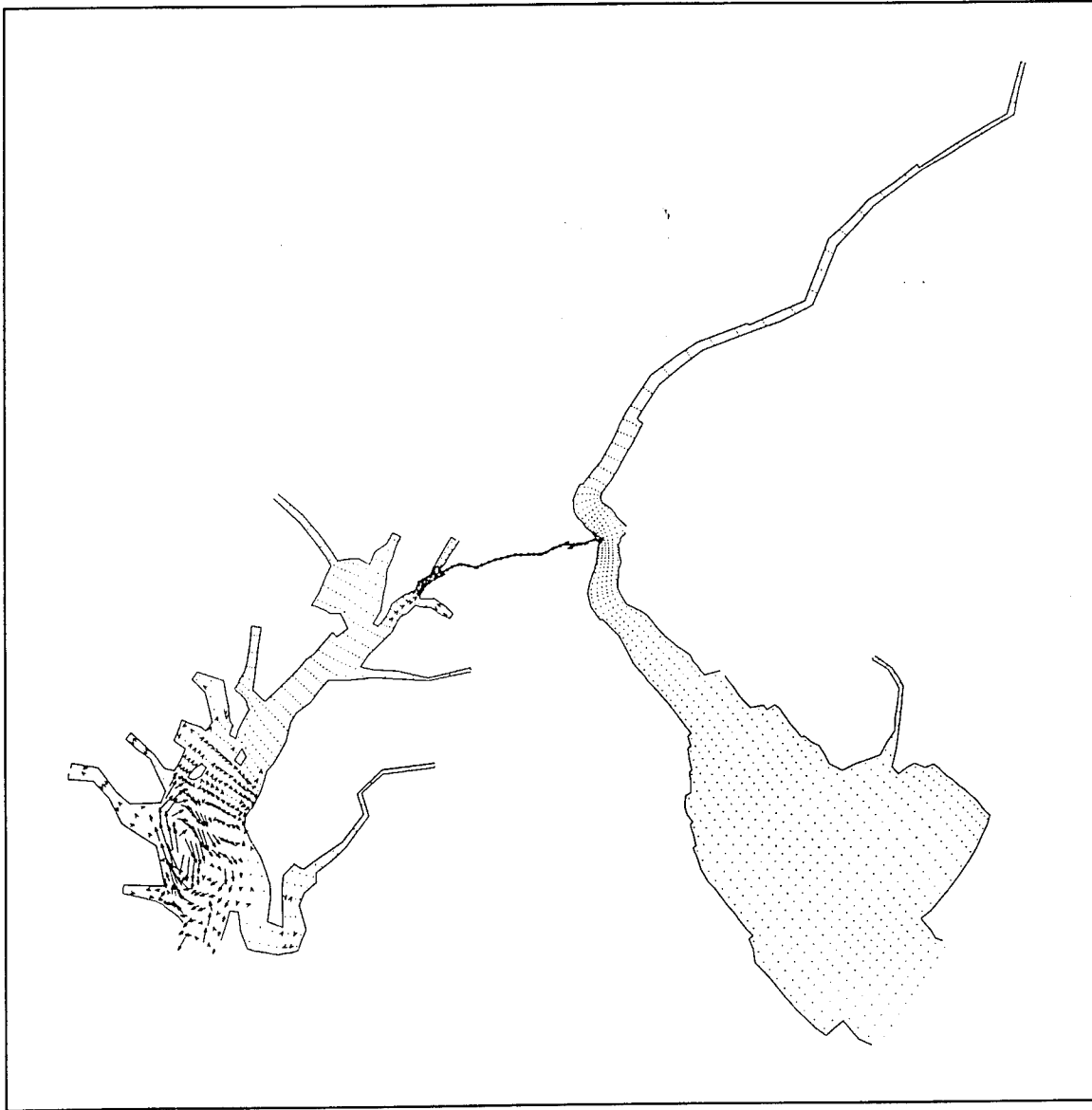
Figure 35c. Differences of seasonal averaged flow (highest-high, 1972) due to channel deepening test 2 in layer 16 (0.8 m)
