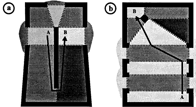
Figure 13: Two examples in which the approach presented here yields suboptimal results. In both cases, the problem is to plan a path from “A” to “B”. (a) The topological planner will chose a sub-optimal path, since it leads only through two intermediate regions (as opposed to three). Such situations occur only if the topological graph contains cycles (which correspond to isolates obstacles in the thresholded grid-based map). (b) The triplet planner fails to move the robot on a straight line, since it looks only two topological regions ahead.
