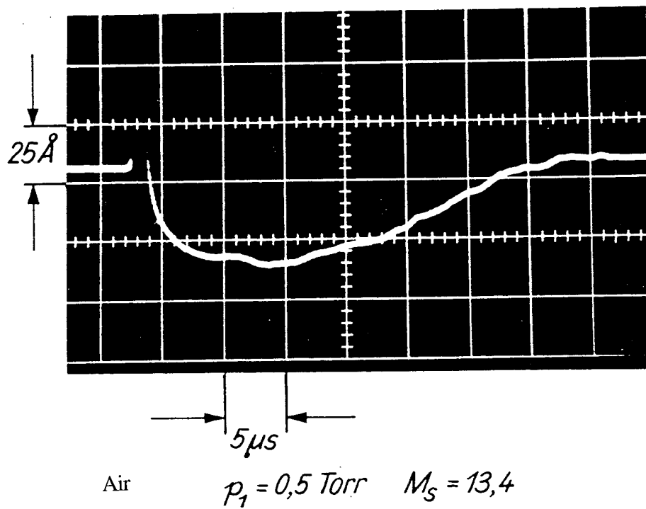
Fig. 7 - Investigation of the Stagnation Region of a Small Sphere
