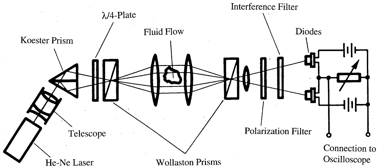
Fig. 3 - Laser-Interferometer (with Compensation of Sensitivity to Vibrations)
