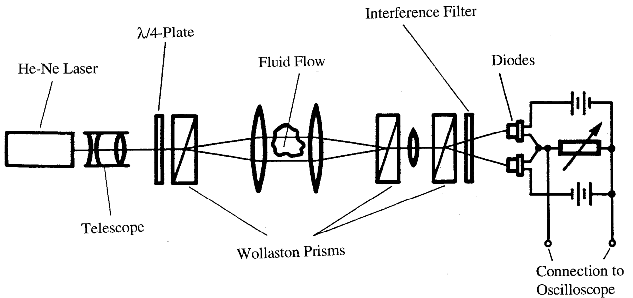
Fig. 2 - Laser-Interferometer
