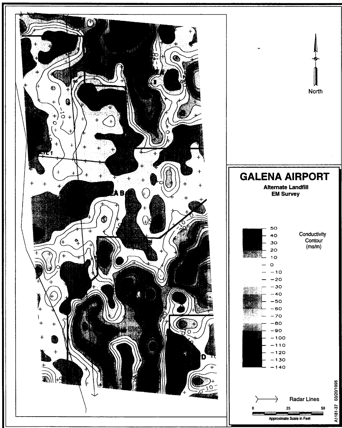
Figure 3.8-1. EM and GPR Contours at the Alternate Landfill
