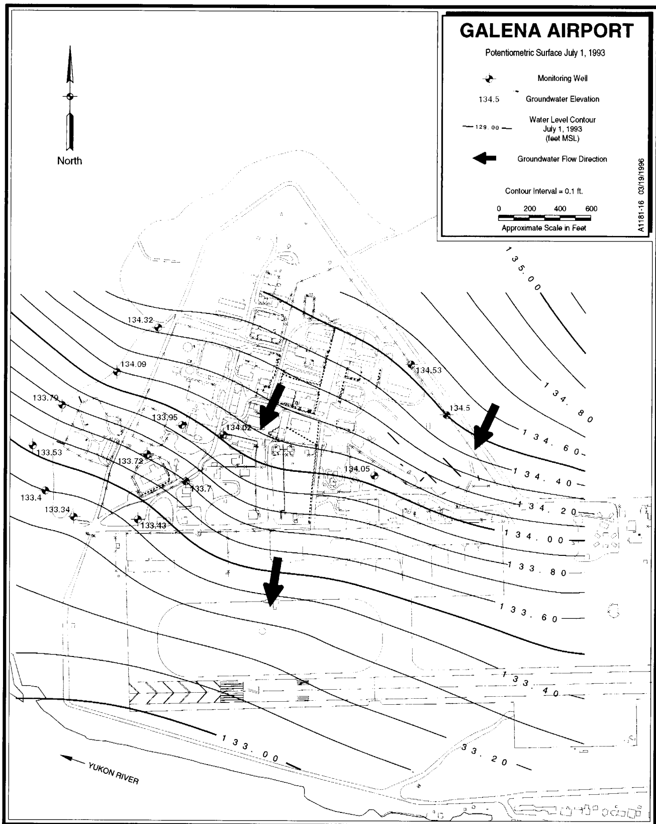
Figure 2.4-7. Galena Airport Basewide Potentiometric Contour Map for July 1993
