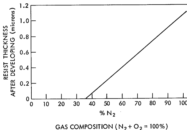
Figure 17—Effect of gas composition on resist thickness.
