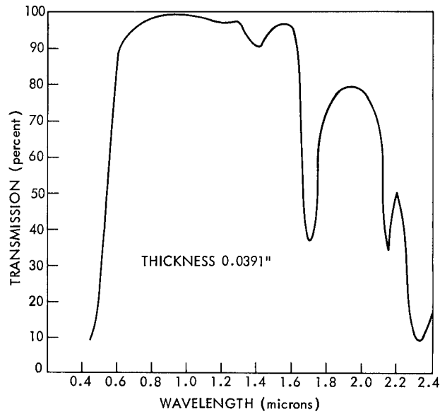
Figure A3—Transmission of supernatant KMER after application of high voltage.
