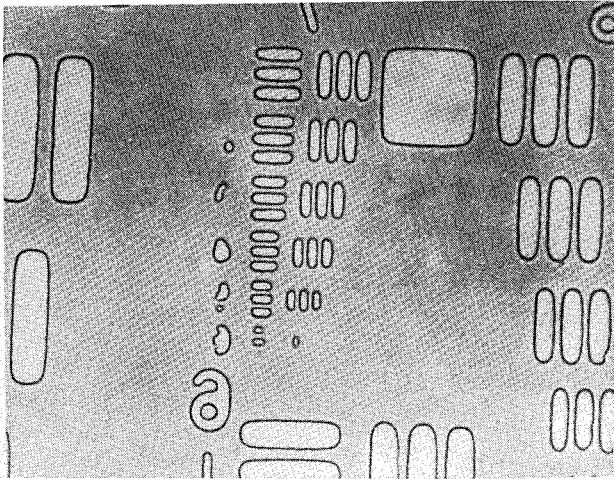
Figure A5—Pattern showing WSR printed and developed on a silicon dioxide surface (500X).
