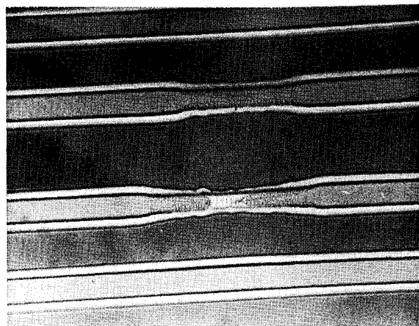
Figure 10—A defect caused by improper coating of the resist.
