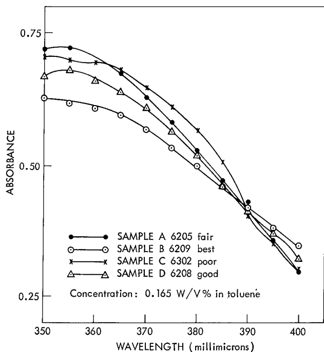
Figure A1—Transmission of four KMER samples.
