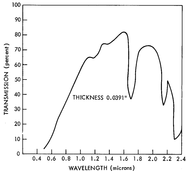
Figure A4—Transmission of KMER sludge after application of high voltage.
