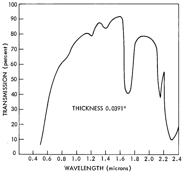
Figure A2—Transmission of normal KMER not subjected to high voltage.
