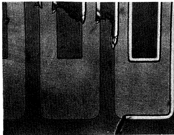
Figure 4—Resist torn away from wafer exposing etched lines (500X).
