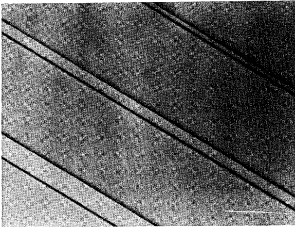
Figure 11—Line widths of 0.0001, 0.00025, and 0.0005 inch printed in 1.7 micron resist (550X).
