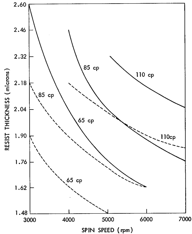
Figure 9—Coating thickness for modified KMER with KMER thickness in microns as a function of spin speed showing viscosity of resist; ----- shows resist coated on spinner with lapsed time to full speed of less than one second; ——— shows resist coated on spinner with lapsed time to full speed of five to fifteen seconds.
