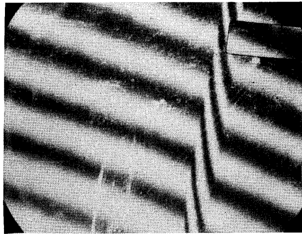
Figure 2—Aluminized wafer showing thickness of oxide (3600 Å) by fringe measurement.
