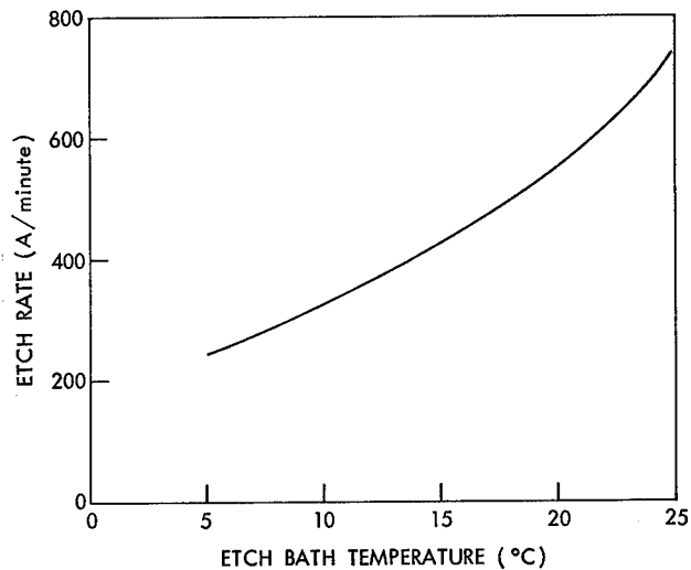
Figure 3—Etch rate of steam-grown silica films in nine percent \text{NH}_4\text{F} -buffered HF.
