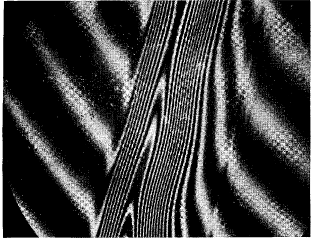
Figure 5—Fringe measurement of resist thickness ( 16 - 9 = 7 fringes, or 1.7 microns).
