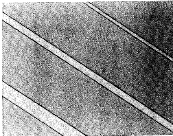
Figure 12—Lines etched in 6000 A oxide with resist removed (550X).
