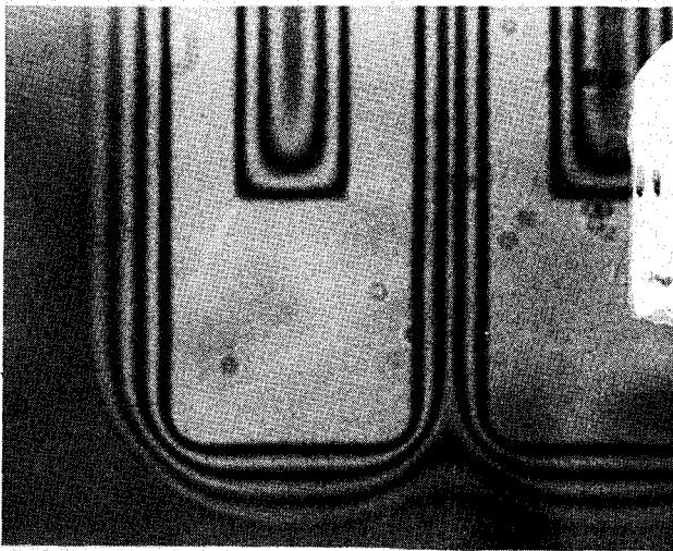
Figure 1—Etched oxide showing undercutting of resist by etch solution (500X).
