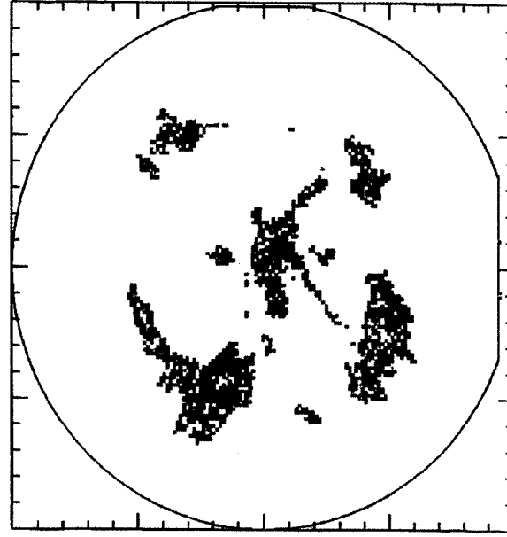
Dislocation Density
