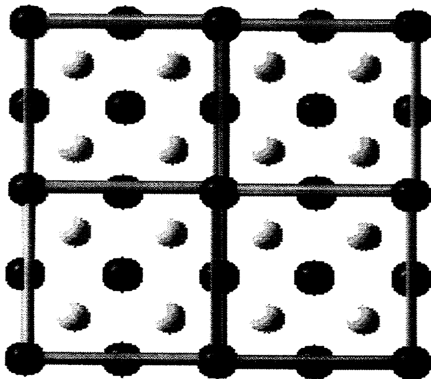
ORDERED DIAMOND TERNARY
