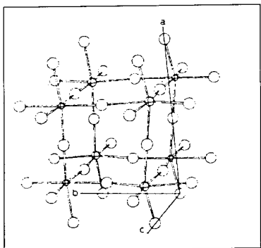
Figure 7. WO 3 structure 16 .
