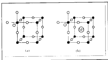
Figure 6. (a) ReO 3 structure; (b) Perovskite-like tungsten bronze structure. Filled circles are W 6+ , open circles are O 2- , M 1 is a metal ion 15 .
