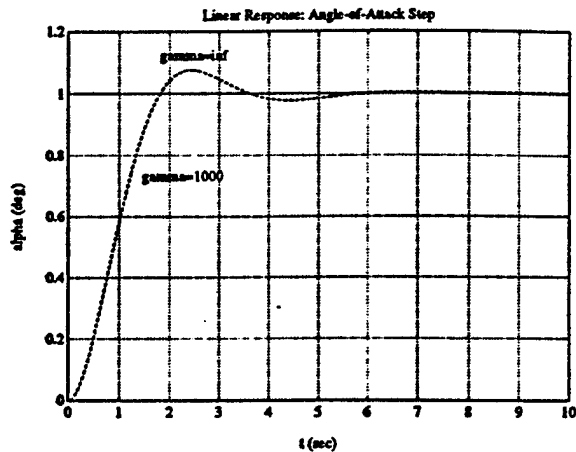
Figure 8. Angle-of-Attack Linear Step Response
