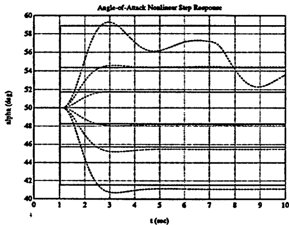
Figure 10. Angle of Attack Nonlinear Step Response
