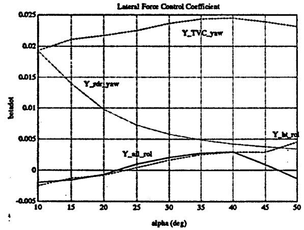
Figure 4. Variation in Lateral Force Control Coefficients with Angle of Attack
