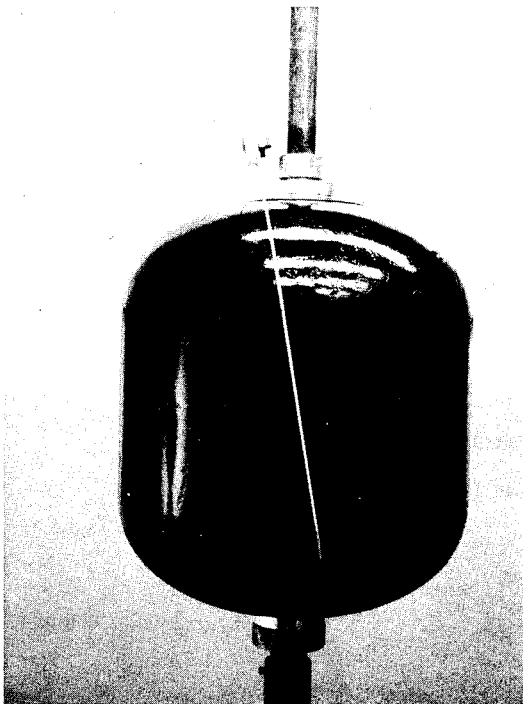
Fig. C-2 Front View of First Polar Encirclement of Roving Around Mandrel
