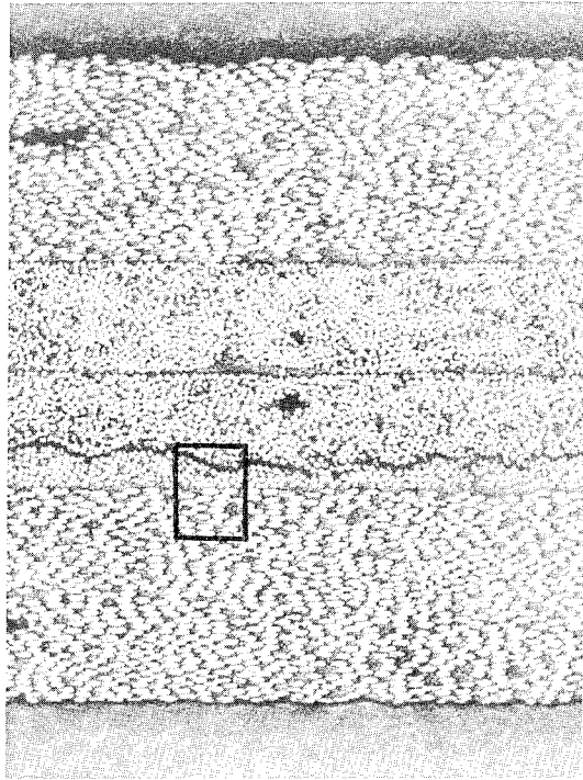
Fig. 13 Cylinder 9, Photomicrograph of Cylinder Wall (Taken at an angle of 19^{\circ}30' with respect to the axis of the cylinder, 80X)
