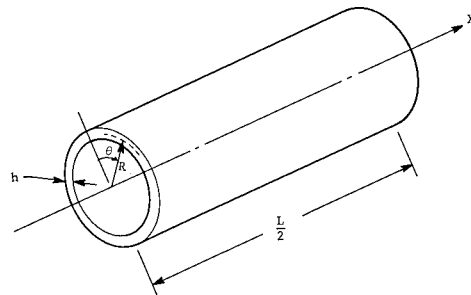
Fig. B-1 Cylindrical Coordinate System for Composite Shell
