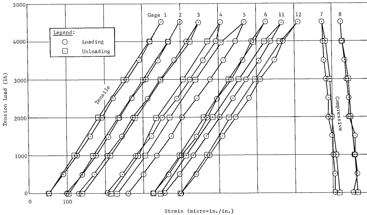
Fig. 3 Cylinder 9, Tension Load vs Strain
