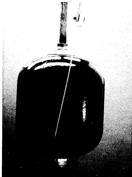
Fig. C-3 Rear View of First Polar Encirclement of Roving Around Mandrel
