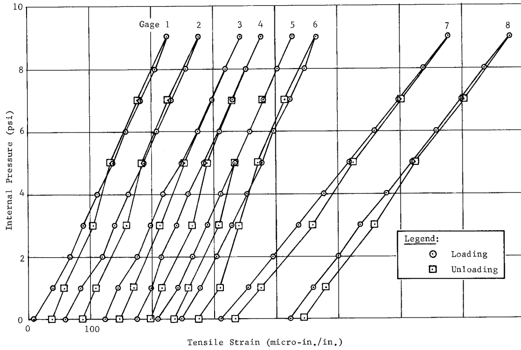
Fig. 2 Cylinder 9, Internal Pressure vs Strain
