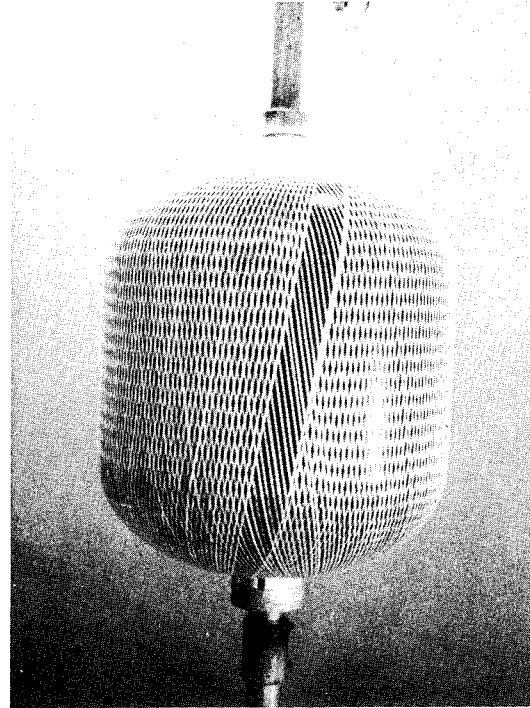
Fig. C-7 Rear View Just Before Mandrel has Completed a 360-deg Rotation
