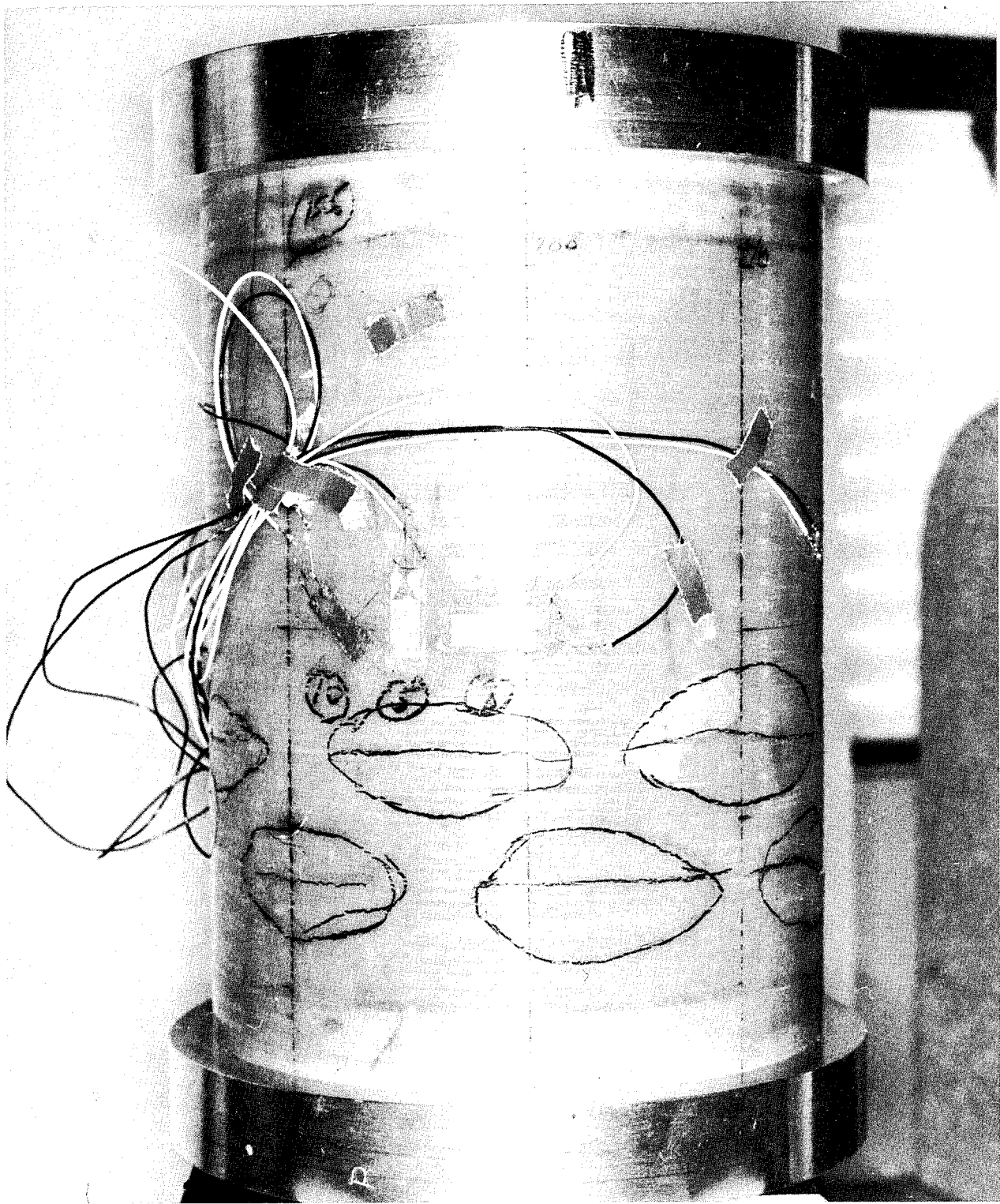
Fig. 8 Cylinder 1 (6-in. dia) after Test
