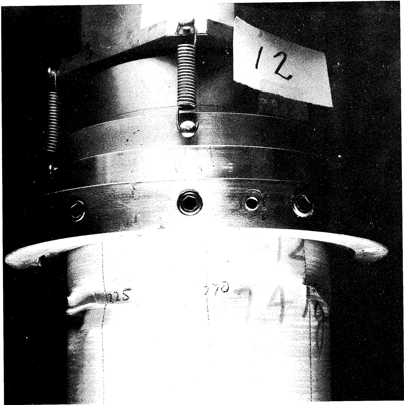
Fig. 6 Cylinder 12 (6-in. dia) in Postbuckled State
