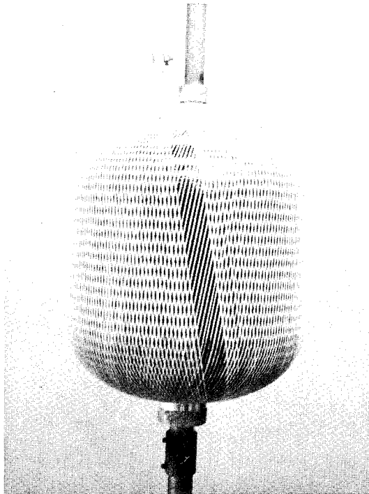
Fig. C-6 Front View Just Before Mandrel has Completed a 360-deg Rotation
