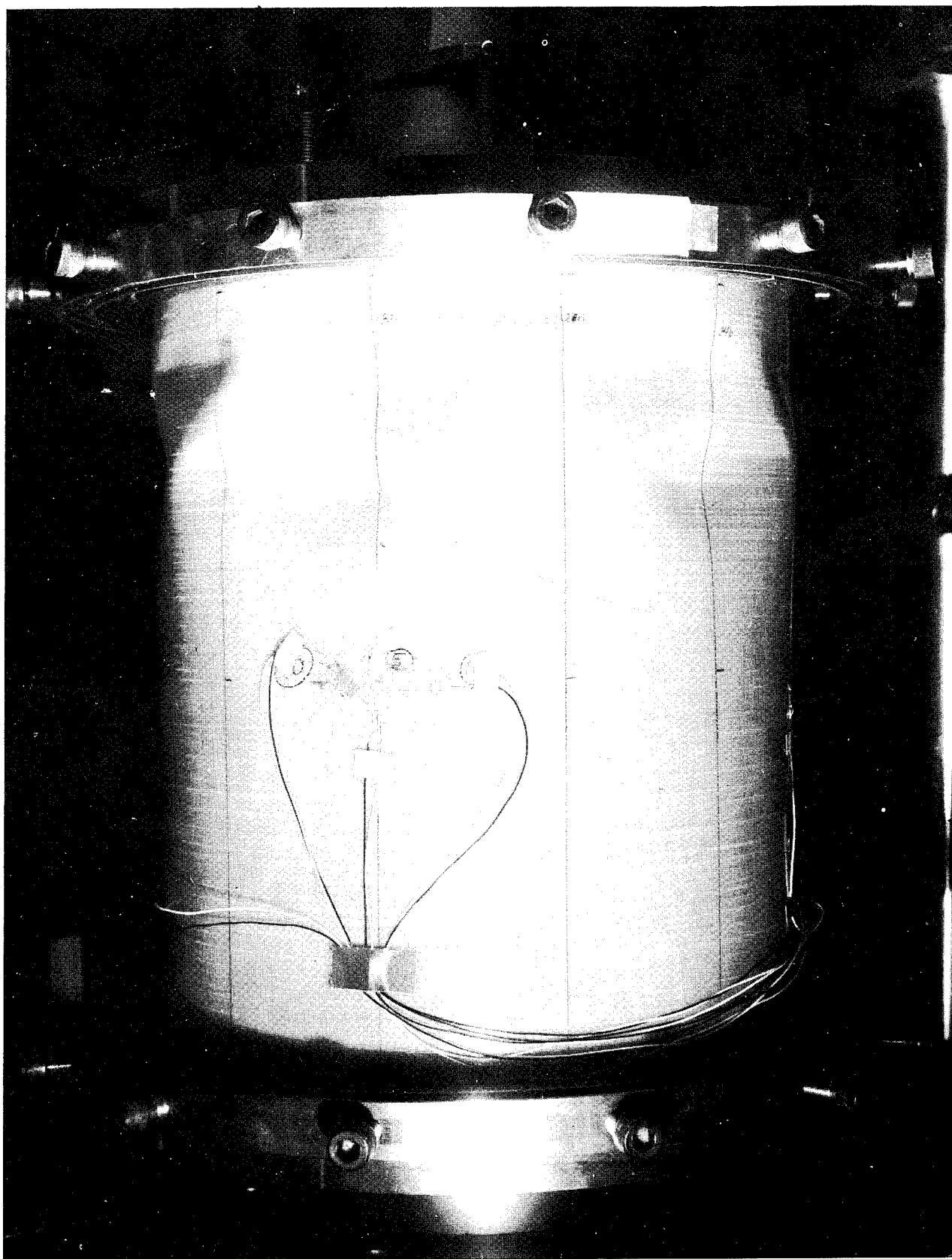
Fig. 9 Cylinder 4 (12-in.dia) in Postbuckled State
