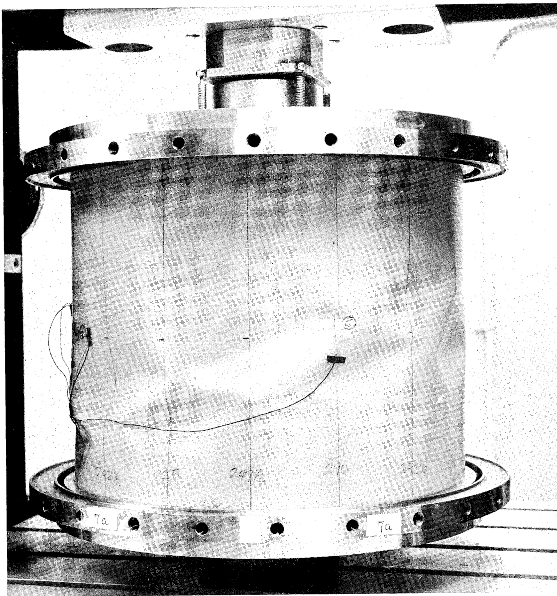
Fig. 15 Cylinder 7a (Shortened 18-in. dia Cylinder) in Postbuckled State
