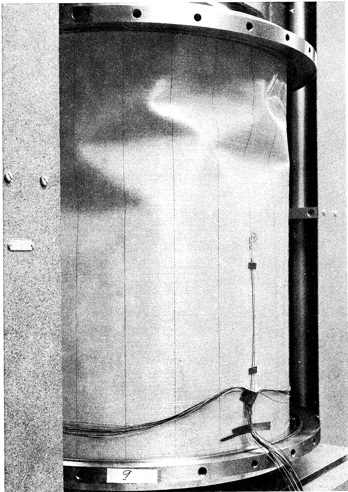
Fig. 12 Cylinder 9 (24-in. dia) in Postbuckled State
