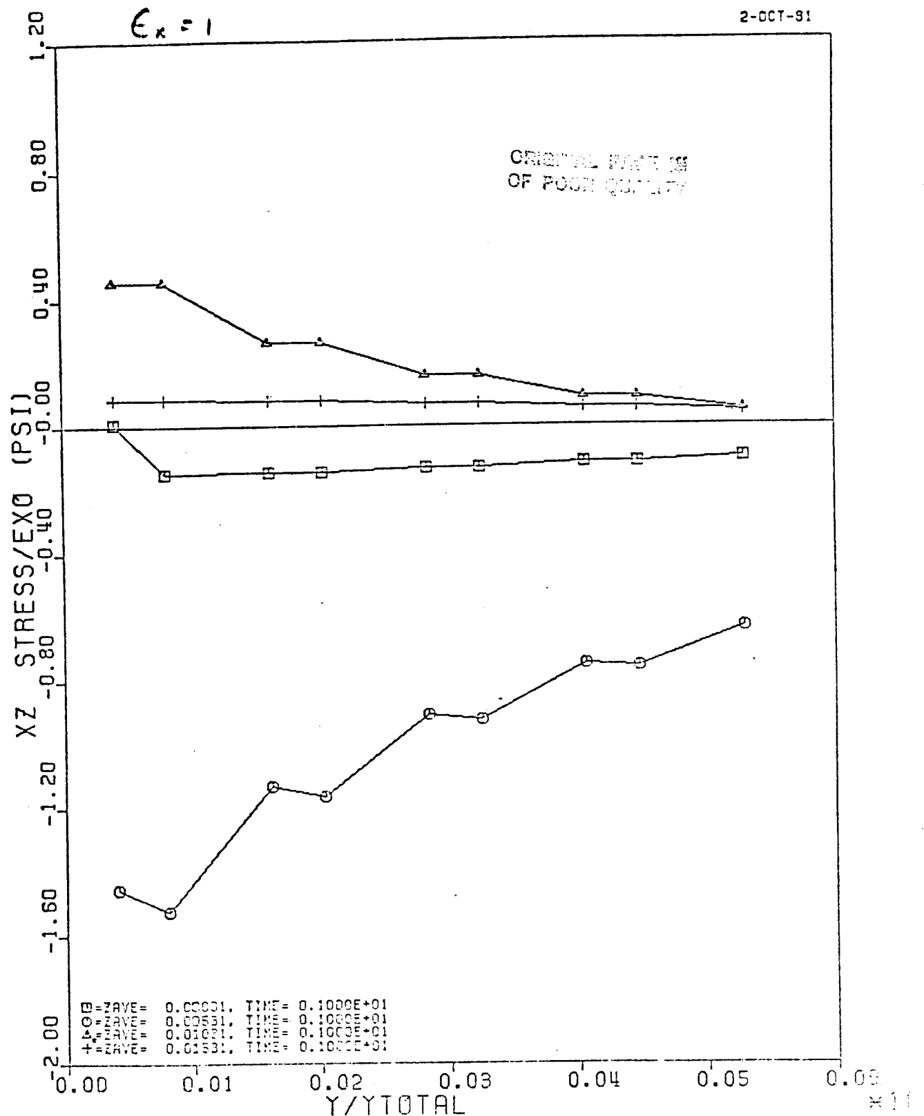
Figure D24: \sigma_{xz} Free Edge Stress for (0/90/+45)_s Laminate as a Function of Y, Uniform Tensile Strain, \epsilon_x D-39
