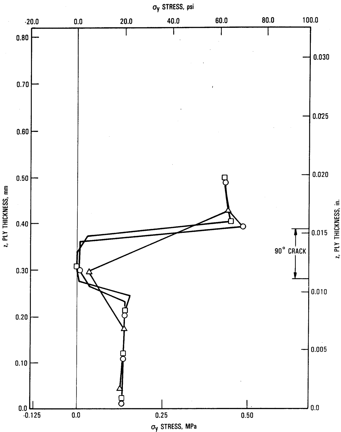
Figure 87: \sigma_y stress gradients near a 90^\circ ply crack in a (0/90/+45)_s laminate.
