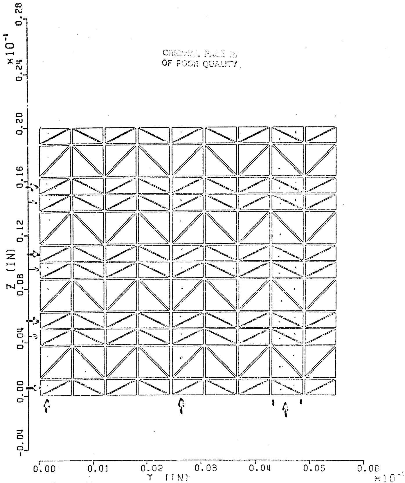
Figure D18: Detail of Finite Element Model Used to Calculate Free Edge Stresses in (0/90/+45)_s Laminate.
