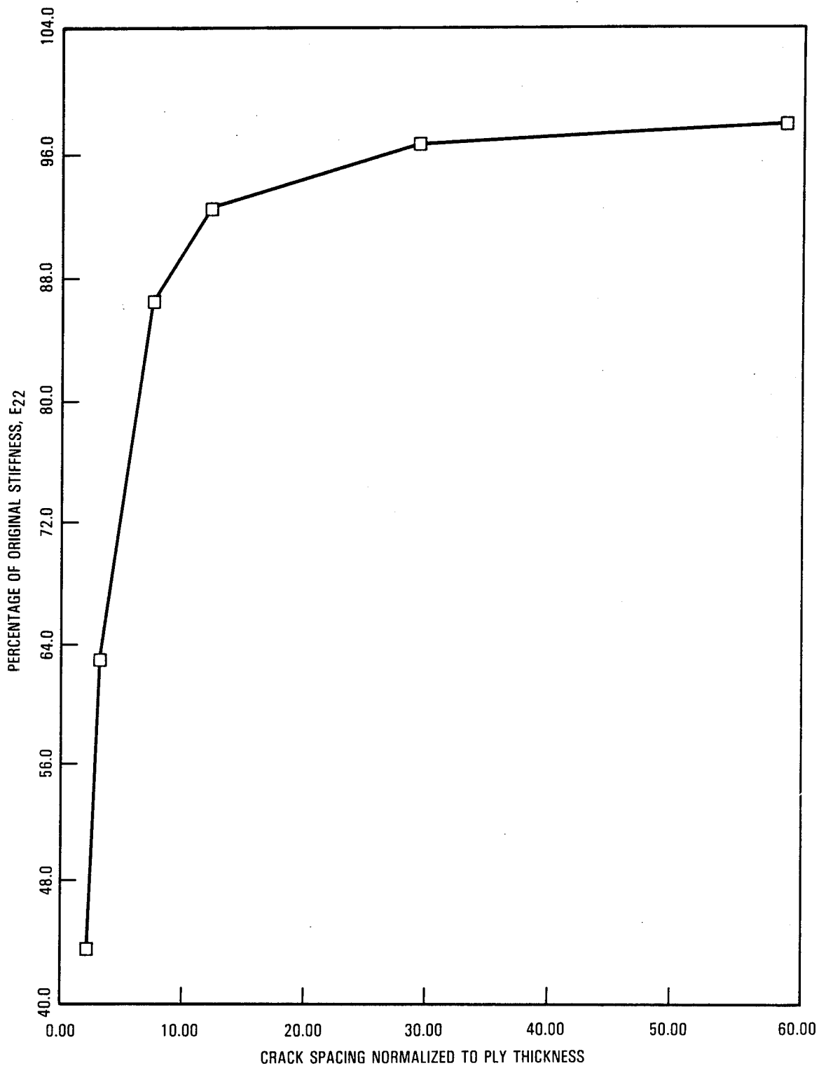
Figure 60: Effective modulus E_2 for a (0/90)_s laminate.
