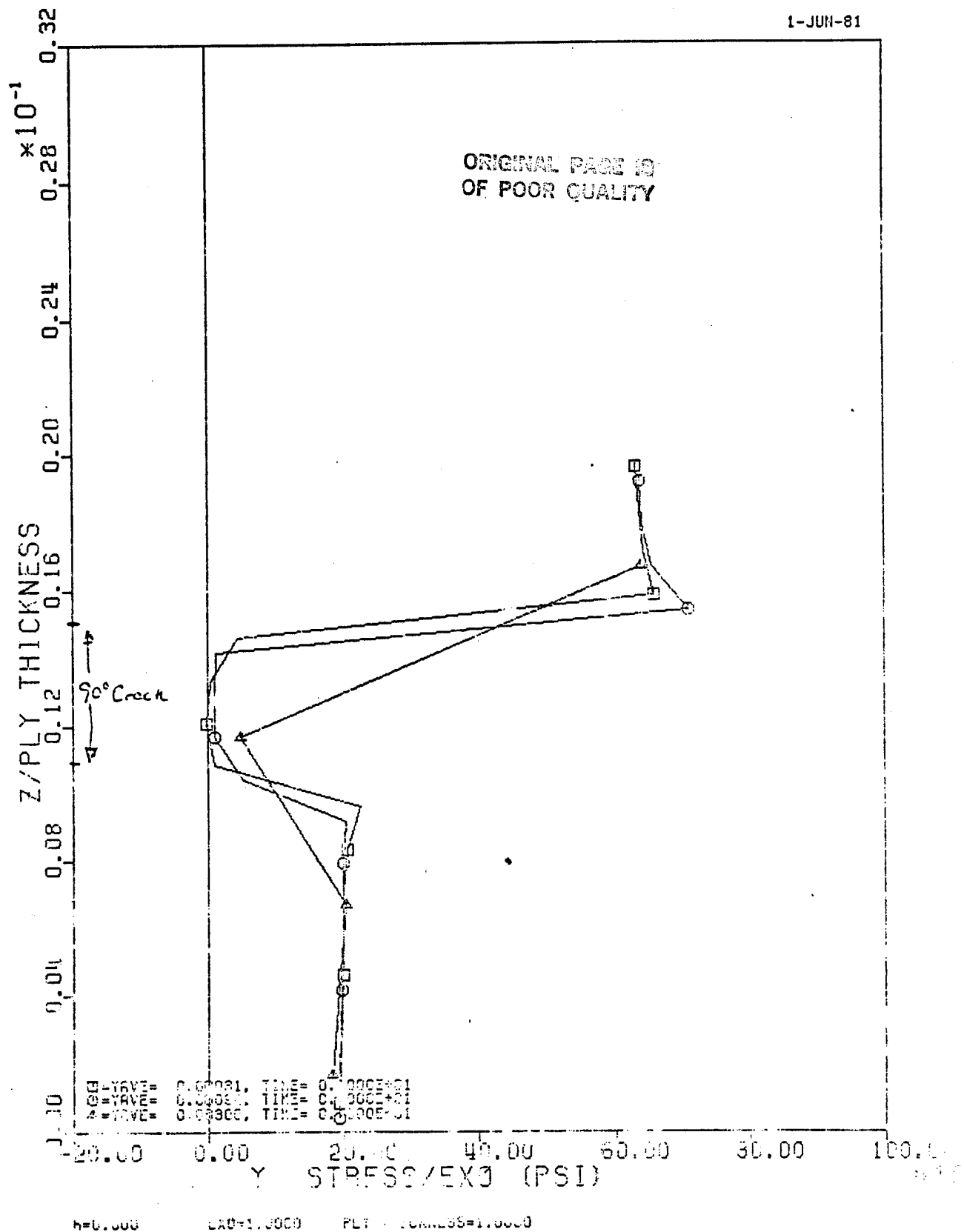
FIGURE D15: \sigma_{yy} Stress as a Function of z
