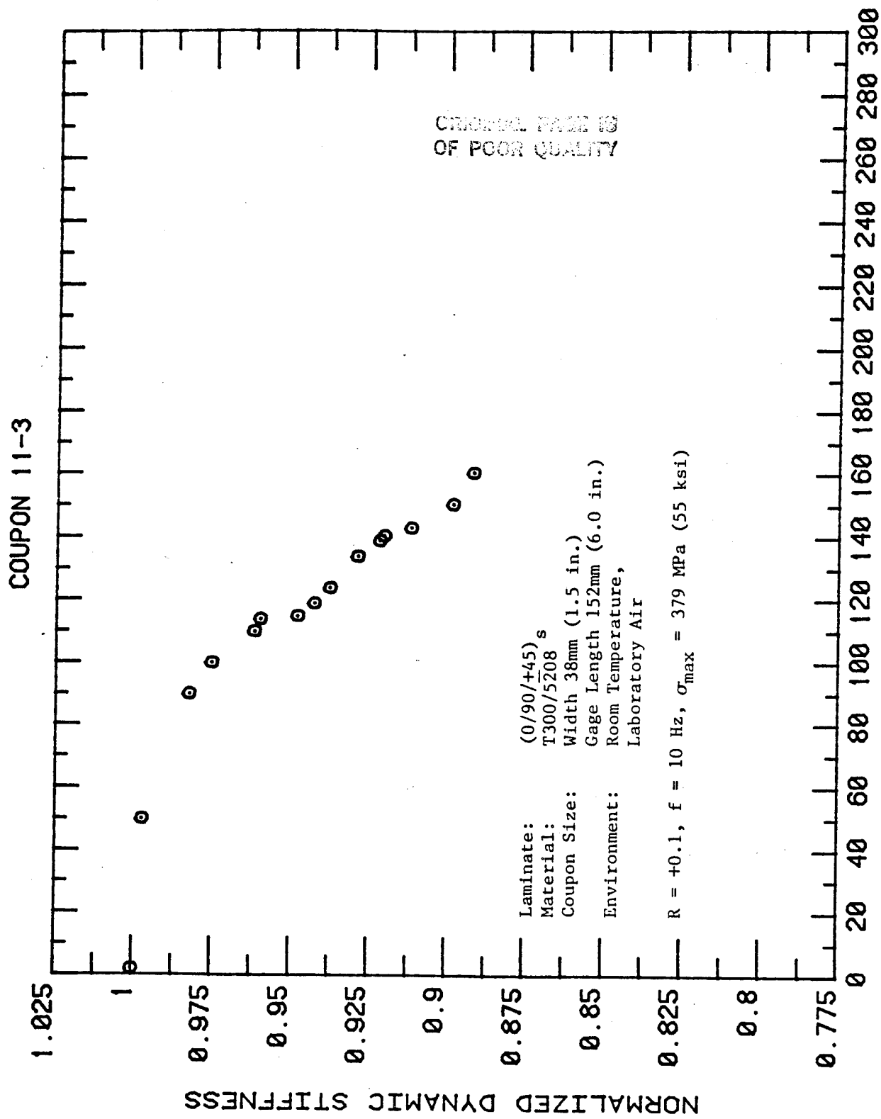
Figure C8: Normalized Dynamic Stiffness vs. Constant Amplitude Fatigue Load Cycles for (0/90/+45) s Laminate Coupon 11-3, \sigma_{\max} = 379 \text{ MPa (55 ksi)}
