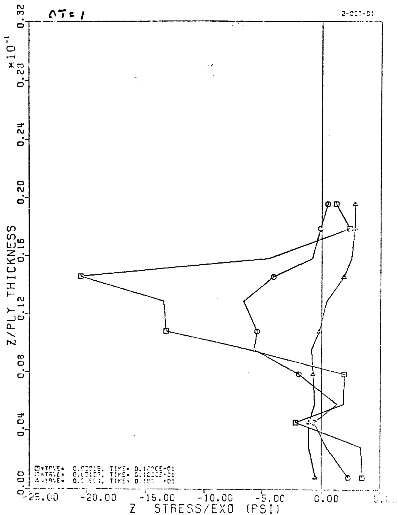
Figure D25: \sigma_z Free Edge Stress for (0/90/+45) Laminate as a Function of z , Uniform temperature Change, D-40 ^{\circ}\text{C} (100 ^{\circ}\text{F} )
