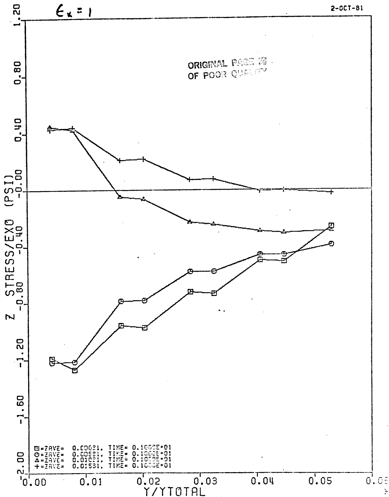
Figure D22: \sigma_z Free Edge Stress for (0/90/+45) s Laminate as a Function of Y, Uniform Tensile Strain, \epsilon_x D-37
