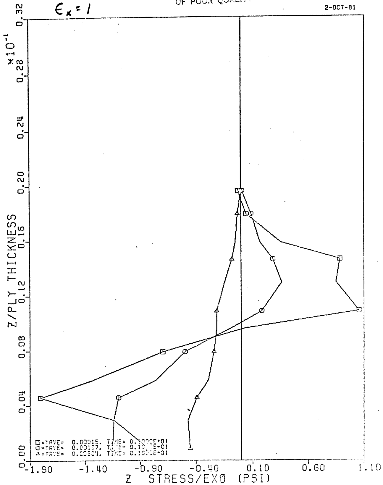
Figure D19: \sigma_z Free Edge Stress for (0/90/+45)_s Laminate as a Function of Z , Uniform Tensile Strain. D-34
