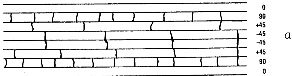
Characteristic damage state for (0/90/45/-45)_s
