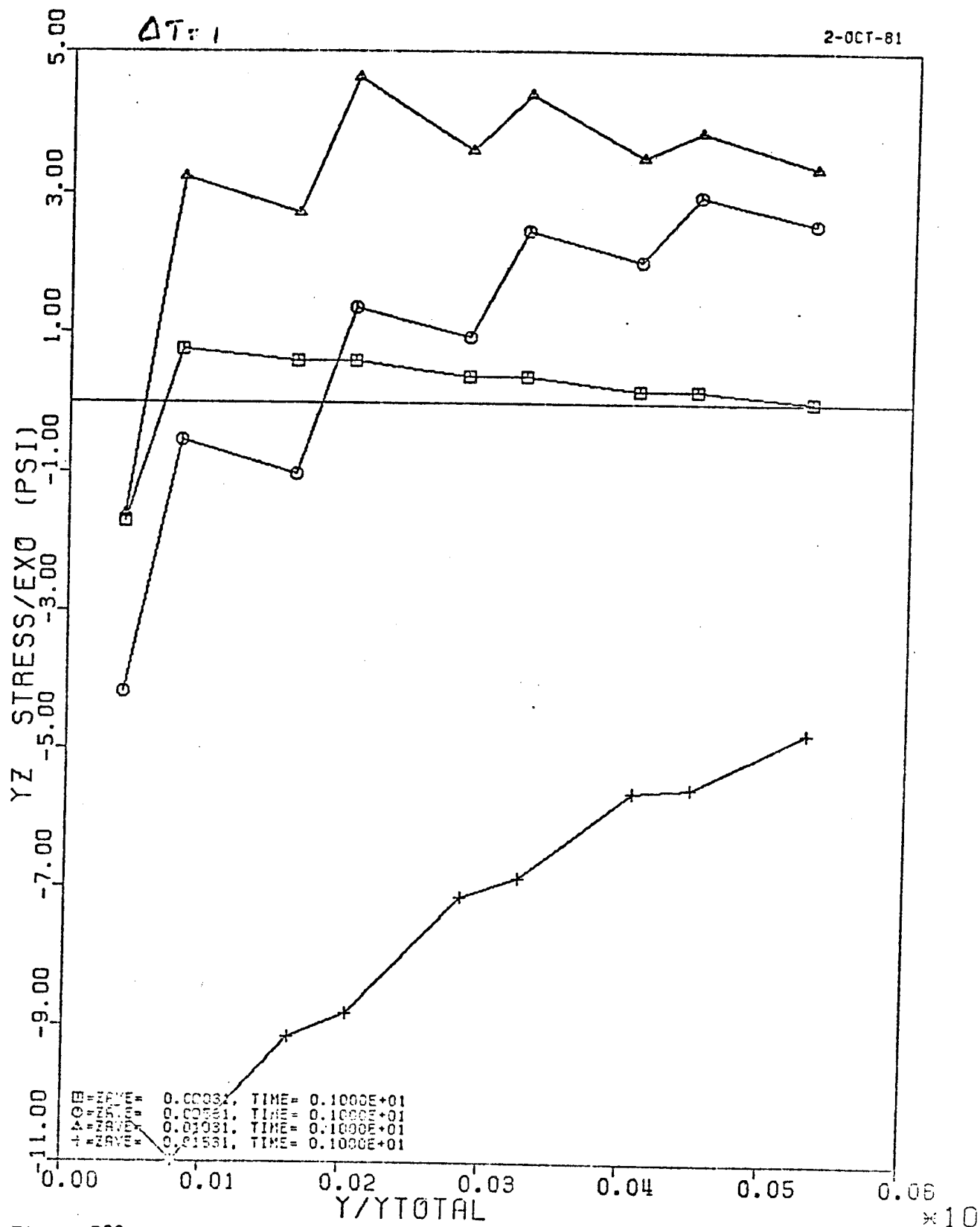
Figure D29 \sigma_{yz} Free Edge Stress for (0/90/+45) Laminate as a Function of Y, Uniform Temperature Change, 0.5^{\circ}\text{C} ( 10^{\circ}\text{F} ).
