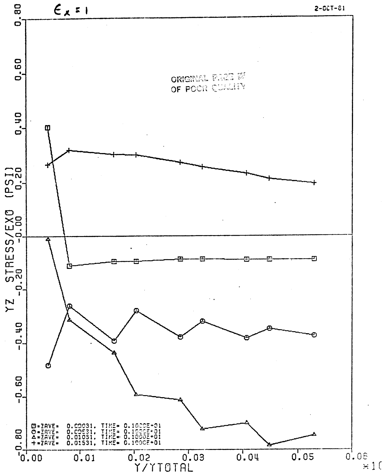
Figure D23: \sigma_{yz} Free Edge Stress for (0/90/+45)_s Laminate as a Function of Y, Uniform Tensile Strain, \epsilon_x D-38
