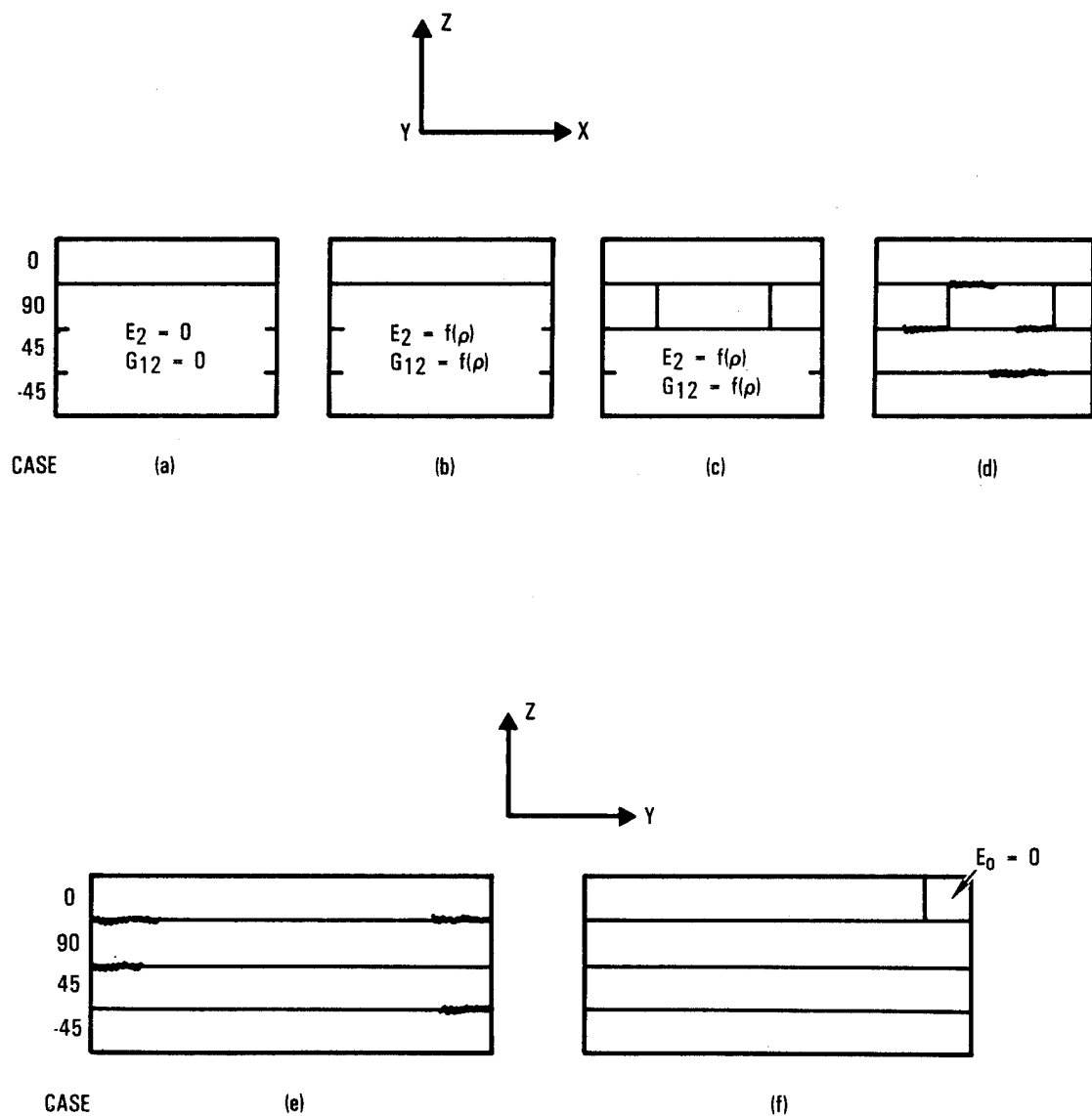
Figure 52: Section models of damage state in a (0/90/+45)_s laminate.
