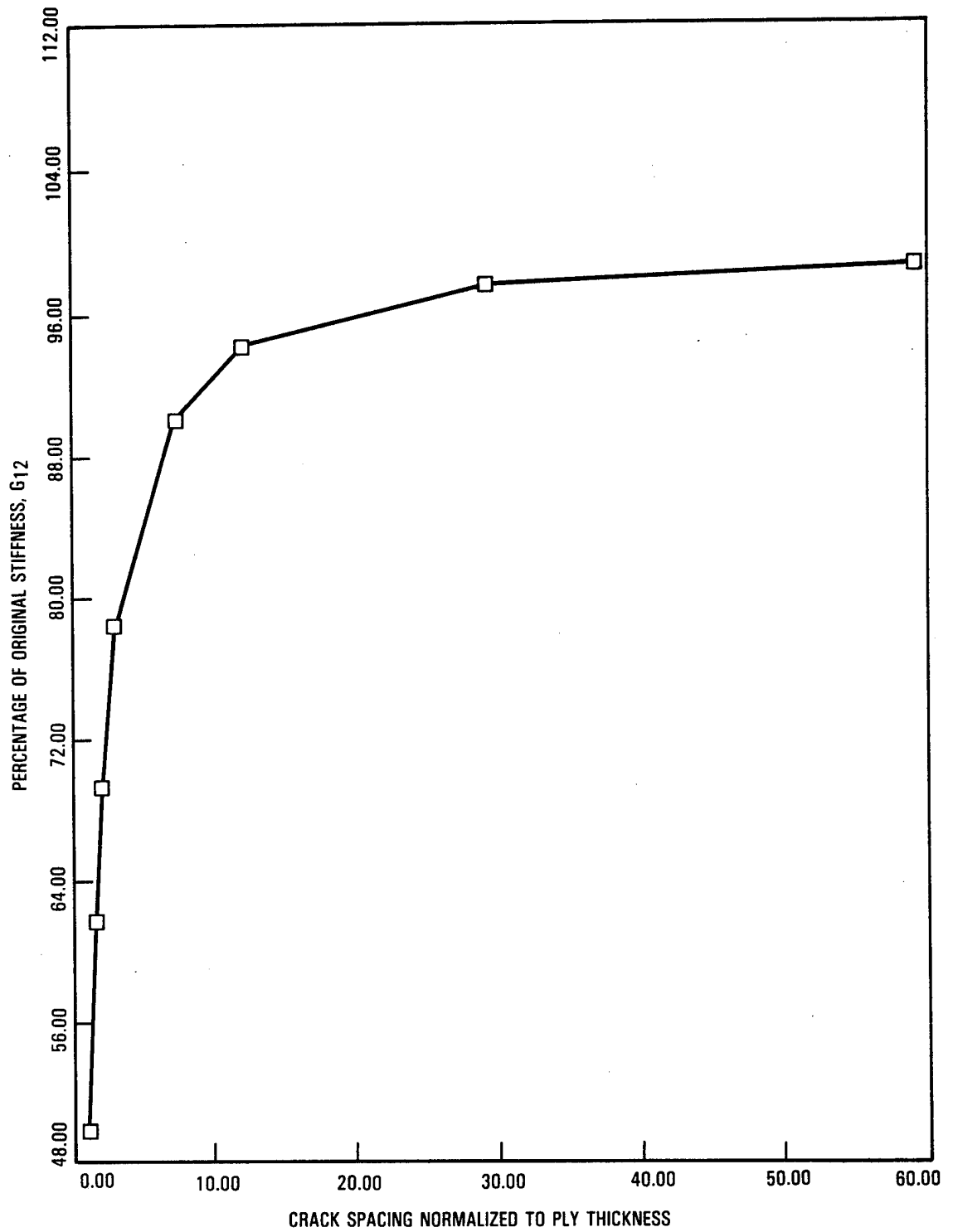
Figure 61: Effective modulus G_{12} for a (0/90)_s laminate.
