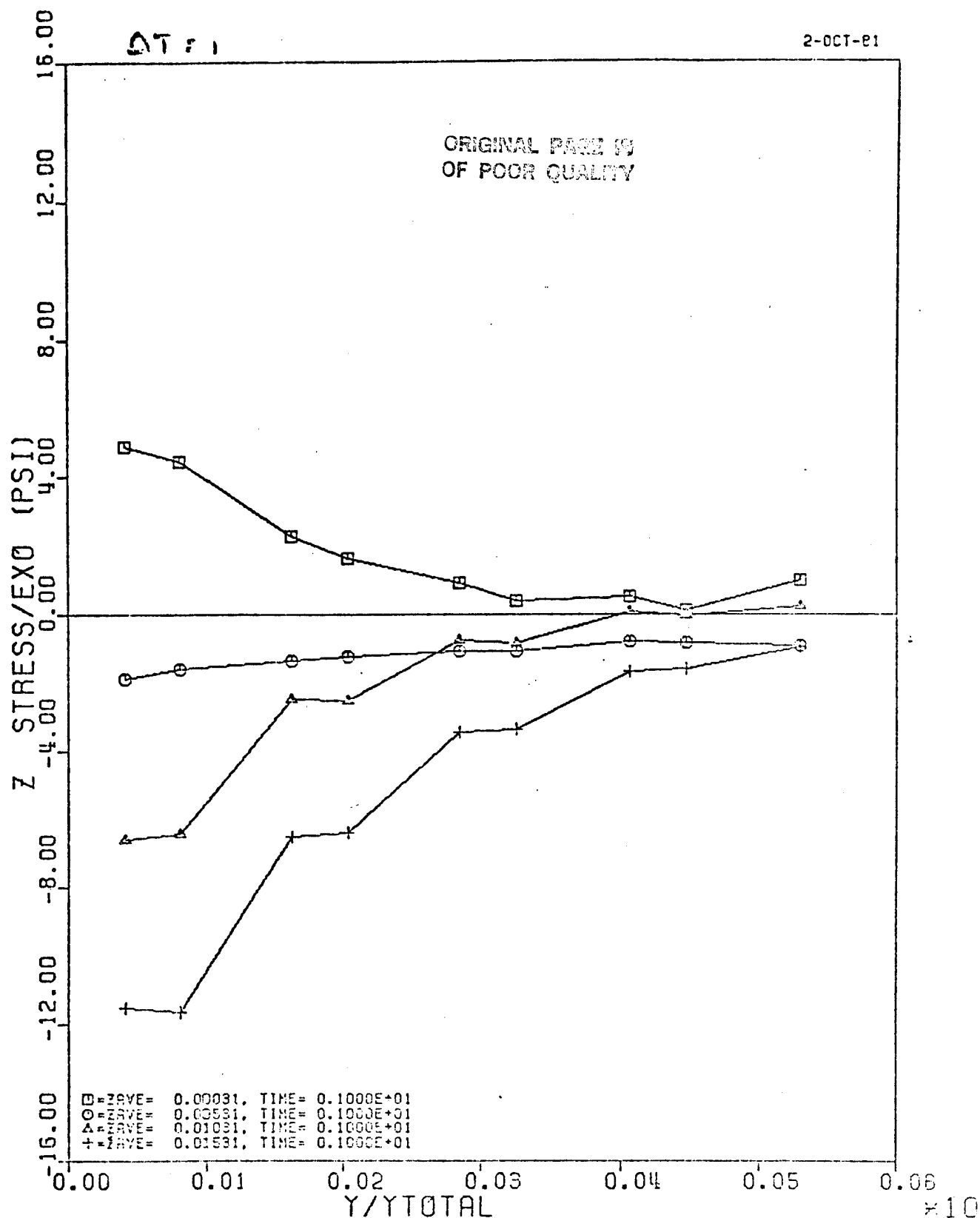
Figure D28: \sigma_z Free Edge Stress for (0/90/+45) s Laminate as a Function of y , Uniform Temperature Change, 0.5°C (10°F).
