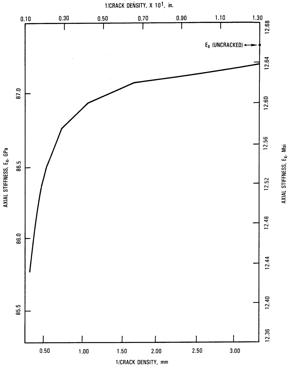
FIGURE 56 (0/90) 5 LAMINATE STIFFNESS VS CRACK DENSITY ( E_x VS \rho^{-1} )
