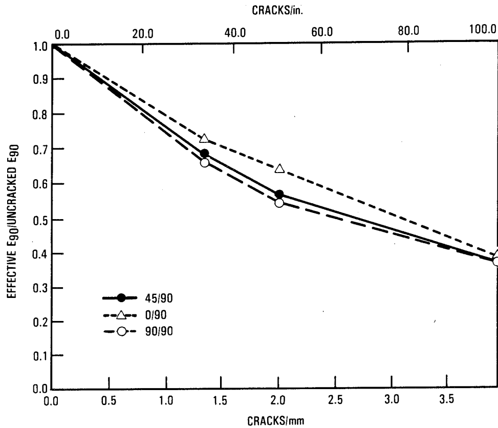
FIGURE 66 . NORMALIZED EFFECTIVE TRANSVERSE MODULUS VERSUS CRACK SPACING.
