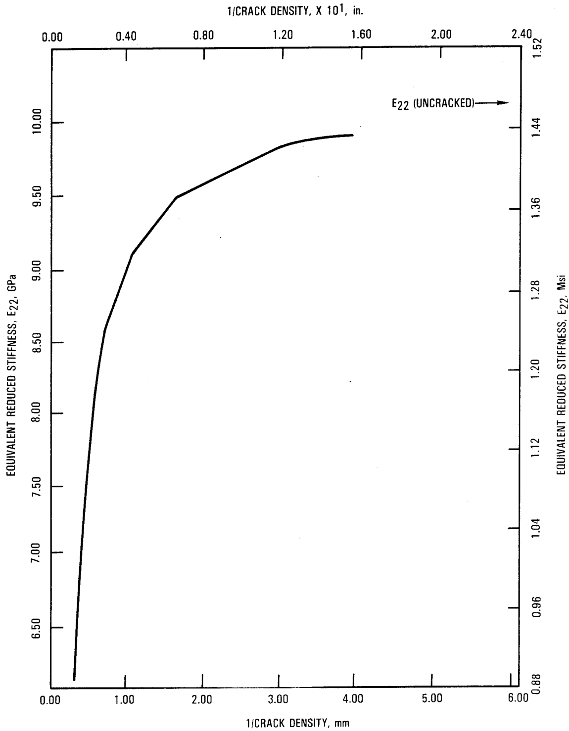
FIGURE 58. EQUIVALENT STIFFNESS VS CRACK DENSITY E_{22}^{EQUIV} VS P-1)
