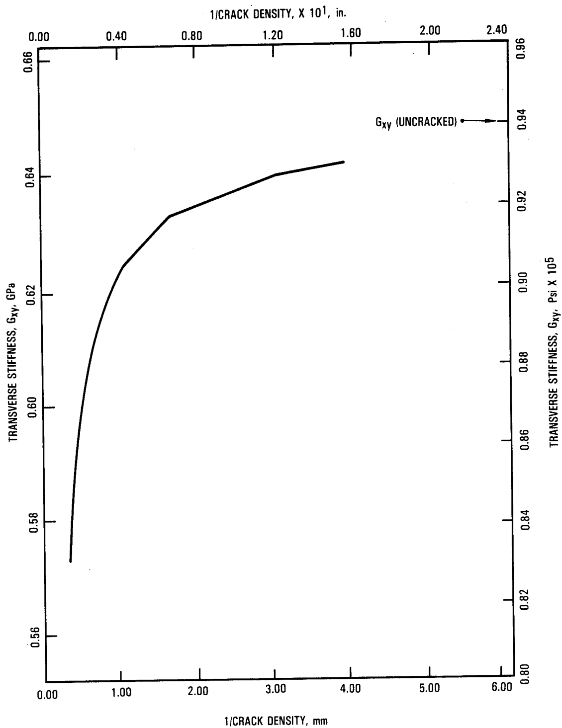
FIGURE 57. (0/90)_s SHEAR STIFFNESS VS CRACK DENSITY ( G_{xy} VS p^{-1} )
