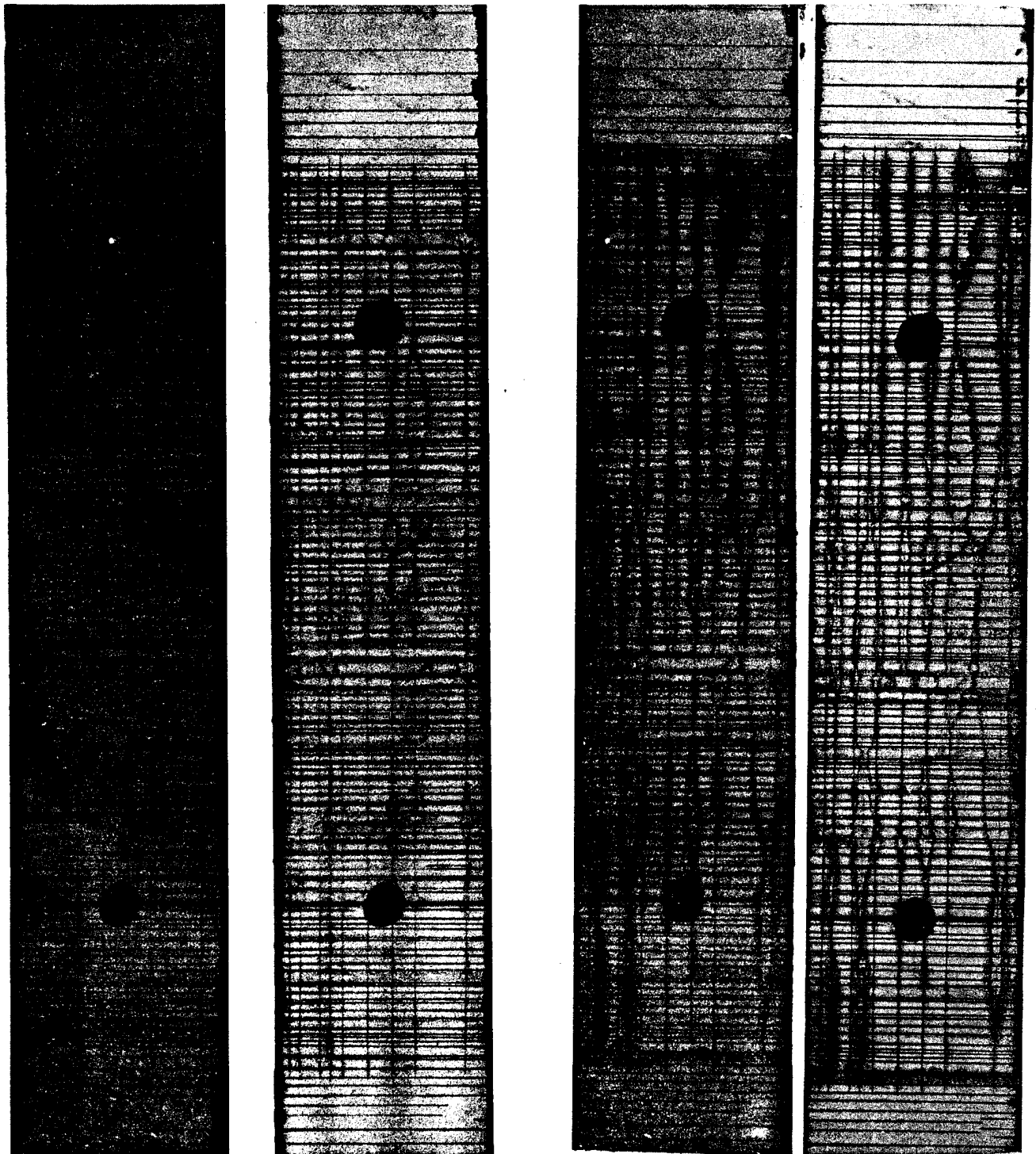
100 000 300 000 600 000 1 000 000 Figure 40: Enhanced x-ray photographs of coupon A22 showing 90° matrix cracking, 0° splits, and delamination; Initial \epsilon = 0.005 .
