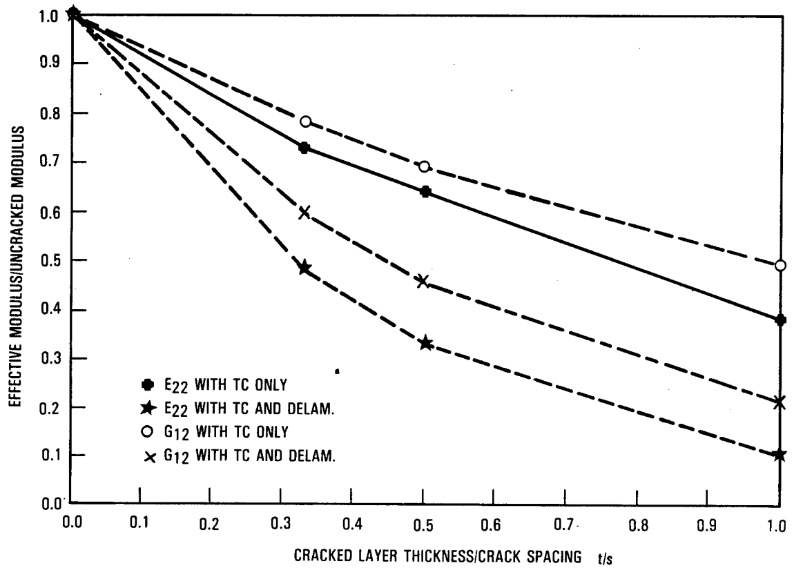
FIGURE 70. NORMALIZED EFFECTIVE MODULUS VERSUS CRACK DENSITY
