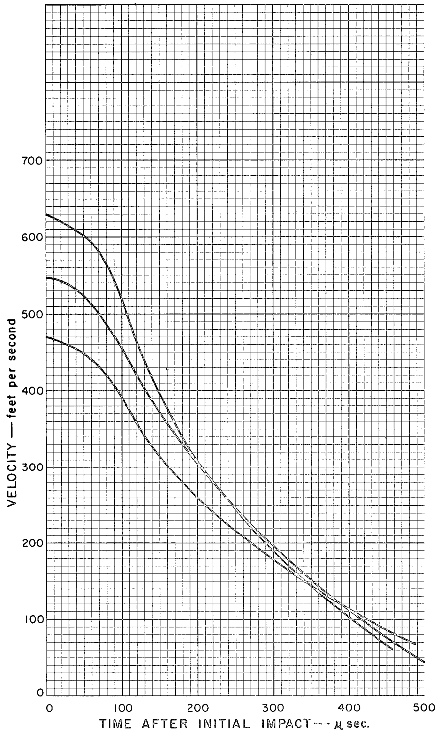
Figure 30. Projectile Velocity as a Function of Time after Initial Impact. Experimental Results for Tests 65-C, 66-C, and 68-C. Material - 19 ounces per square yard Nylon Felt.
