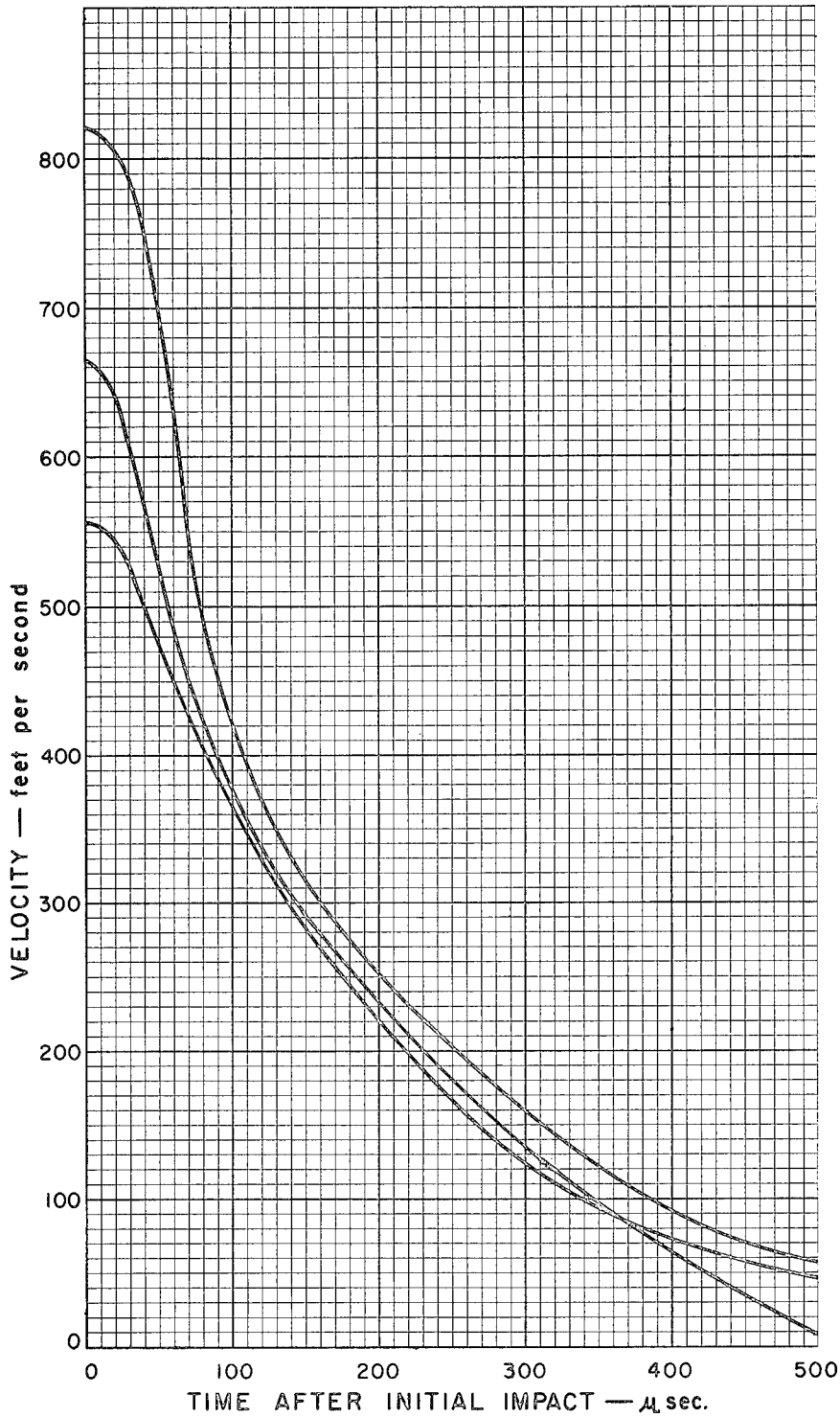
Figure 15. Projectile Velocity as a Function of Time after Initial Impact. Experimental Results for Tests 21-C, 24-C, and 25-C. Material - 40 ounces per square yard Polypropylene Felt.
