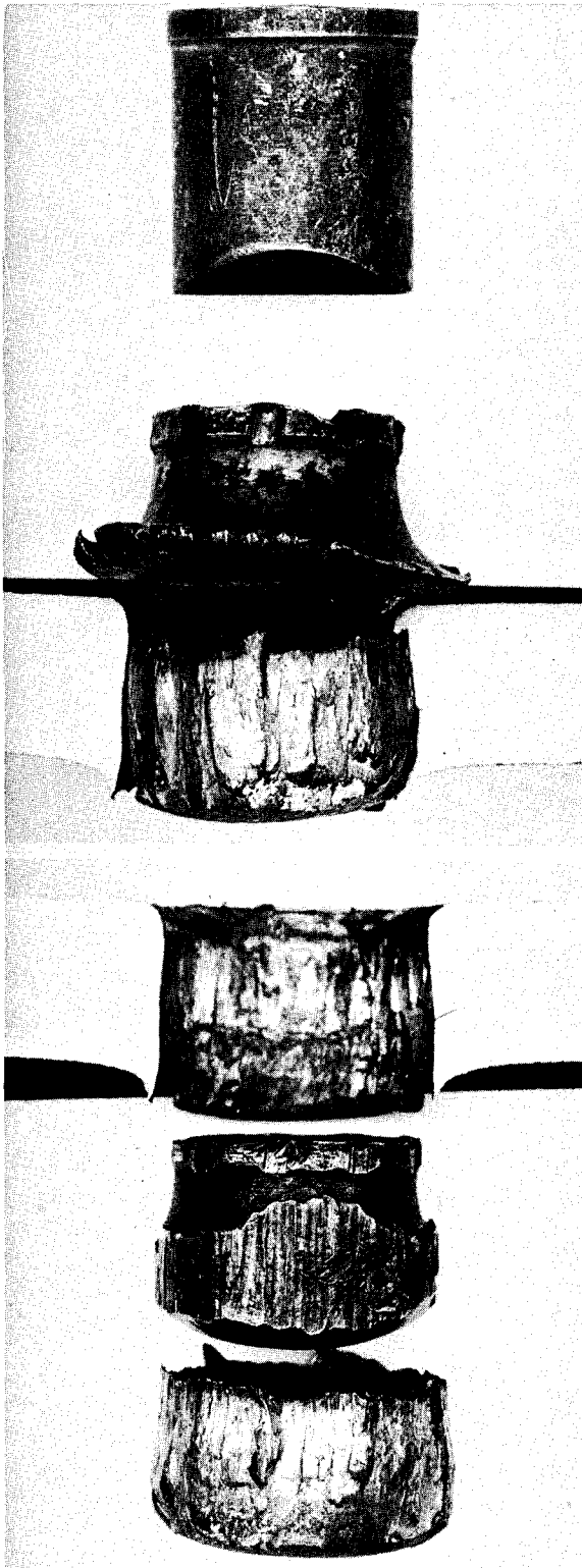
Figure 1. Rigid Plate Perforation by Blunt Fragments
