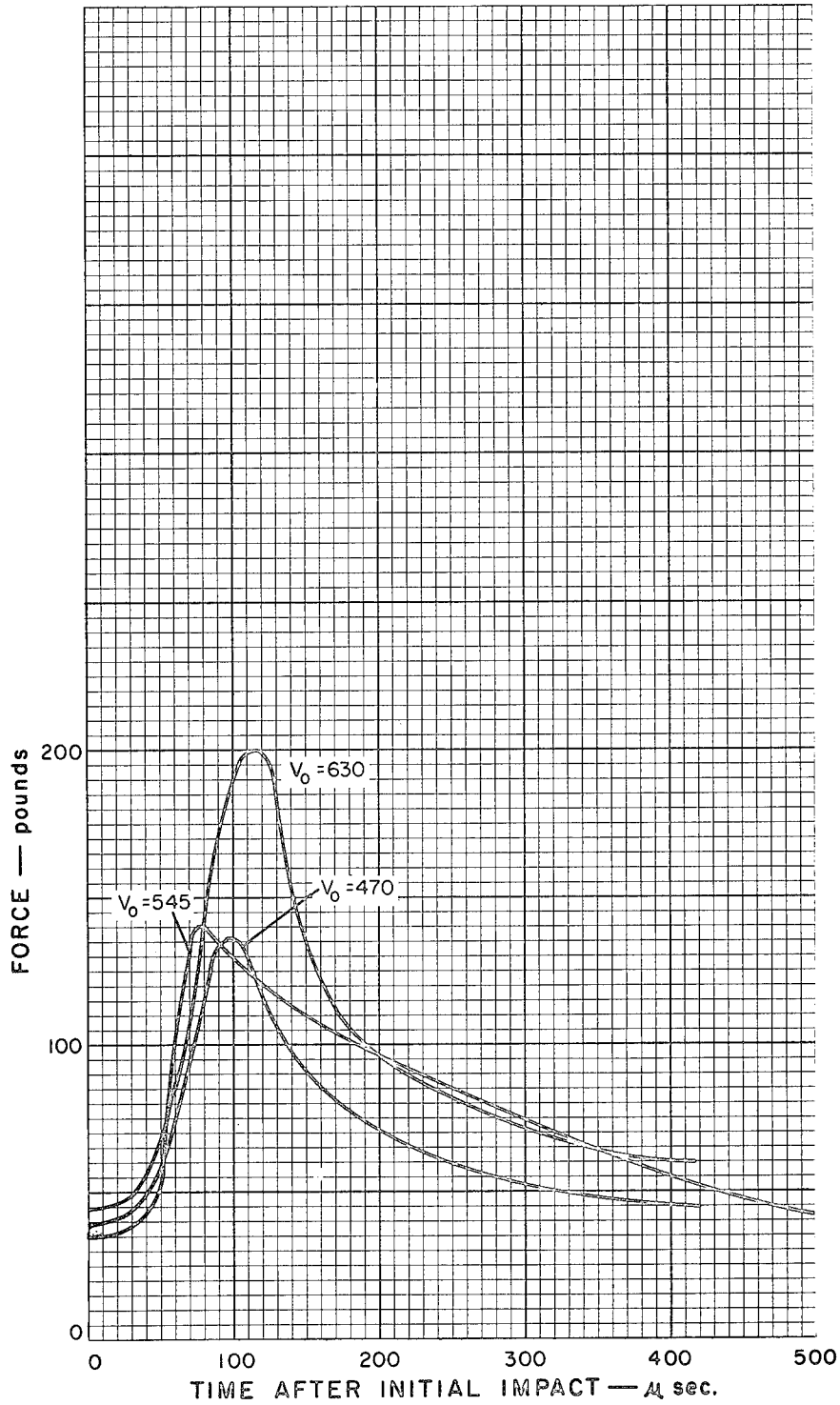
Figure 31. Force Opposing Projectile Motion as a Function of Time after Initial Impact. Experimental Results for Tests 65-C, 66-C, and 68-C. Material - 19 ounces per square yard Nylon Felt.
