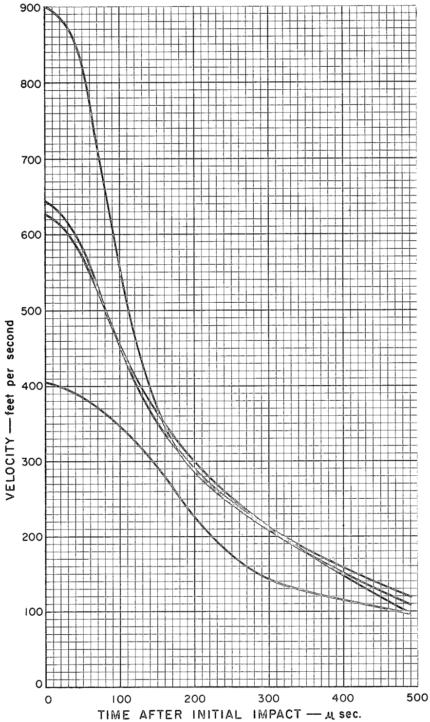
Figure 27. Projectile Velocity as a Function of Time after Initial Impact. Experimental Results for Tests 33-C, 36-C, 39-C, and 40-C. Material - 43 ounces per square yard Nylon Felt.
