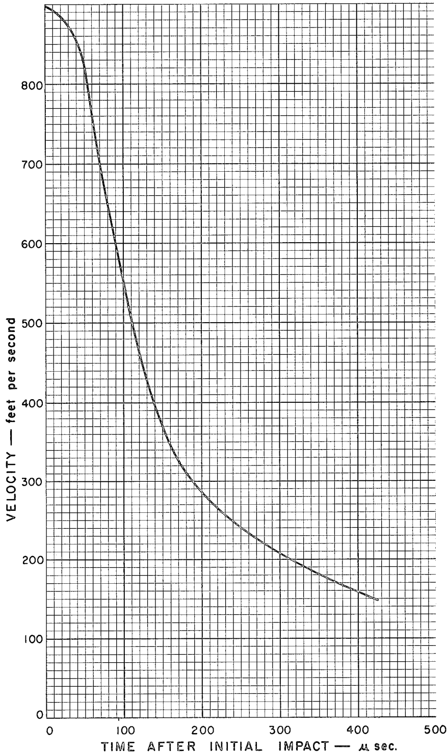
Figure 9. Projectile Velocity as a Function of Time after Initial Impact. Test No. 40-C, Impact Velocity - 900 feet per second. Material - 43 ounces per square yard Nylon Felt.
