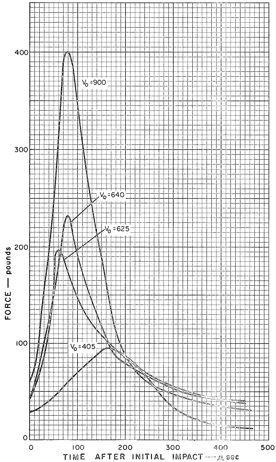
Figure 28. Force Opposing Projectile Motion as a Function of Time after Initial Impact. Experimental Results for Tests 33-C, 36-C, 39-C, and 40-C. Material - 43 ounces per square yard Nylon Felt.
