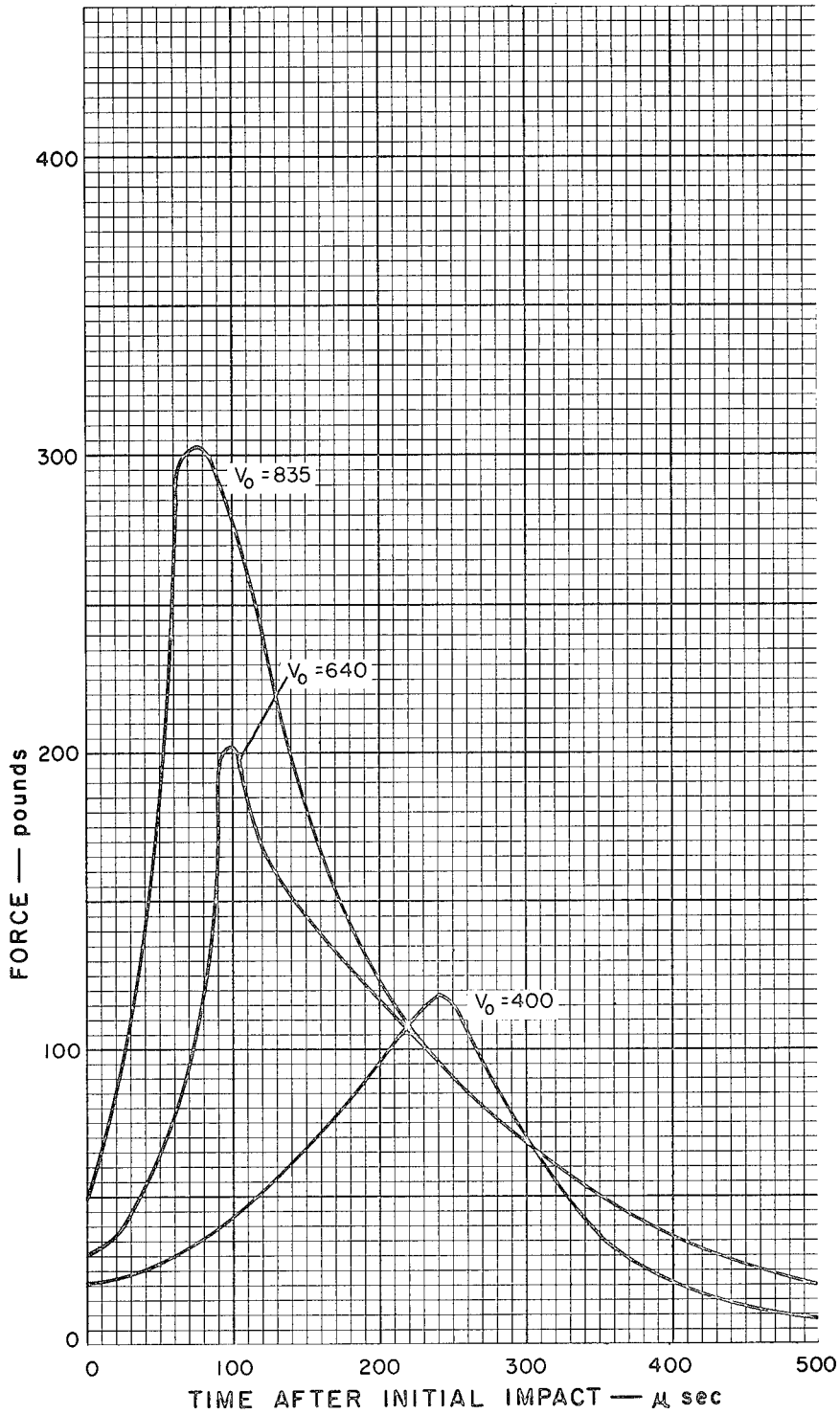
Figure 25. Force Opposing Projectile Motion as a Function of Time after Initial Impact. Experimental Results for Tests 7-C, 15-C, and 19-C. Material - 53 ounces per square yard Nylon Felt.
