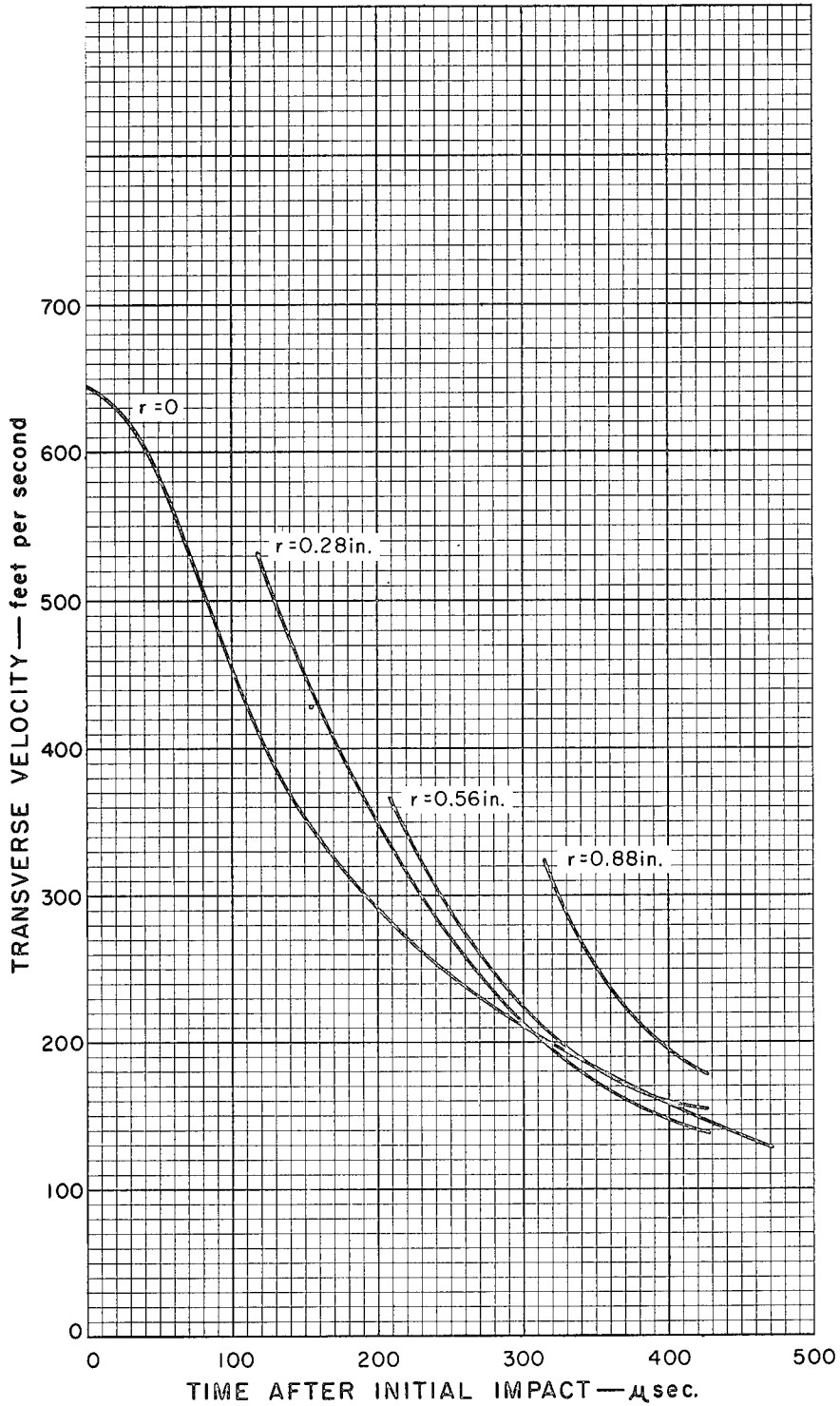
Figure 36. Transverse Velocity of Felt Material at Several Radii as a Function of Time after Initial Impact. Test No. 33-C. Material - 43 ounces per square yard Nylon Felt.
