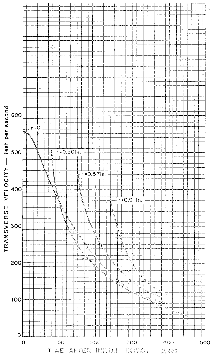
Figure 33. Transverse Velocity of Felt Material at Several Radii as a Function of Time after Initial Impact. Test No. 24-C. Material - 40 ounces per square yard Polypropylene Felt.
