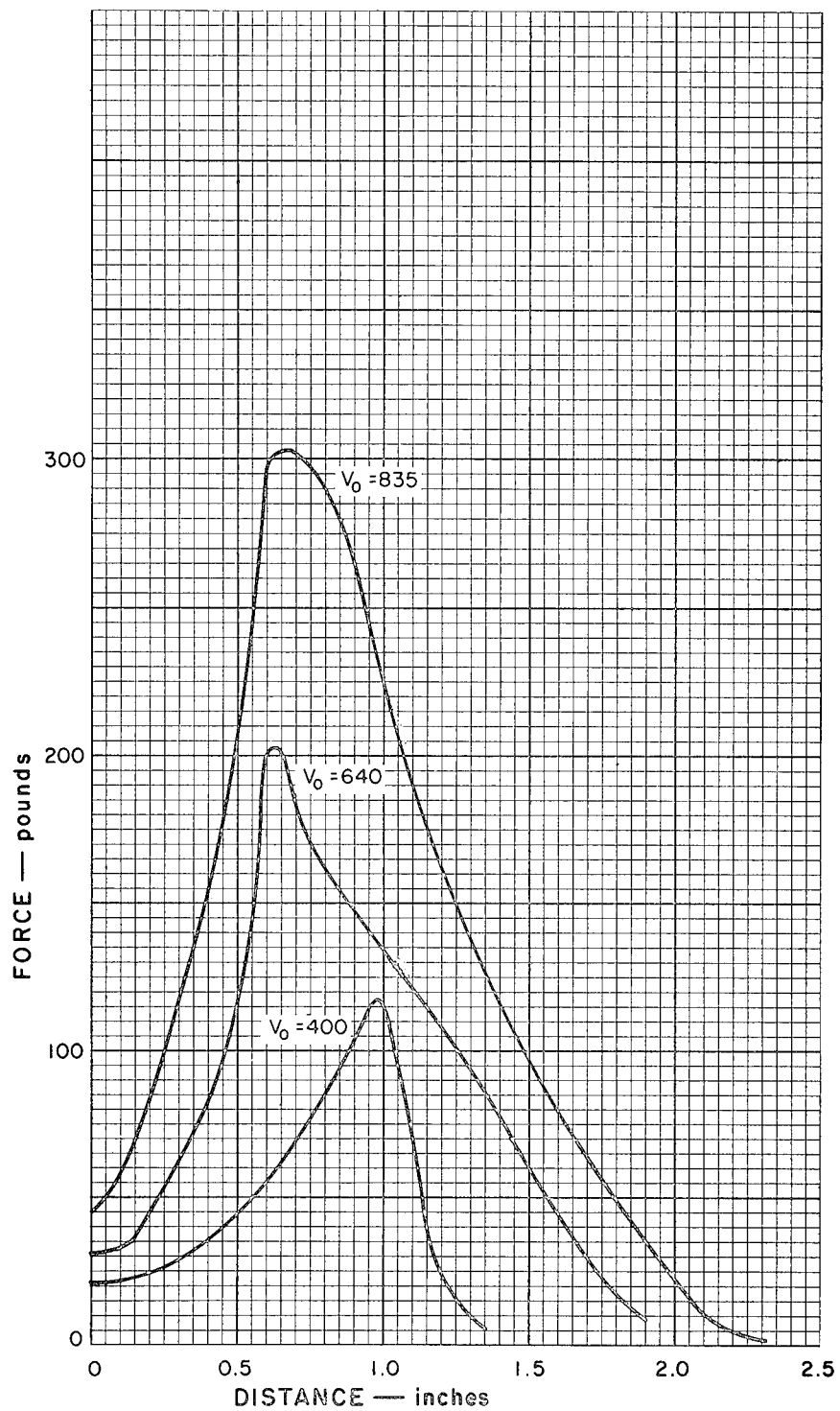
Figure 26. Force Opposing Projectile Motion as a Function of Distance Traveled. Experimental Results for Tests 7-C, 15-C, and 19-C. Material - 53 ounces per square yard Nylon Felt.
