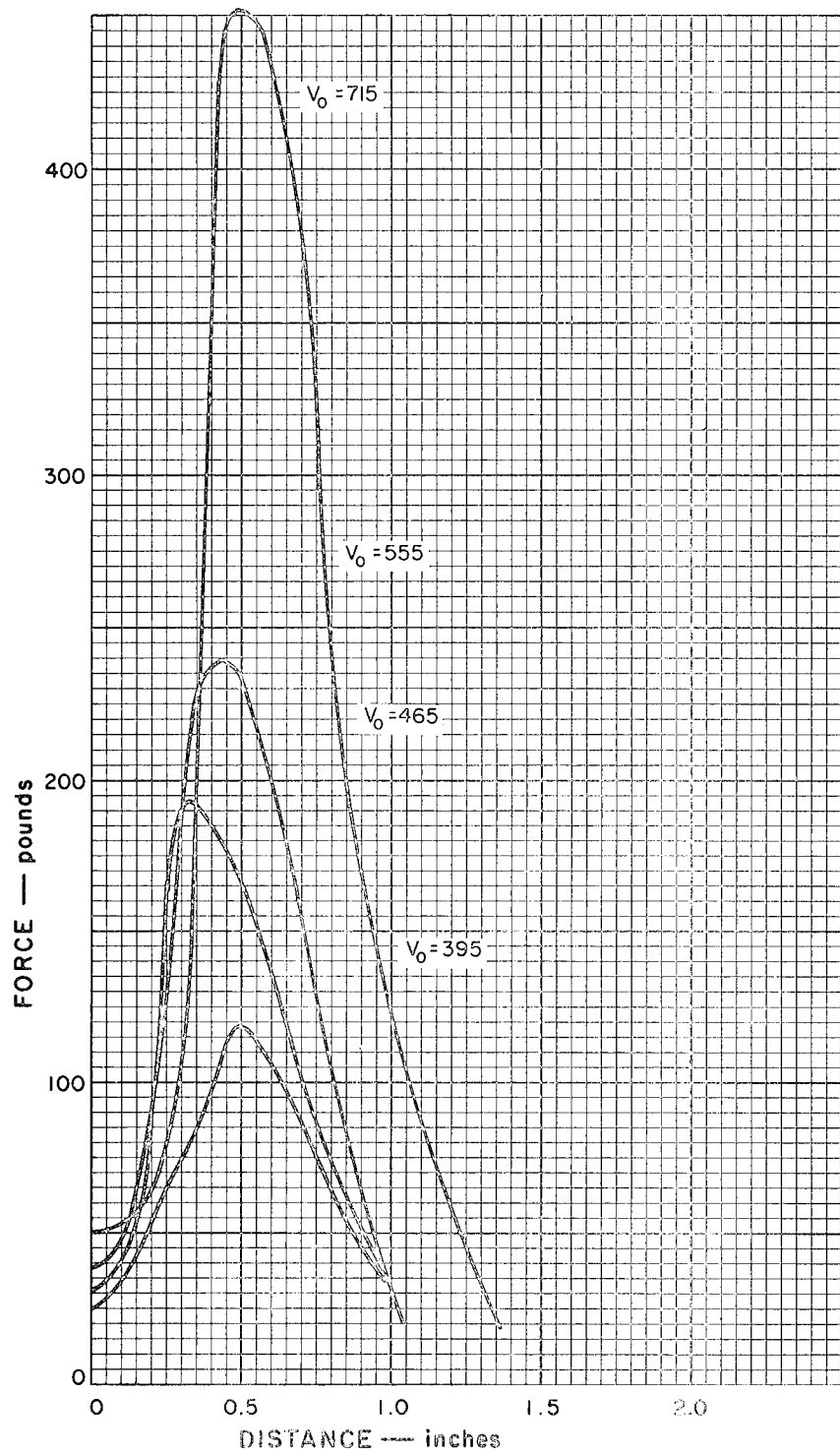
Figure 20. Force Opposing Projectile Motion as a Function of Distance Traveled. Experimental Results for Tests 42-C, 43-C, 44-C, and 49-C. Material - 42 ounces per square yard Dacron Felt.
