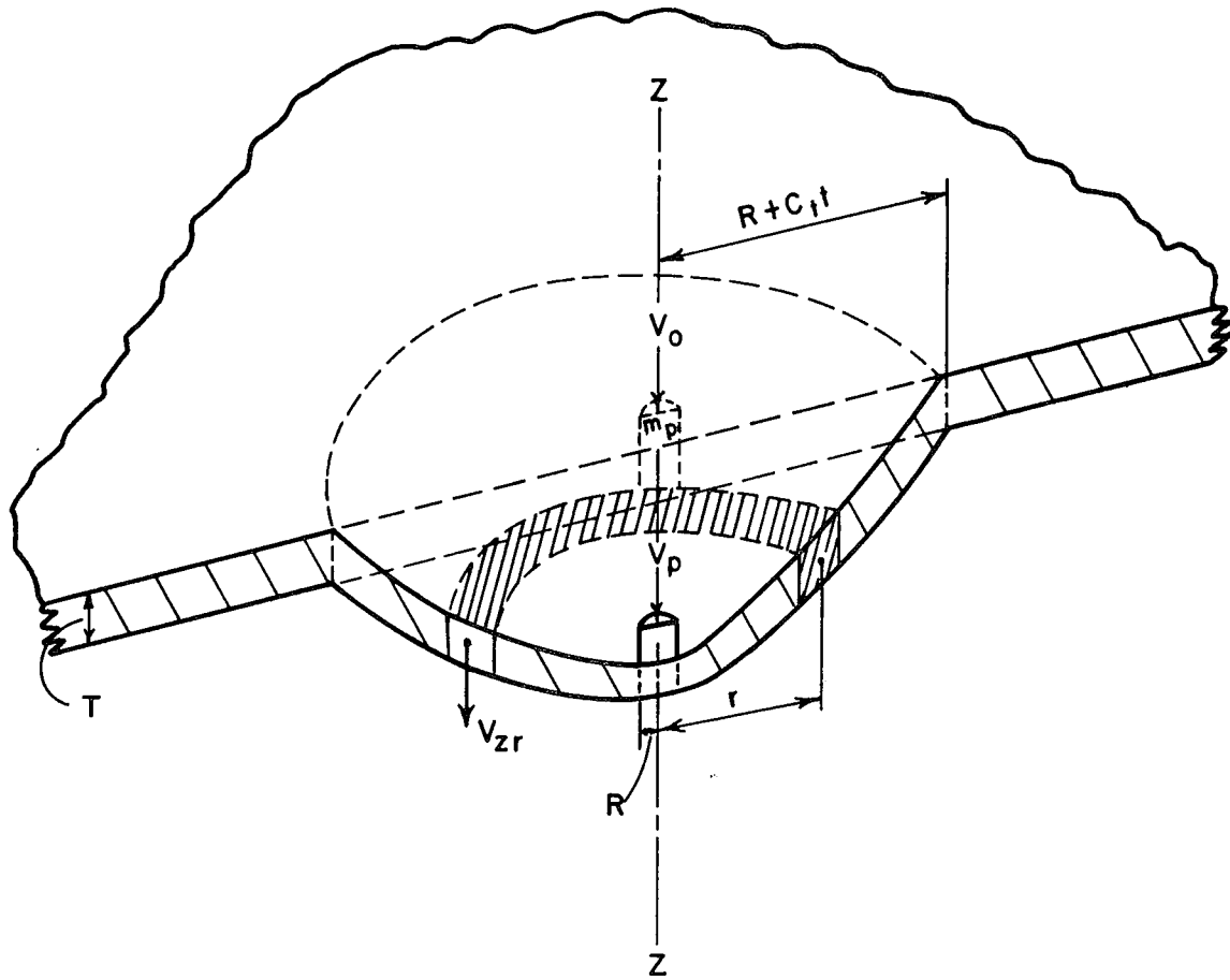
Figure 40. Transverse Impact of a Cylindrical Projectile and a Sheet of Felt Material
