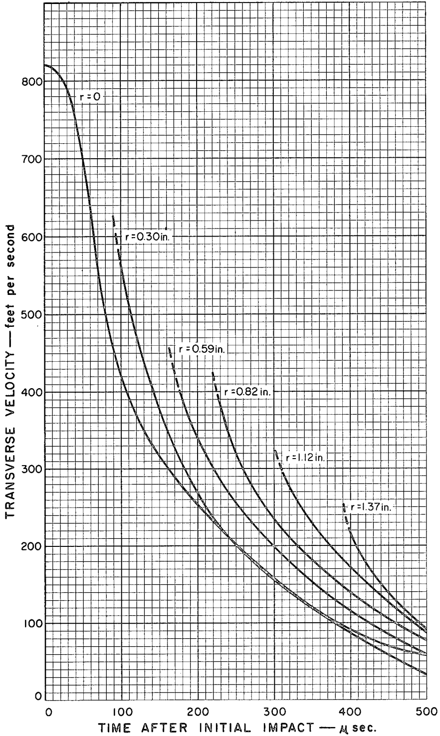
Figure 34. Transverse Velocity of Felt Material at Several Radii as a Function of Time after Initial Impact. Test No. 25-C. Material - 40 ounces per square yard Polypropylene Felt.
