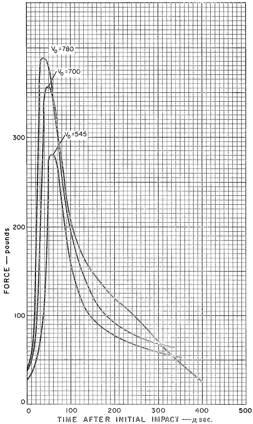
Figure 22. Force Opposing Projectile Motion as a Function of Time after Initial Impact. Experimental Results for Tests 58-C, 59-C, and 62-C. Material - 43 ounces per square yard Orlon Felt.
