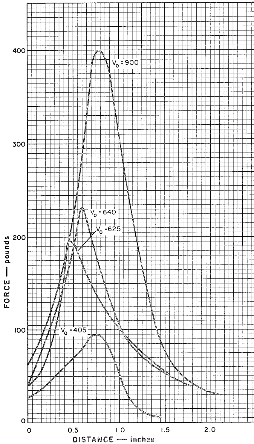
Figure 29. Force Opposing Projectile Motion as a Function of Distance Traveled. Experimental Results for Tests 33-C, 36-C, 39-C, and 40-C. Material - 43 ounces per square yard Nylon Felt.
