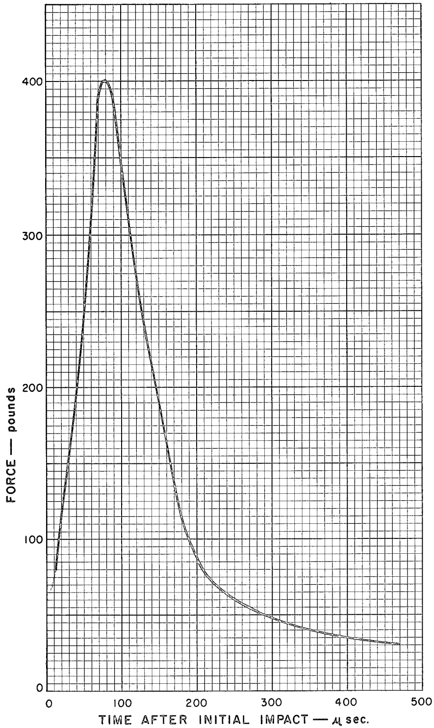
Figure 10. Force Opposing Projectile Motion as a Function of Time after Initial Impact. Test No. 40-C, Impact Velocity - 900 feet per second. Material - 43 ounces per square yard Nylon Felt.
