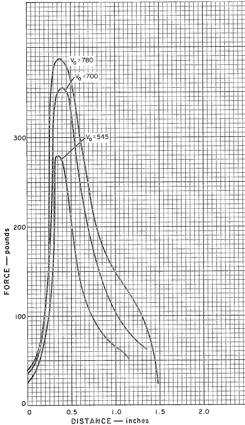
Figure 23. Force Opposing Projectile Motion as a Function of Distance Traveled. Experimental Results for Tests 58-C, 59-C, and 62-C. Material - 43 ounces per square yard Orlon Felt.
