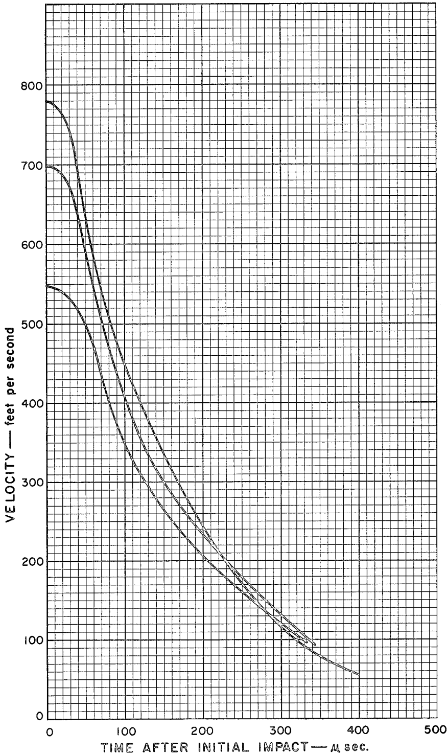
Figure 21. Projectile Velocity as a Function of Time after Initial Impact. Experimental Results for Tests 58-C, 59-C, and 62-C. Material - 43 ounces per square yard Orlon Felt.
