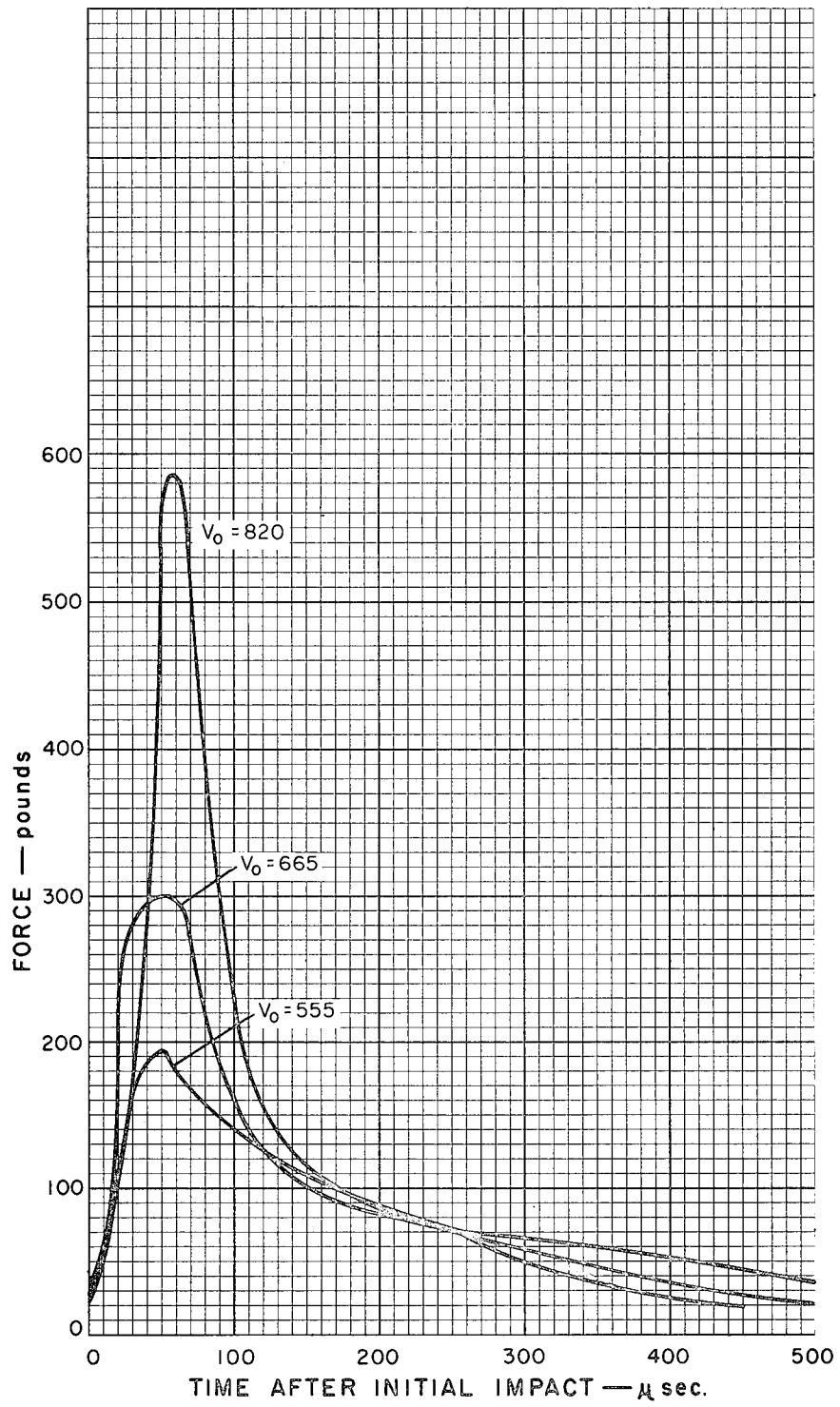
Figure 16. Force Opposing Projectile Motion as a Function of Time after Initial Impact. Experimental Results for Tests 21-C, 24-C, and 25-C. Material - 40 ounces per square yard Polypropylene Felt.
