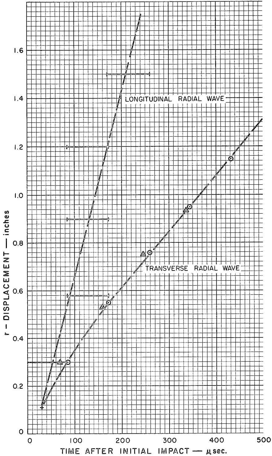
Figure 14. Relationship Between Radial Displacement and Time of Arrival for the Longitudinal and Transverse Radial Wave Fronts. Test No. 40-C, Impact Velocity - 900 feet per second. Material - 43 ounces per square yard Nylon Felt.
