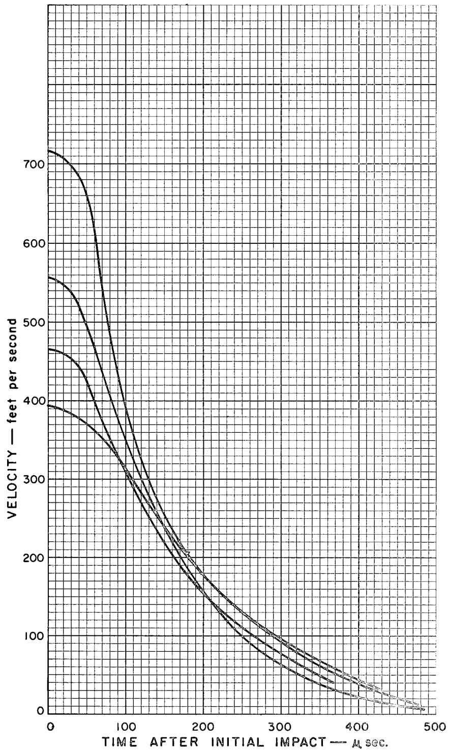
Figure 18. Projectile Velocity as a Function of Time after Initial Impact. Experimental Results for Tests 42-C, 43-C, 44-C, and 49-C. Material - 42 ounces per square yard Dacron Felt.
