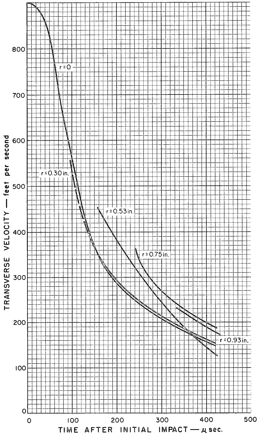
Figure 13. Transverse Velocity of Felt Material at Several Radii as a Function of Time after Initial Impact. Test No. 40-C, Impact Velocity - 900 feet per second. Material - 43 ounces per square yard Nylon Felt. ( r - Position of Station at Time of Arrival of Transverse Wave)
