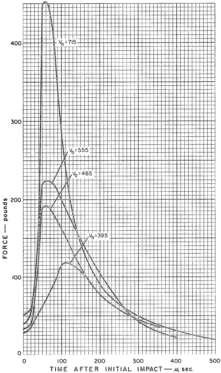
Figure 19. Force Opposing Projectile Motion as a Function of Time after Initial Impact. Experimental Results for Tests 42-C, 43-C, 44-C, and 49-C. Material - 42 ounces per square yard Dacron Felt.
