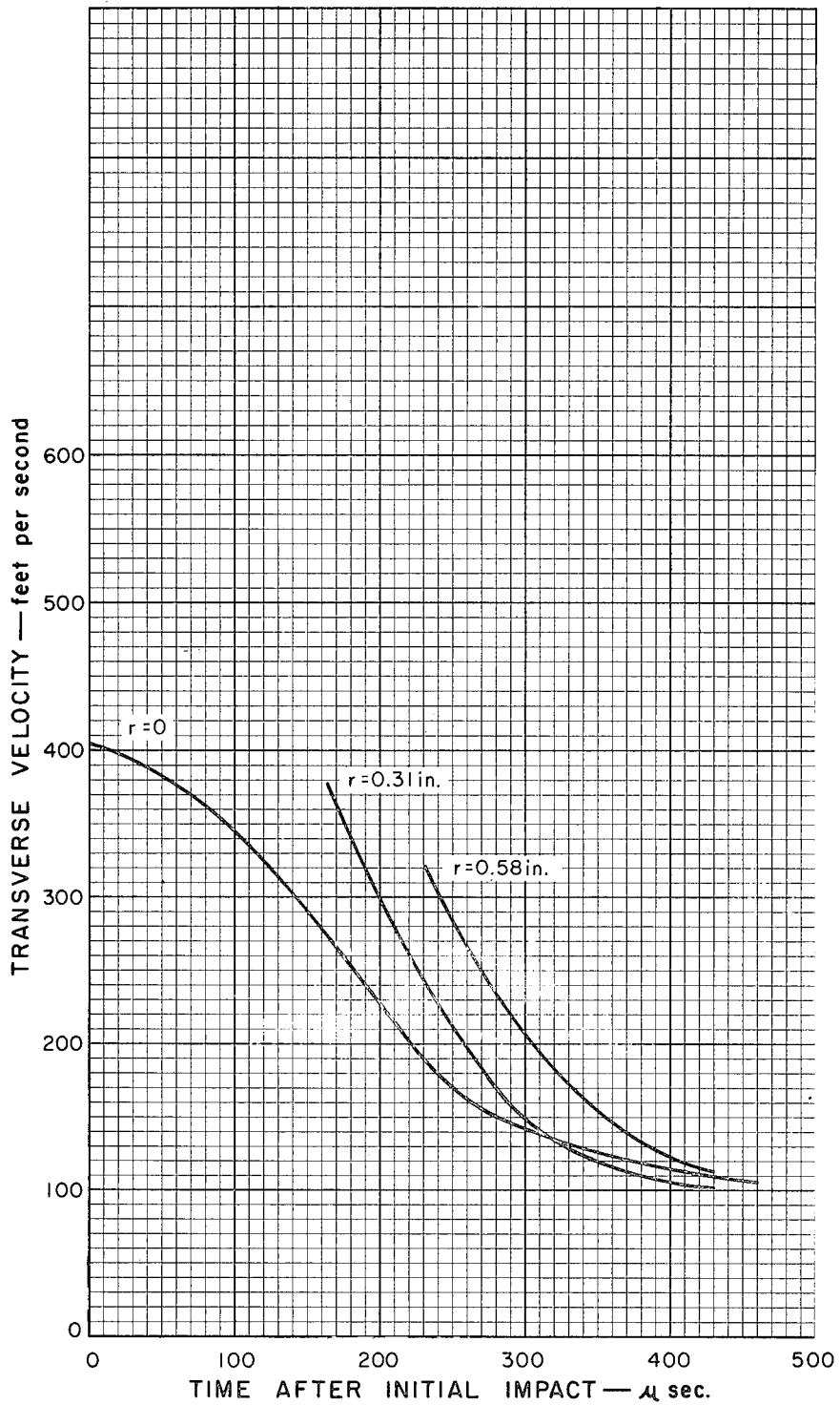
Figure 35. Transverse Velocity of Felt Material at Several Radii as a Function of Time after Initial Impact. Test No. 39-C. Material - 43 ounces per square yard Nylon Felt.
