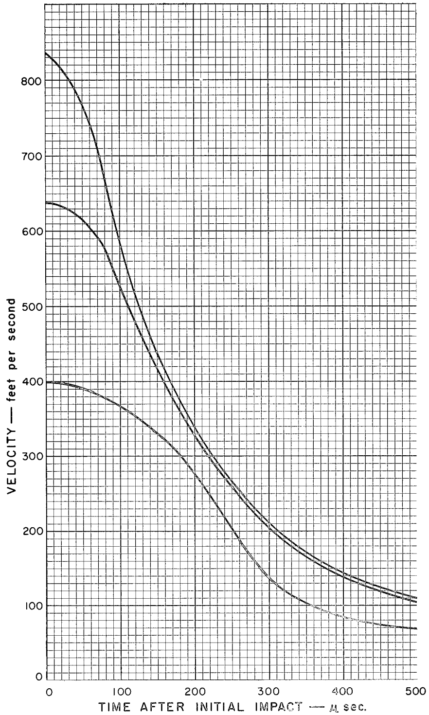
Figure 24. Projectile Velocity as a Function of Time after Initial Impact. Experimental Results for Tests 7-C, 15-C, and 19-C. Material - 53 ounces per square yard Nylon Felt.
