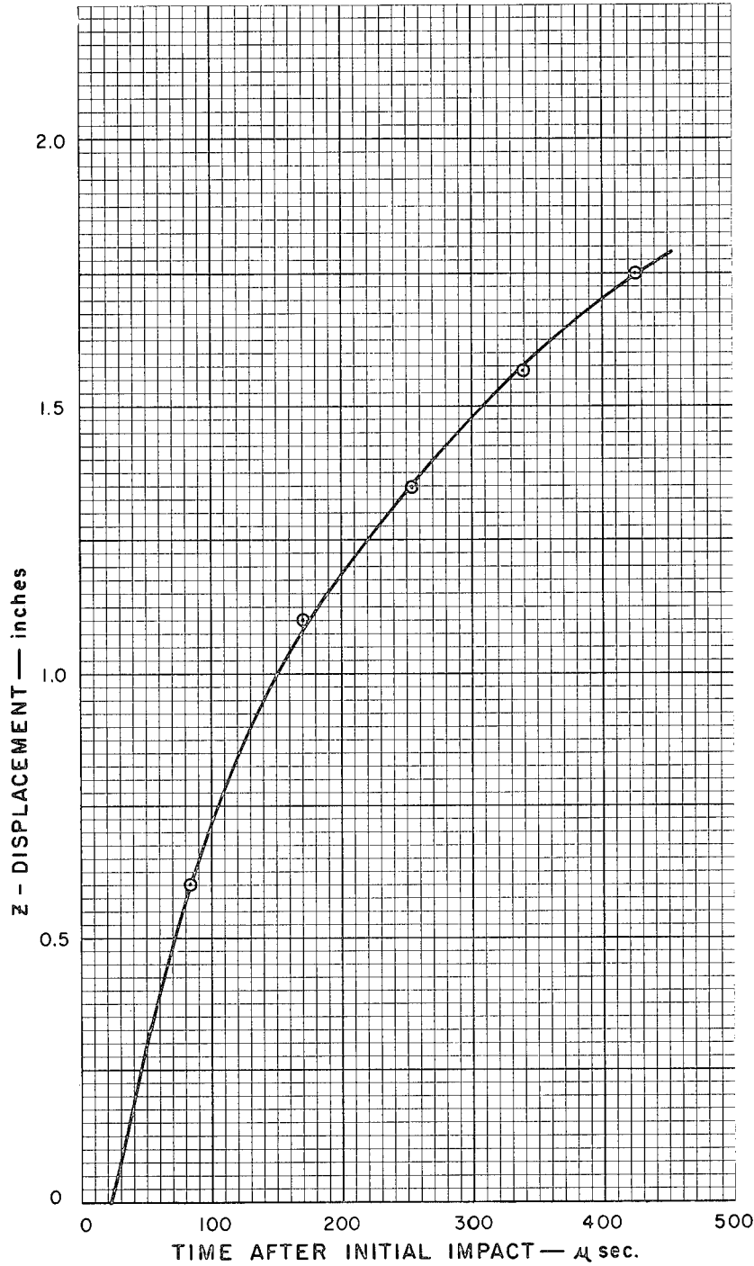
Figure 8. Axial Displacement of the Center Arc-Gap as a Function of Time after Initial Impact of the Projectile with the Front Surface of the Felt. Test No. 40-C, Impact Velocity - 900 feet per second. Material - 43 ounces per square yard Nylon Felt.
