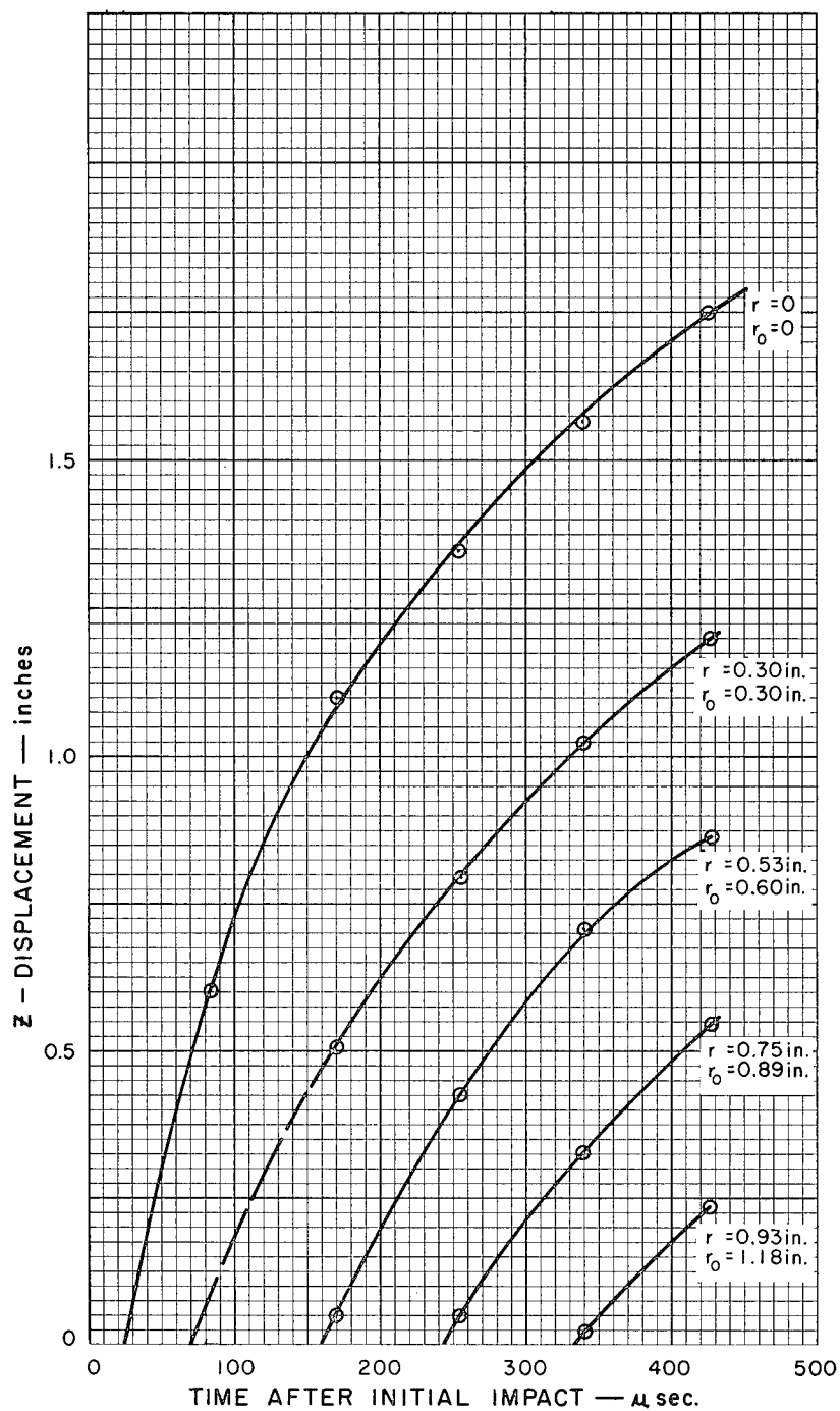
Figure 12. Transverse Displacement of Felt Material at Several Radii as a Function of Time after Initial Impact. Test No. 40-C, Impact Velocity - 900 feet per second. Material - 43 ounces per square yard Nylon Felt. ( r_0 - Initial Position of Station; r - Position of Station at Time of Arrival of Transverse Wave)
