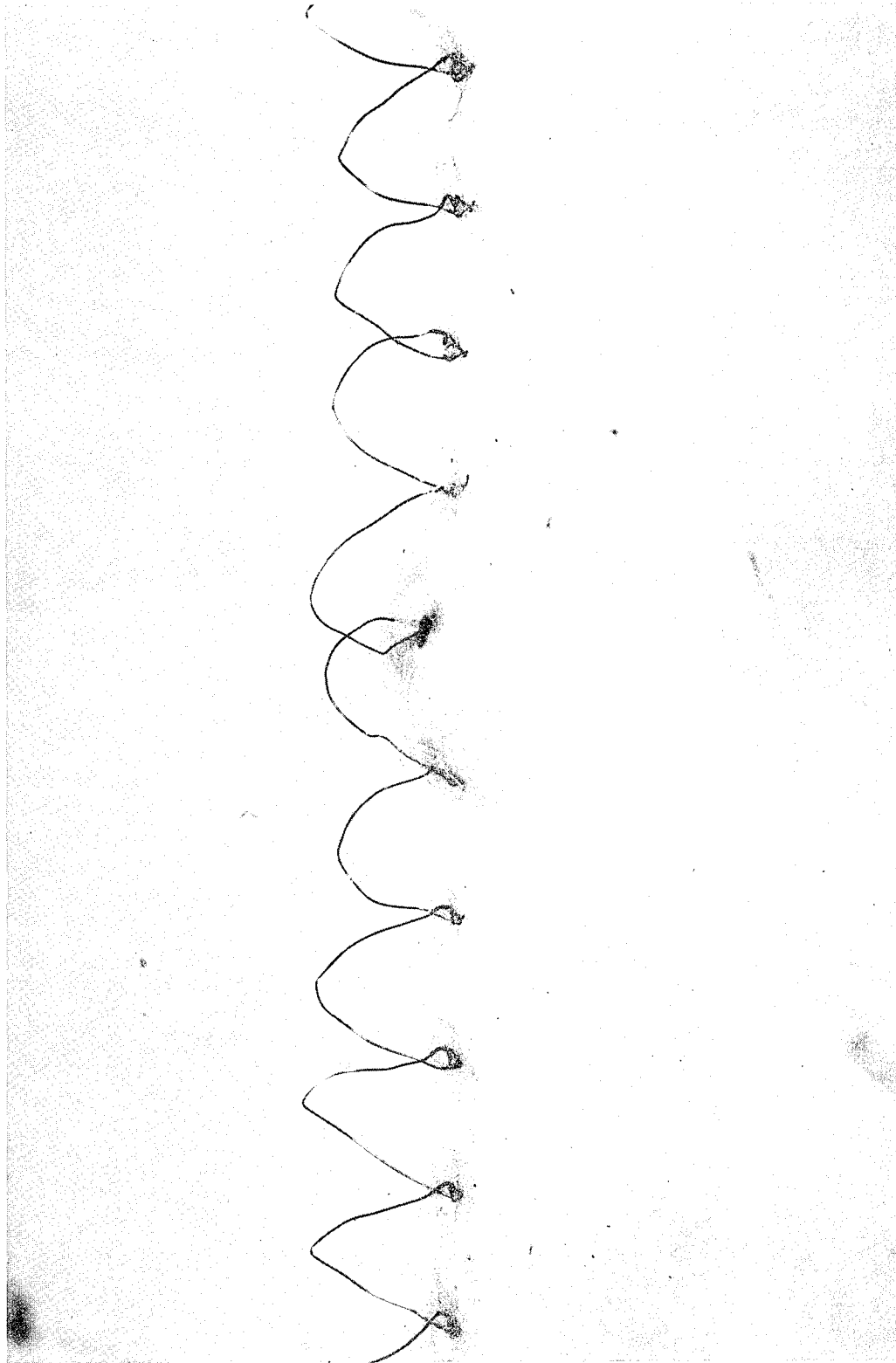
Figure 4. Attachment of Spark Gap Wire to Rear Surface of Nylon Felt Sample
