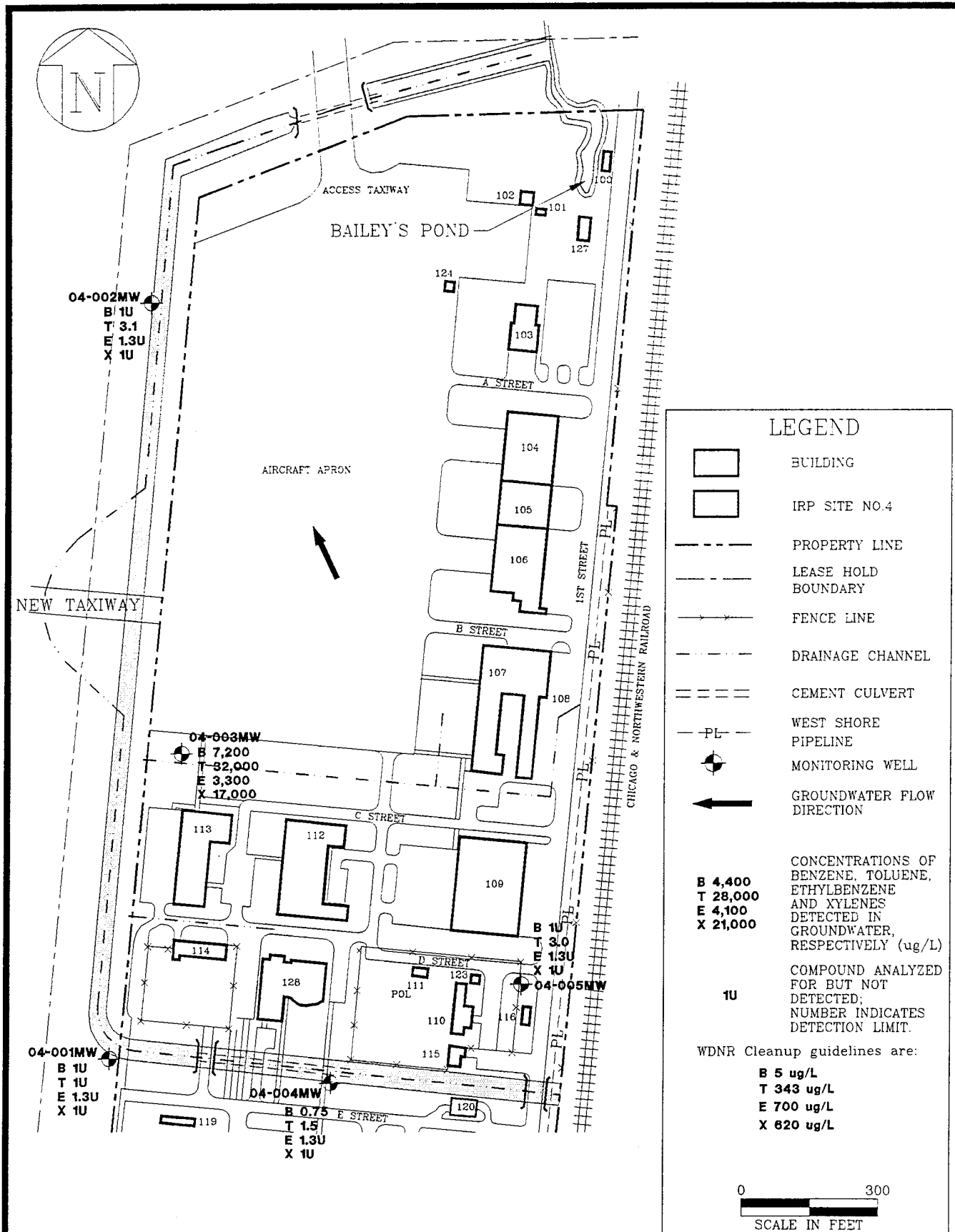
FIGURE 5.21 BENZENE, TOLUENE, ETHYLBENZENE, AND XYLENES DETECTED IN GROUND- WATER (FIRST ROUND SAMPLING) 128th ARW, Gen. Billy Mitchell Field ANGB Milwaukee, Wisconsin
