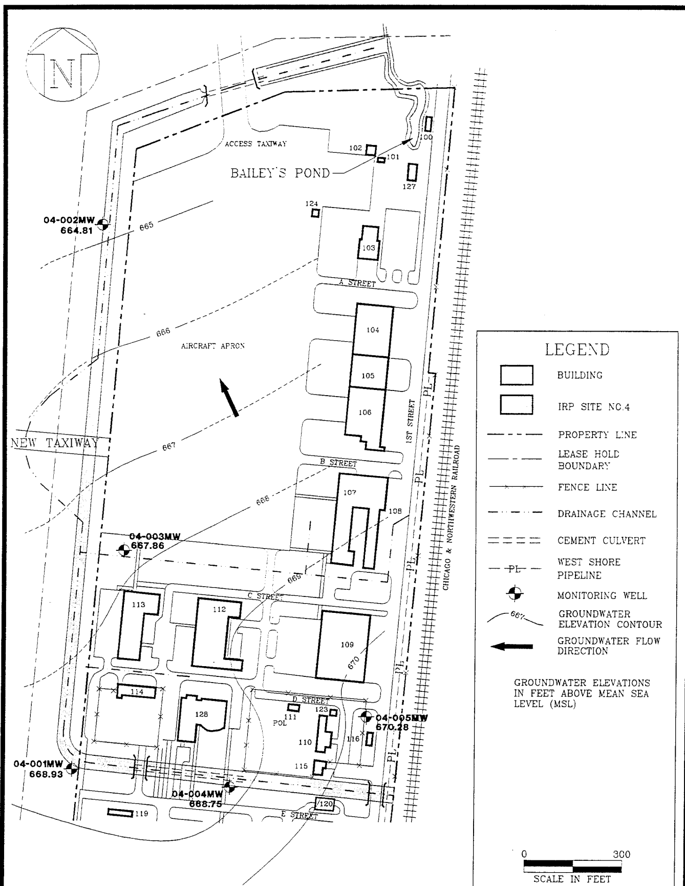
FIGURE 5.15 MONITORING WELL GROUNDWATER ELEVATIONS (MSL) 20 DECEMBER 1994
