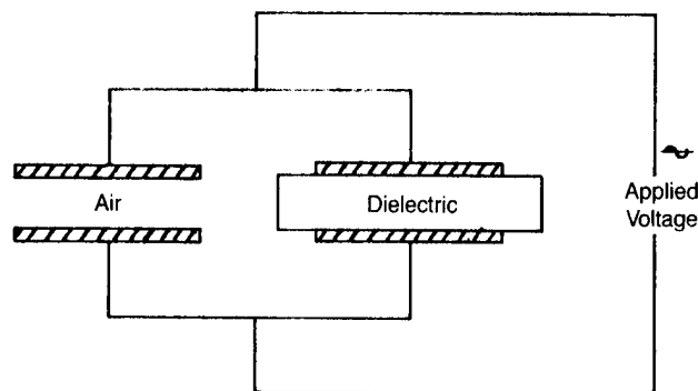
Figure 5-4. Permittivity (Dielectric Constant) Schematic
