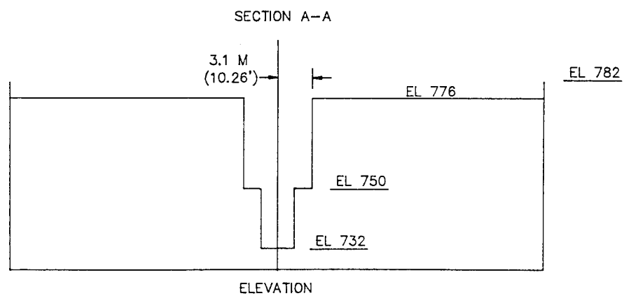
TYPE 19 WEIR DESIGN
