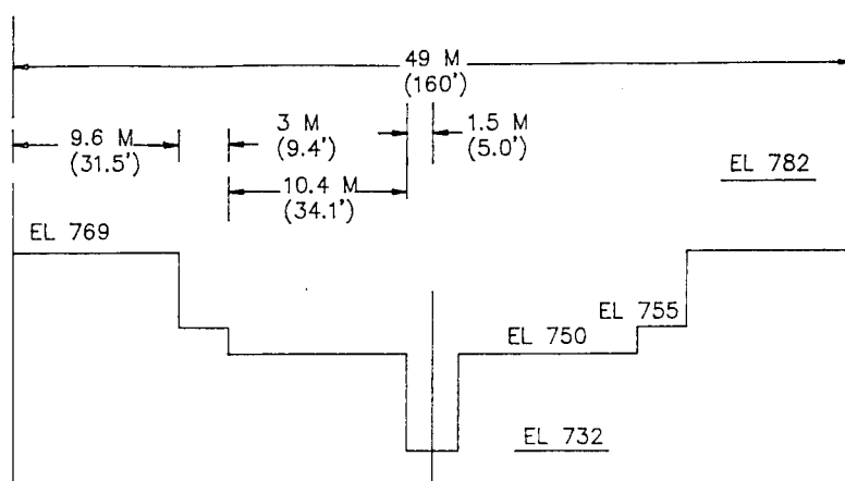
TYPE 8 WEIR - ELEVATION
