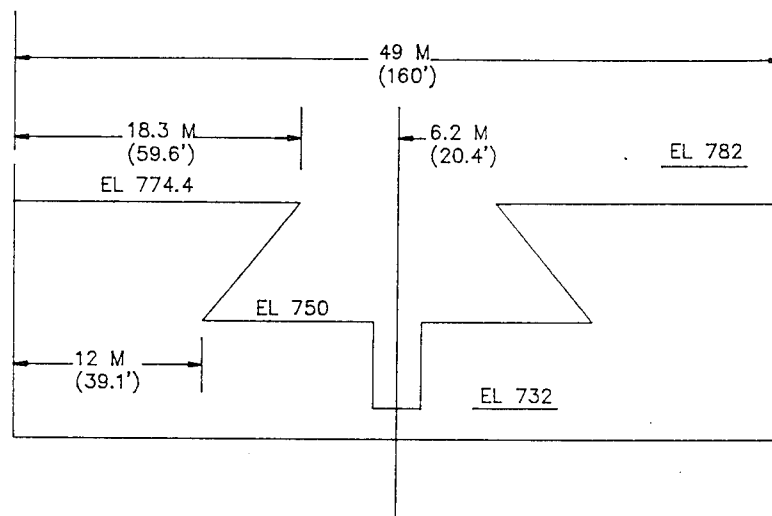
TYPE 14 WEIR - ELEVATION
