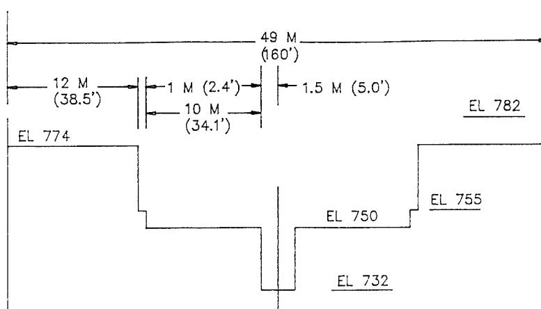
TYPE 11 WEIR - ELEVATION
