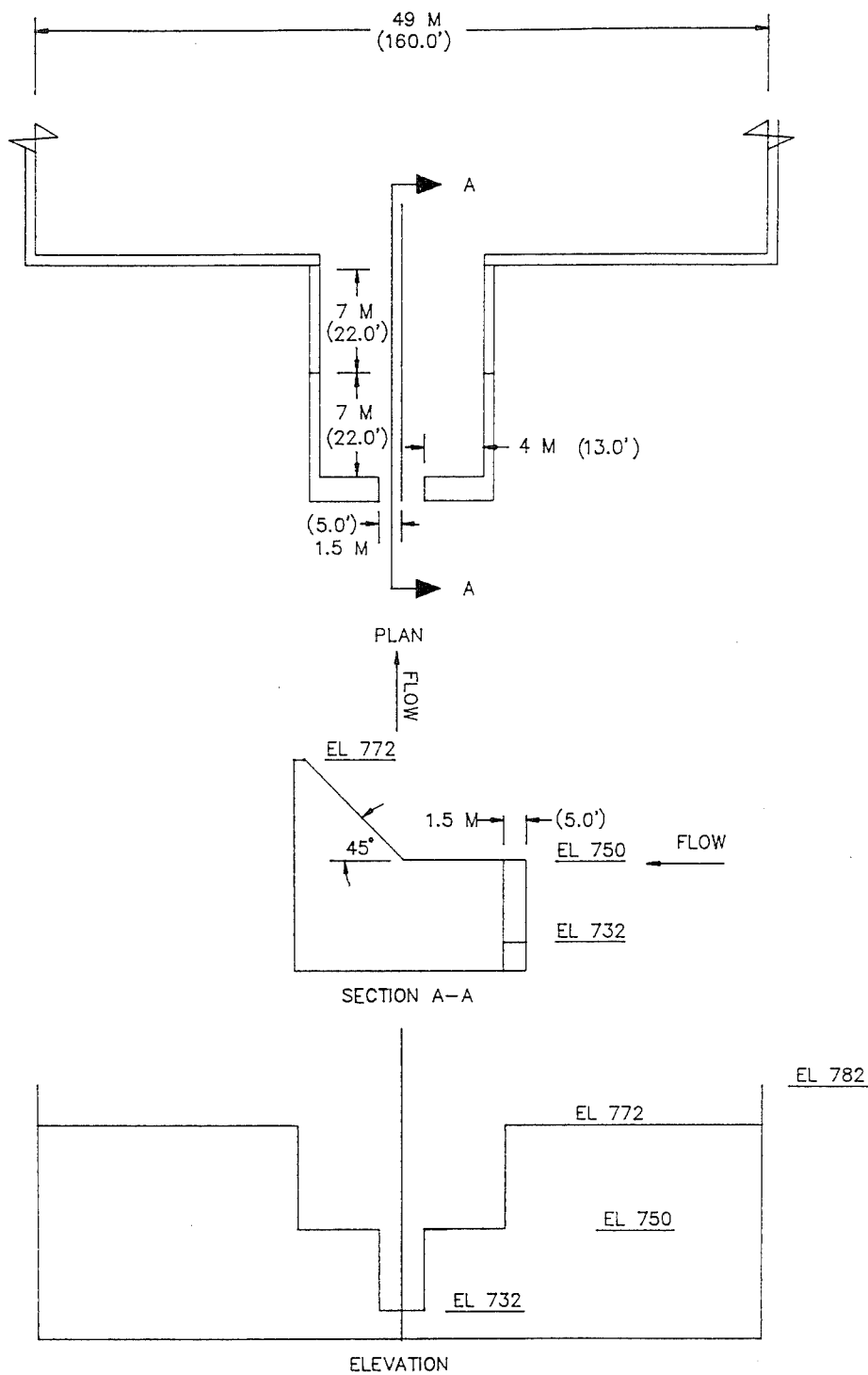
TYPE 20 WEIR DESIGN
