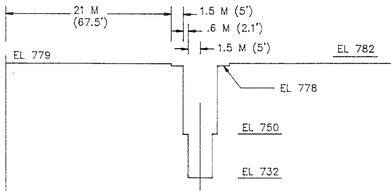
TYPE 6 WEIR - ELEVATION
