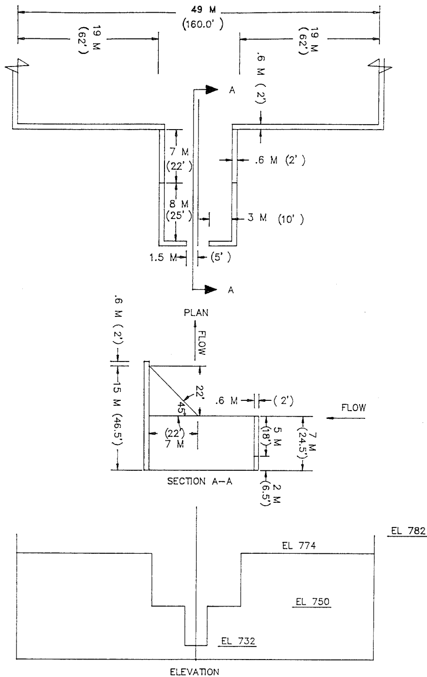
TYPE 22 WEIR DESIGN
