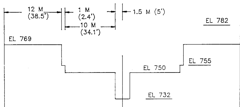
TYPE 10 WEIR - ELEVATION
