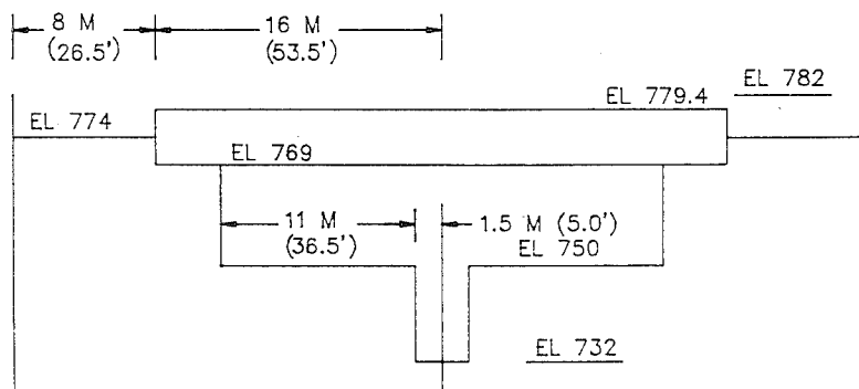
TYPE 12 WEIR - ELEVATION
