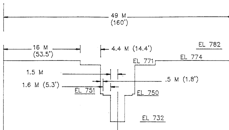
TYPE 5 WEIR - ELEVATION
