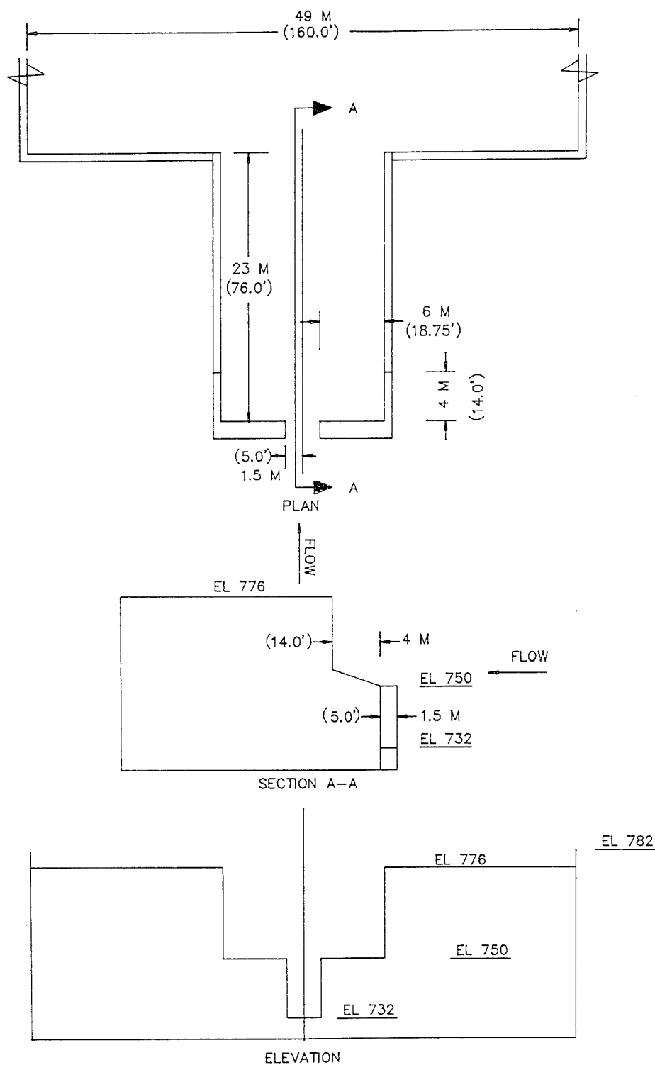
TYPE 16 WEIR DESIGN
