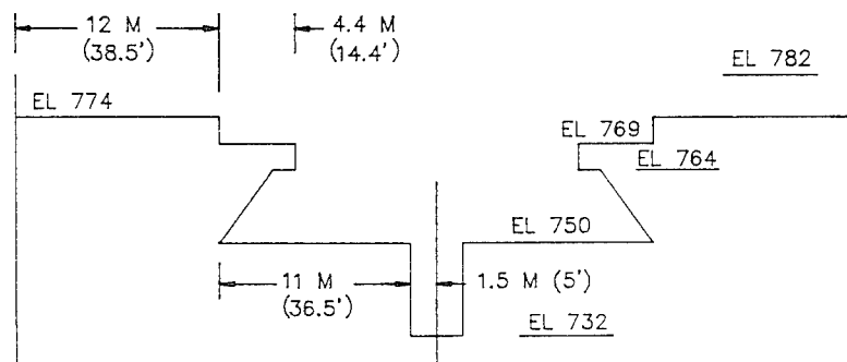
TYPE 13 WEIR - ELEVATION
