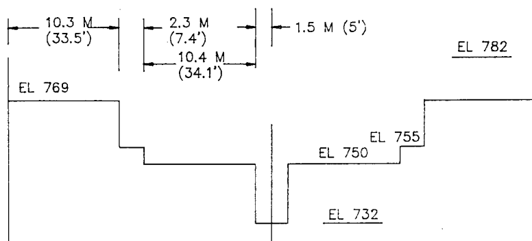
TYPE 9 WEIR - ELEVATION
