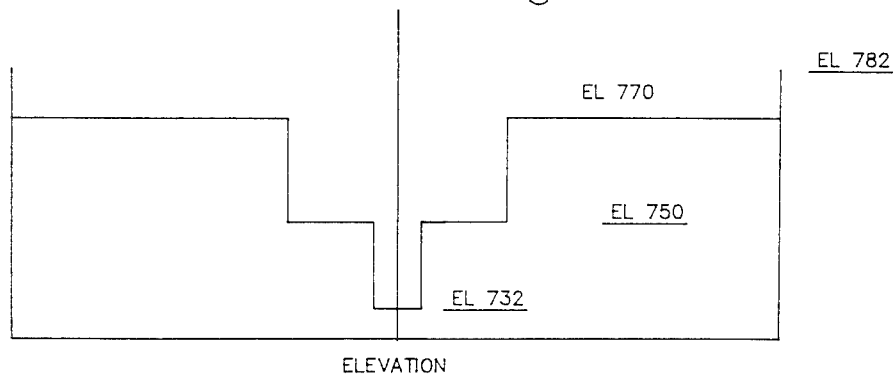
TYPE 25 WEIR DESIGN
