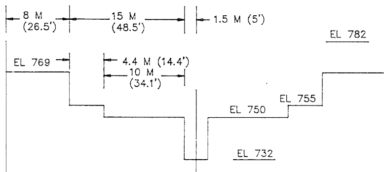
TYPE 7 WEIR - ELEVATION
