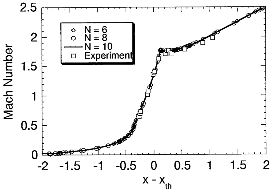
Fig. 20. Wall Mach number for the converging-diverging nozzle.
