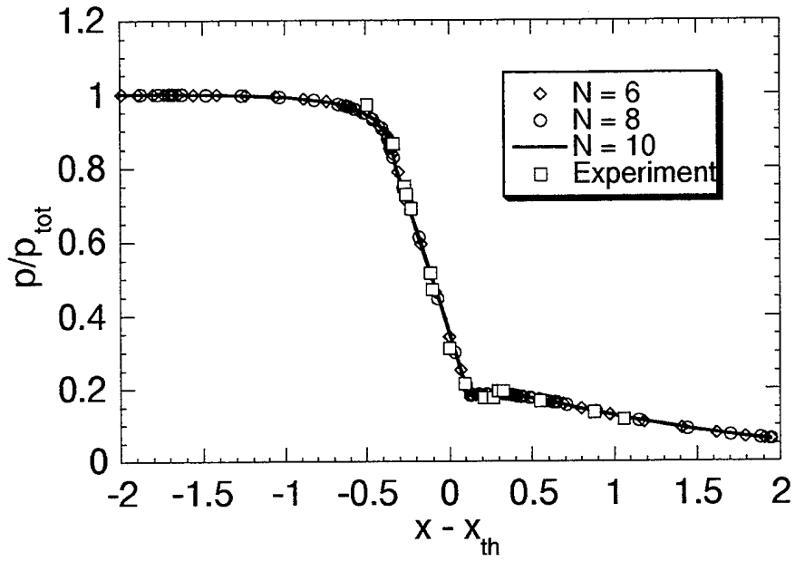
Fig. 19. Wall pressure of the converging-diverging nozzle
