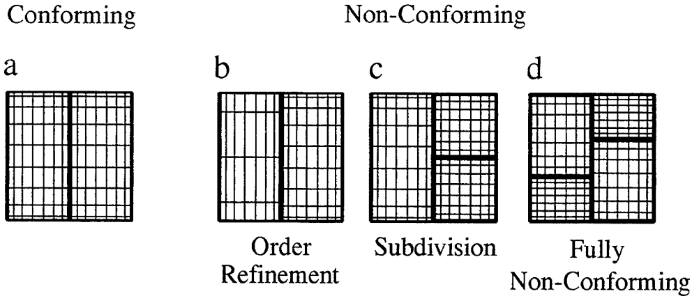
Fig. 1 Conforming vs. non-conforming grids
