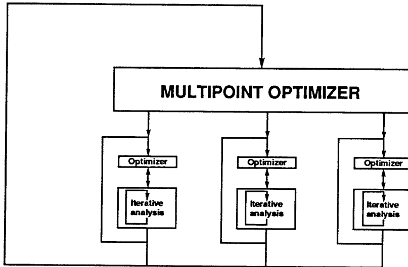
Fig. 12. Multipoint, multilevel SAND-NAND optimization with iteratively solved state equations.
