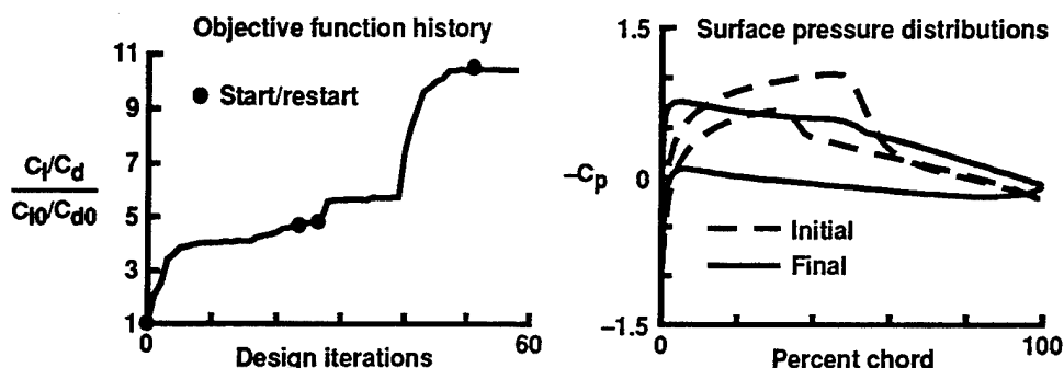
Fig. 5. Objective function and surface pressure distributions for turbulent transonic airfoil improvement.
