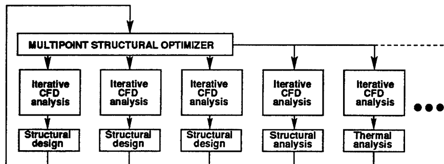
Fig. 16. Multipoint, multilevel hybrid structural optimization with MDA.
