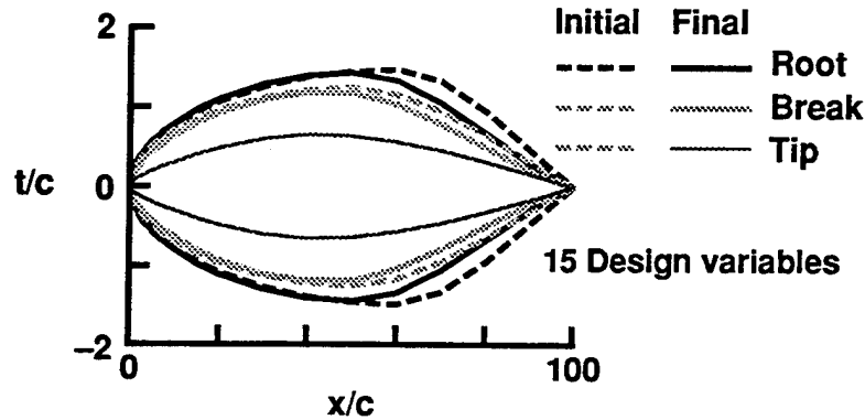
Fig. 3. Wing section thickness distributions for HSCT 24E design improvement.
