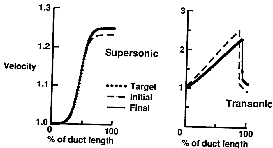
Fig. 8. Nozzle velocity distributions for supersonic and transonic flow SAADO feasibility demonstration.
