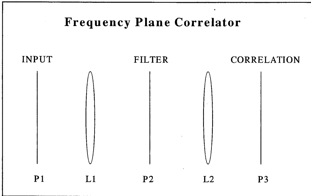
Figure 3. Schematic of a Frequency Plane Correlator.
