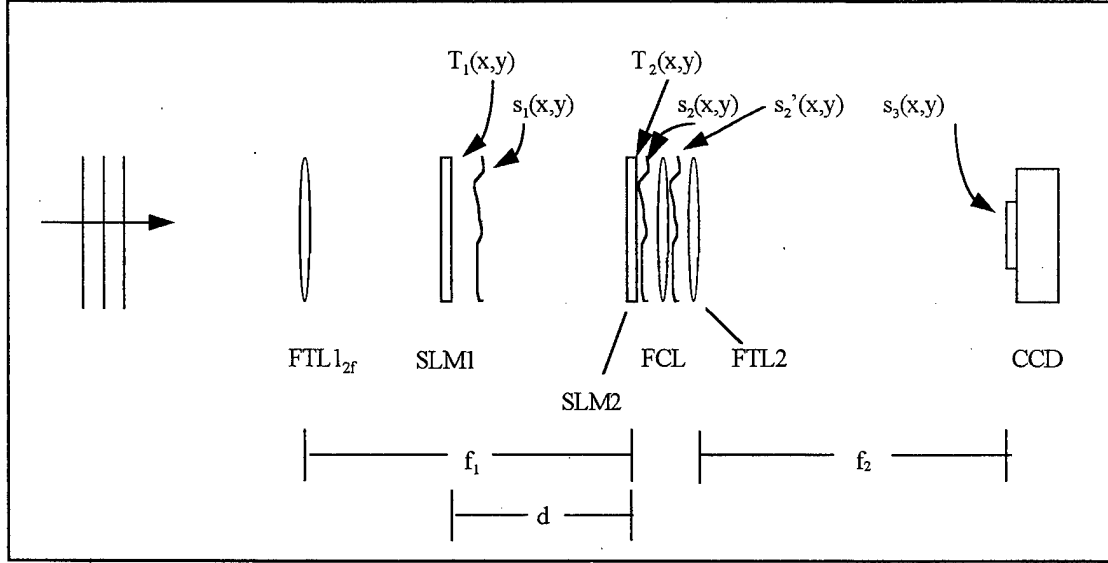
Figure 11. Model for 2f correlator including (conceptual) phase compensation lens, FCL, behind SLM2..
