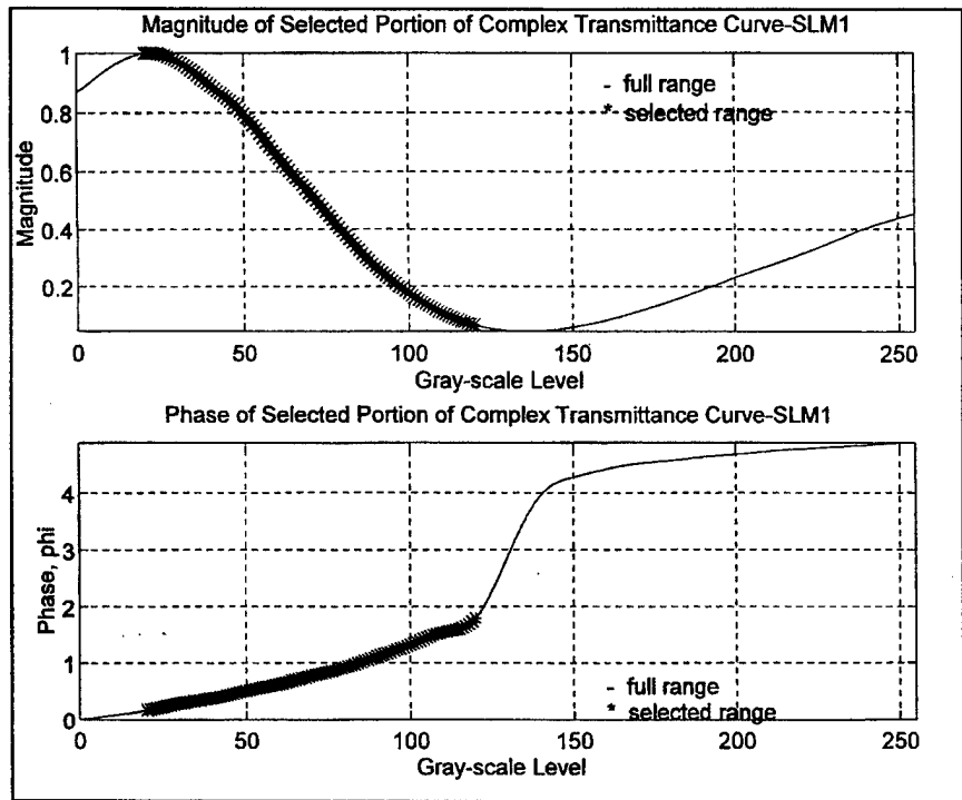
Figure 24. Selected portion of input SLM's complex operating curve for gray-scale values 20-120 (highlighted points). Upper curve is transmittance magnitude and lower curve is transmittance phase.
