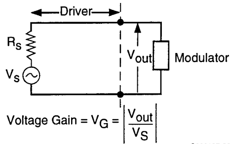
Figure 4-11. Circuit Schematic of a Typical RF Source Driving a Modulator
