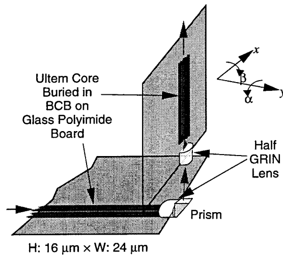
Figure 3-6. Schematic of Polymer Backplane Experiment
