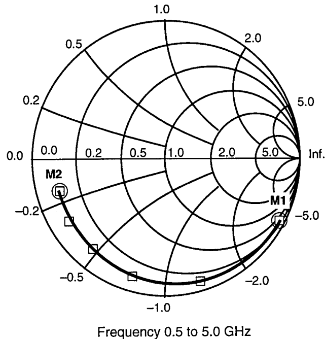
Figure 4-7b. Measured Input Impedance of the Modulator at a Bias of -7.6 V
