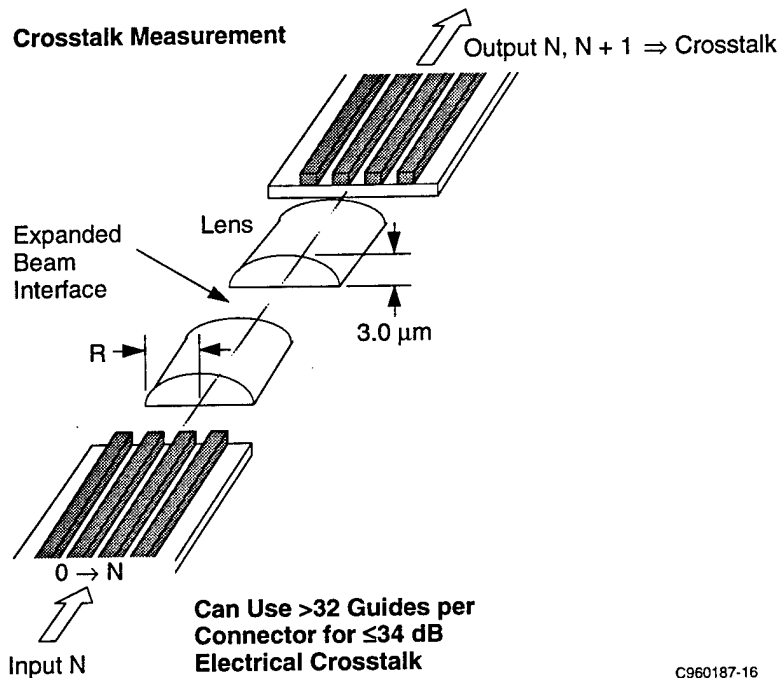
Figure 3-5. Crosstalk Evaluation of Board-to-Backplane Connector
