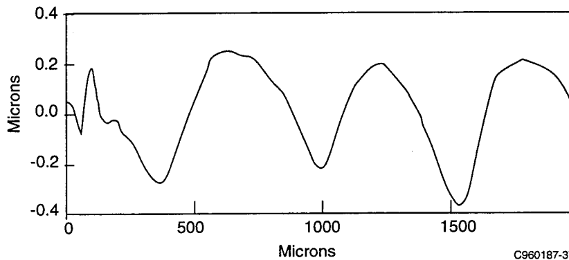
Figure 4-22. Variation in Surface Height of Glass:Polyimide Substrate after Planarization with BCB
