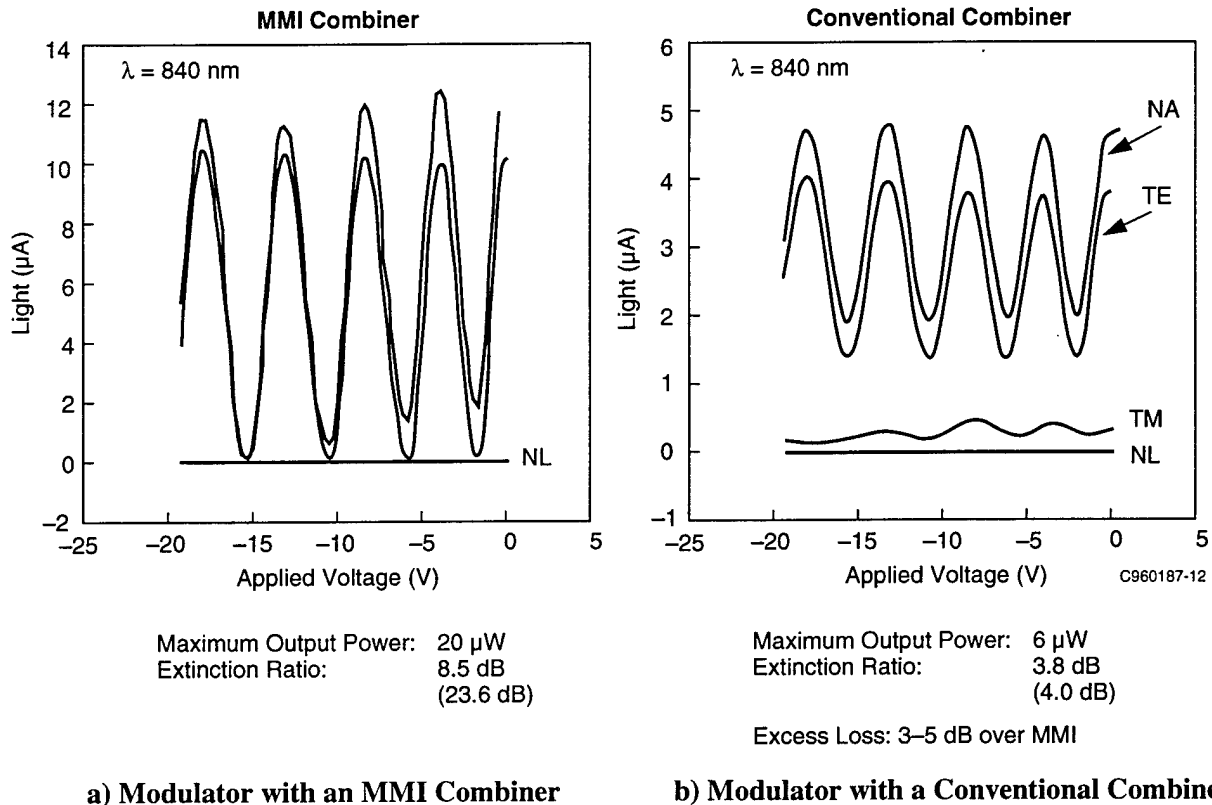
Figure 4-5. Light Transmitted vs. Applied Voltage
