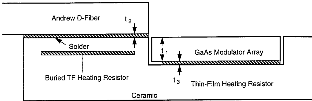
Figure 3-2a. Single-Mode Pigtail Assembly Technique
