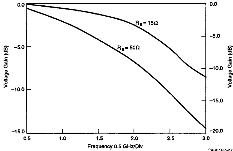
Figure 4-12. Calculated Complex Gain of the Circuit for Various Source Impedances
