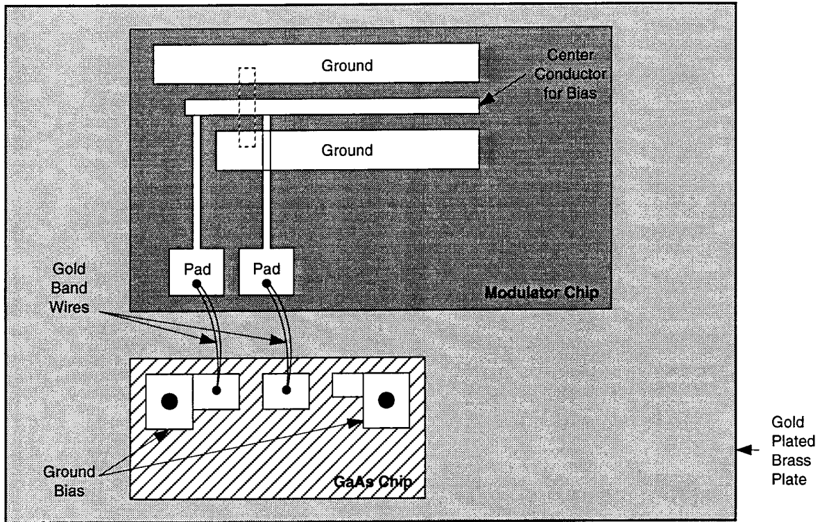
Figure 4-6. Modulator Packaged for On-wafer RF Measurements
