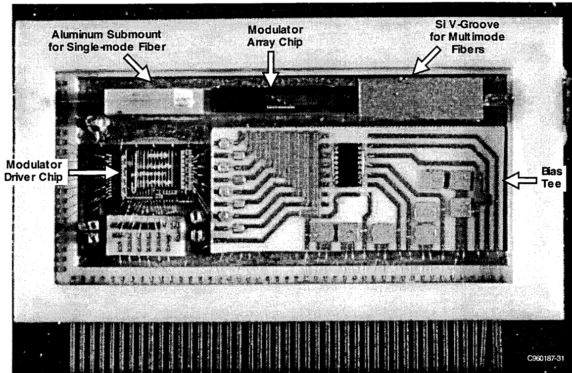
Figure 4-17. Completed Waveguide-Modulator-Based Package
