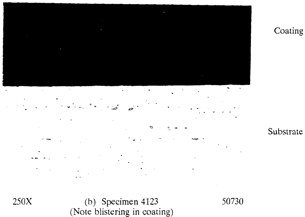
FIGURE 8. PHOTOMICROGRAPHS DOCUMENTING NONCORRODED SURFACES SPECIMENS 2112 AND 4123
