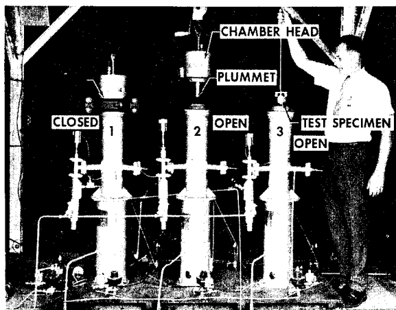
FIGURE 140.—Impact-test chambers.
