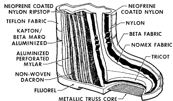
FIGURE 103.—Pressure-garment-assembly boot.
