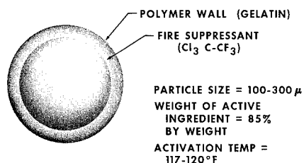
FIGURE 61.—Encapsulated fire-suppressant particle (microballoon).
