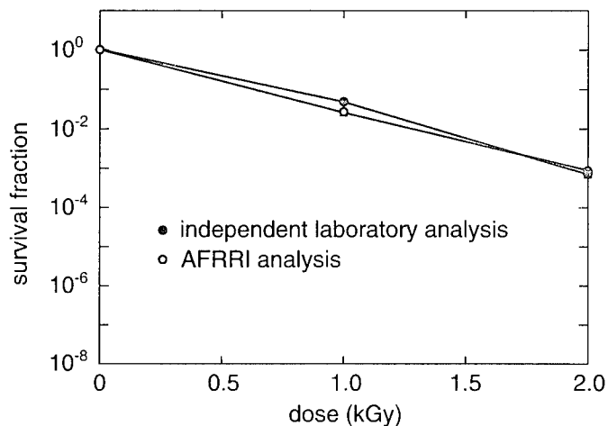
Fig. 3. Survival fractions of dry B. pumilus spores after selected doses of neutron radiation; validation of the AFRRRI technique used for spore survival analyses after neutron irradiation compared to analyses performed by the independent commercial laboratory. The filled circle (●) represents survival data determined by the independent commercial laboratory, and the open circle (○) represents survival data determined by AFRRRI. Each data point represents spore survival obtained from 2-11 cellulose fiber spore-impregnated strips.
