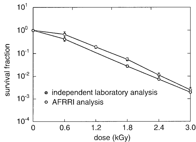
Fig. 4. Survival of dry B. subtilis spores after \gamma irradiation. The filled circle ( \odot ) represents survival data determined by the independent commercial laboratory, and the open circle ( \circ ) represents survival data determined by AFRRRI. Each data point represents spore survival from 3-13 cellulose fiber spore-impregnated strips.
