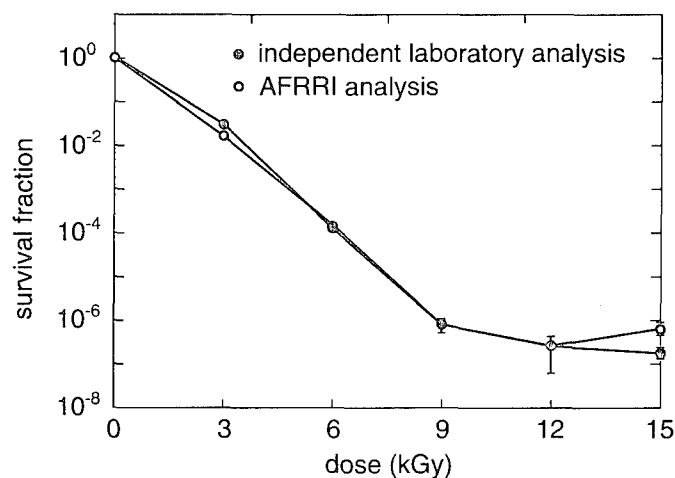
Fig. 2. Survival fractions of dry B. pumilus spores after selected doses of \gamma radiation; validation of the AFRRRI technique used for spore survival analyses after \gamma -irradiation compared to analyses performed by the independent commercial laboratory. The filled circle (●) represents survival data determined by the independent commercial laboratory, and the open circle (○) represents survival data determined by AFRRRI. Each data point represents spore survival obtained from analyzing 2-11 cellulose fiber spore-impregnated strips.
