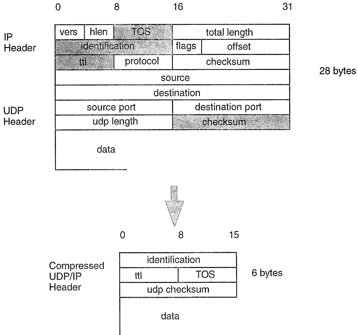
Fig. 3 - UDP/IP compression scheme
