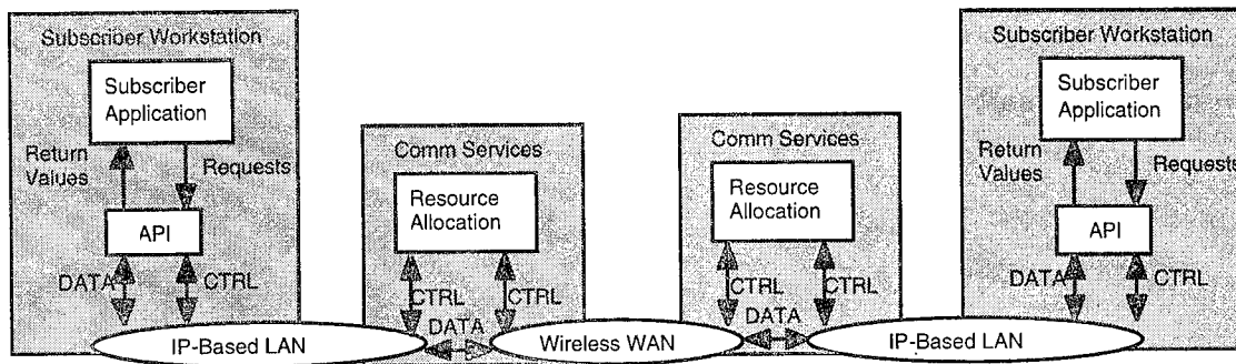
Fig. 5 - Data/Voice Integration Phase 2 API/CS architecture
