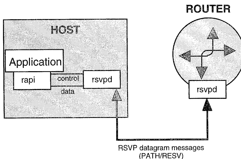
Fig. 7 - RAPI/RSVPD operation
