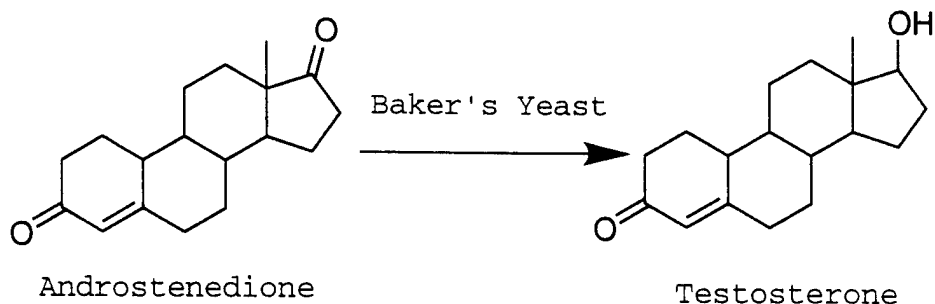
Scheme 1.7 Androstenedione reduction
