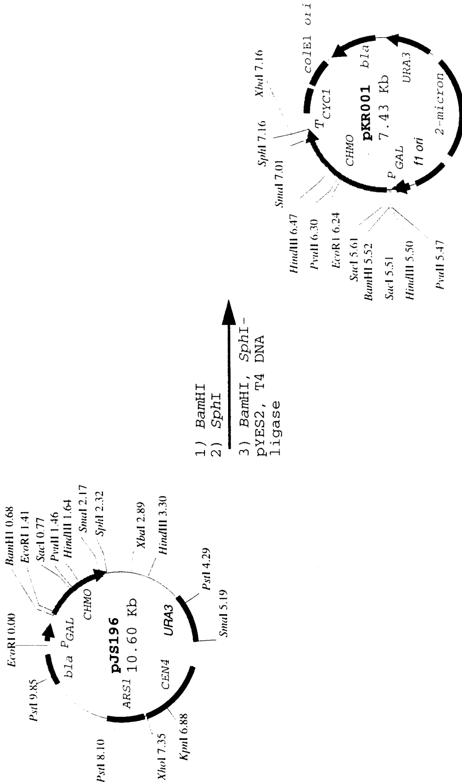
Scheme 2.2 pKR001 Construction
