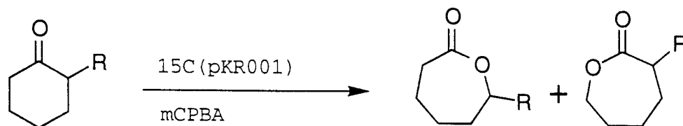
Scheme 2.11
