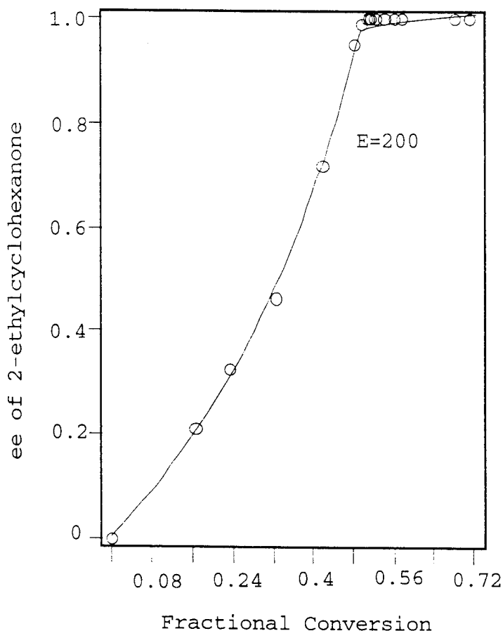
Figure 2.18 Determination of the E for the Yeast-mediated Baeyer-Villiger Oxidation of 2-ethylcyclohexanone
