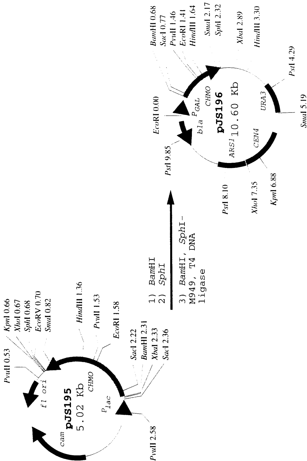
Scheme 2.1 continued
