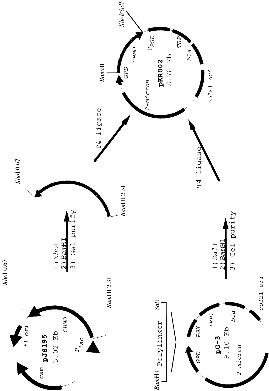
Scheme 2.3 pKR002 Construction
