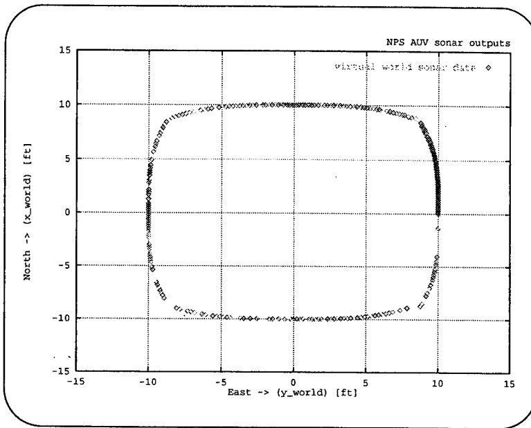
Figure 5.1 Sonar Data from Virtual World.
