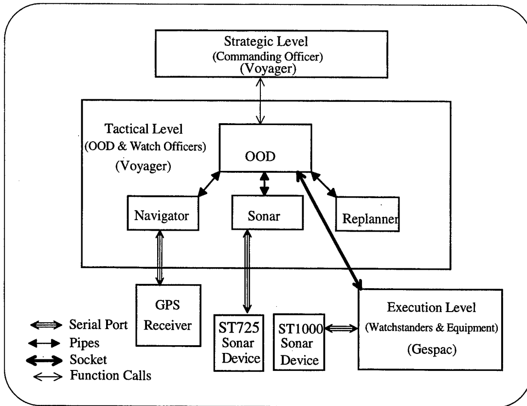
Figure 2.1 Current Software Architecture and Communication Modes.
