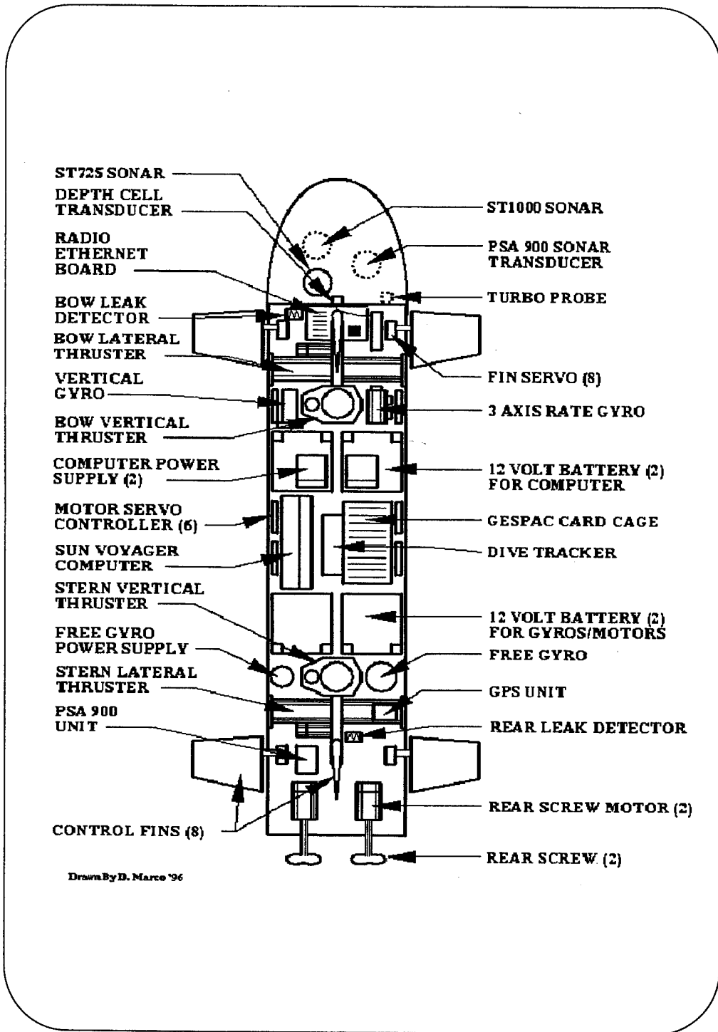
Figure 1.1. Internal View of Phoenix (Marco 96).
