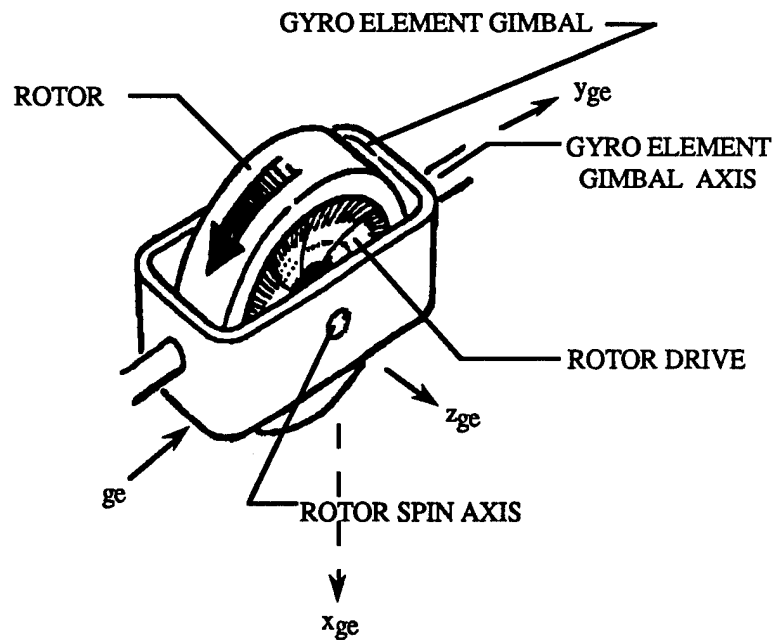
FIGURE 14-2. THE GYROELEMENT
