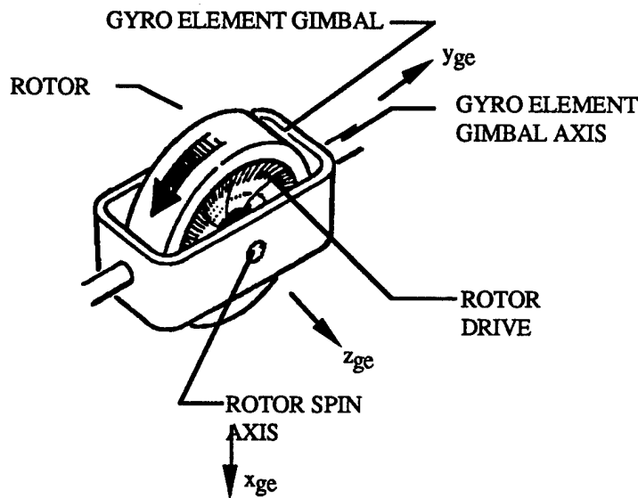
FIGURE 13-1. GYRO ELEMENT
