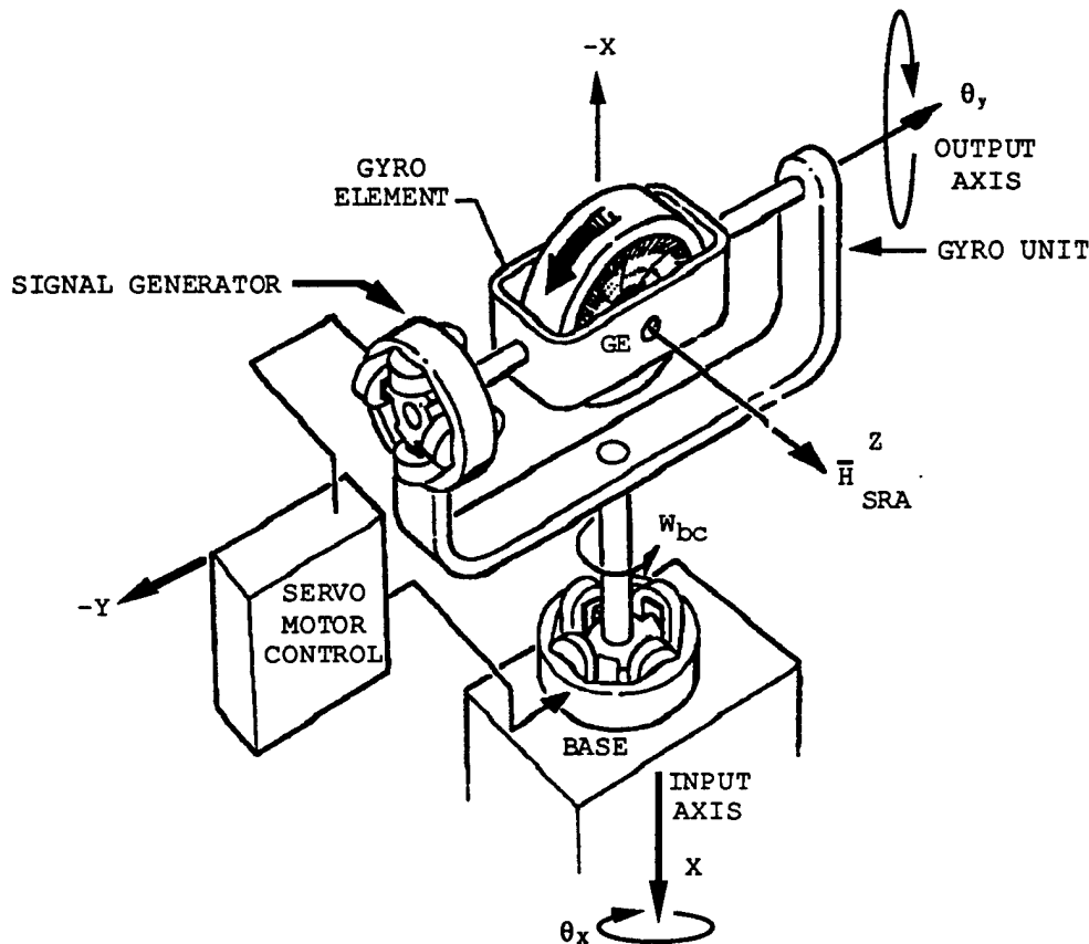
FIGURE 15-2. MECHANICAL SCHEME FOR SINGLE-AXIS STABLE PLATFORM
