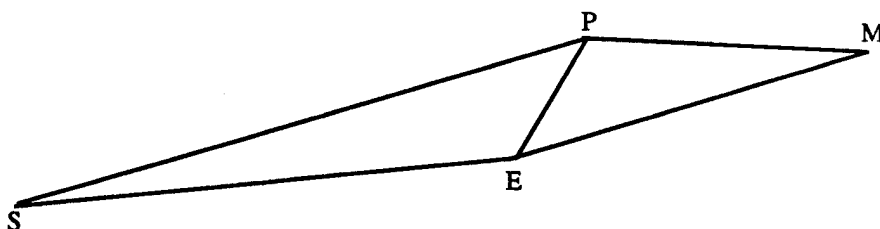
FIGURE 5-1. THE SUN, MOON, AND EARTH SYSTEMS
