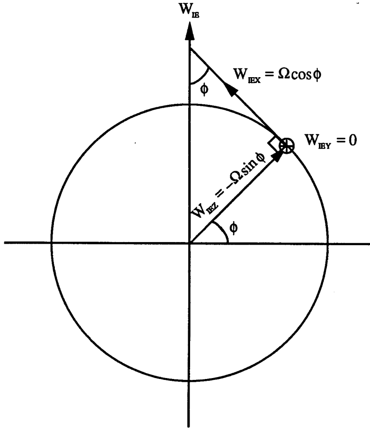
FIGURE 17-3. DECOMPOSITION OF THE EARTH RATE INTO NED COMPONENTS
