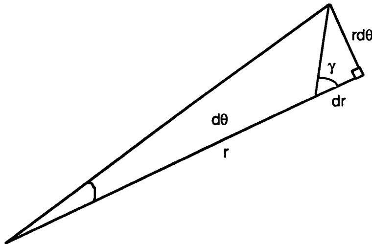
FIGURE 22-2 DEPICTION OF \cot \gamma = \frac{dr}{rd\theta}
