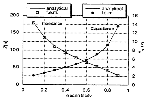
Fig.2: Comparison between analytical (f.e.m.) data of the characteristic TEM impedance and of the normalized Capacitance (ratio C/\epsilon_0 ) per unit length, plotted versus the excentricity of the cross section.
