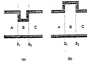
Figure 2: Geometry of (a) a thick iris and (b) a stub discontinuity.
