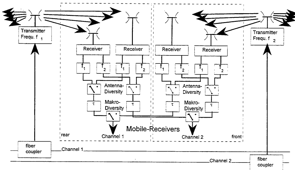
Diversity-Concept Base-to-Mobile-Station
