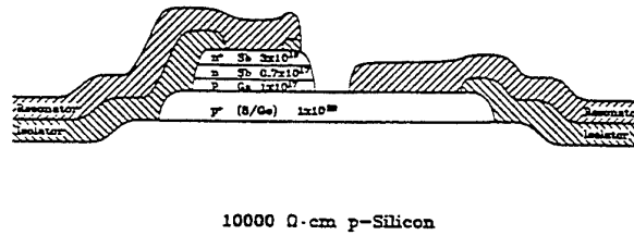
Fig. 8: Cross section of a coplanar IMPATT diode.
