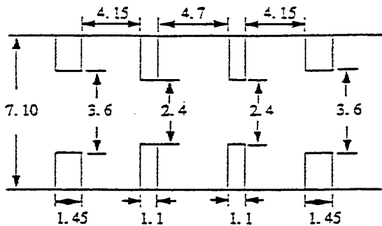
Figure 5: Geometry of a bandpass filter for the Ka-band. Dimensions are given in mm.
