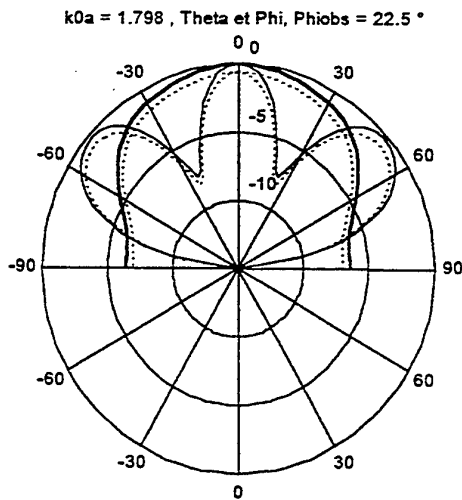
Figure 4 : Polar power radiation pattern for configuration #2 with 3° extended sources. — infinite internal impedance ..... finite internal impedance : R = 1k\Omega , C = 1 pF
