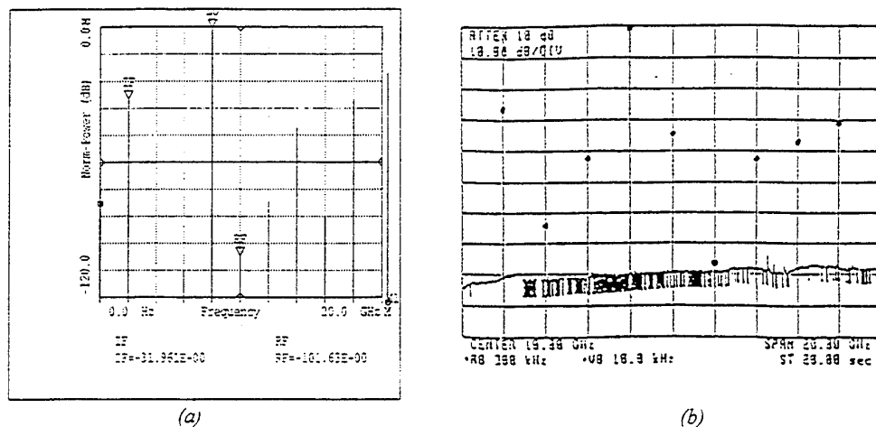
Figure 2 : Mixer normalised output power. (a) computed results by FEM-MDS. (b) experimental results.
