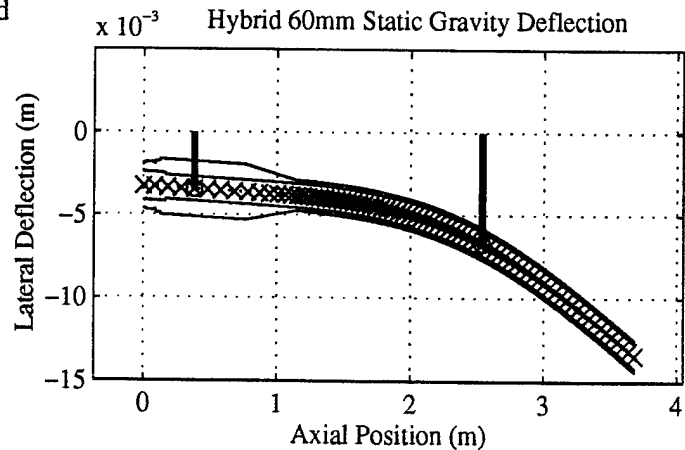
Figure 17 Gravity Droop Computed in Section 12 of <hybrid60.m>.
