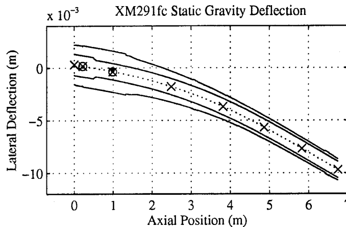
Figure 14 Gravity Deflection Computed in Sections 11 to 14 of <XM291fc.m>.
