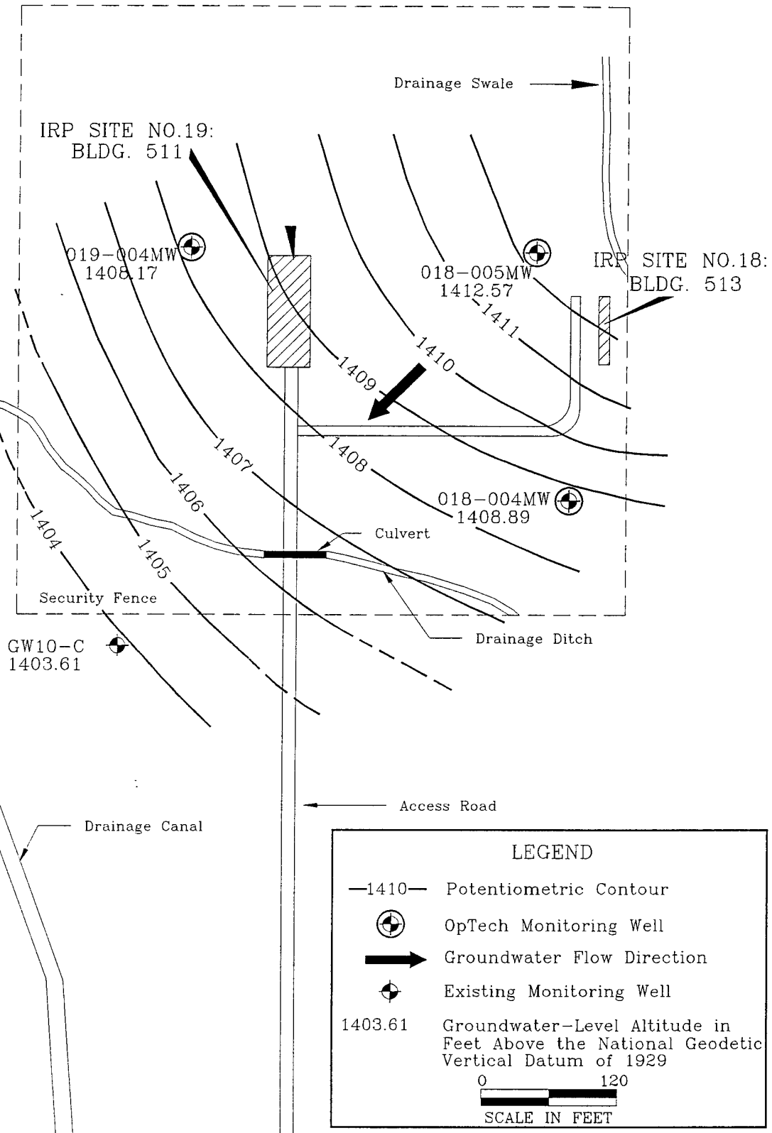
POTENTIOMETRIC SURFACE MAP AS OF 28 MARCH 1992 FOR IRP SITES NO.18 AND NO.19 Duluth Air National Guard Base Duluth, Minnesota
