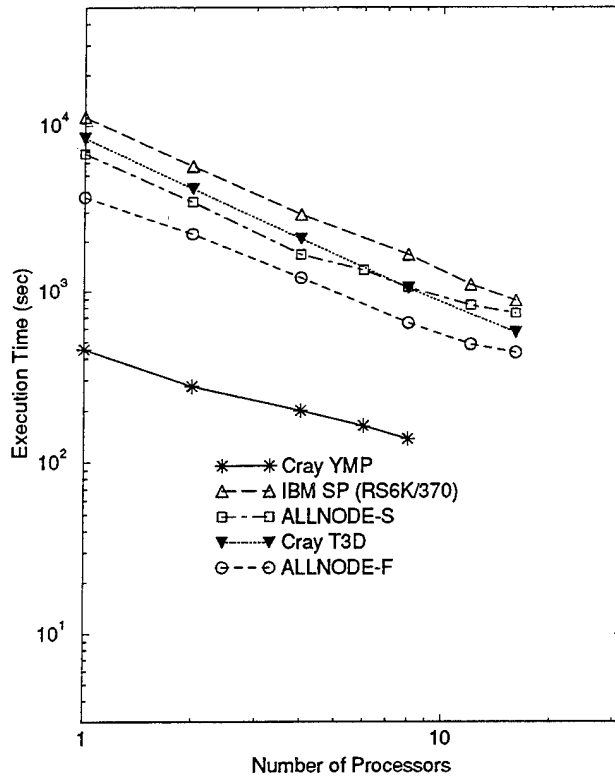
Figure 9: Execution time of Euler on computing platforms
