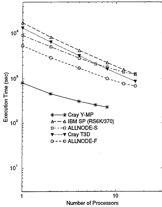
Figure 8: Execution time of Navier-Stokes on computing platforms
