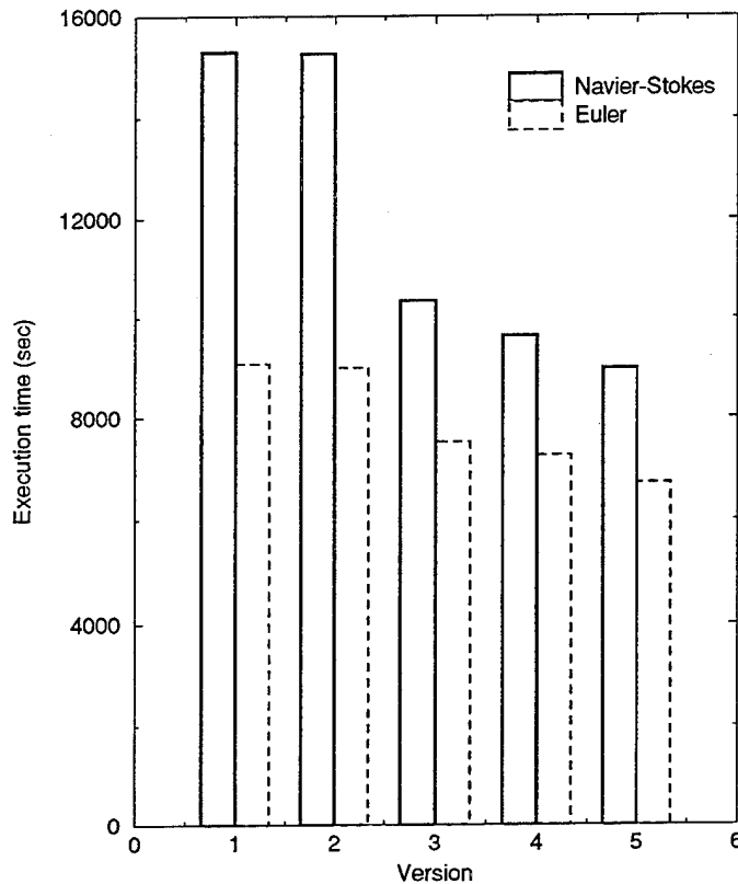
Figure 2: Execution time on a single processor (RS6000/560)
