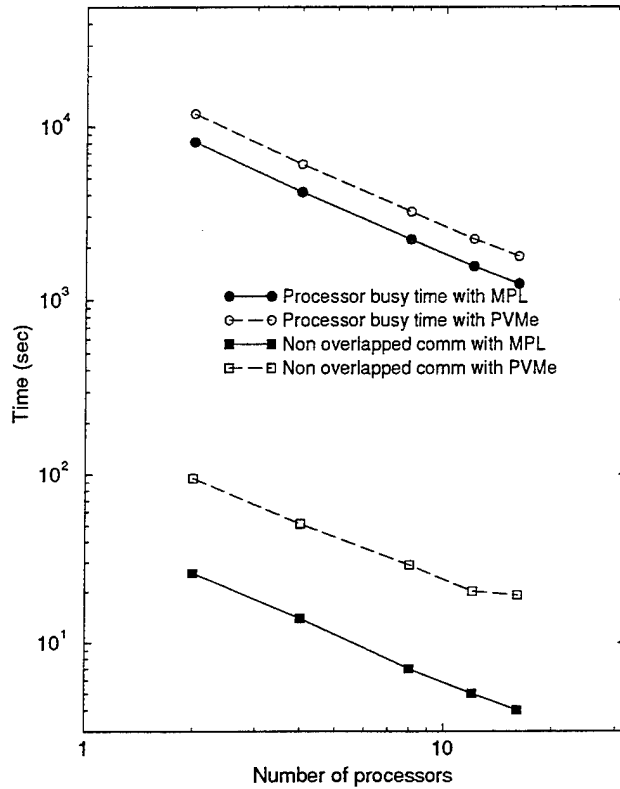
Figure 10: Comparison of MPL and PVMe (Navier-Stokes; IBM SP)
