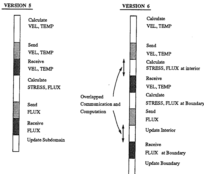
Figure 3: Timeline of processor activity
