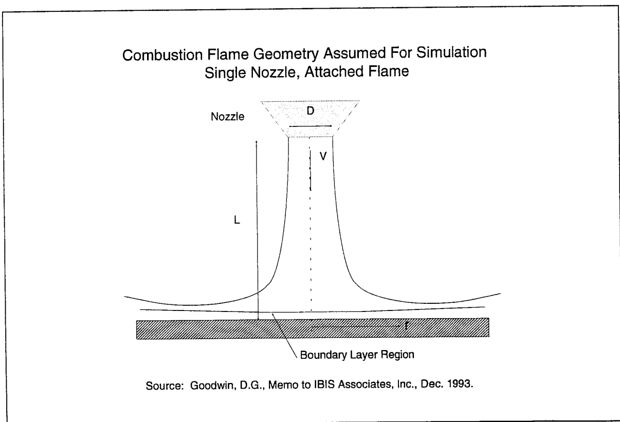
Figure 7. Combustion Flame Geometry
