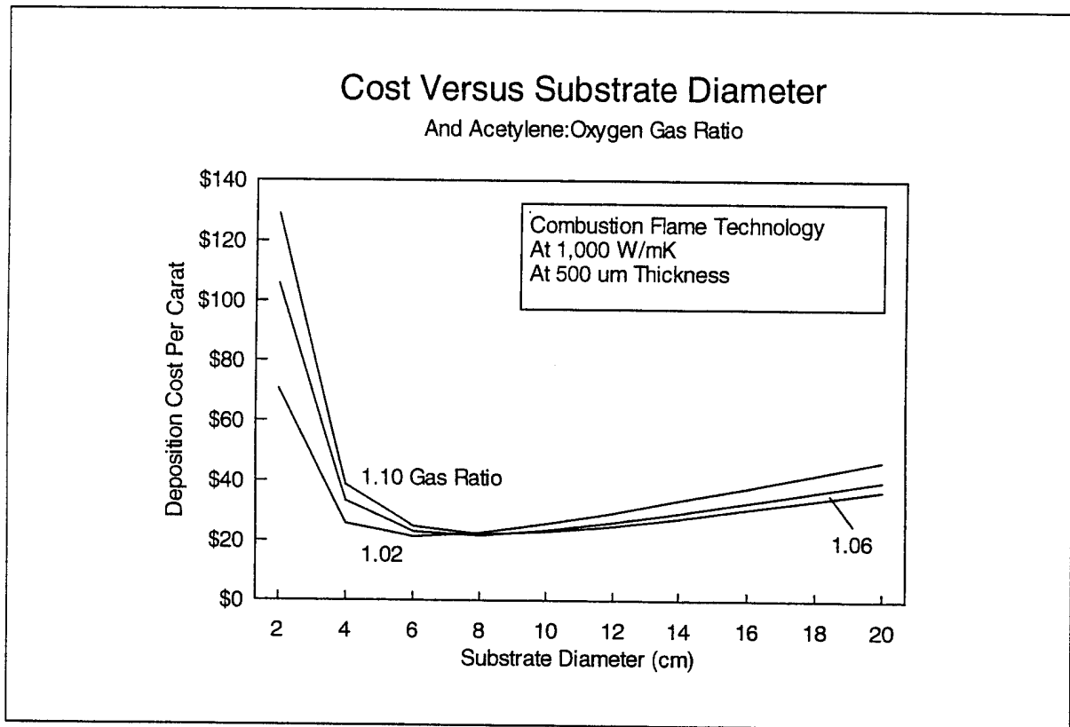
Figure 12. Combustion Flame Results
