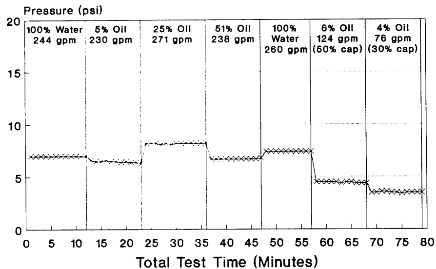
Figure 60: Surge Tank Crude Oil Test Series Influent Line Pressure vs. Time
