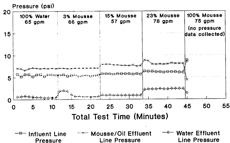
Figure 40: Alfa-Laval Mousse With Emulsion Breaker Test Series Influent and Effluent Line Pressure vs. Time
