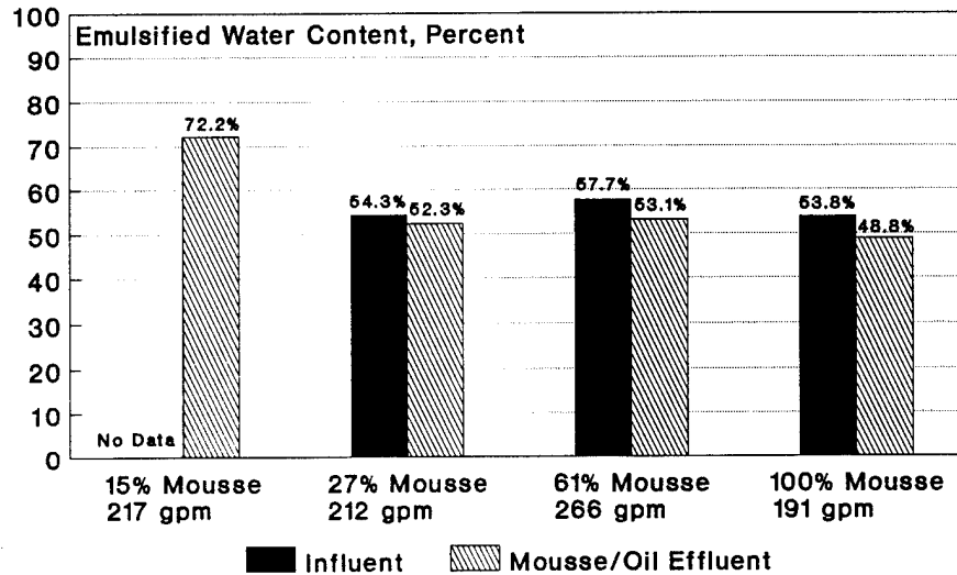
Figure 101: Vortoil Mousse Test Series Emulsified Water Content Before and After Separation
