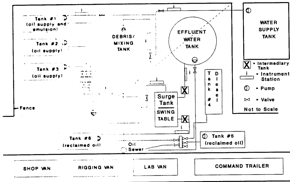
Figure 55: Test Facility Set-Up for Surge Tank
