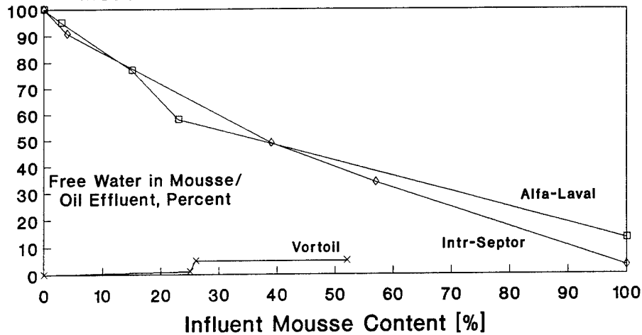
Figure 160: Separator Performance Comparison: Mousse With Emulsion Breaker Test Series: Free Water Content of Mousse/Oil Effluent vs. Influent Mousse Content
