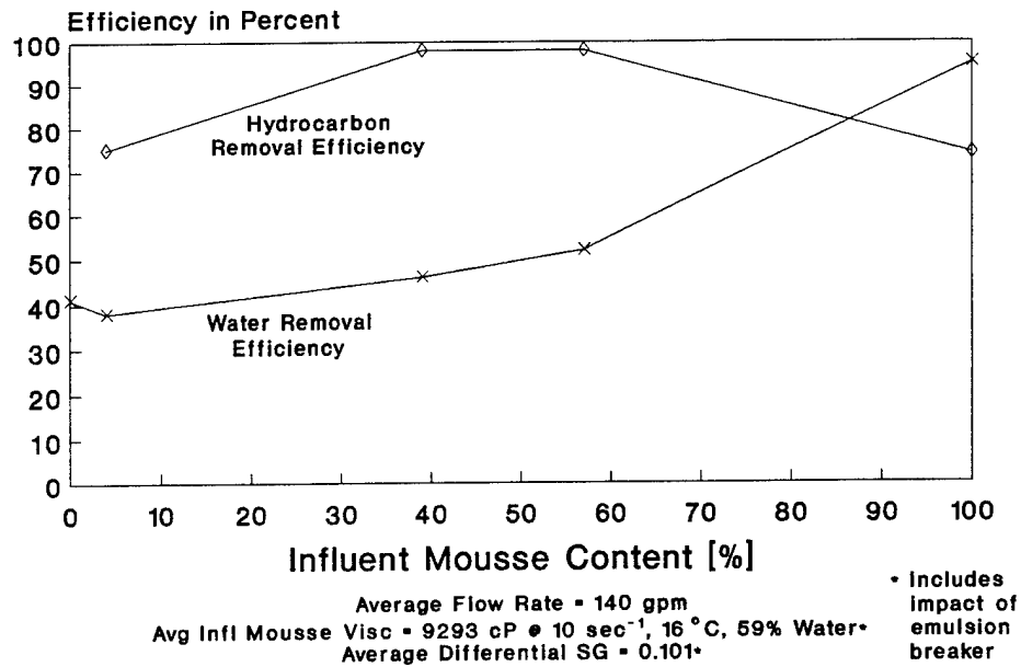
Figure 129: Intr-Septor Mousse With Emulsion Breaker Test Series Efficiency vs. Influent Mousse Content
