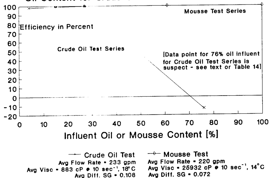
Figure 90: Impact of Mousse on Vortoil: Comparison of Hydrocarbon Removal Efficiency vs. Influent Mousse/ Oil Content for Crude Oil and Mousse Test Series
