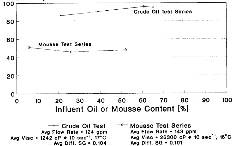
Figure 126: Impact of Mousse on Intr-Septor: Comparison of Hydrocarbon Removal Efficiency for Crude Oil and Mousse Test Series
