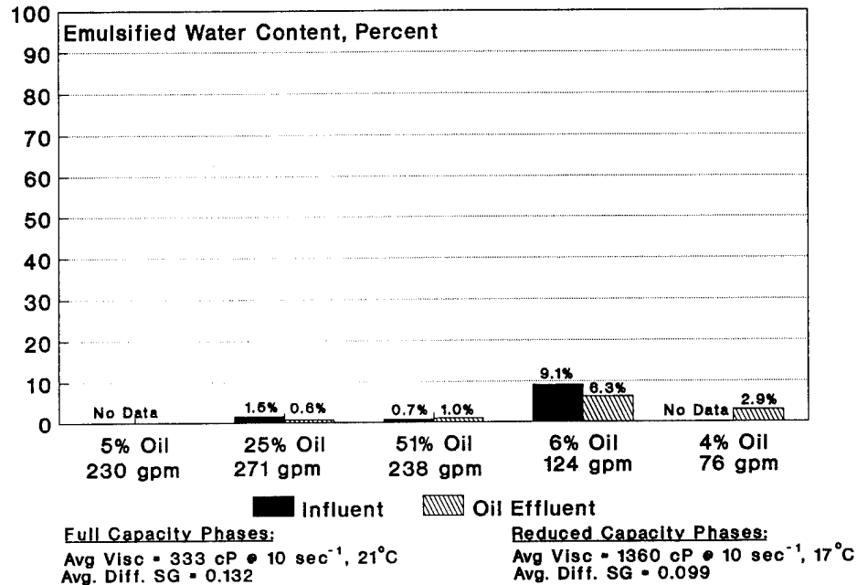
Figure 59: Surge Tank Crude Oil Test Series Emulsified Water Content Before and After Separation
