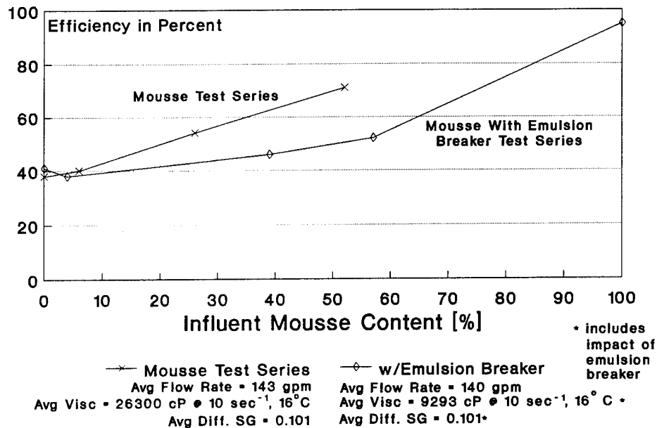
Figure 136: Impact of Emulsion Breaker on Intr-Septor: Comparison of Water Removal Efficiency for Mousse and Mousse With Emulsion Breaker Test Series
