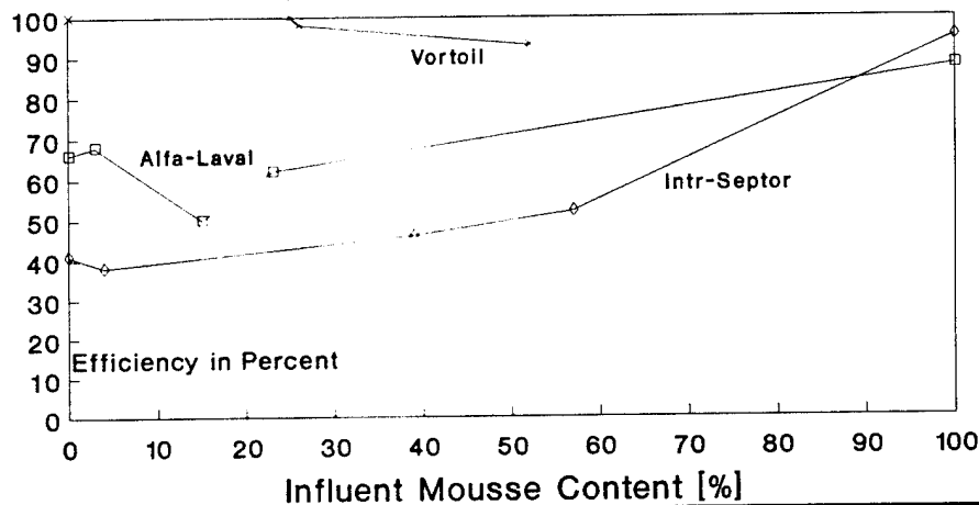
Figure 161: Separator Performance Comparison: Mousse With Emulsion Breaker Test Series: Water Removal Efficiency vs. Influent Mousse Content
