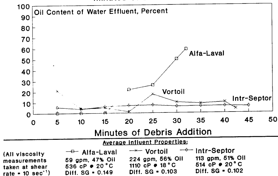
Figure 165: Separator Performance Comparison: Debris Test Series Oil Content of Water Effluent Stream vs. Minutes of Debris Addition
