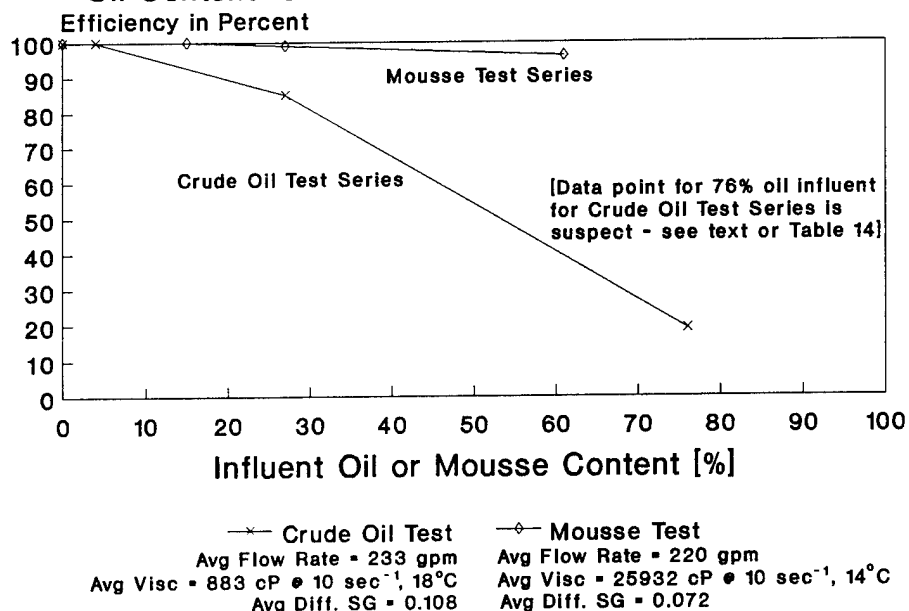
Figure 89: Impact of Mousse on Vortoil: Comparison of Water Removal Efficiency vs. Influent Mousse/ Oil Content for Crude Oil and Mousse Test Series
