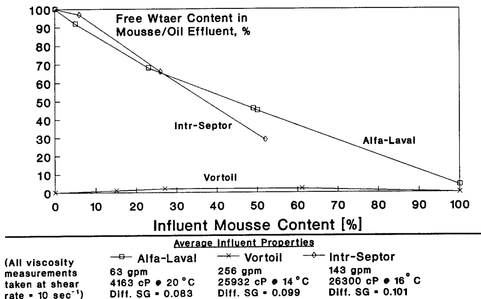
Figure 154: Separator Performance Comparison: Mousse Test Series Free Water Content of Mousse/Oil Effluent vs. Influent Mousse Content
