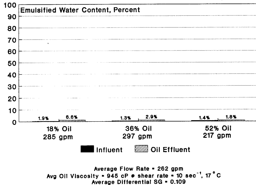
Figure 65: Surge Tank Sea Motion Test Series Emulsified Water Content Before and After Separation
