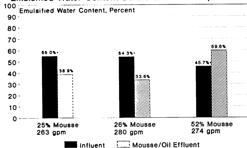
Figure 102: Vortoil Mousse With Emulsion Breaker Test Series Emulsified Water Content Before and After Separation
