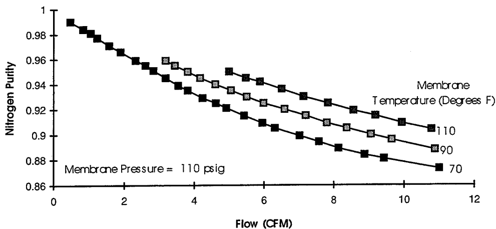
FIGURE 10. VARIATION OF FLOW WITH NITROGEN PURITY AT MEMBRANE TEMPERATURES OF 70, 90, AND 110°F AND A CONSTANT MEMBRANE PRESSURE OF 110 PSIG
