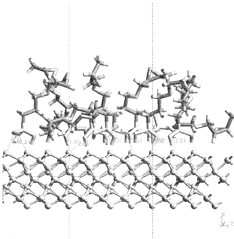
Figure 3.4 Distance of surface aluminium and silane oxygen interactions
