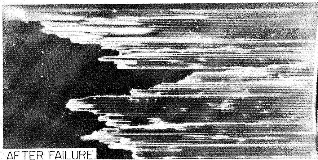
Figure 34e. Typical Sequence of Photographs of Tensile Failure Specimen Showing Distribution of Fiber Breaks Prior to Failure (Specimen A-7)
