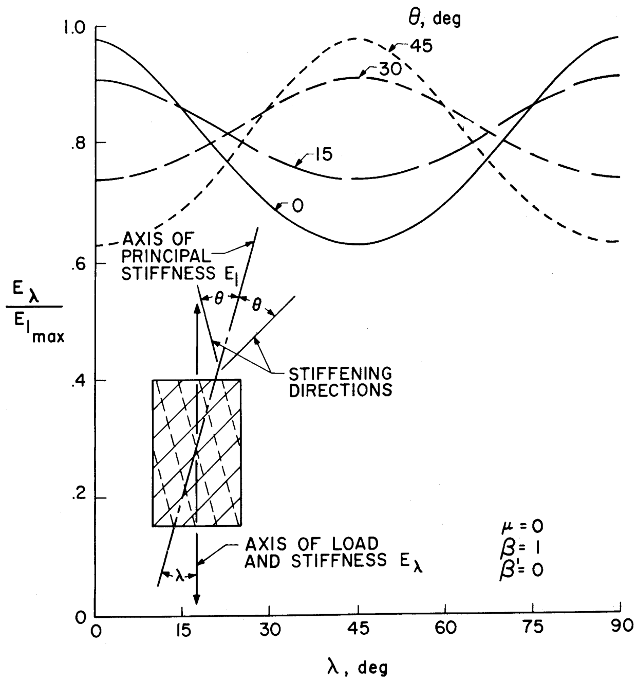
Figure 2lg. Combined Effects of Variations in Angles of Orientation of Holes, Transverse Effectiveness, and Poisson's Ratio on Stretching Stiffness
