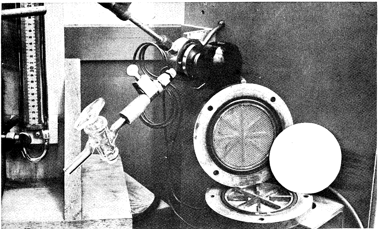
Figure 12. Open Permeation Cell with Test Specimen.
