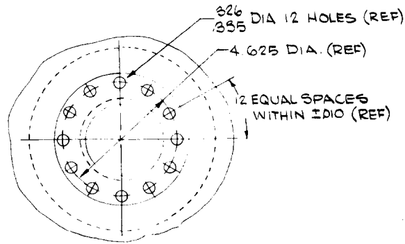
VIEW B-B
