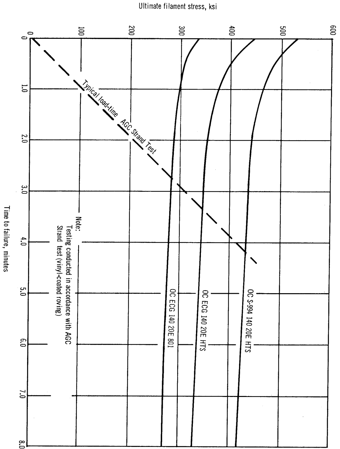
Figure 30. Ultimate Filament Stress vs Time to Failure
