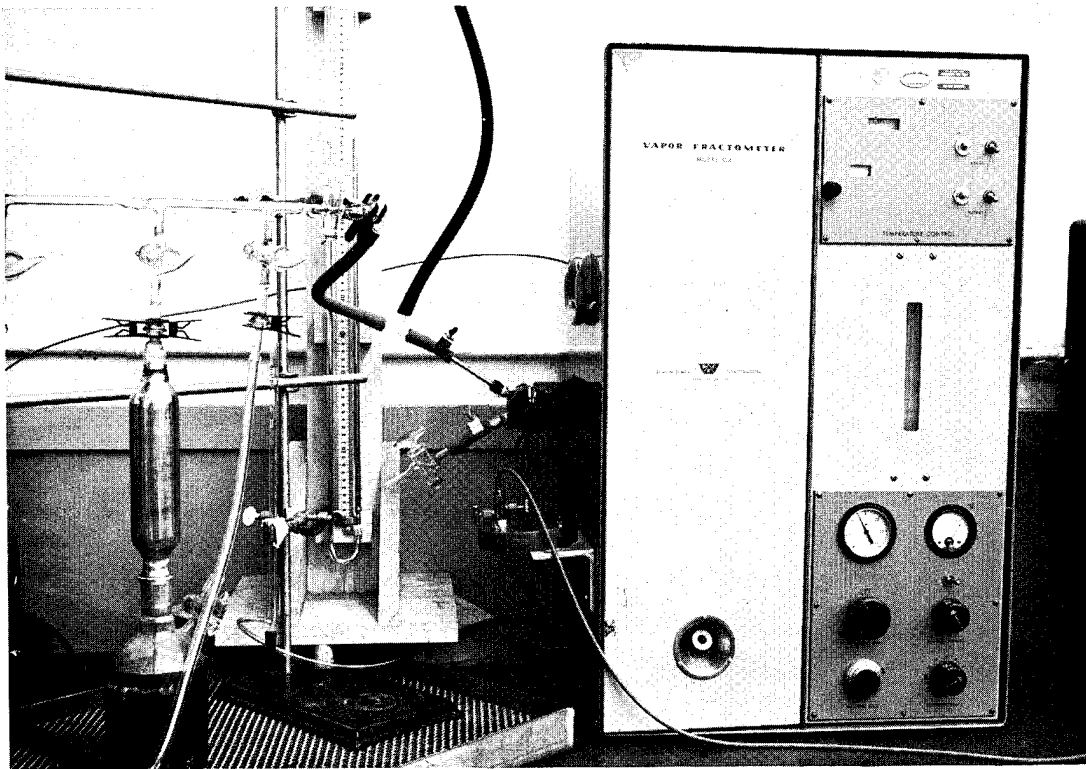
Figure 13. Permeability Measuring Equipment.
