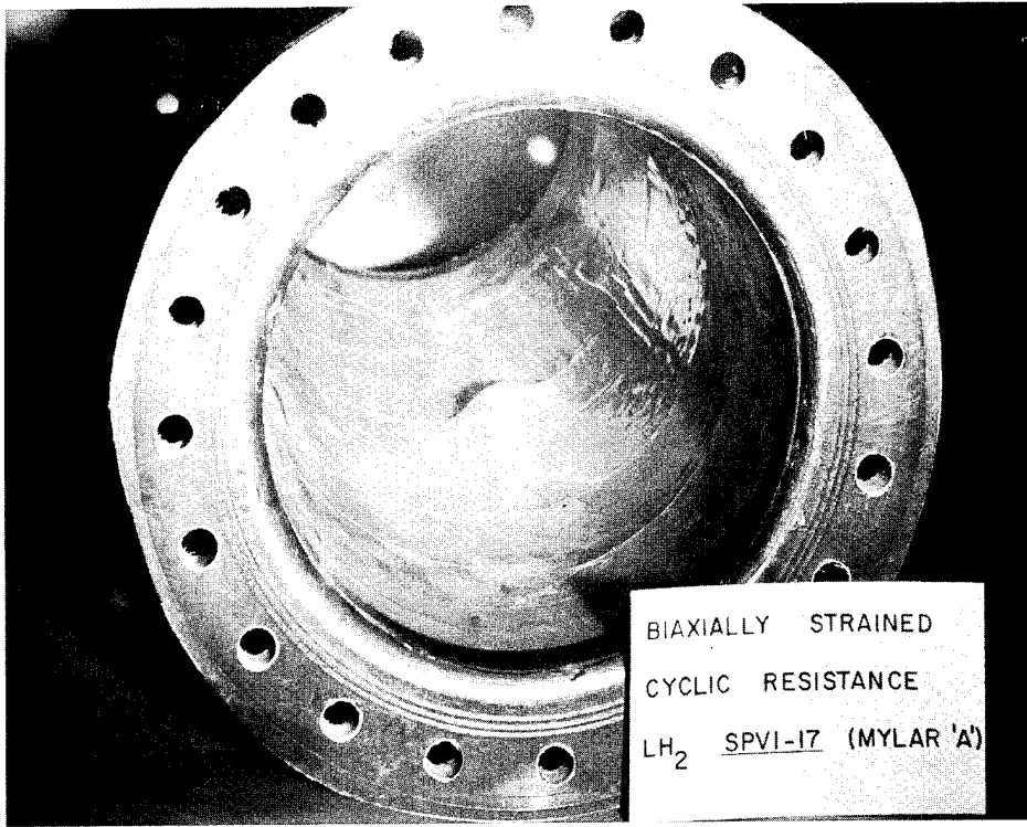
Figure 31. Mylar Lined Specimen SPV 1-17; After Test.
