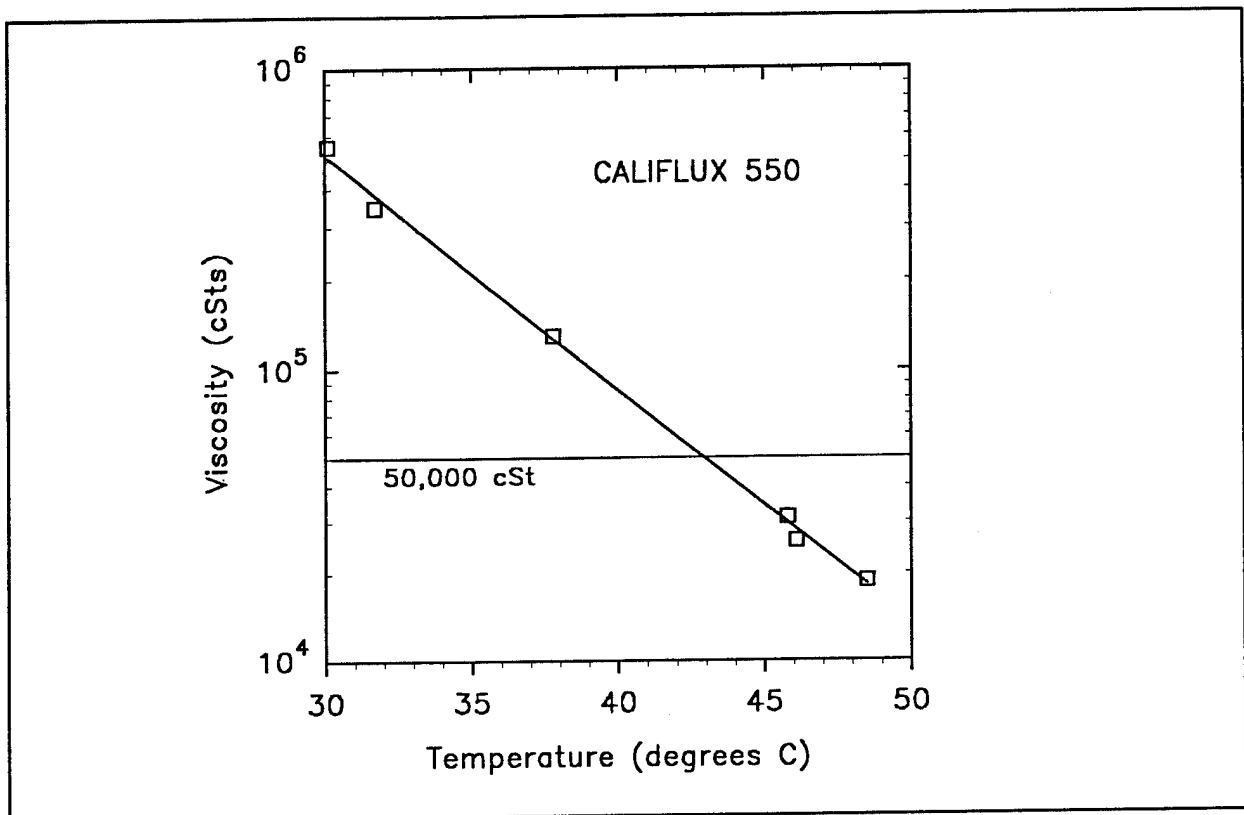
Figure 5 CALIFLUX 550 Viscosity Versus Temperature
