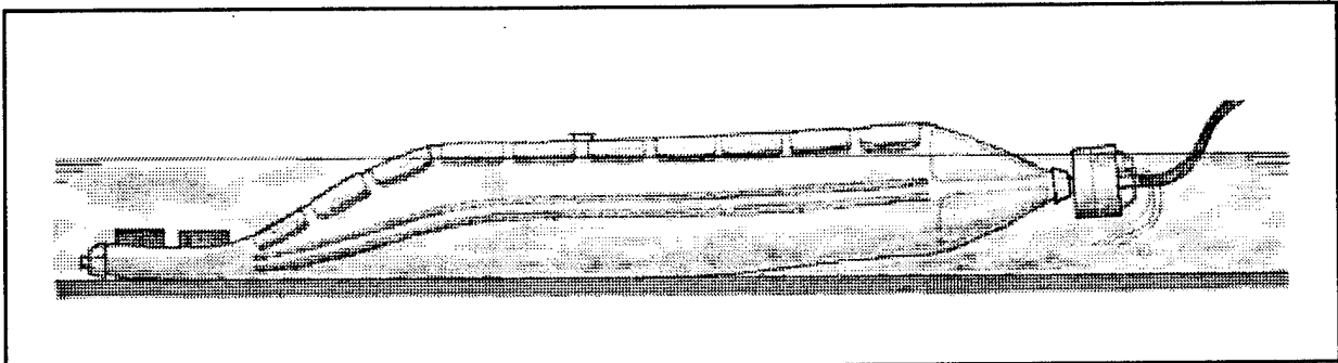
Figure 8 Weight Assisted Offloading Arrangement
