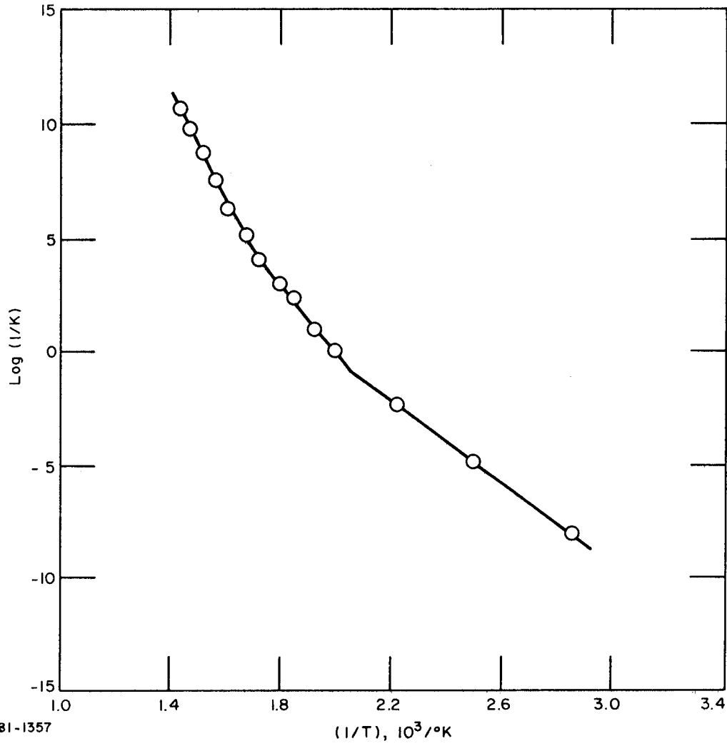
Figure 31 SHIFT FUNCTION OF POLYIMIDE P
