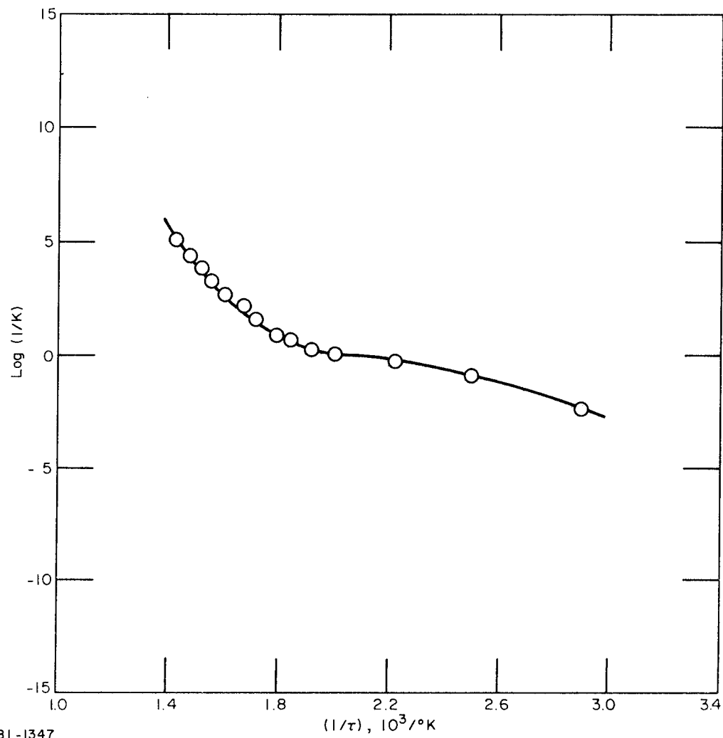
Figure 21 SHIFT FUNCTION OF PYRRONE L
