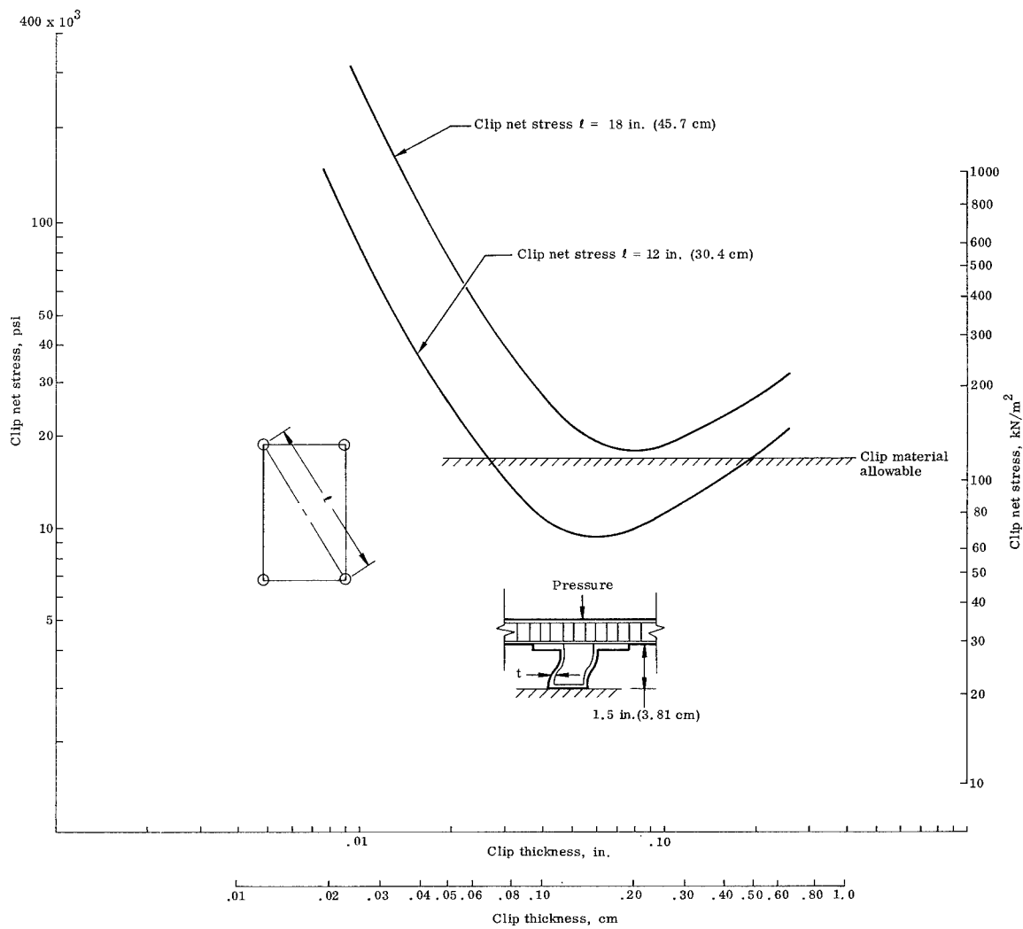
FIGURE 6. FLEXIBLE CLIP STRESSES [PHENOLIC GLASS SUBSTRATE AND CLIP, TEMPERATURE = 1260°R (700°K), PRESSURE = 2.73 psi (18.1 kN/m 2 )]
