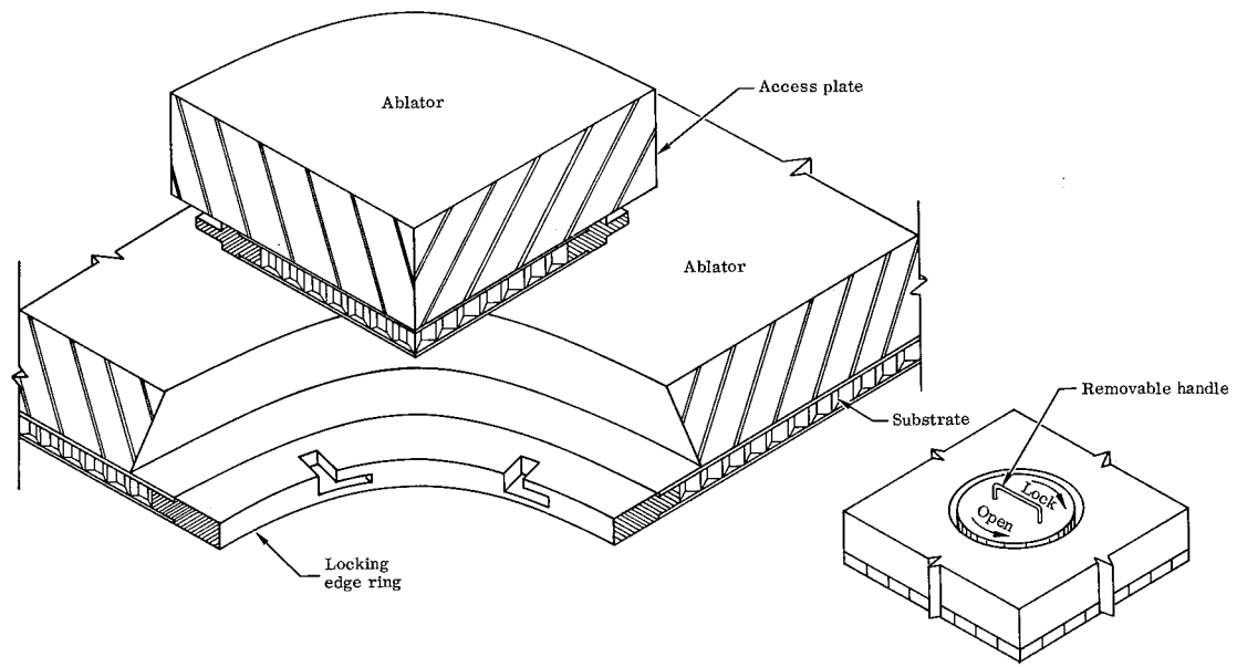
(b). REFURBISHABLE PANEL--ACCESS CONCEPT
