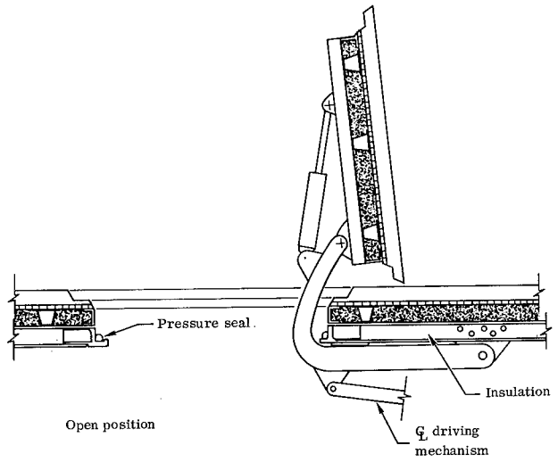
(a). THERMOSTRUCTURAL PANEL IN A HATCH AREA
