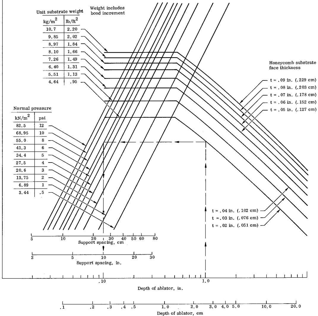
FIGURE 11. REQUIRED SUPPORT SPACING VERSUS PRESSURE [PHENOLIC/GLASS SUBSTRATE PANEL WITH LDNP ABLATOR, PANEL TEMPERATURE = 740°R (411°K)]
