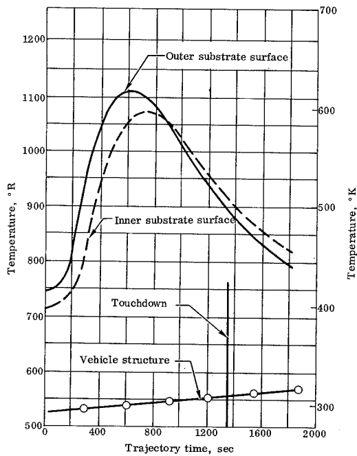
FIGURE 19. TEMPERATURE HISTORY OF CROWN PANEL (UNDERSHOOT TRAJECTORY)
