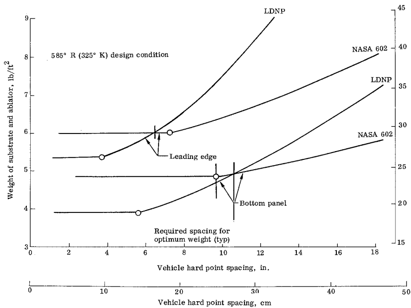
(b). PANEL WEIGHT SENSITIVITY
