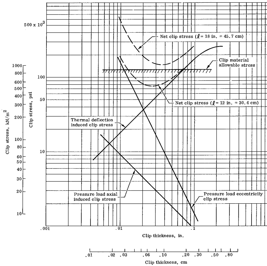
FIGURE 5. FLEXIBLE CLIP STRESSES [(STEEL SUBSTRATE WITH STEEL CLIPS, TEMPERATURE = 1260°R (700°K), PRESSURE = 2.73 psi (18.1 kN/m 2 )]
