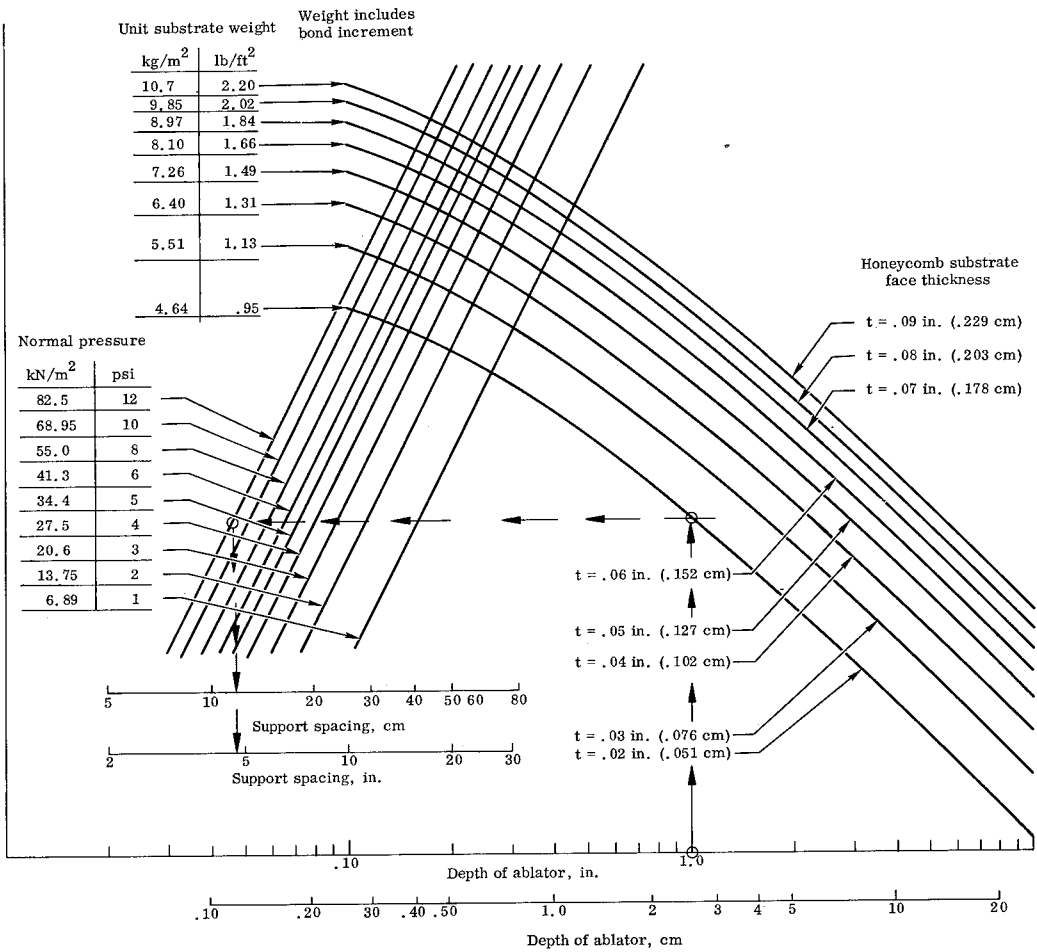
FIGURE 9. REQUIRED SUPPORT SPACING VERSUS PRESSURE [PHENOLIC/GLASS SUBSTRATE PANEL WITH LDNP ABLATOR, PANEL TEMPERATURE = 585° R (325° K)]
