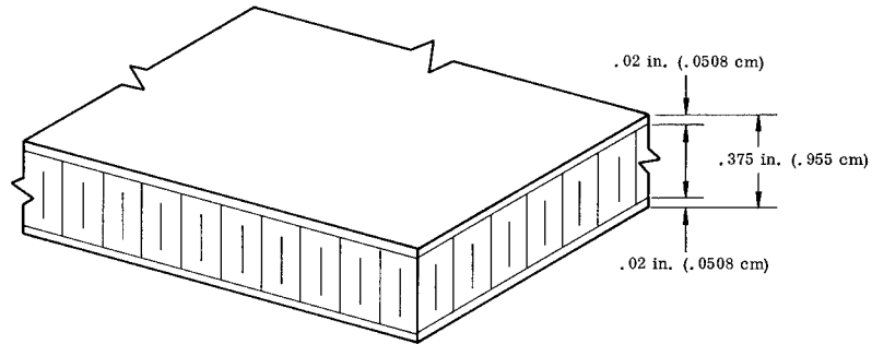
(a) PLASTIC SANDWICH PANEL; PHENOLIC GLASS
