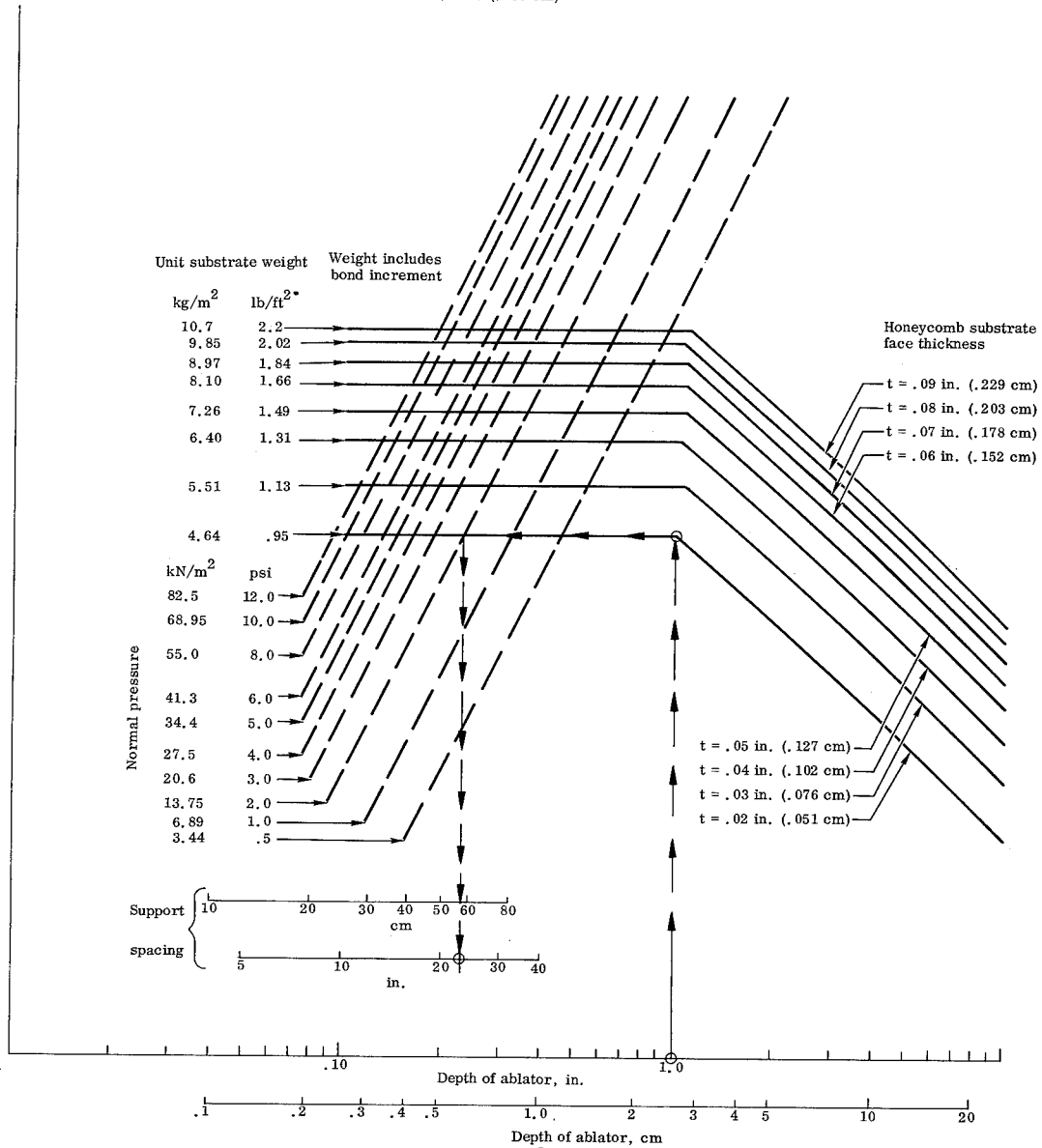
FIGURE 10. REQUIRED SUPPORT SPACING [PHENOLIC/GLASS SUBSTRATE PANEL WITH NASA 602 ABLATOR, PANEL TEMPERATURE = 740°R (411°K), 3/8 in. (.955 cm) DEPTH PANEL]
