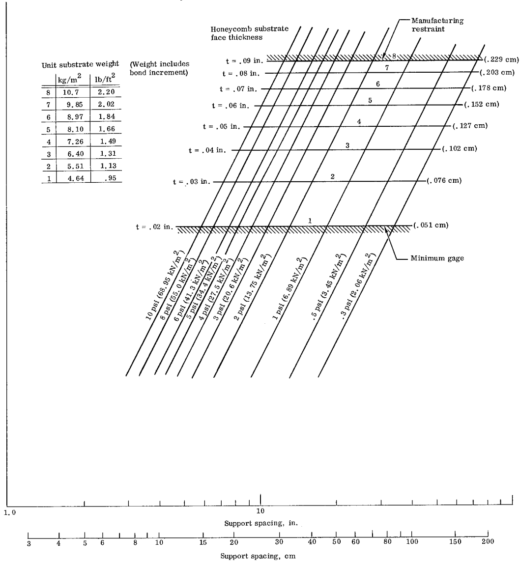
FIGURE 13. REQUIRED SUPPORT SPACING VERSUS PRESSURE FOR NASA 602 OR LDNP ABLATOR [PHENOLIC/GLASS SUBSTRATE PANEL, PANEL TEMPERATURE = 1260° R (700° K)]
