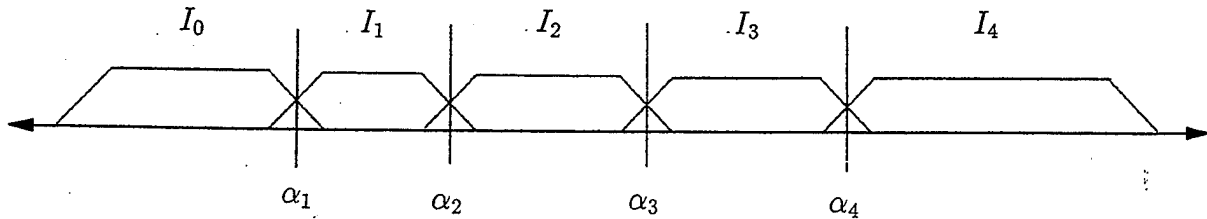
Figure 3.1 Arbitrary Partition of Time into Adjacent Intervals
