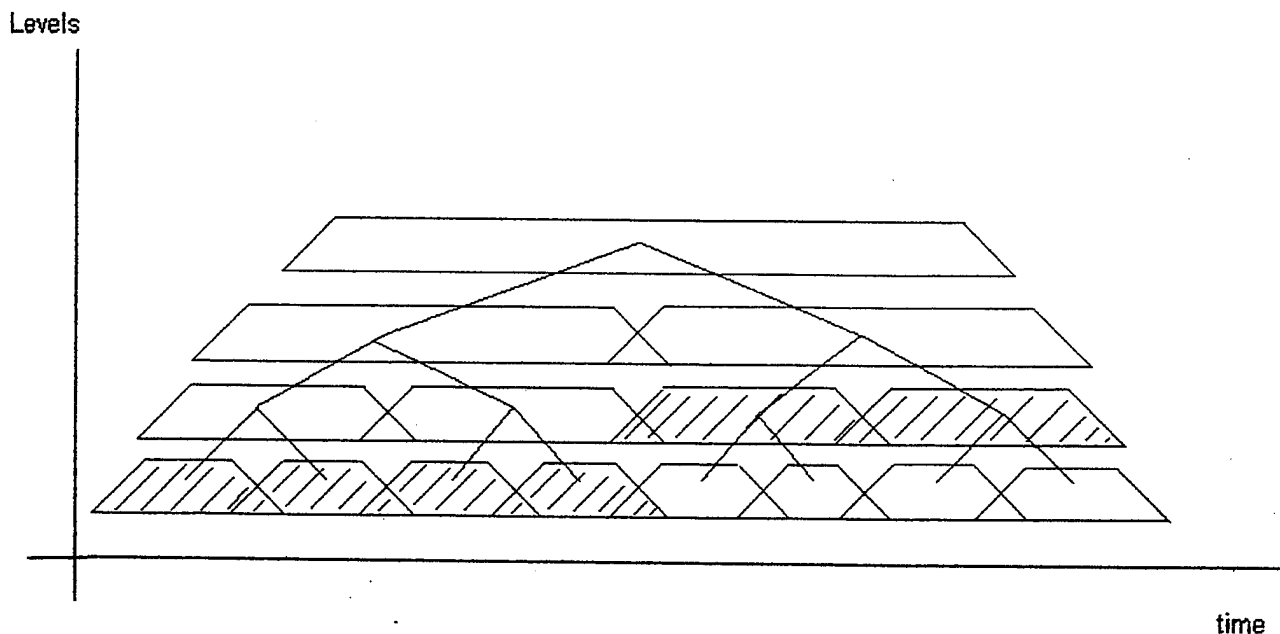
Figure 4.8 Cosine packet transform: The tree configuration
