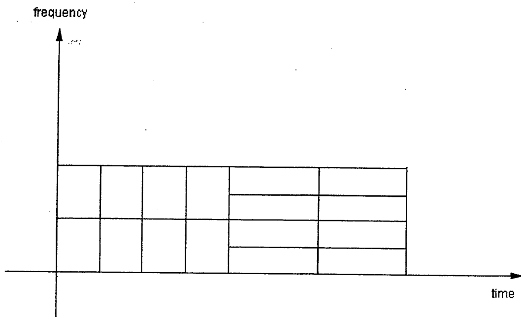
Figure 4.9 Tiling diagram corresponding to Figure 4.8
